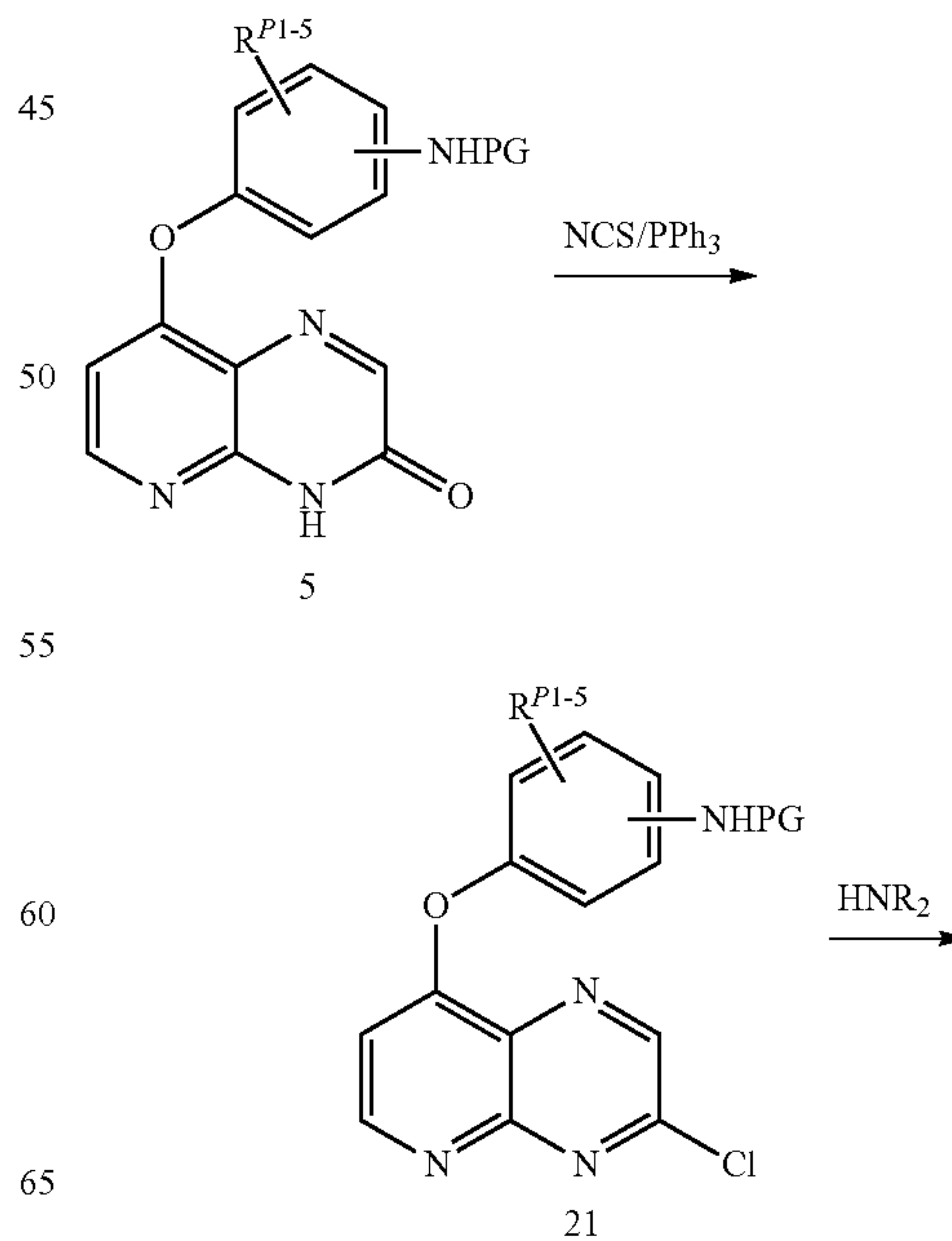
Scheme 6
