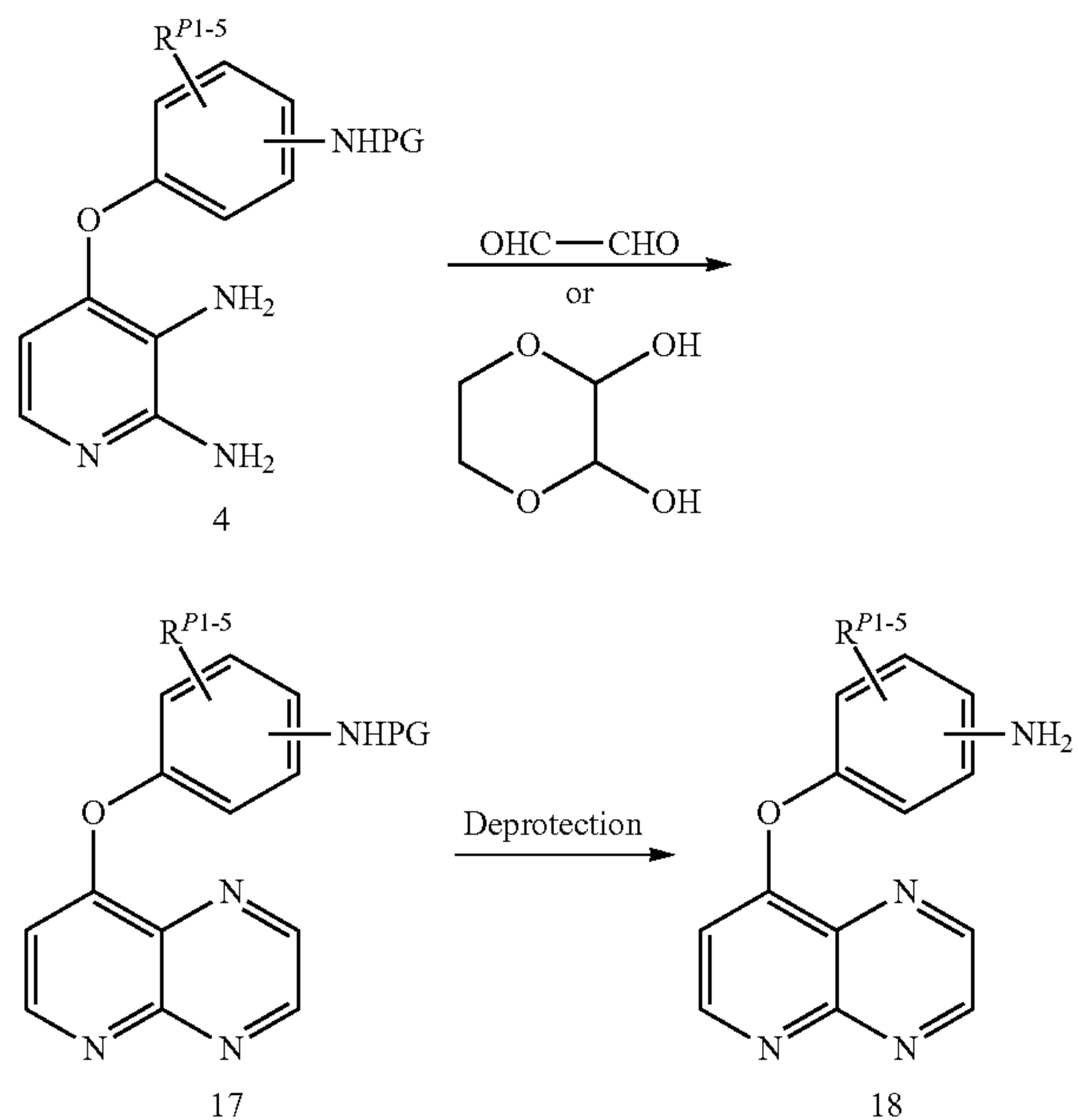
Scheme 4
