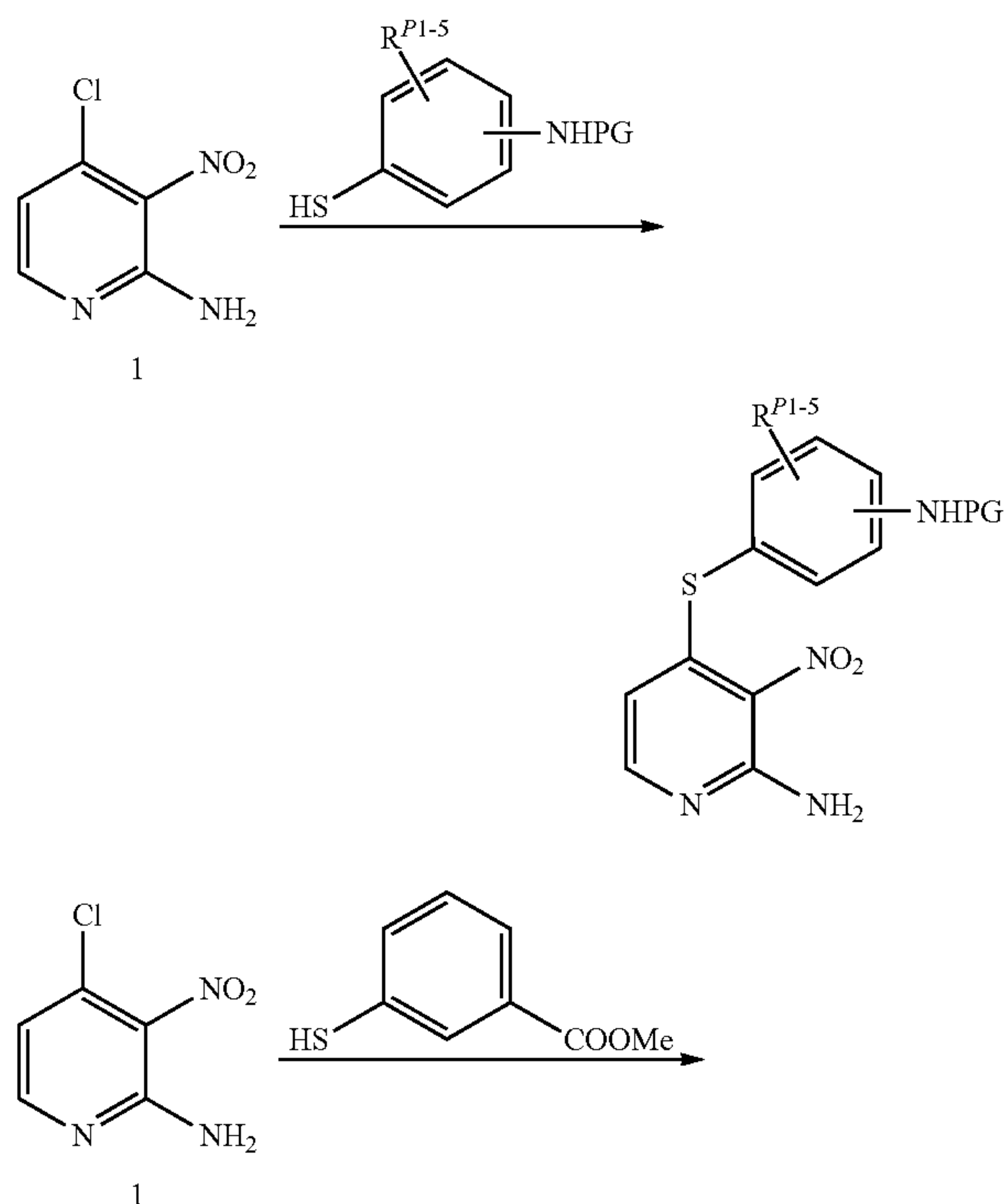
Scheme 11
