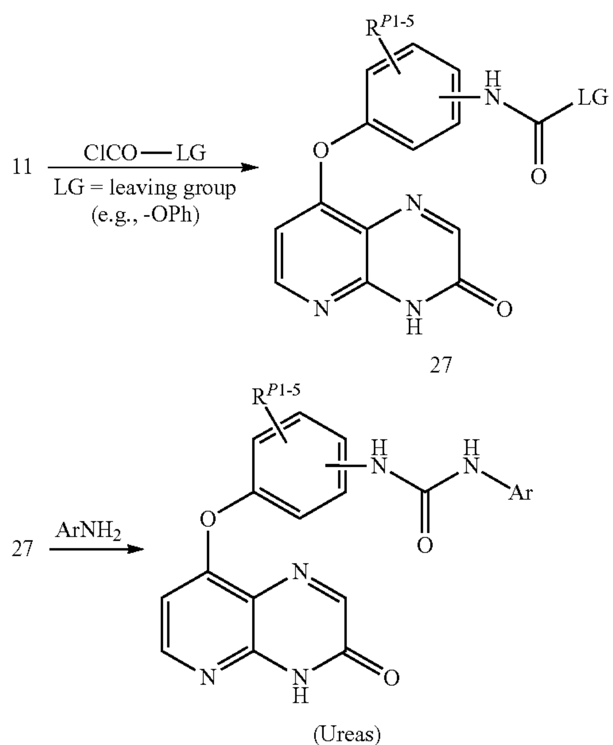
Scheme 8
