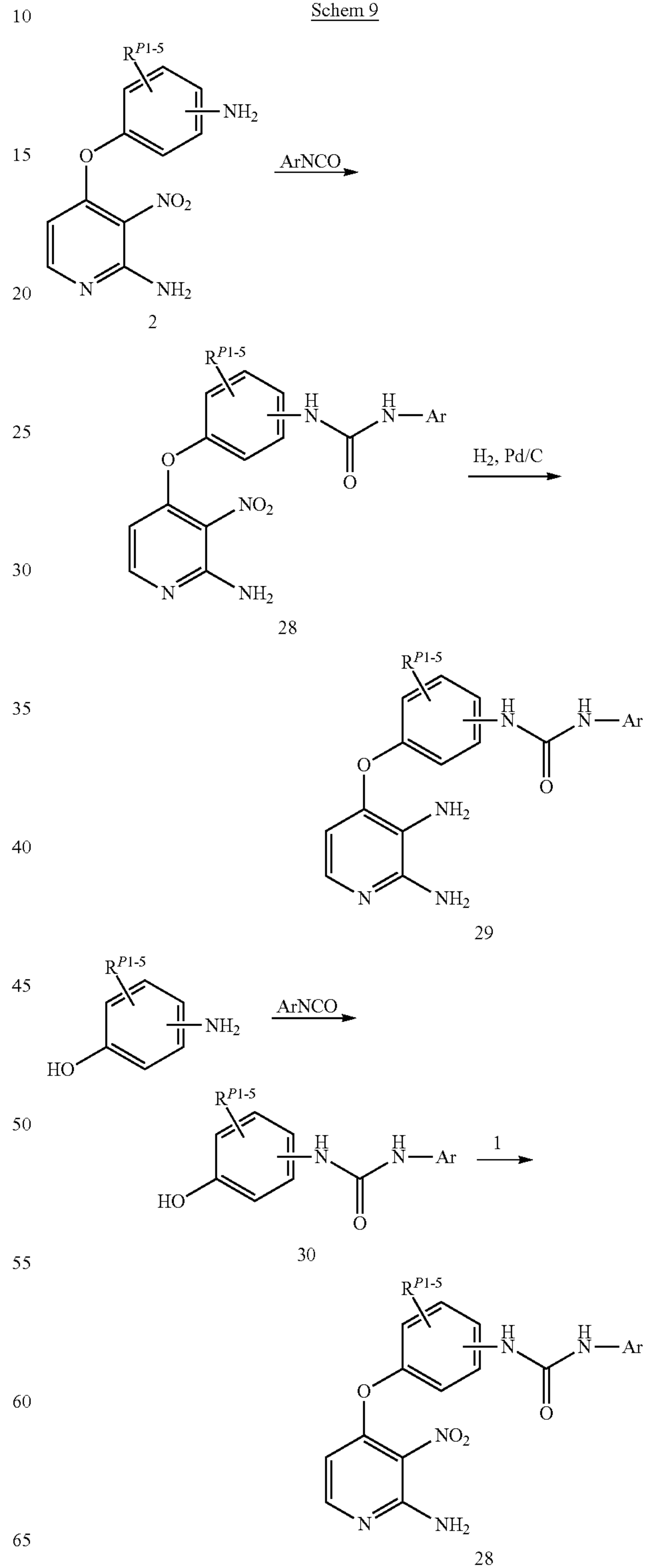
Scheme 9
