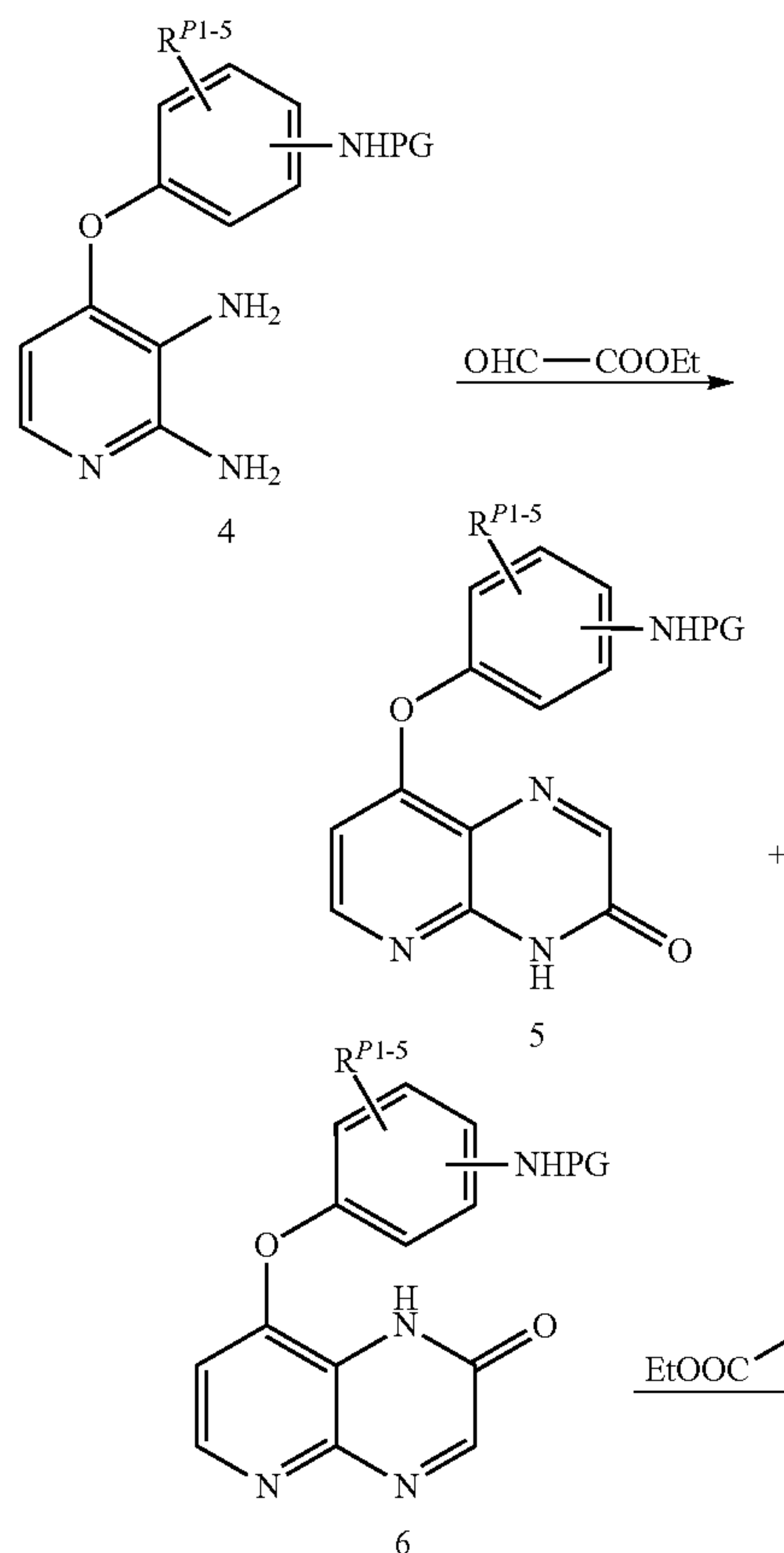
Scheme 2
