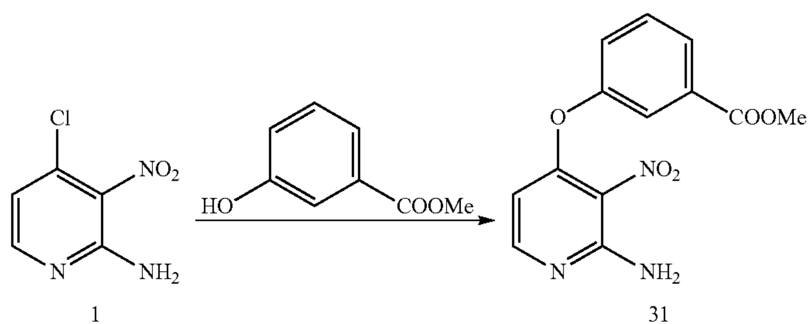
Scheme 10
