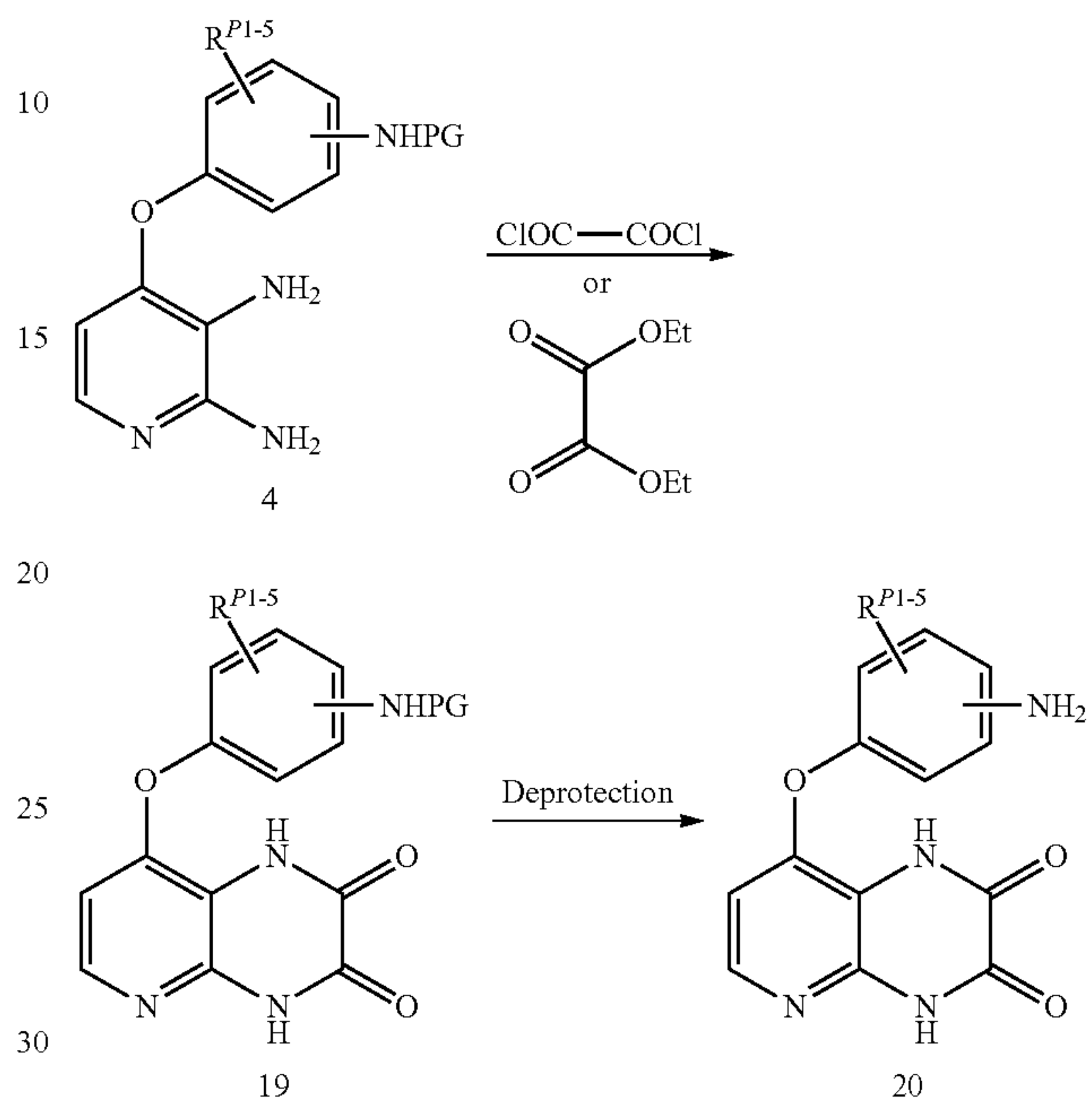
Scheme 5
