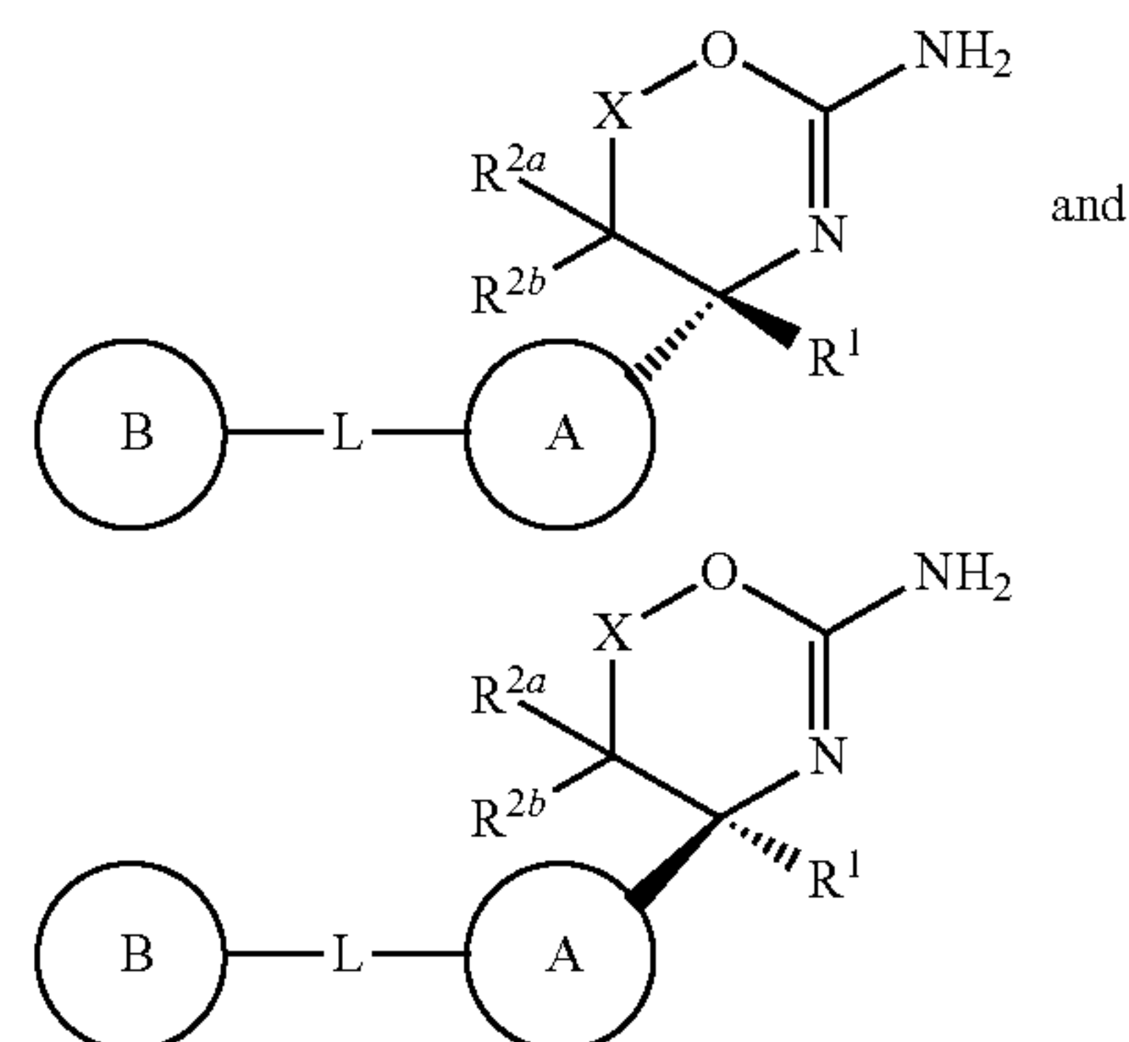
[Chemical Formula 78]
