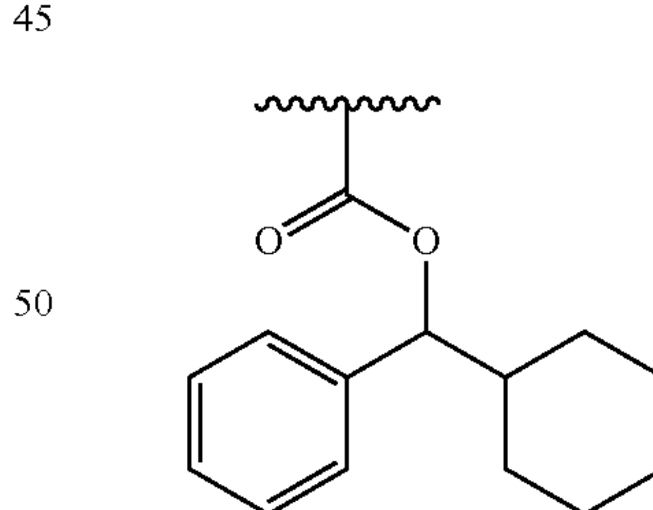
[Chemical Formula 34]
