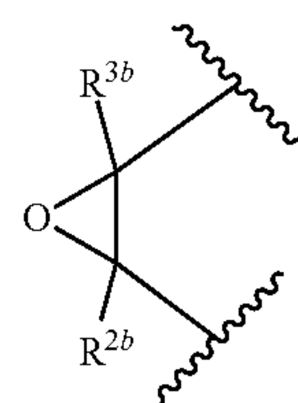
[Chemical Formula 8]
