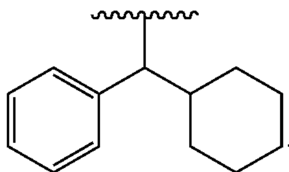
[Chemical Formula 26]
