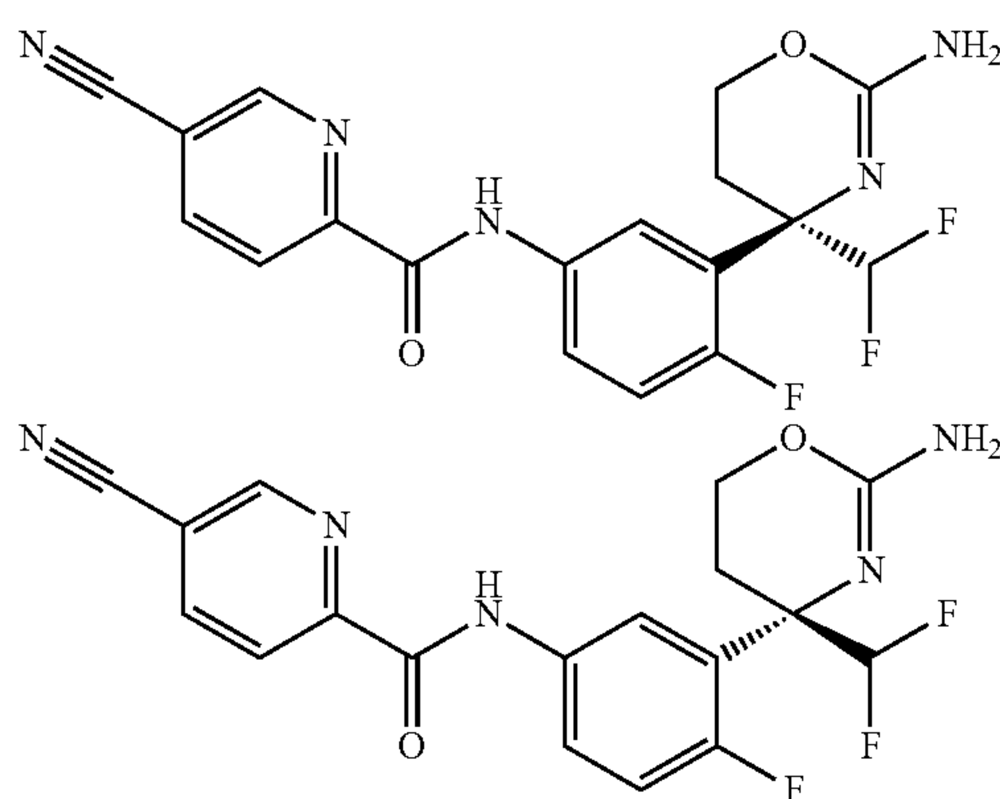
[Chemical Formula 17]
