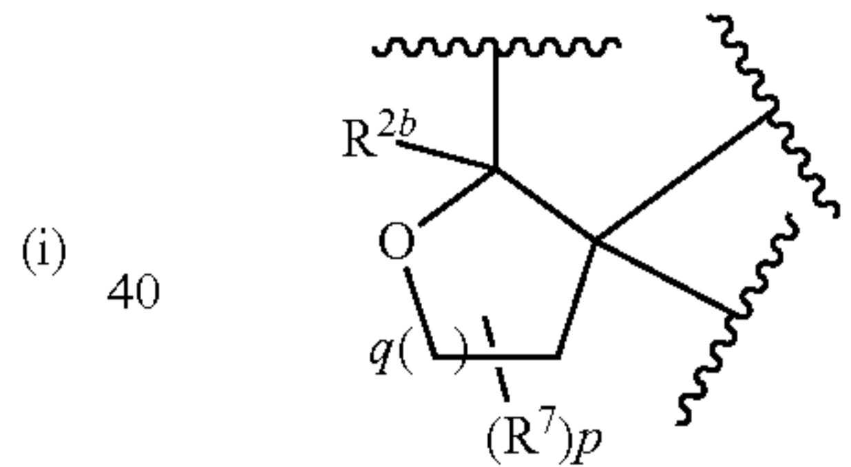
[Chemical Formula 4]
