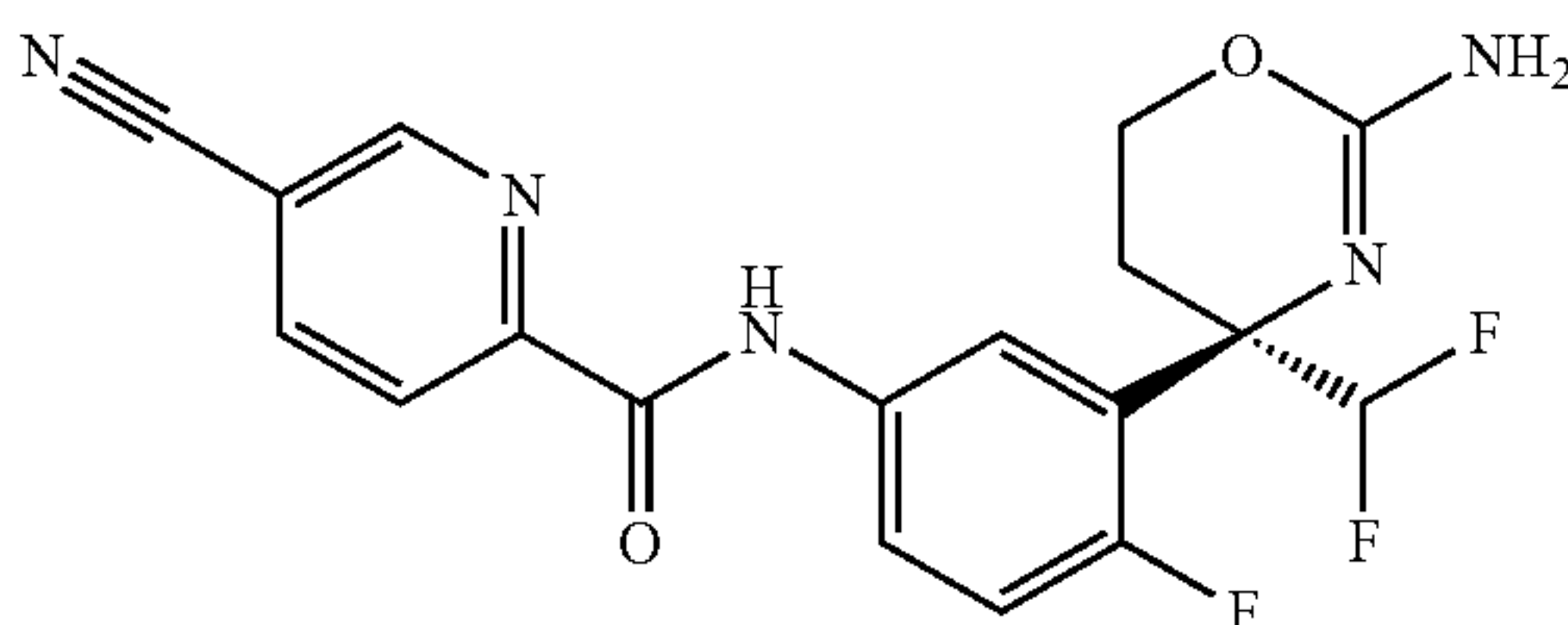
[Chemical Formula 76]
