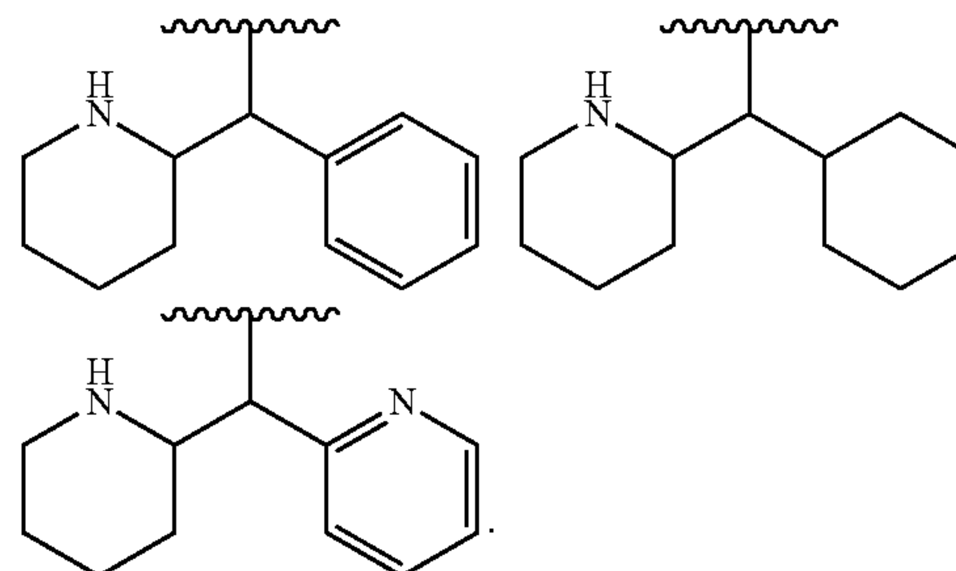
[Chemical Formula 28]
