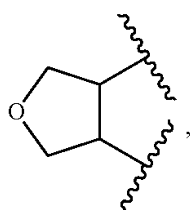
[Chemical Formula 75]
