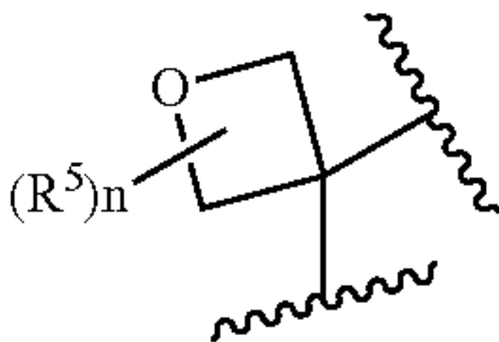
[Chemical Formula 44]
