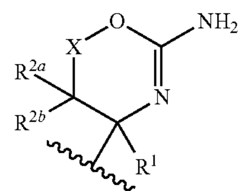
[Chemical Formula 52]
