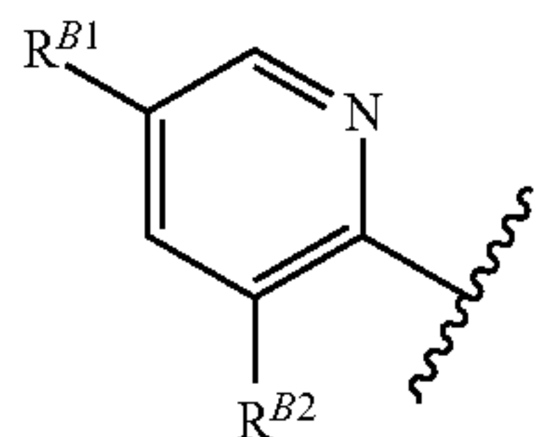
[Chemical Formula 56]
