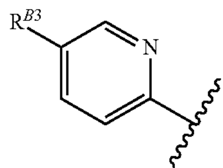
[Chemical Formula 58]
