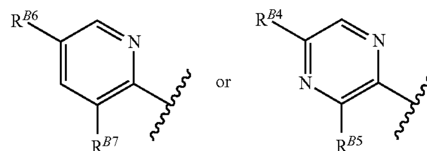
[Chemical Formula 10]
