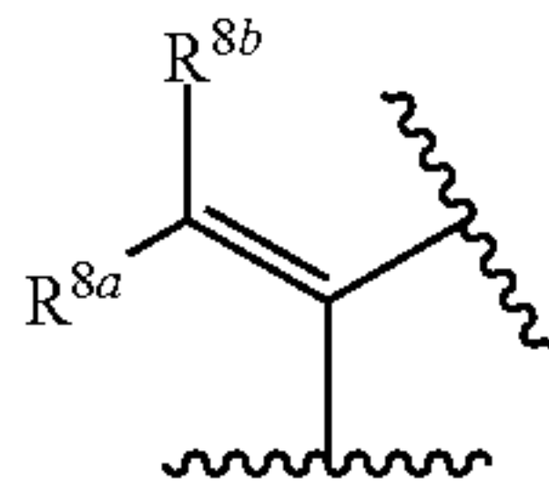
[Chemical Formula 48]
