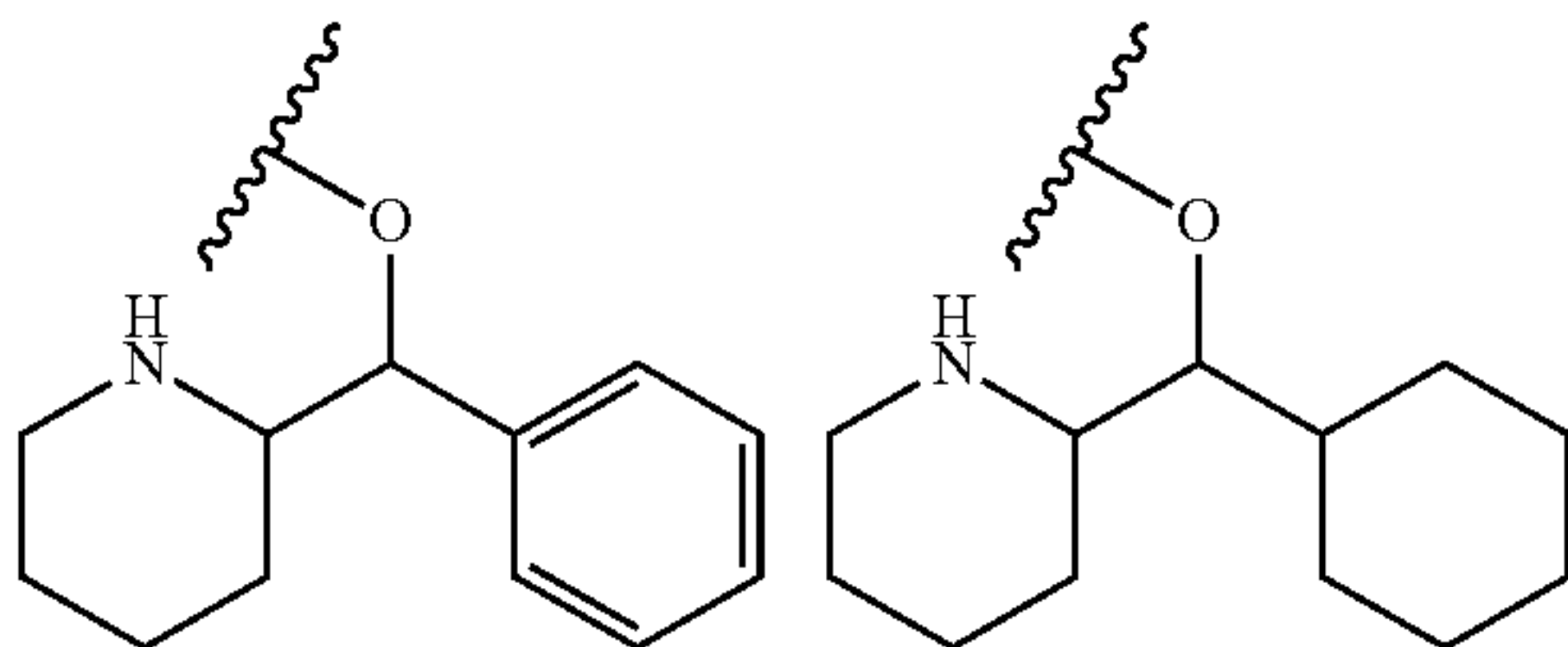
[Chemical Formula 32]
