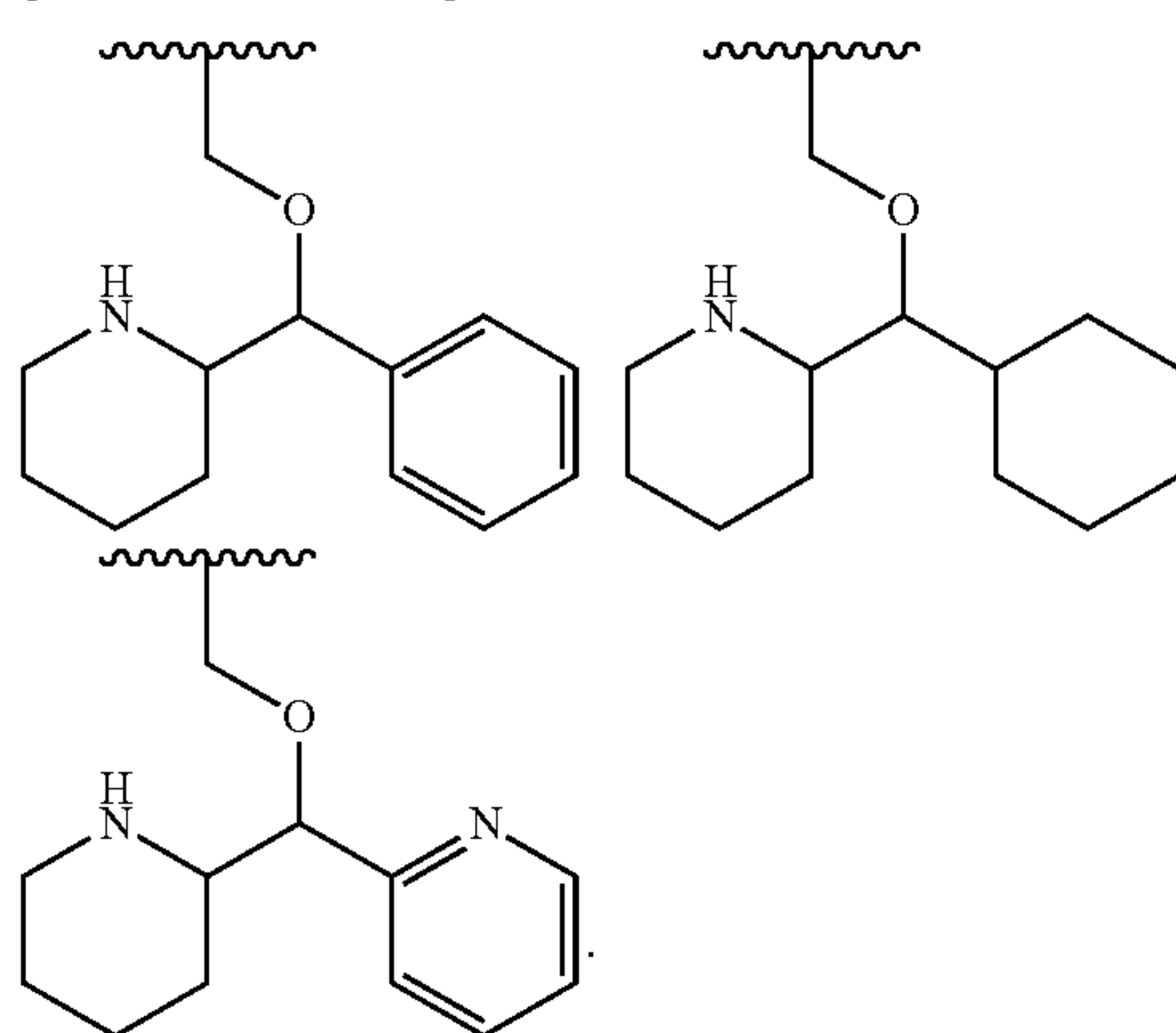
[Chemical Formula 40]
