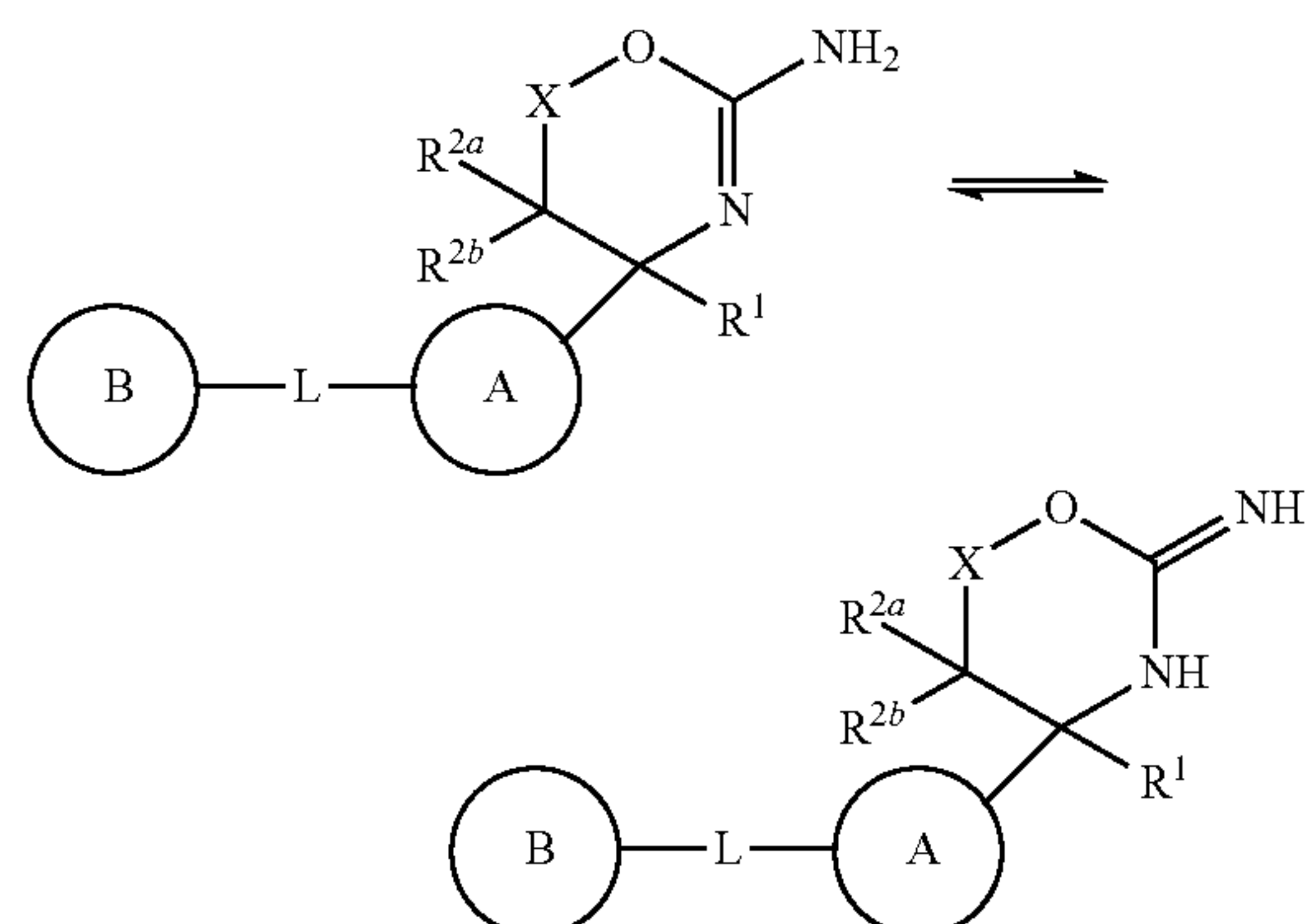
[Chemical Formula 77]
