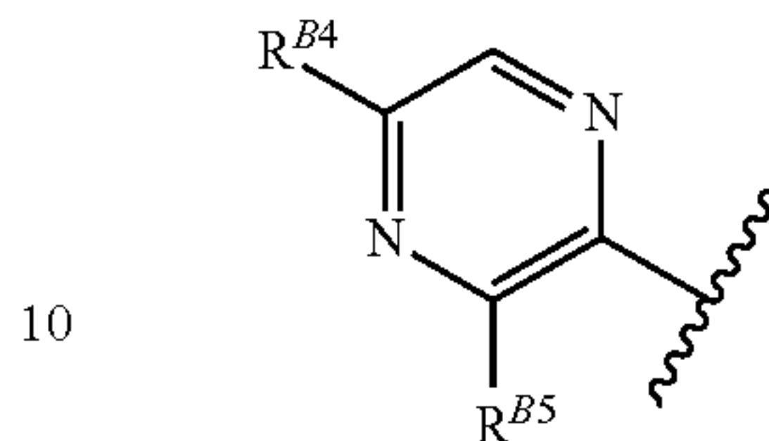
5 [Chemical Formula 61]
