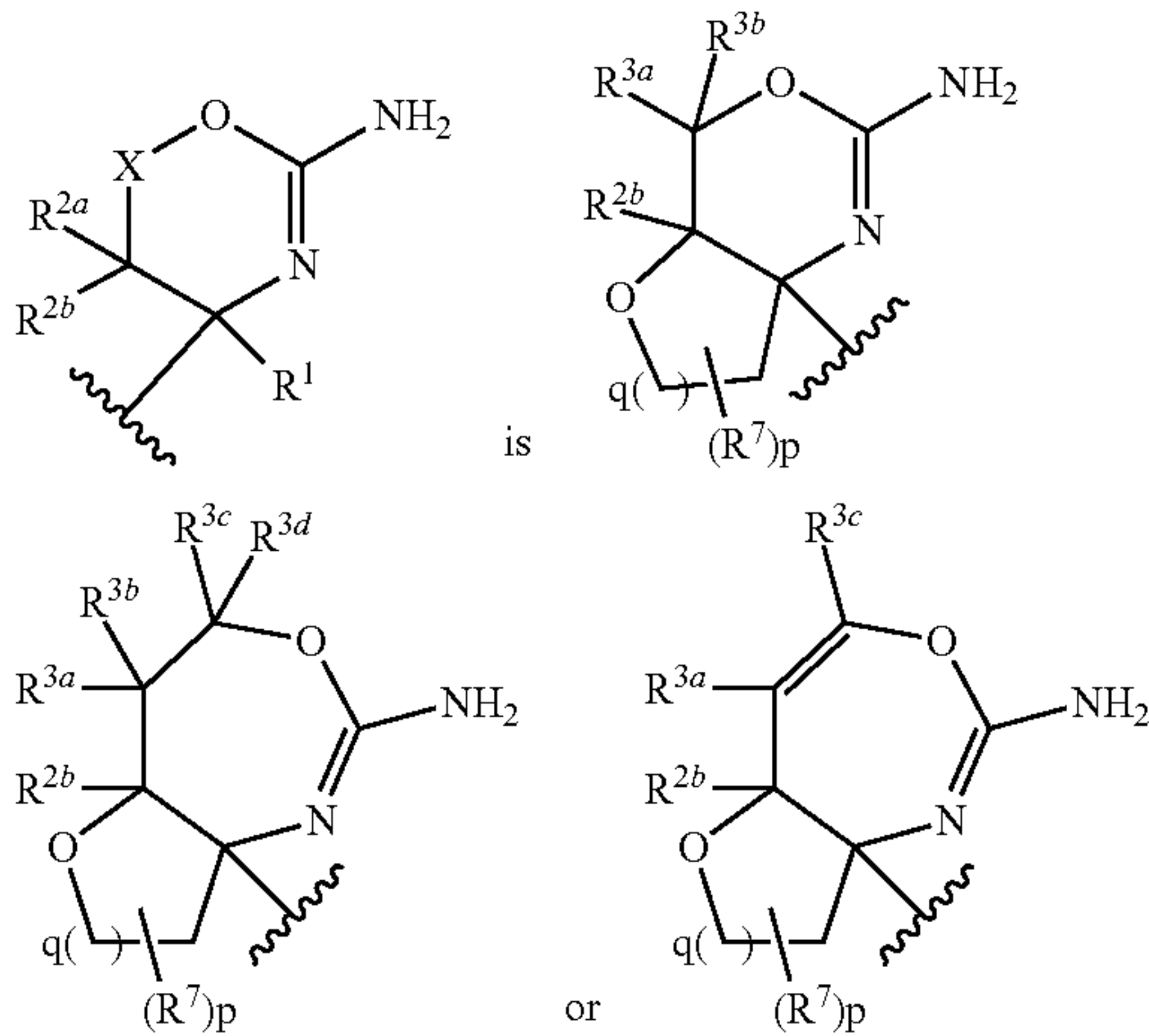
[Chemical Formula 47]
