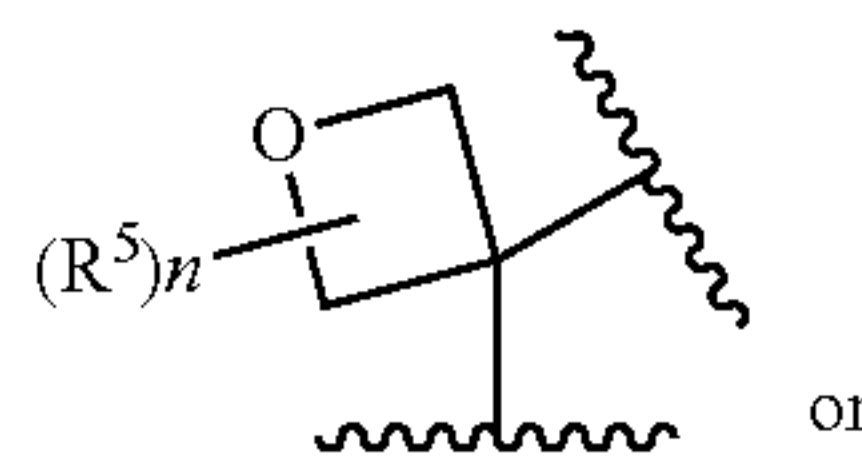
[Chemical Formula 3]
