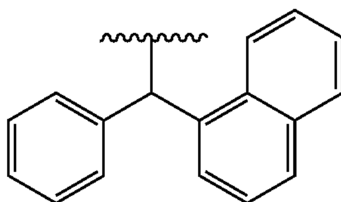
[Chemical Formula 25]
