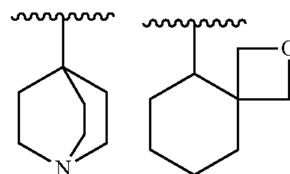
[Chemical Formula 24]
