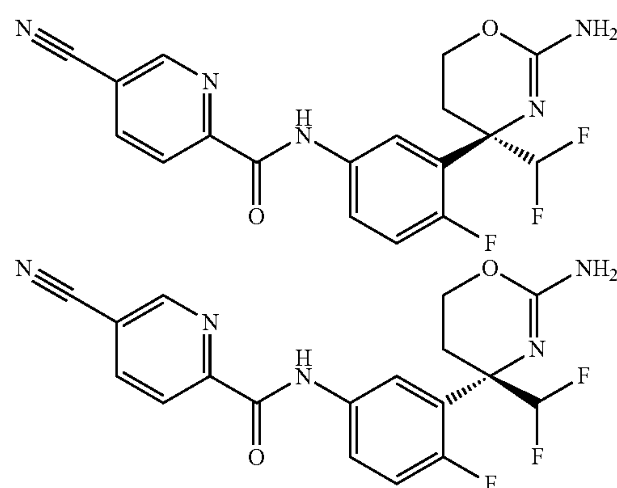
[Chemical Formula 15]
