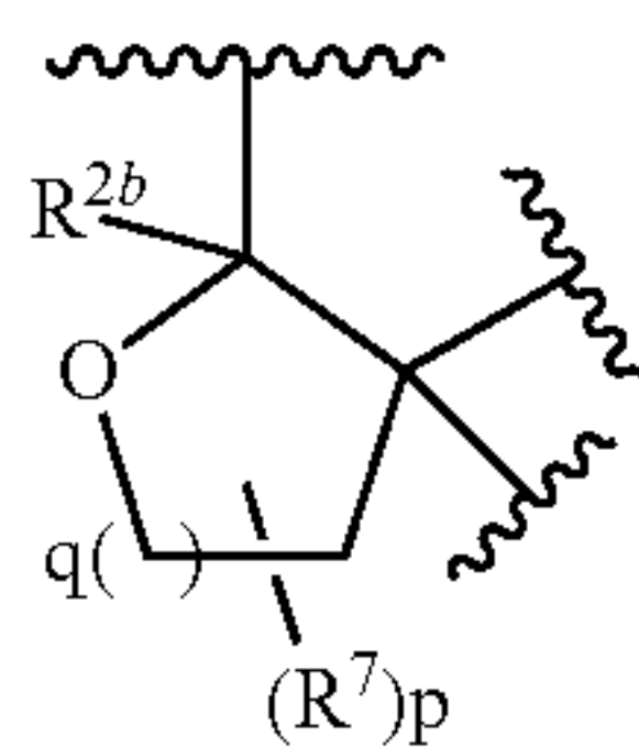
[Chemical Formula 46]
