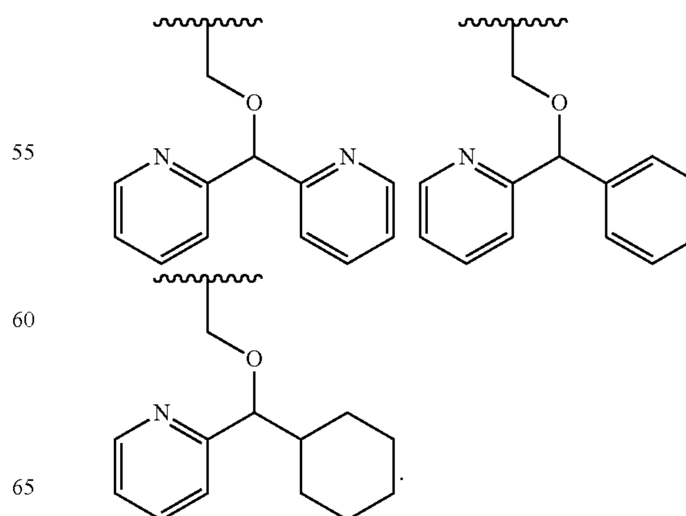
[Chemical Formula 39]
