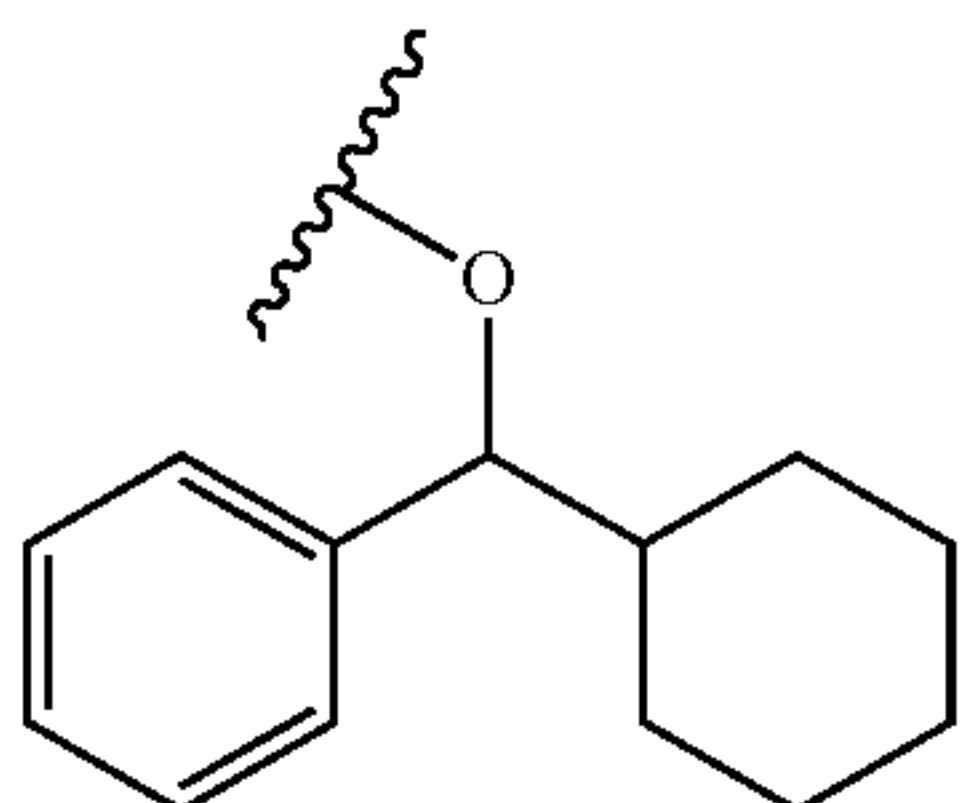
[Chemical Formula 30]
