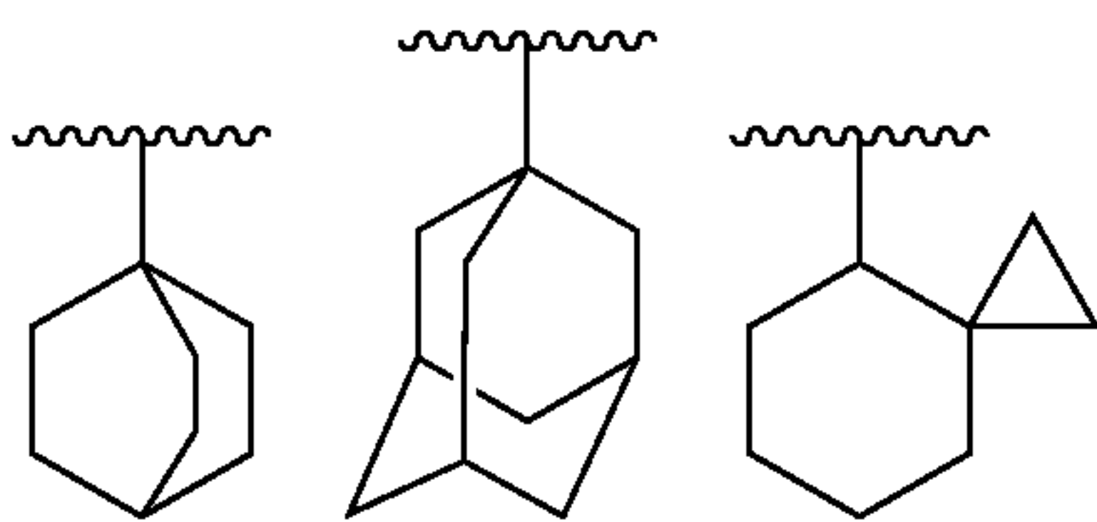
[Chemical Formula 23]
