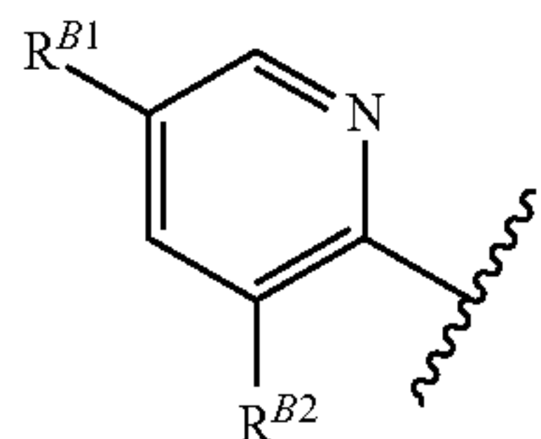
[Chemical Formula 57]
