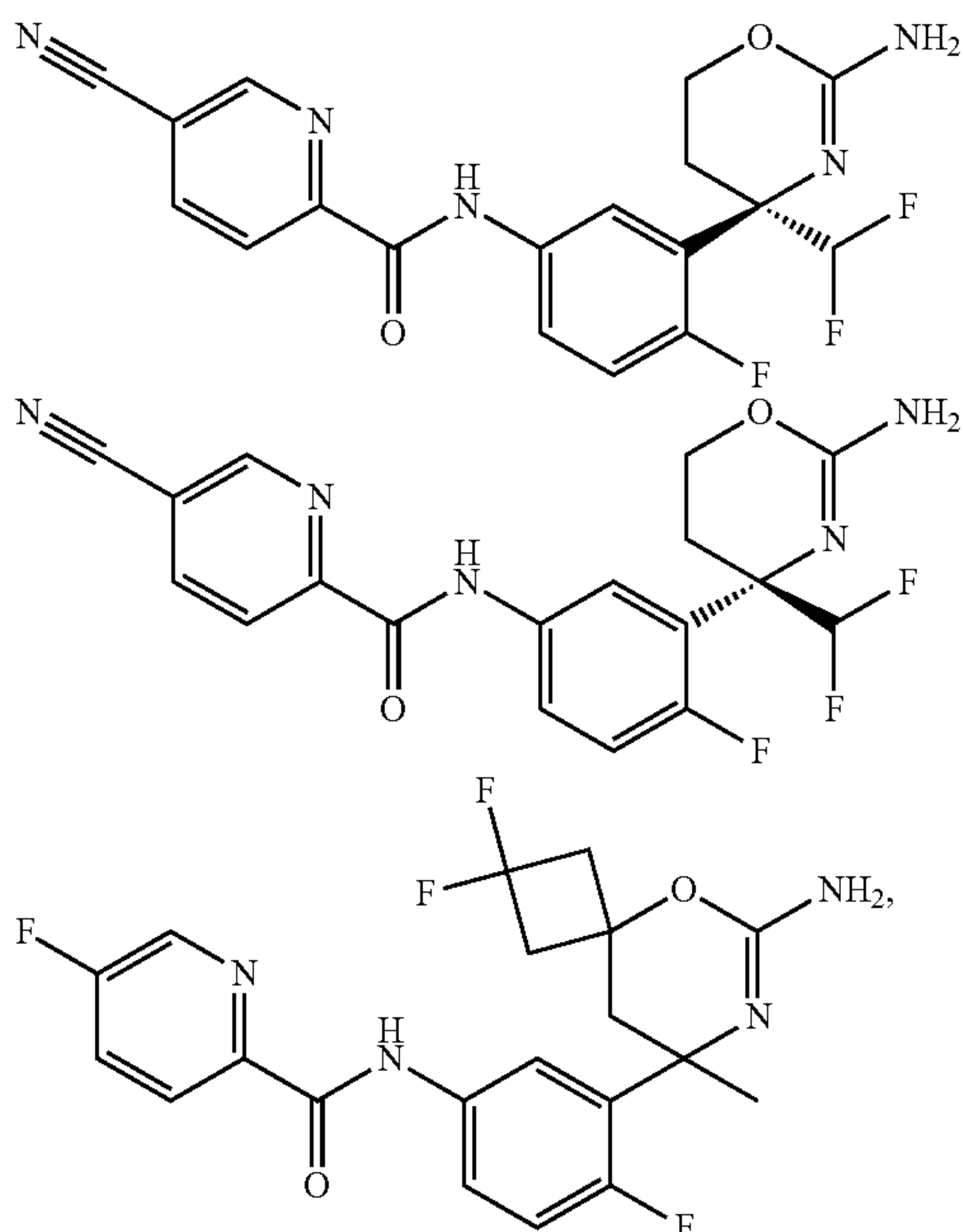
[Chemical Formula 6]
