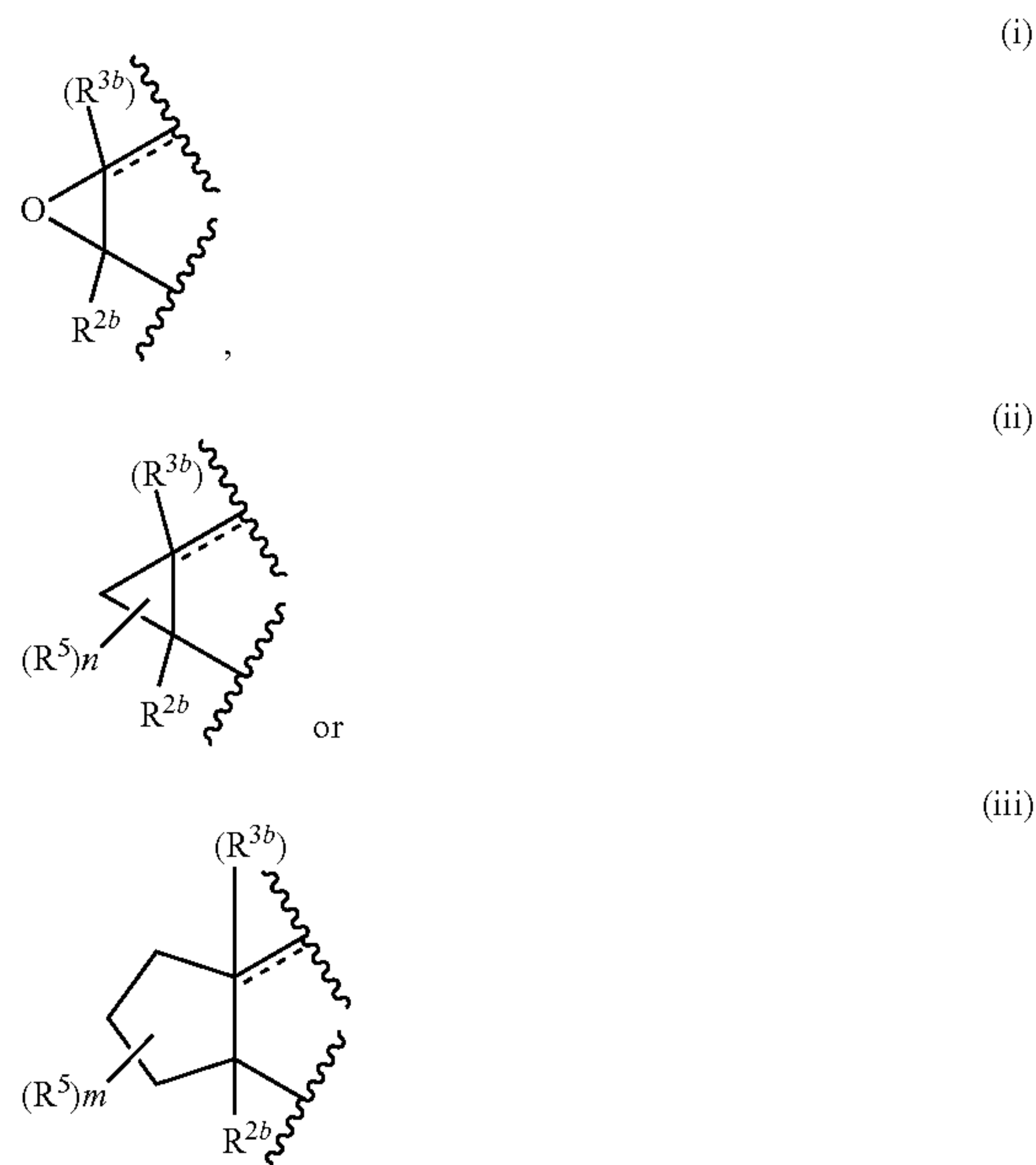
[Chemical Formula 68]
