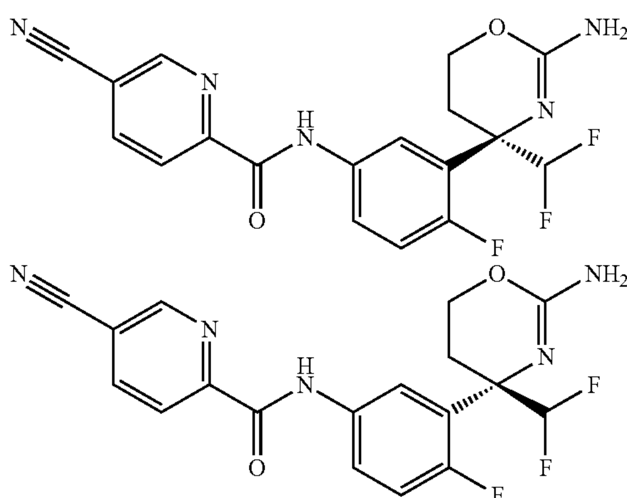
[Chemical Formula 13]
