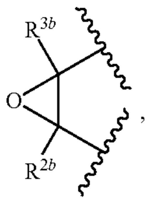
[Chemical Formula 2]
