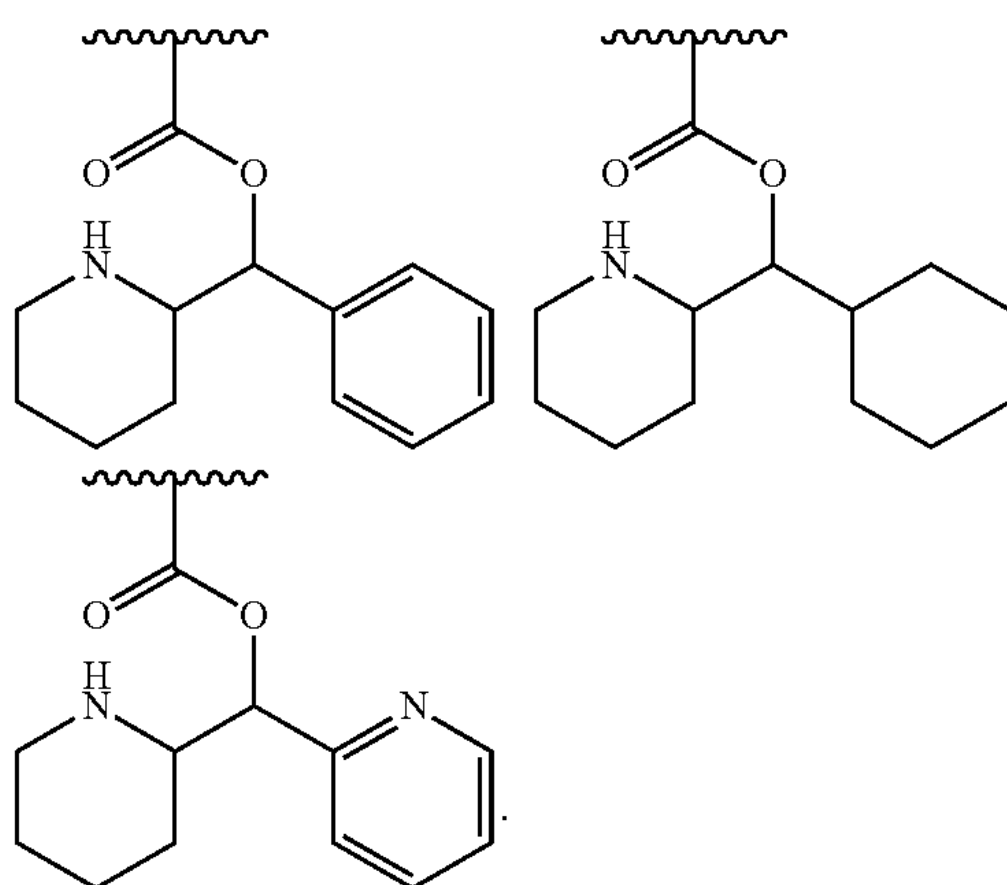
[Chemical Formula 36]
