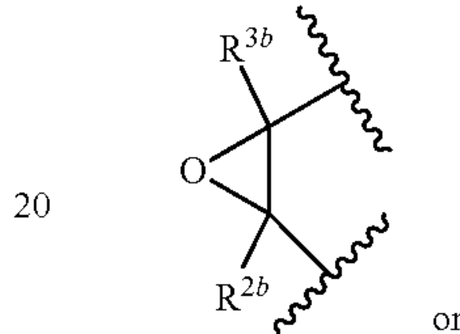
[Chemical Formula 18]
