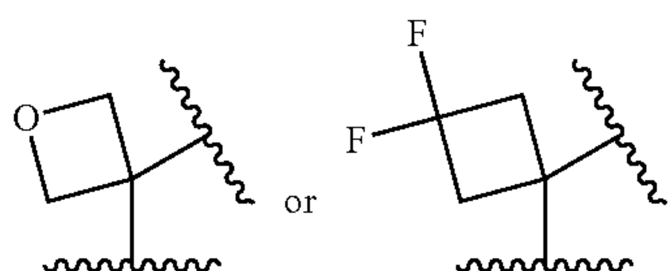
[Chemical Formula 74]
