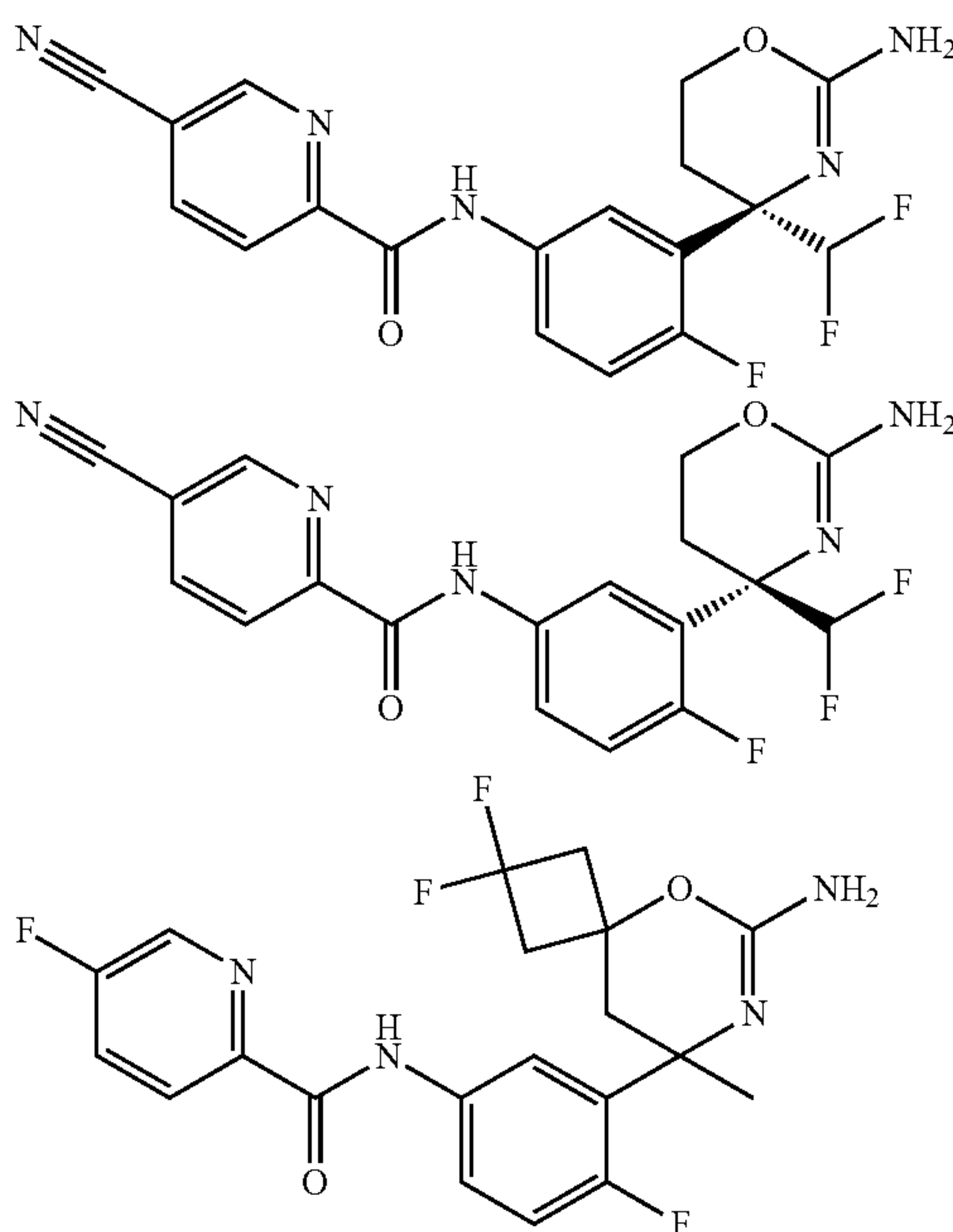
[Chemical Formula 14]
