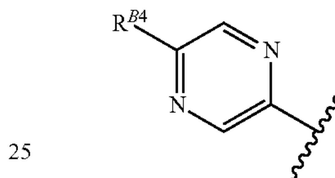
20 [Chemical Formula 62]
