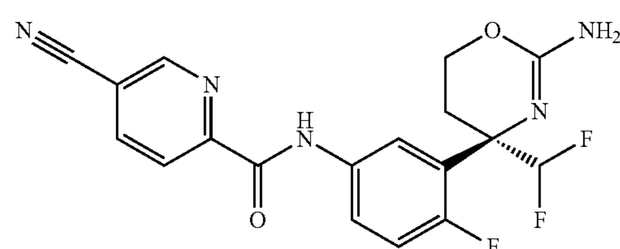
[Chemical Formula 16]
