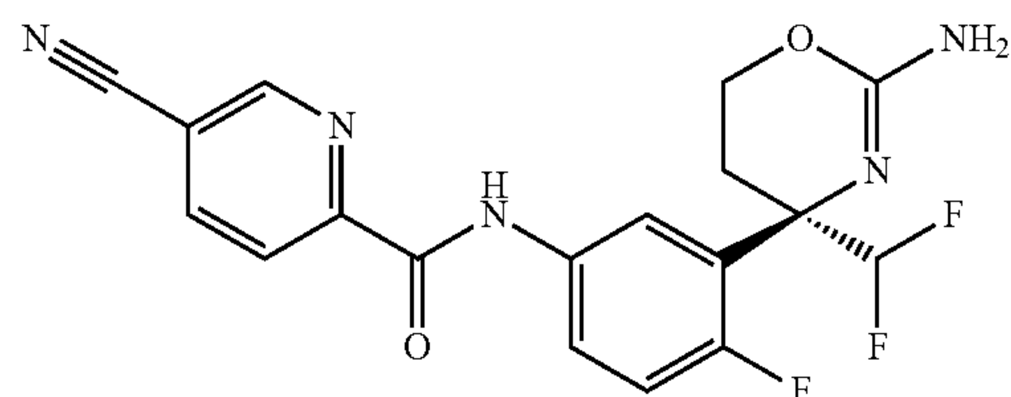
[Chemical Formula 9]
