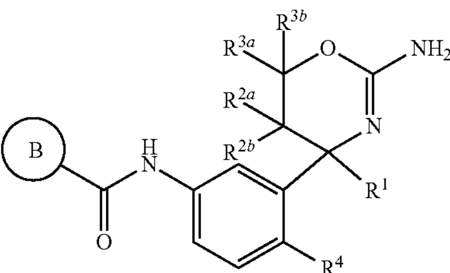
[Chemical Formula 50]
