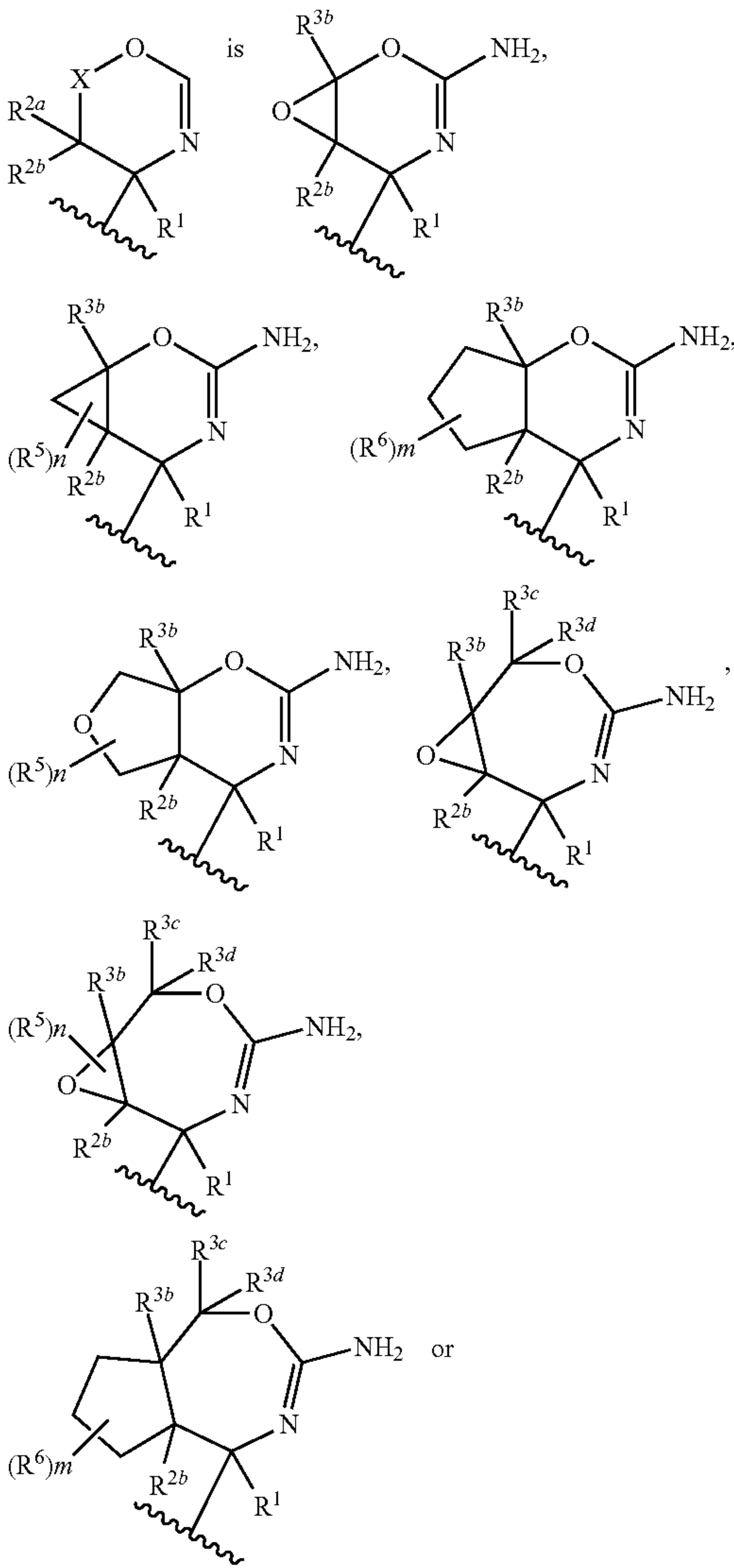
[Chemical Formula 43]
