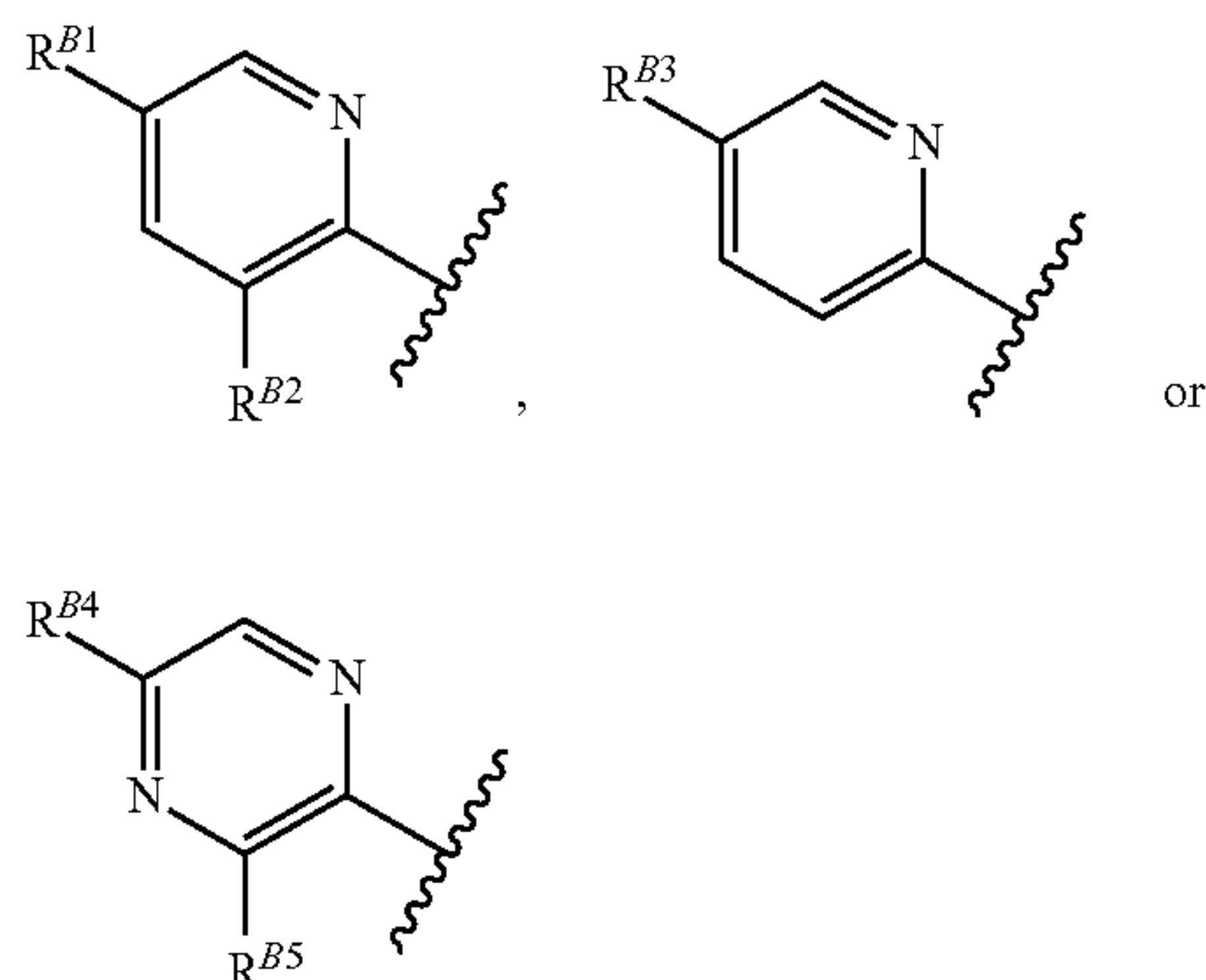
[Chemical Formula 19]
