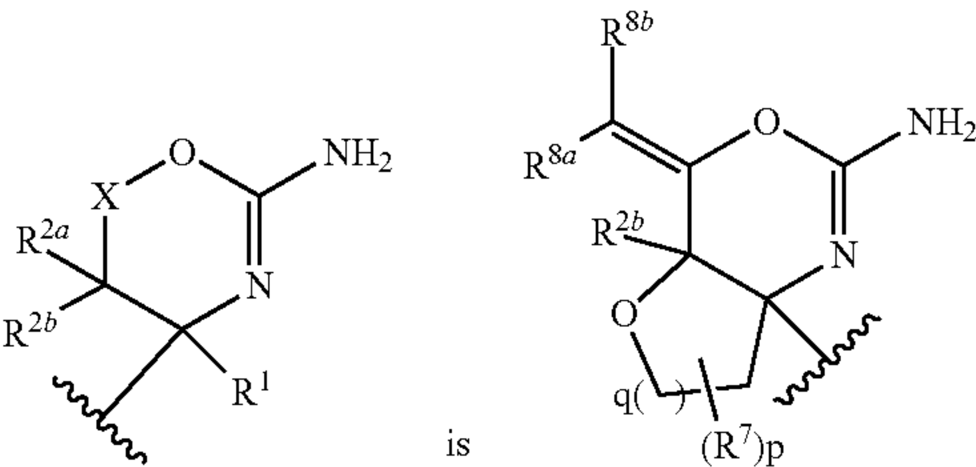
[Chemical Formula 49]
