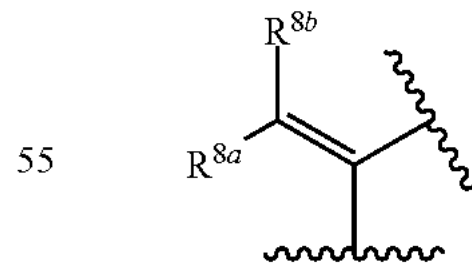
[Chemical Formula 5]
