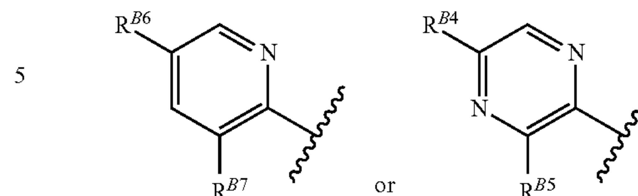
[Chemical Formula 21]
