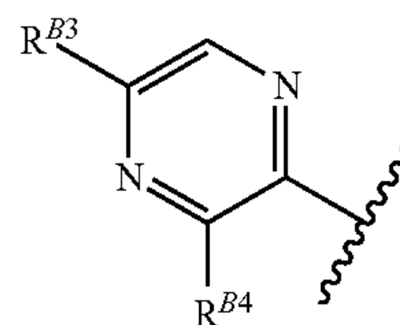
[Chemical Formula 66]
