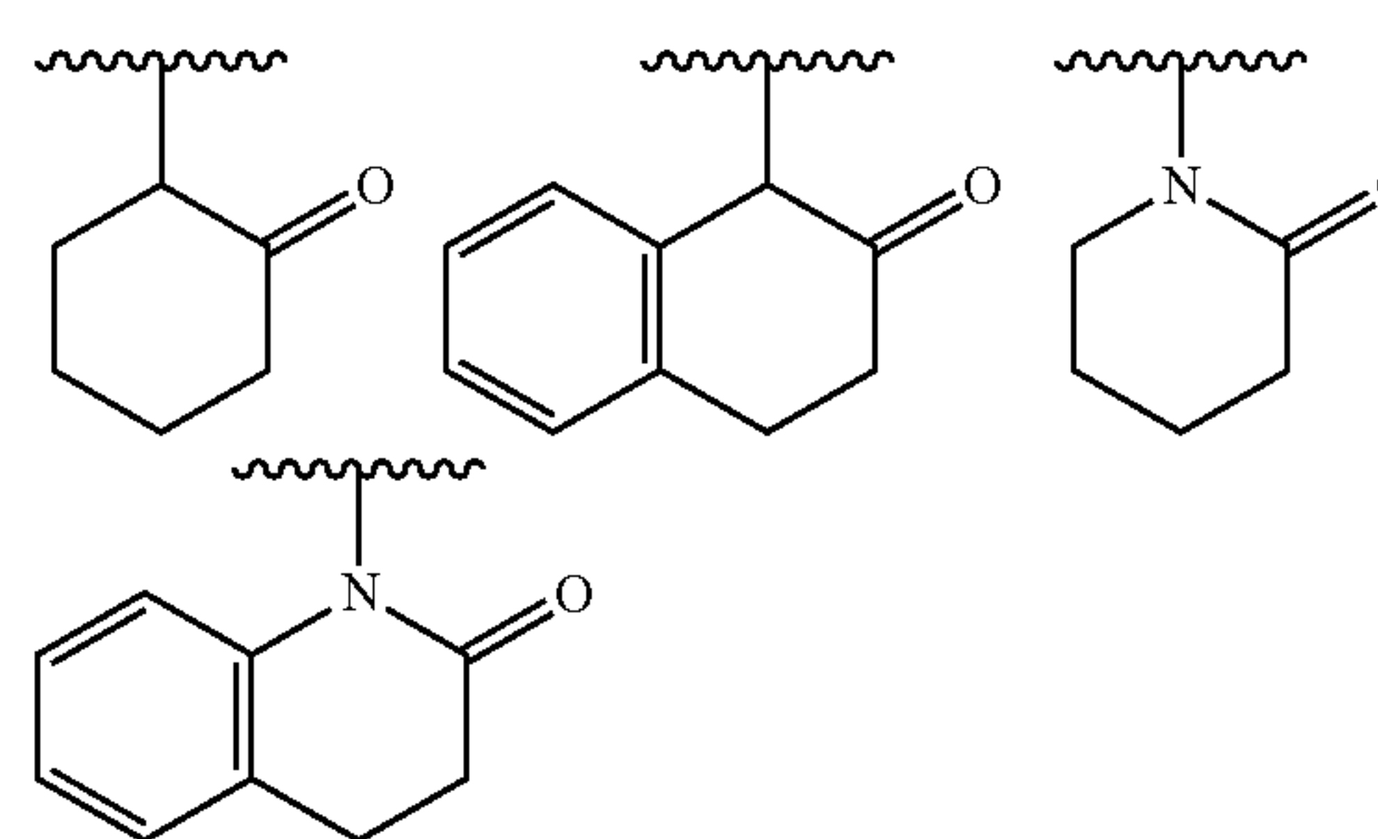
[Chemical Formula 41]
