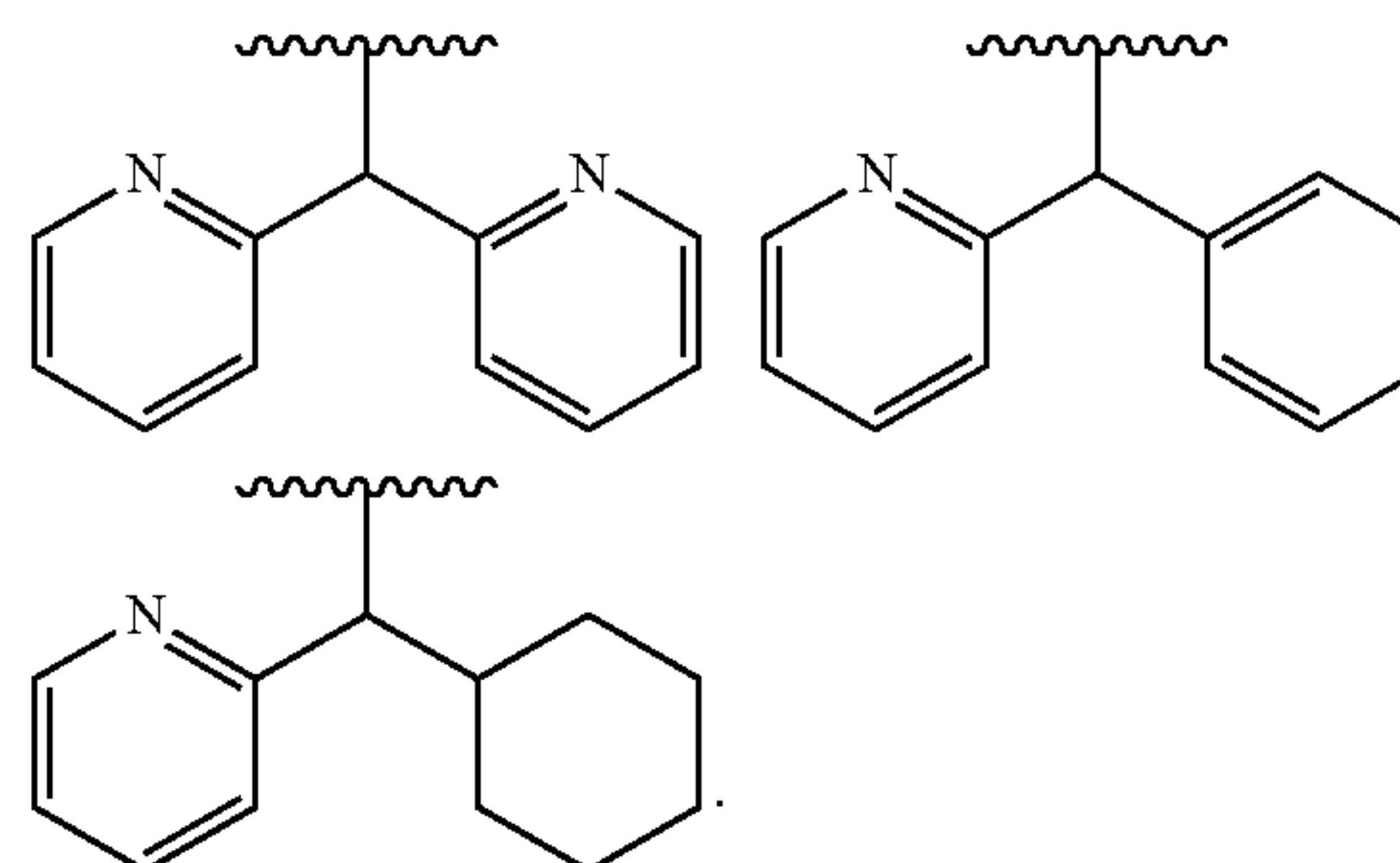
[Chemical Formula 27]
