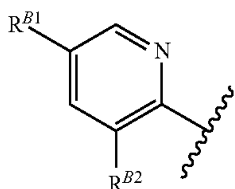
[Chemical Formula 63]
