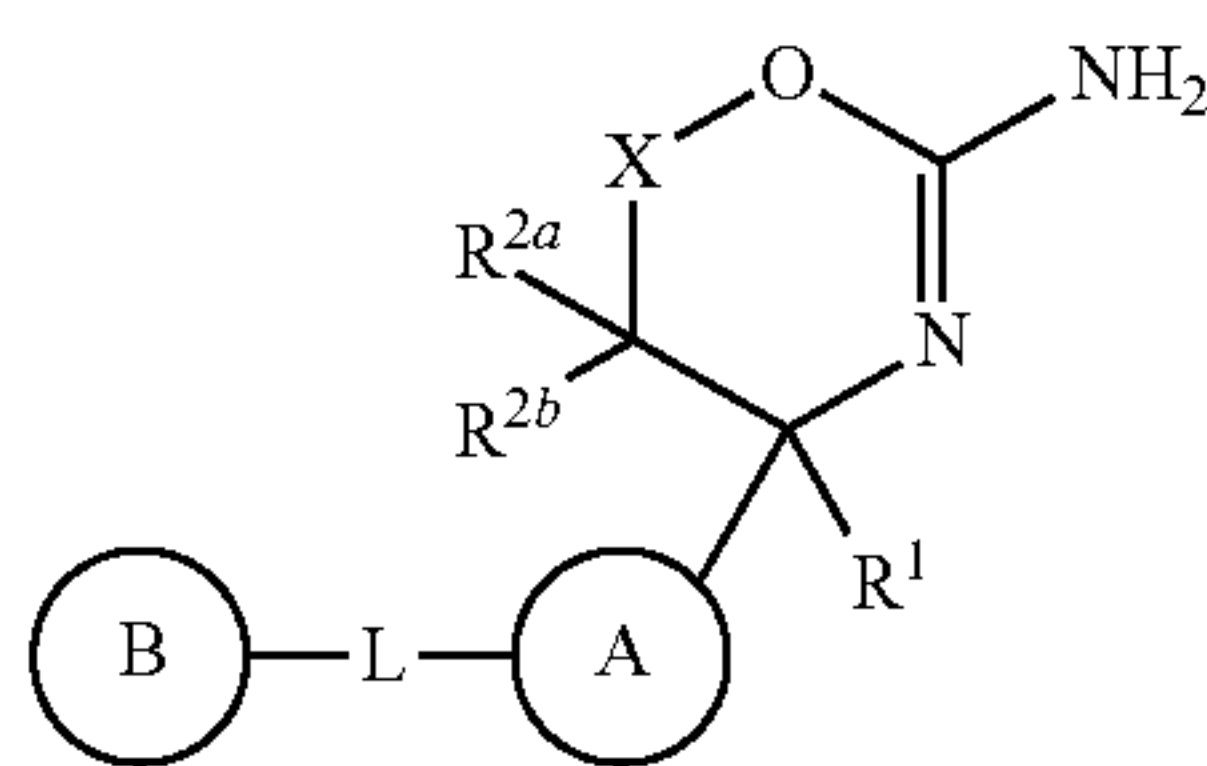
[Chemical Formula 7]
