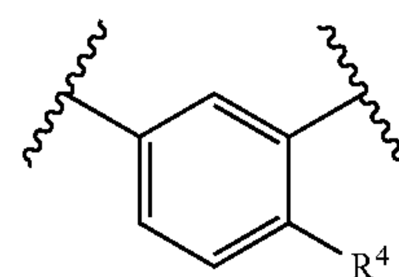
[Chemical Formula 11]
