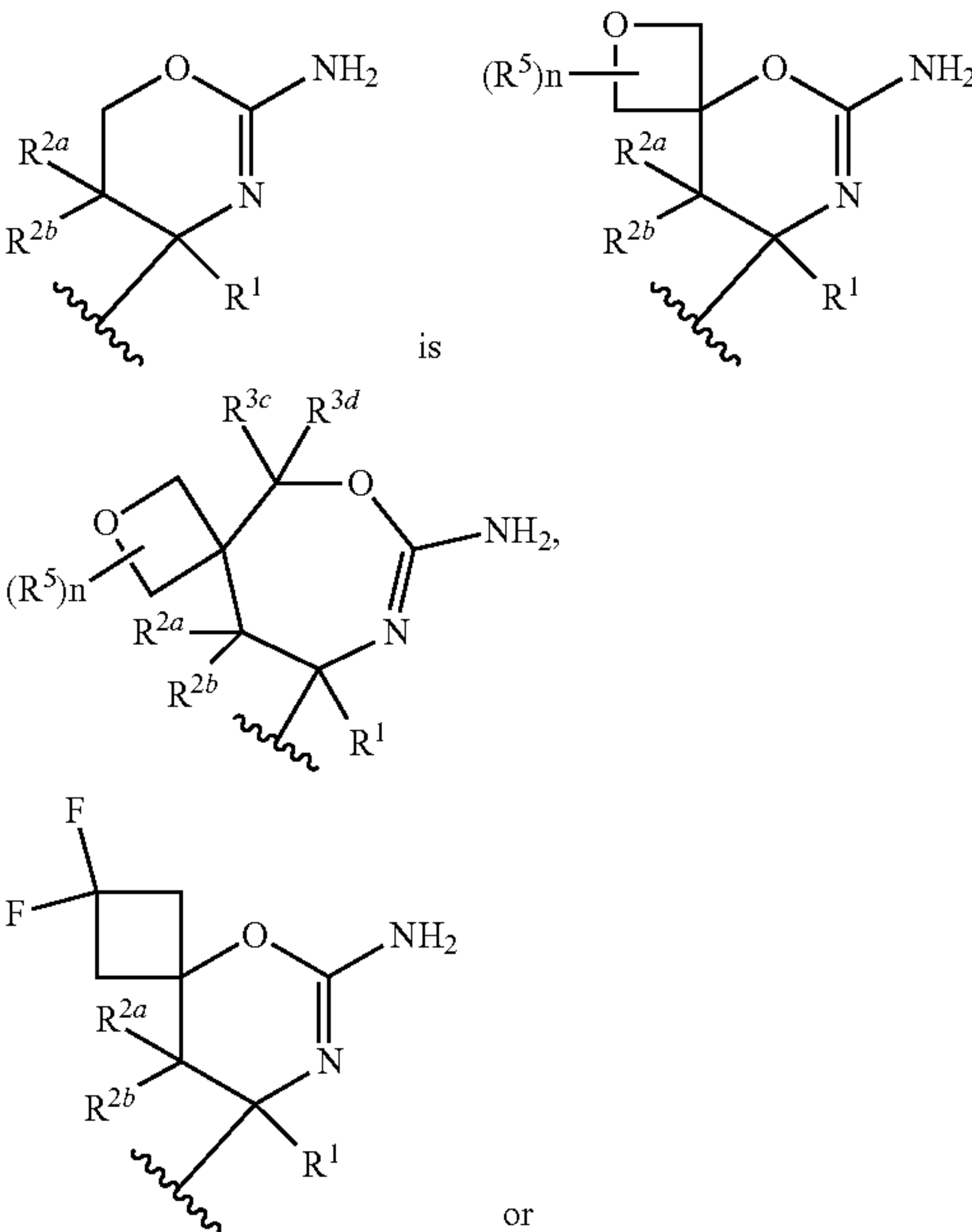
[Chemical Formula 45]
