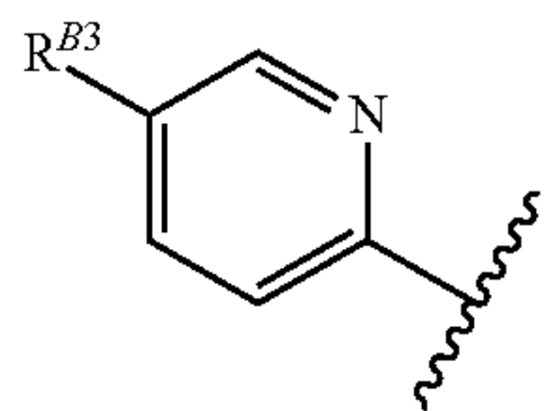
[Chemical Formula 59]
