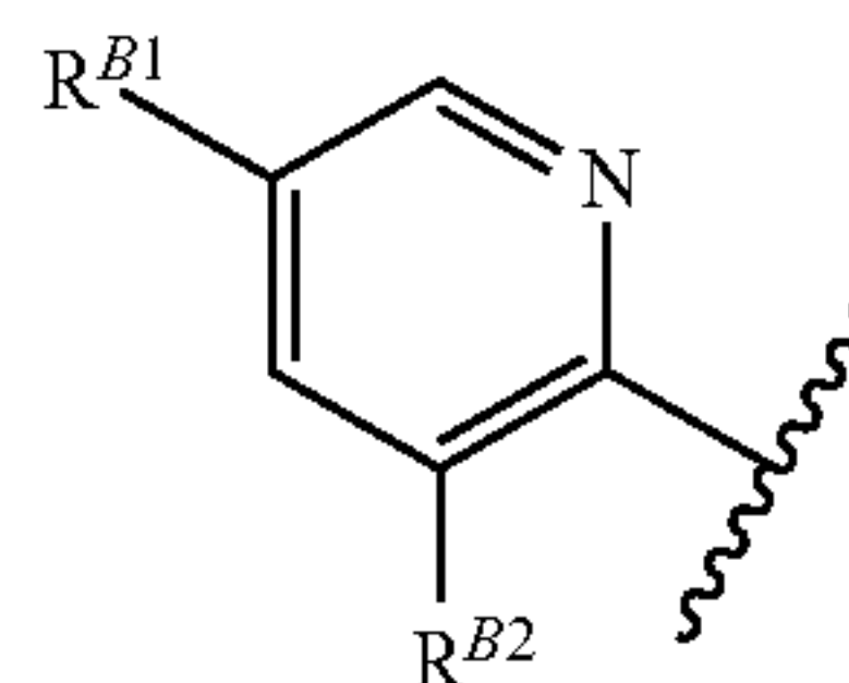
[Chemical Formula 64]
