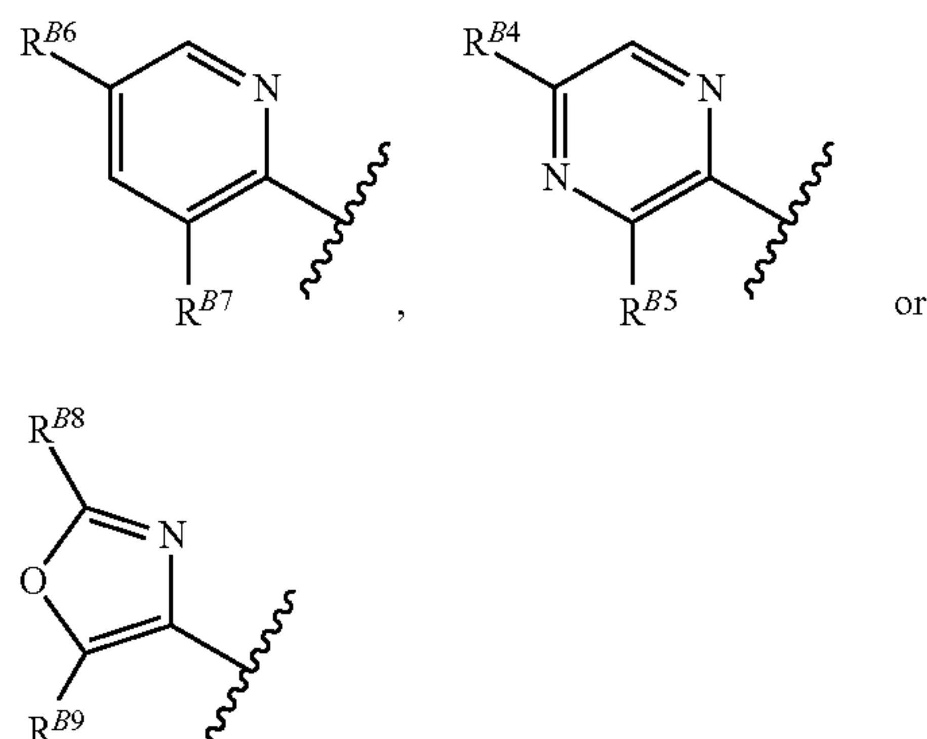
[Chemical Formula 20]
