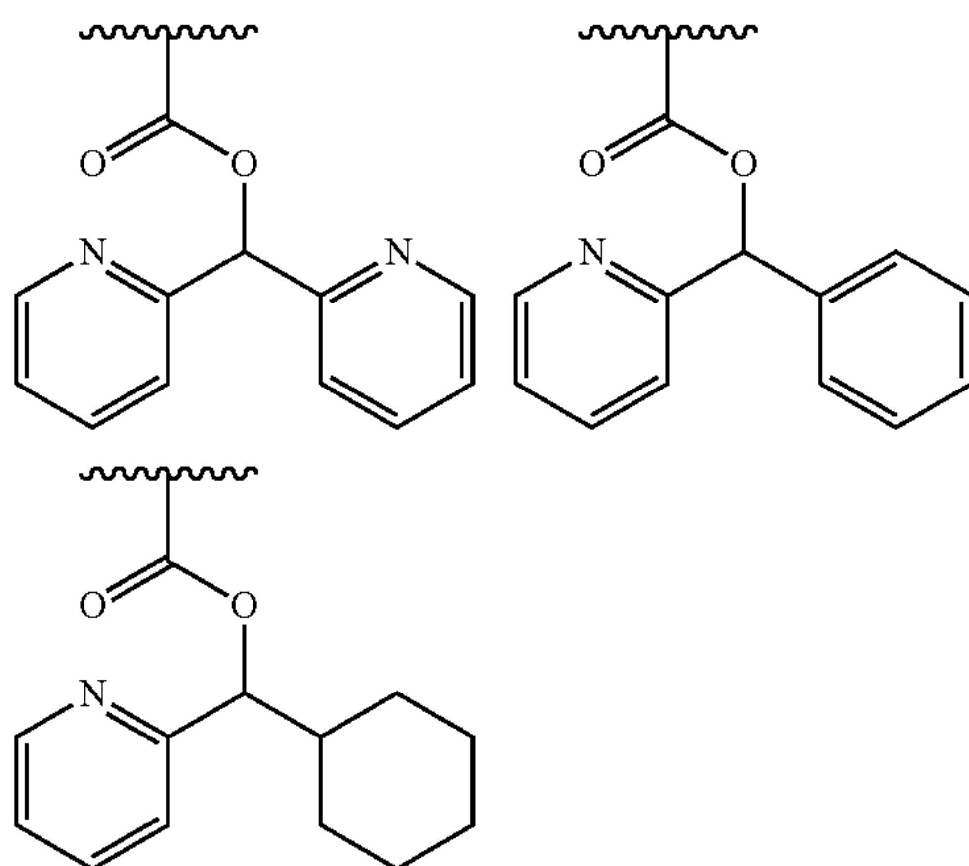
[Chemical Formula 35]
