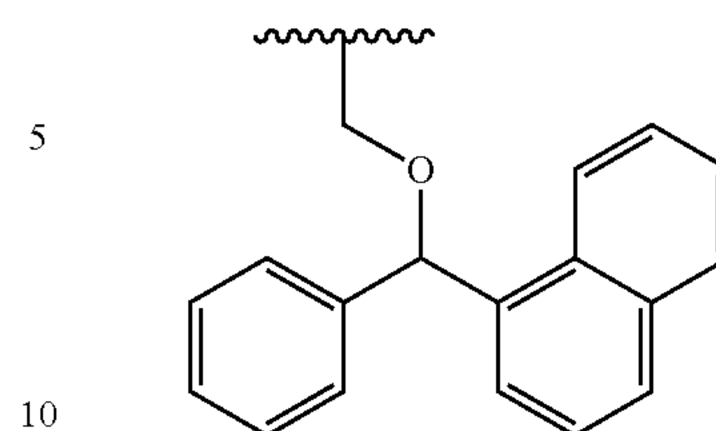
[Chemical Formula 37]
