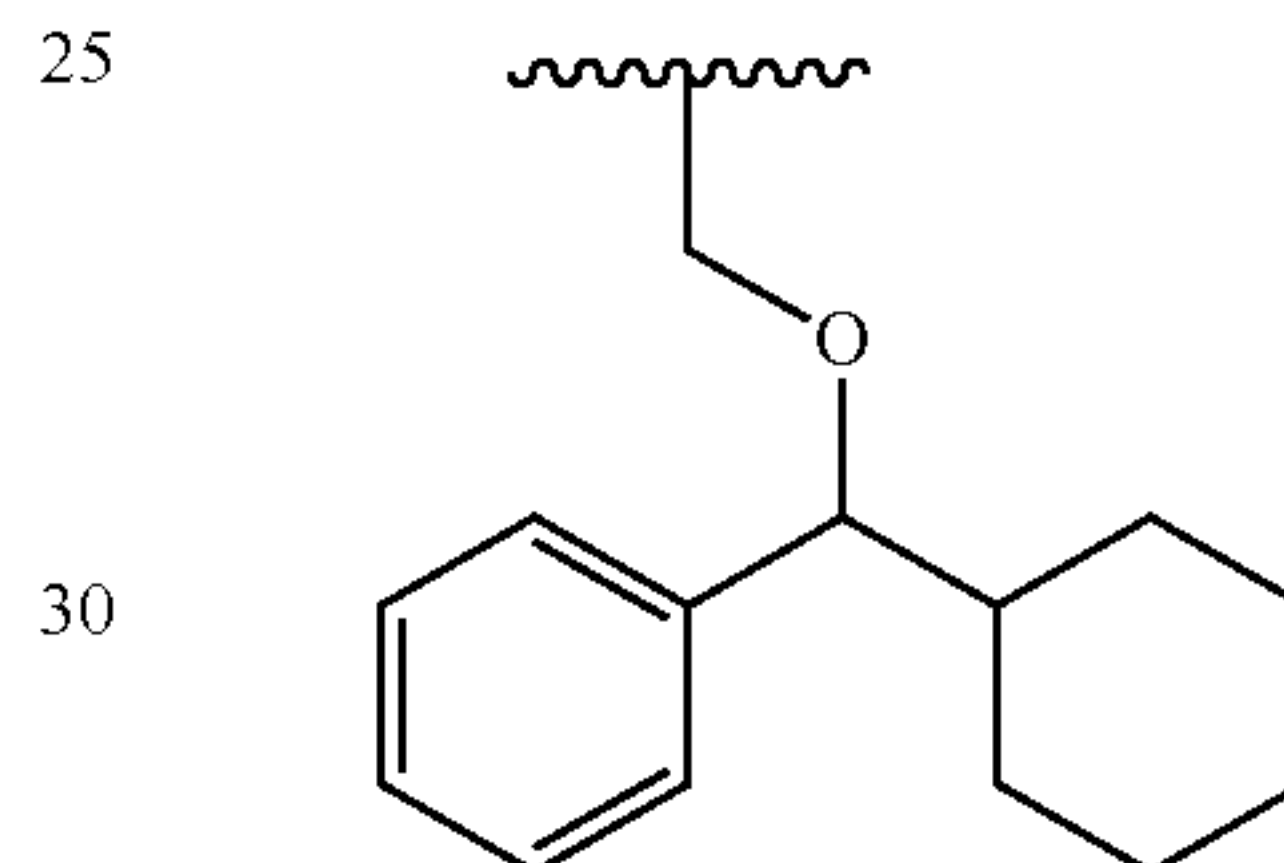
[Chemical Formula 38]
