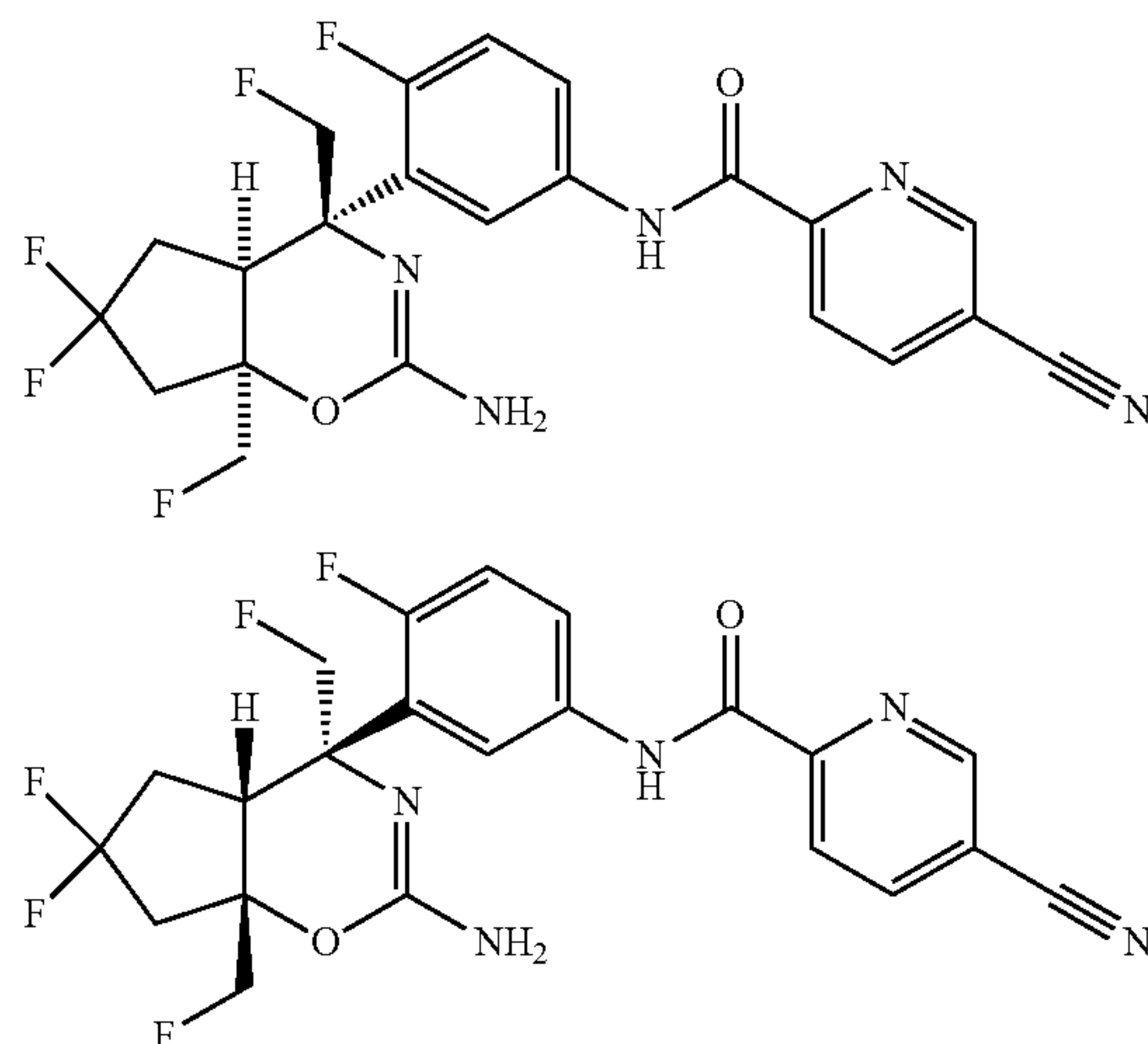
[Chemical Formula 69]
