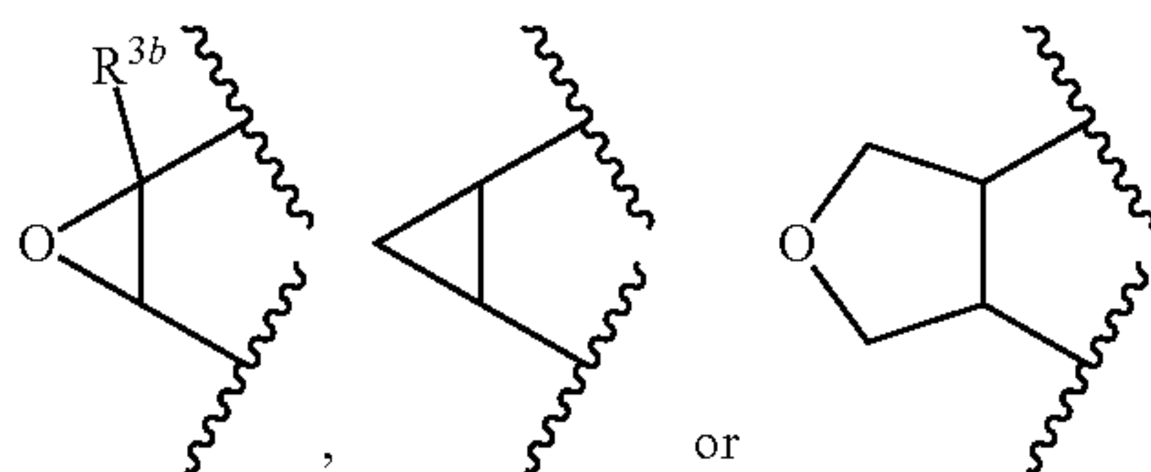
[Chemical Formula 73]
