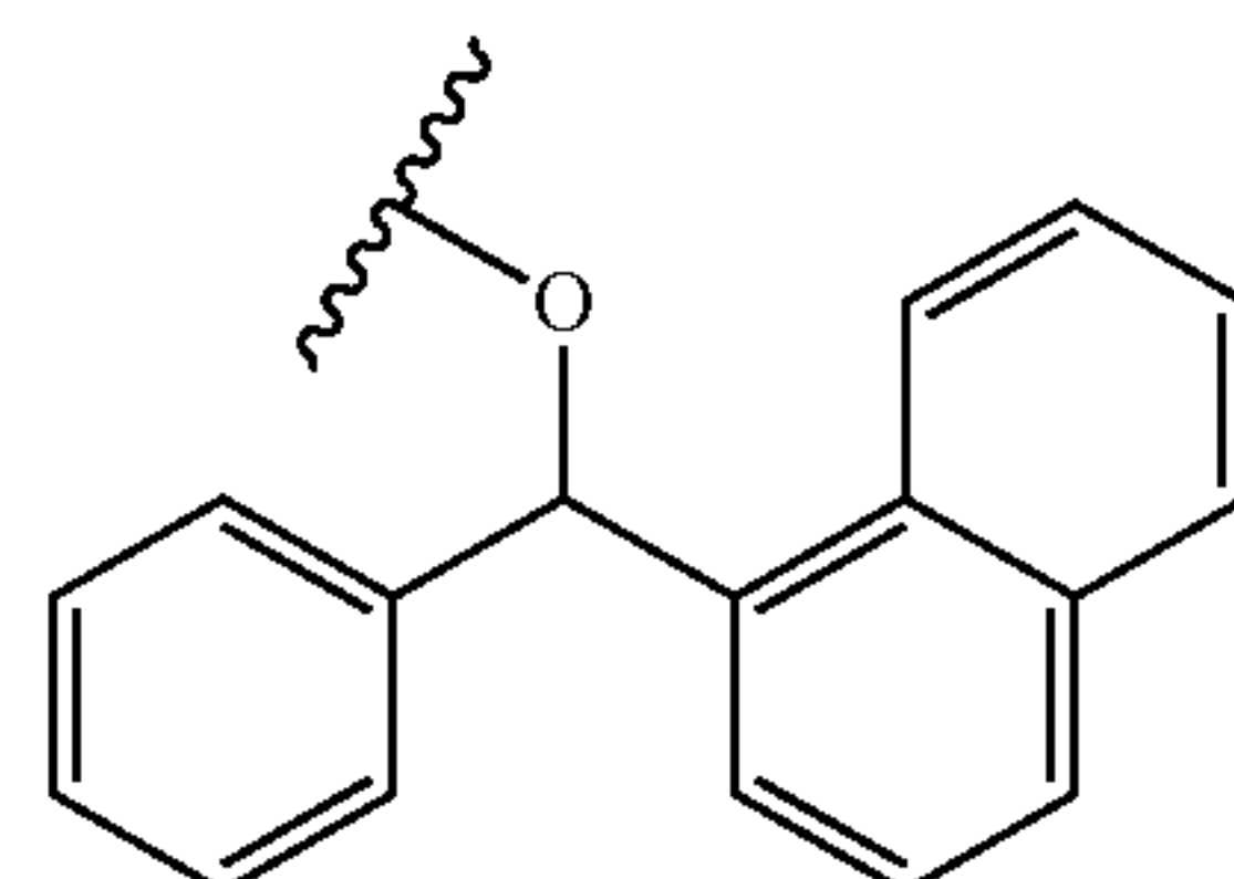
[Chemical Formula 29]
