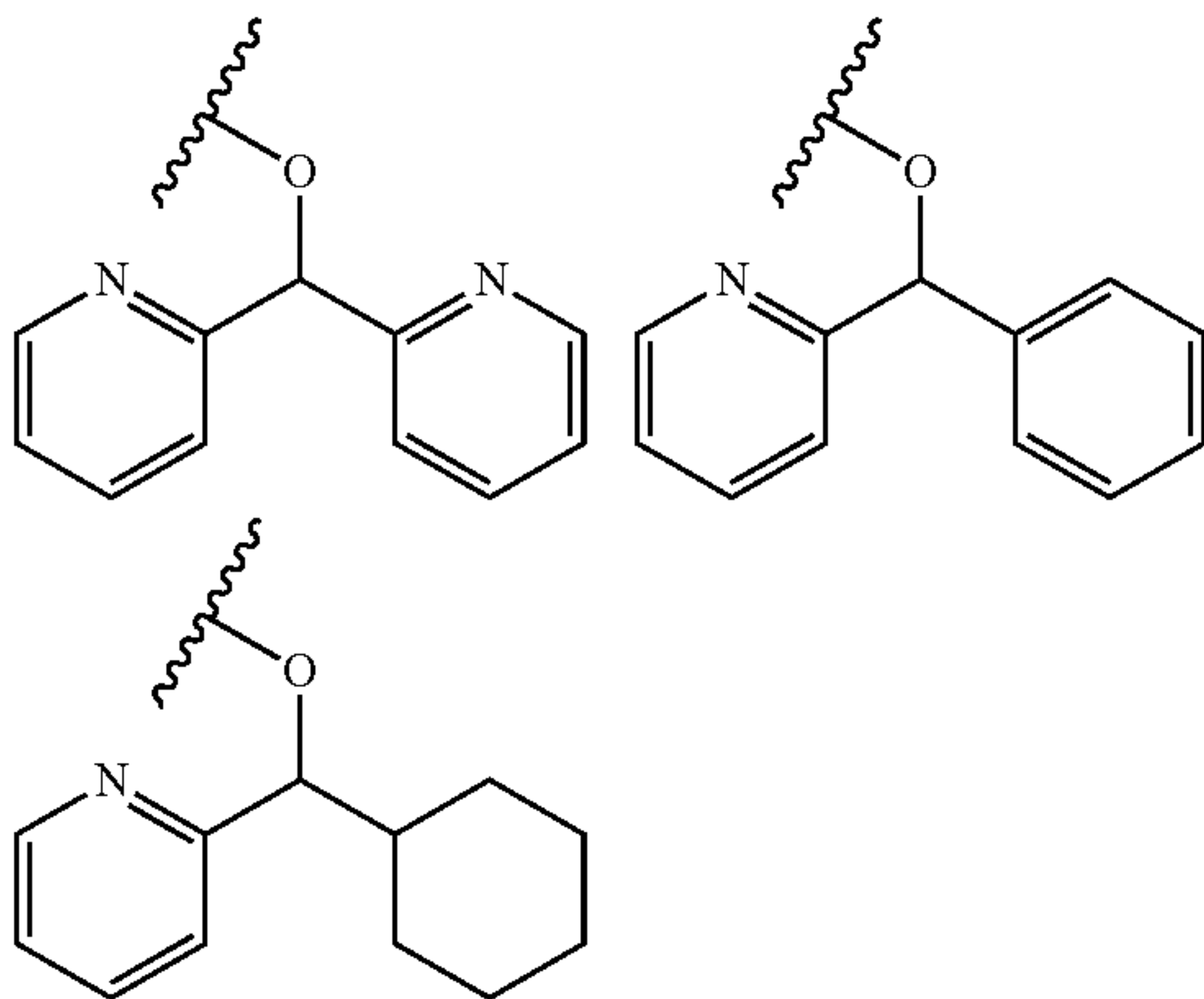
[Chemical Formula 31]
