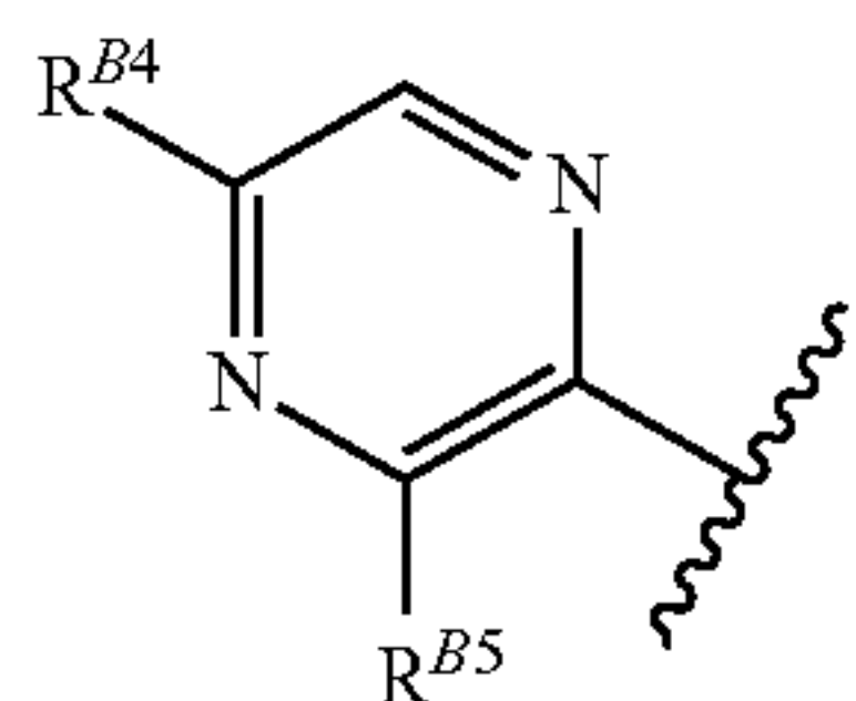
[Chemical Formula 60]
