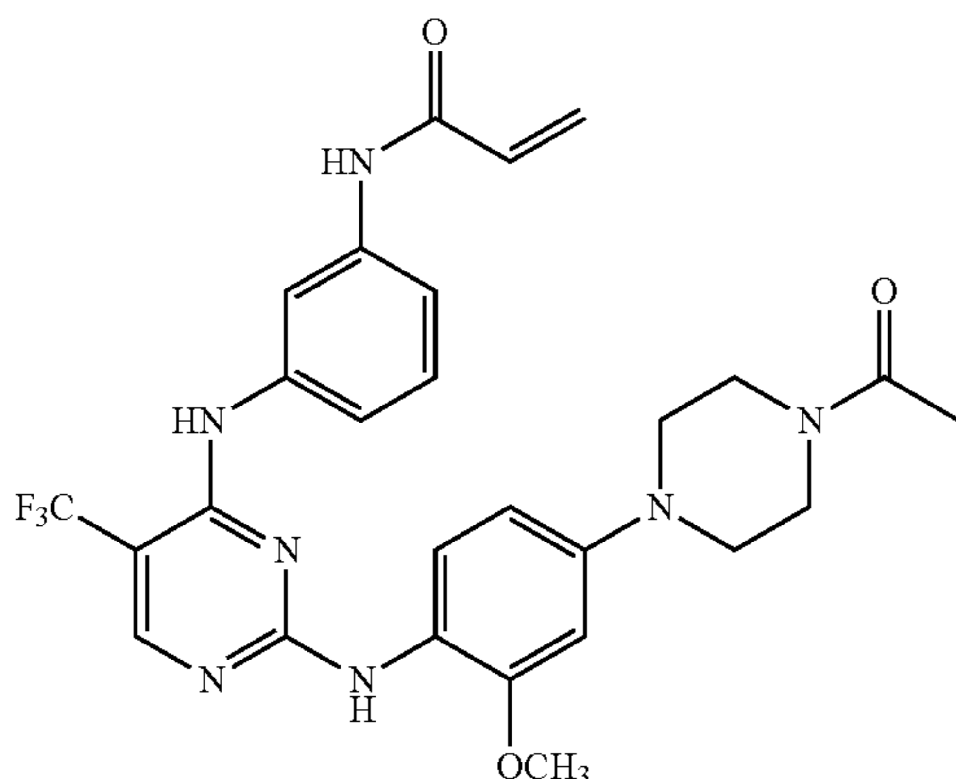
Compound 1
