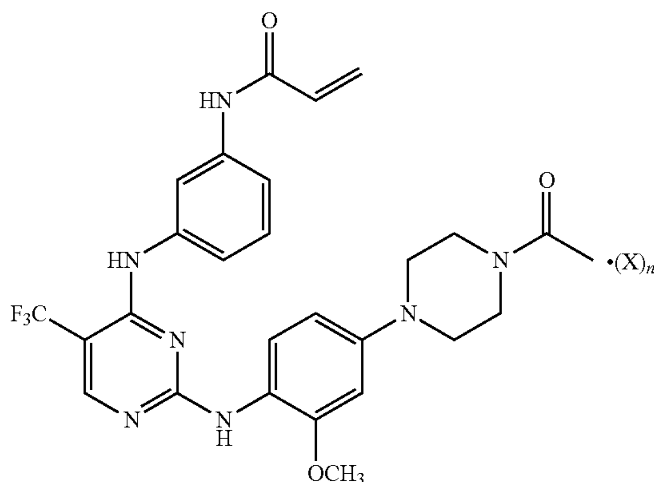
Compound 2
