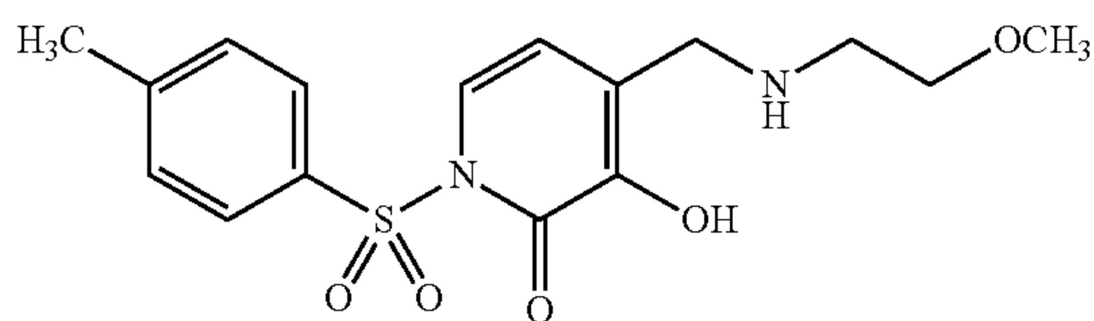
1-(4'-Methylbenzenesulfonyl)-3-hydroxy-4-[(2-methoxyethylamino)methyl]-pyridin-2(1H)-one
