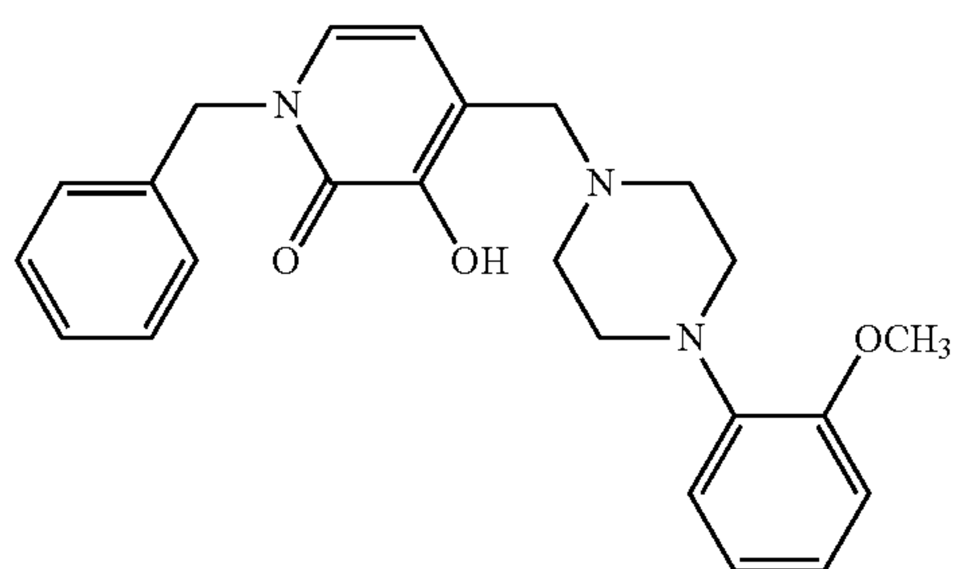
1-Benzyl-3-hydroxy-4-[4-(2-methoxyphenyl)piperazin-1-ylmethyl]pyridin-2(1H)-one
