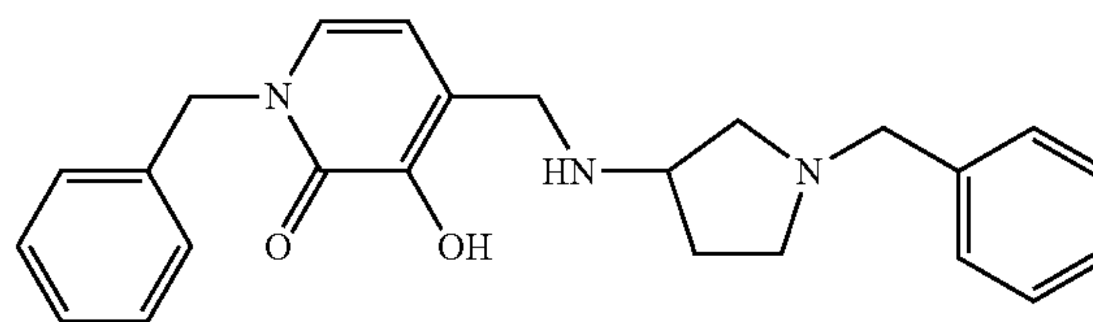
1-Benzyl-3-hydroxy-4-[(1-benzylpyrrolidin-3-ylamino)methyl]pyridin-2(1H)-one
