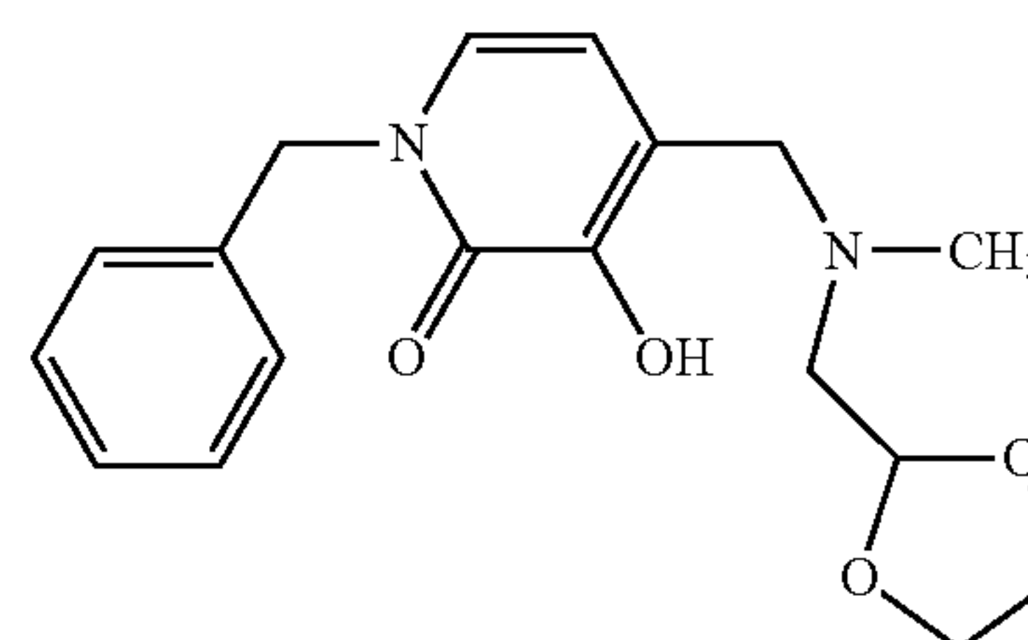
1-Benzyl-3-hydroxy-4-[[1,3]dioxolan-2-ylmethylmethylamino)methyl]pyridin-2(1H)-one
