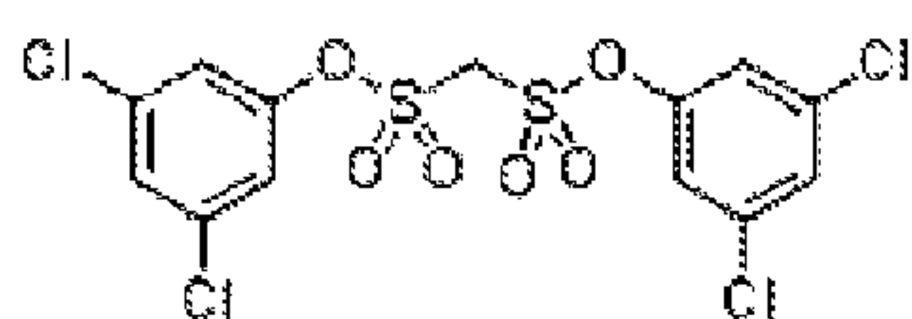
XC-ESI-4 C_{13}H_6Cl_4O_6S_2 Exact Mass: 463.8516 Mol. Wt.: 466.1410
