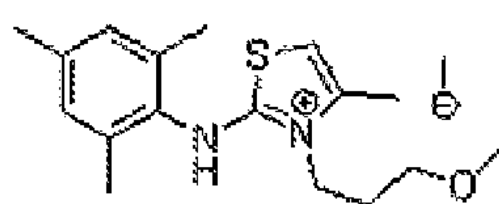
XC-ESI-7 C_{17}H_{25}IN_2OS Exact Mass: 432.0732 Mol. Wt.: 432.3627
