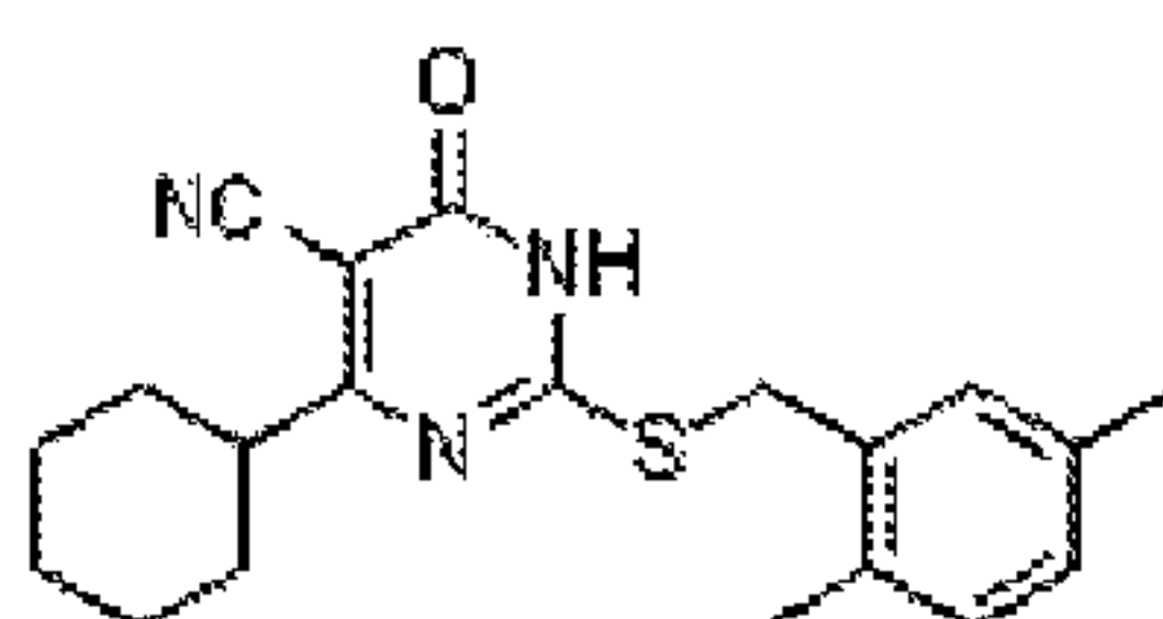
XC-ESI-8 C_{20}H_{23}N_3OS Exact Mass: 353.1562 Mol. Wt.: 353.4811
