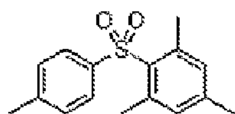
XC-ESI-5 C_{10}H_{10}O_2S Exact Mass: 274.1028 Mol. Wt.: 274.3779
