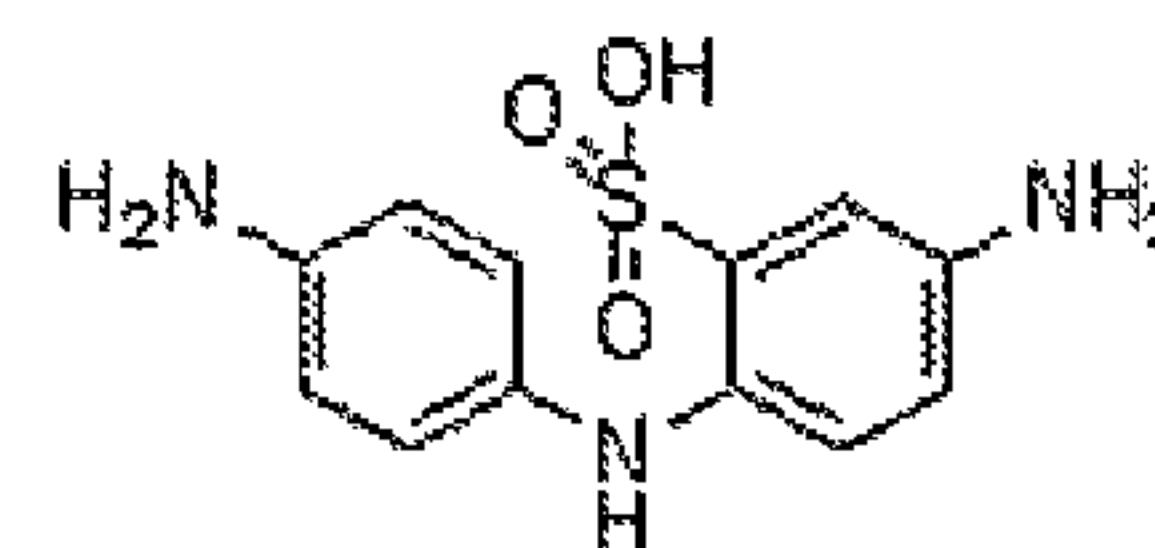
XC-ESI-10 C_{12}H_{13}N_3O_3S Exact Mass: 279.0678 Mol. Wt.: 279.3149
