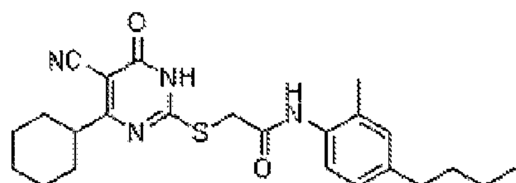
XC-ESI-6 C_{24}H_{30}N_4O_2S Exact Mass: 438.2099 Mol. Wt.: 438.5856
