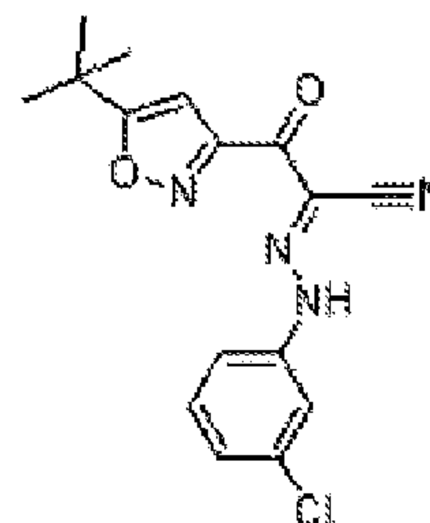
XC-ESI-9 C_{16}H_{15}ClN_4O_2 Exact Mass: 330.0884 Mol. Wt.: 330.7689
