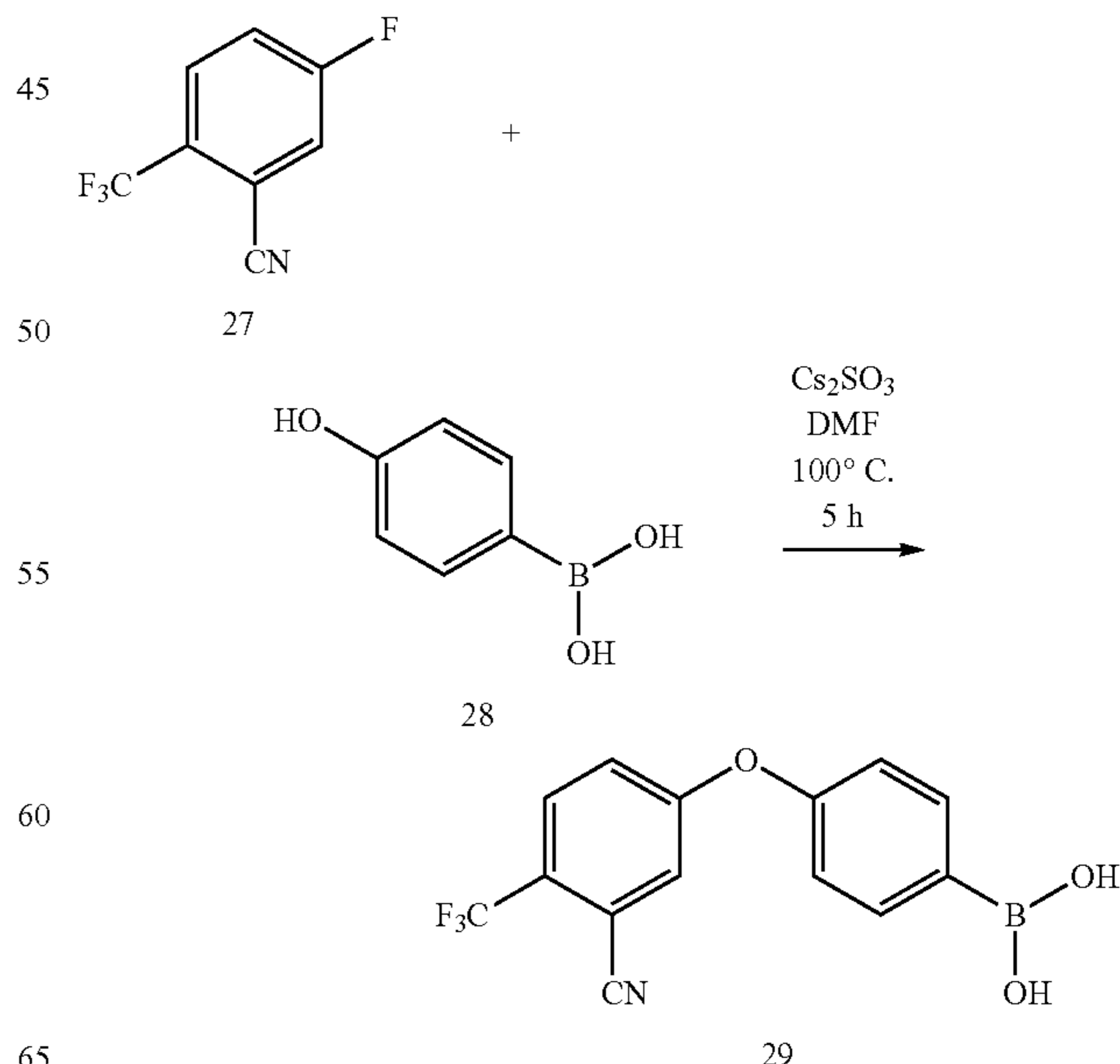
Scheme 18
