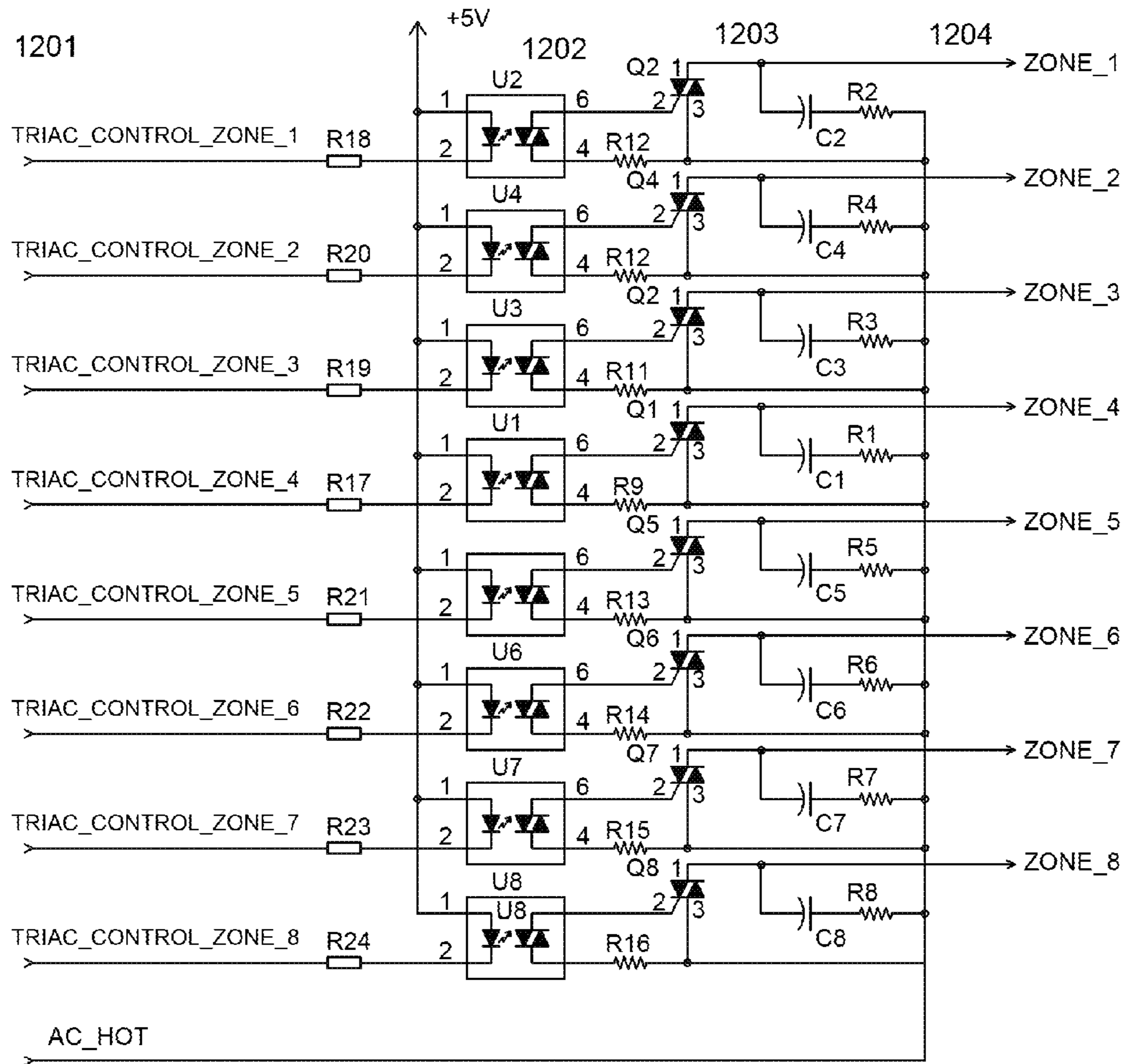
MASTER DIMMING CONTROLLER ZONE DIMMER CIRCUITS
