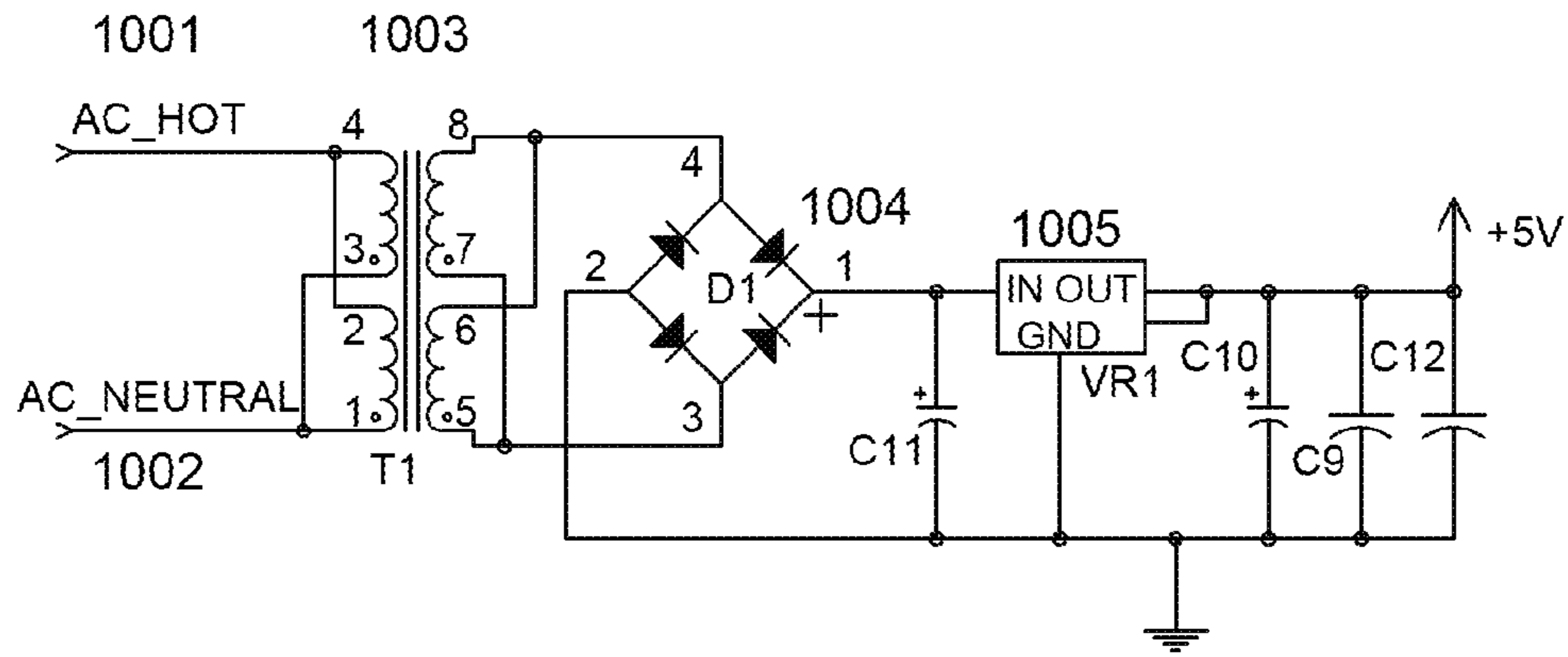
KEYPAD POWER SUPPLY
