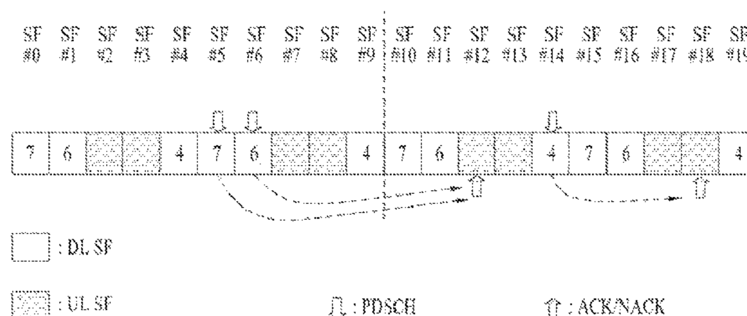
PDSCH-ACK/NACK timing (UL-DL configuration #1)
