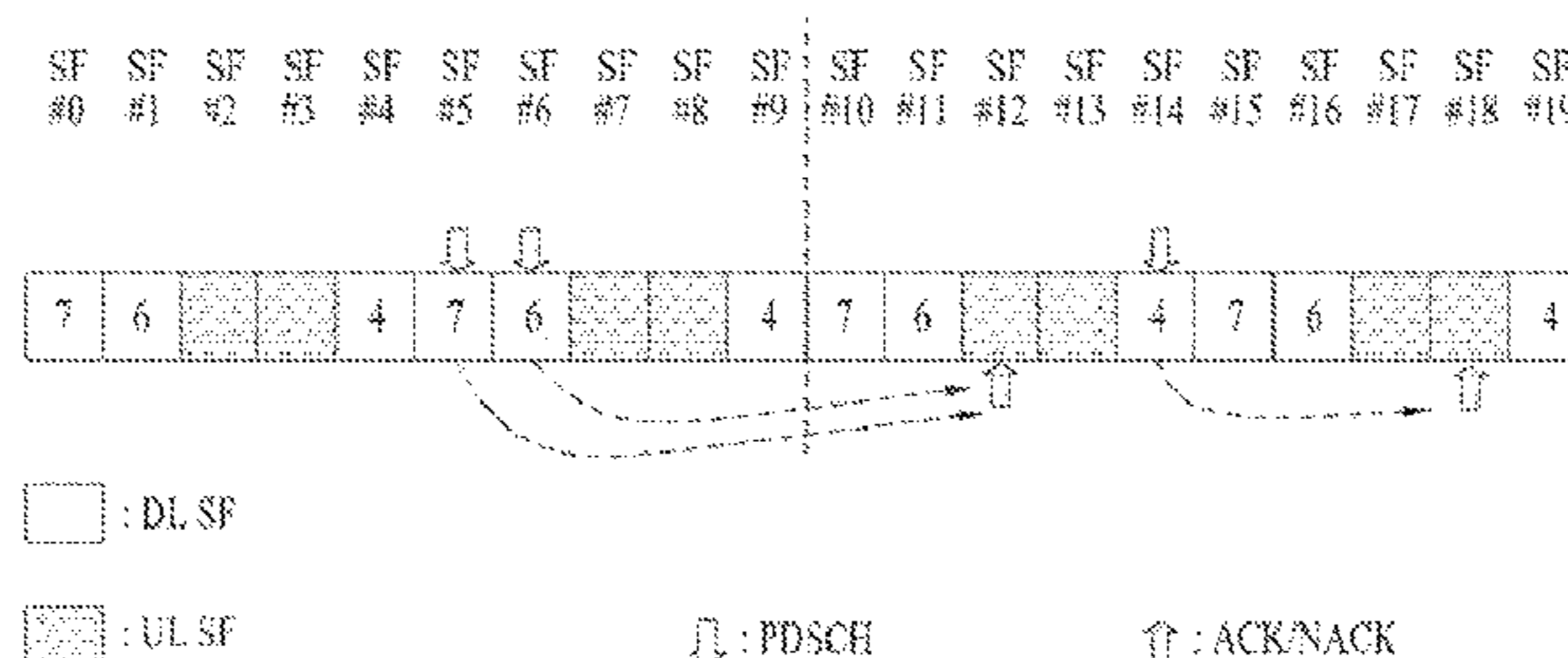
PDSCH-ACK/NACK timing (UL-DL configuration #1)
