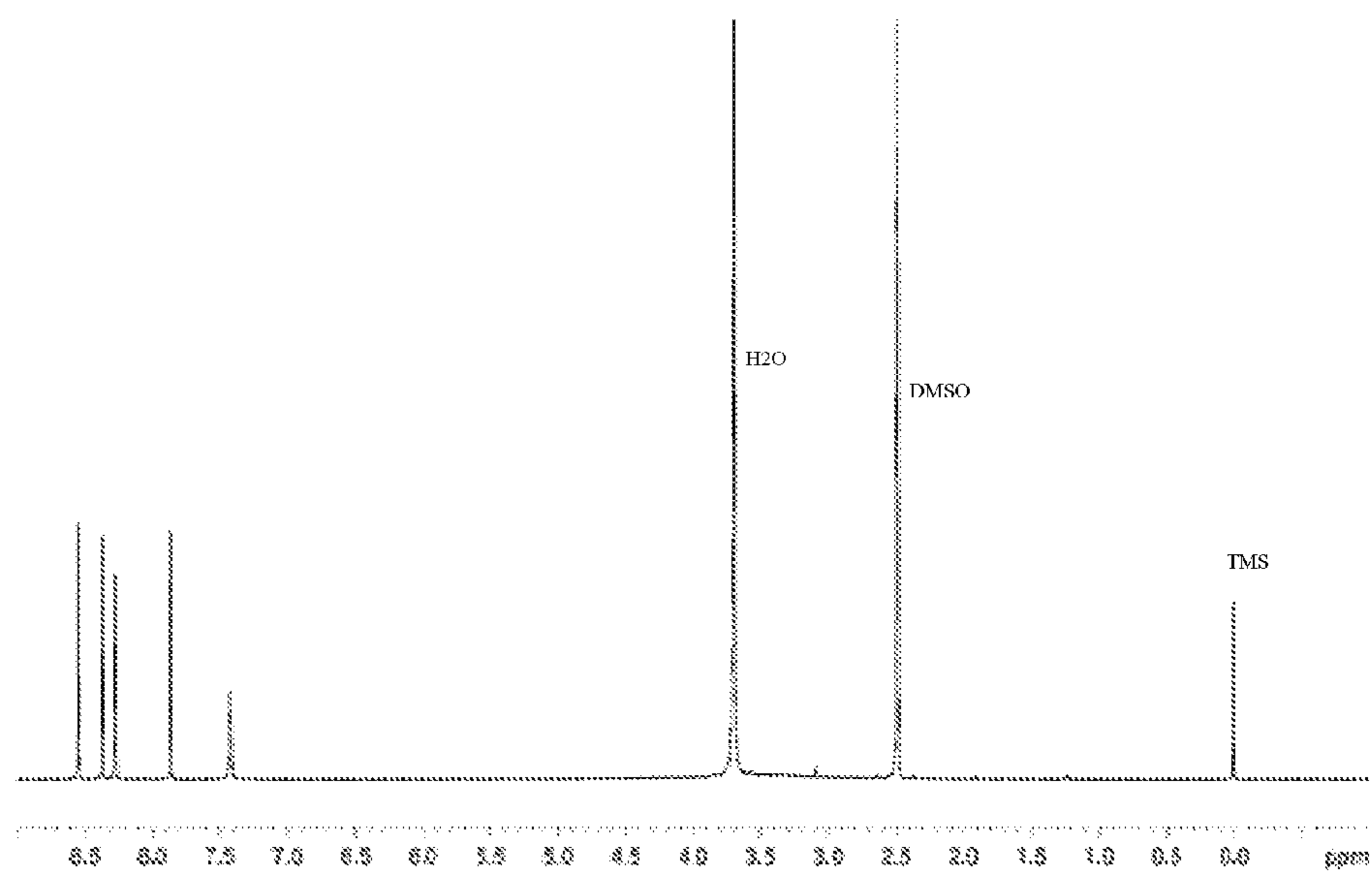
Fig. 5: ^1\text{H} NMR spectrum of the compound of the formula (I)
