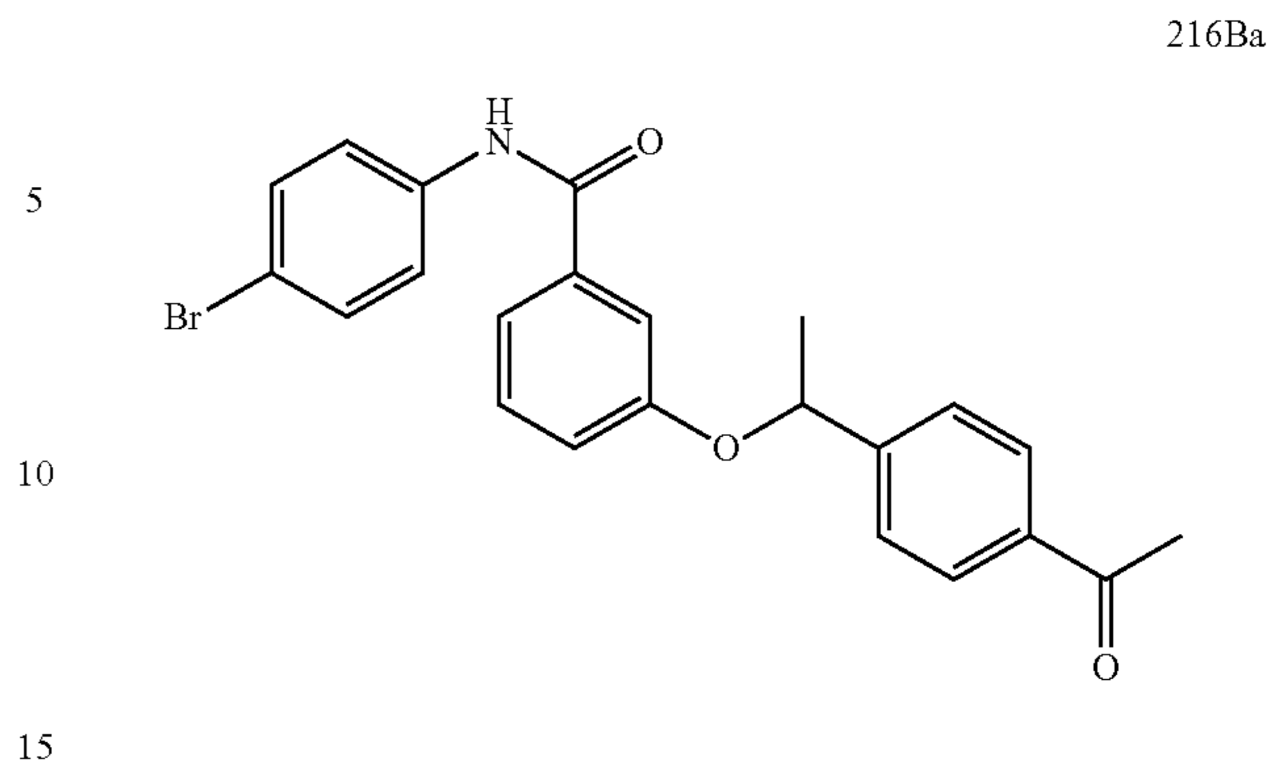
3-(1-(4-acetylphenyl)ethoxy)-N-(4-bromophenyl)benzamide (216Ba)
