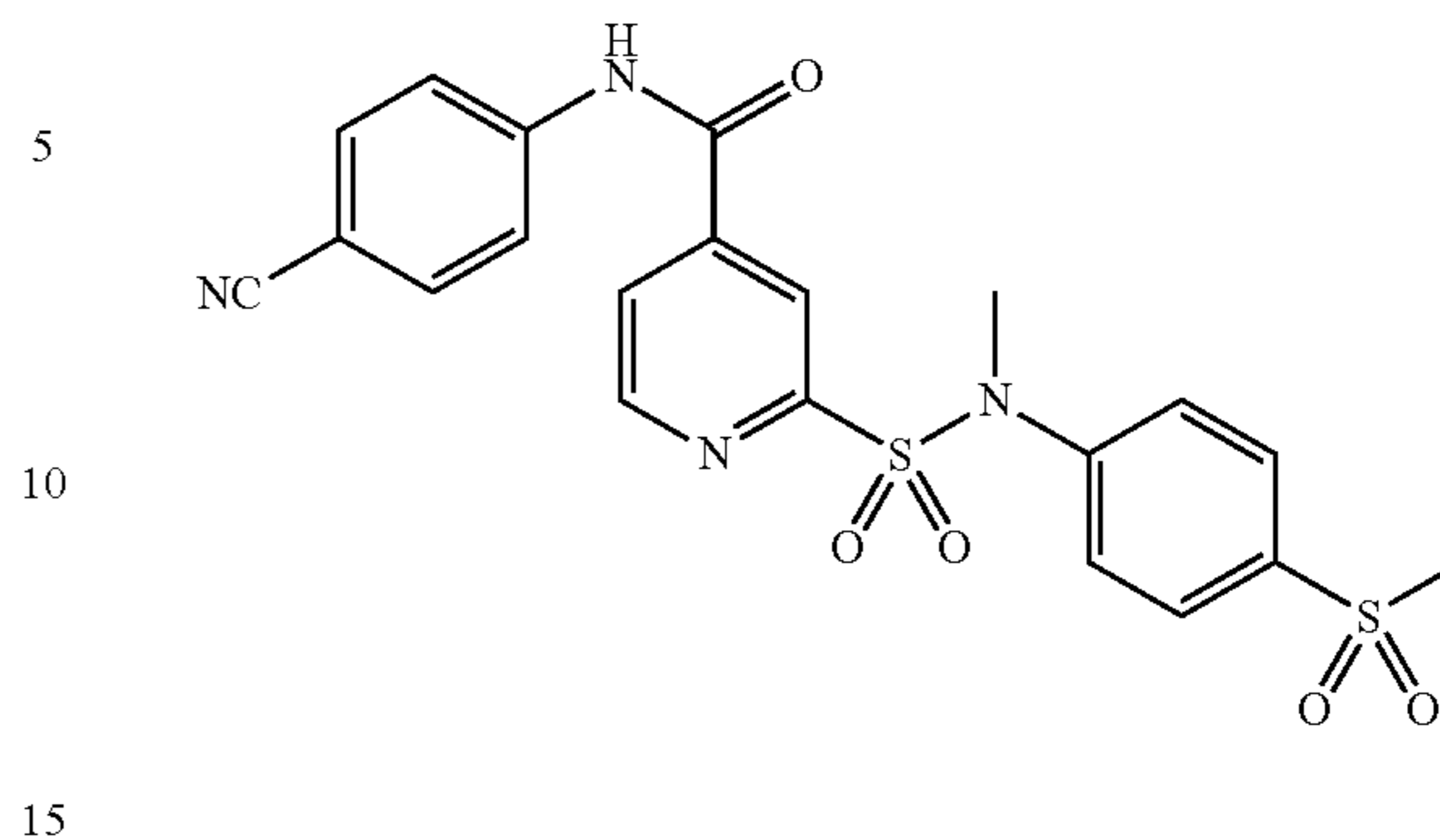
N-(4-cyanophenyl)-2-(N-methyl-N-(4-(methylsulfonyl)phenyl)sulfamoyl)-isonicotinamide (203As)
