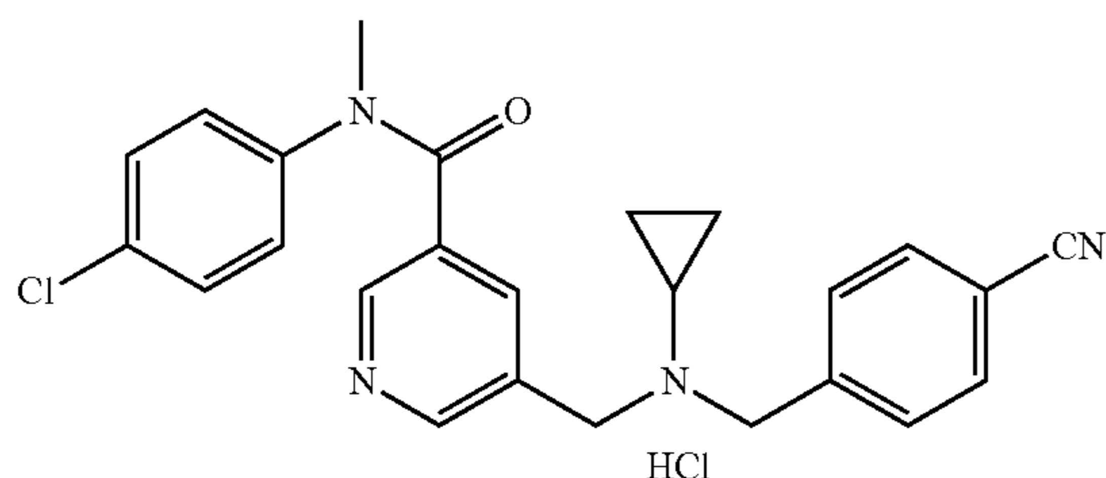
N-(4-chlorophenyl)-5-(((4-cyanobenzyl)(cyclopropyl)amino)methyl)-N-methylnicotinamide hydrochloride (225p)
