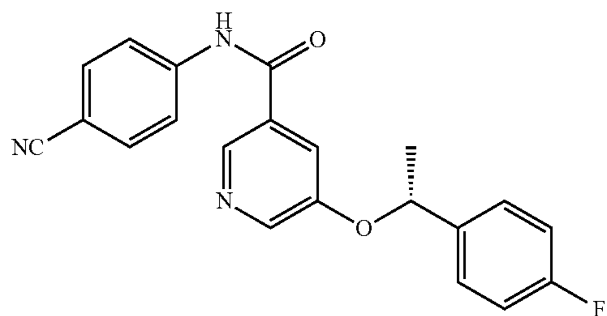
(R)-N-(4-cyanophenyl)-5-(1-(4-fluorophenyl)ethoxy)nicotinamide (216r)
