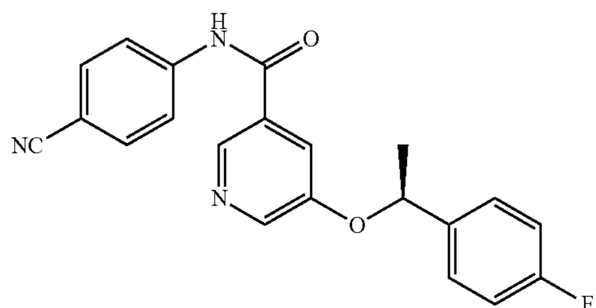
(S)-N-(4-cyanophenyl)-5-(1-(4-fluorophenyl)ethoxy)nicotinamide (216s)
