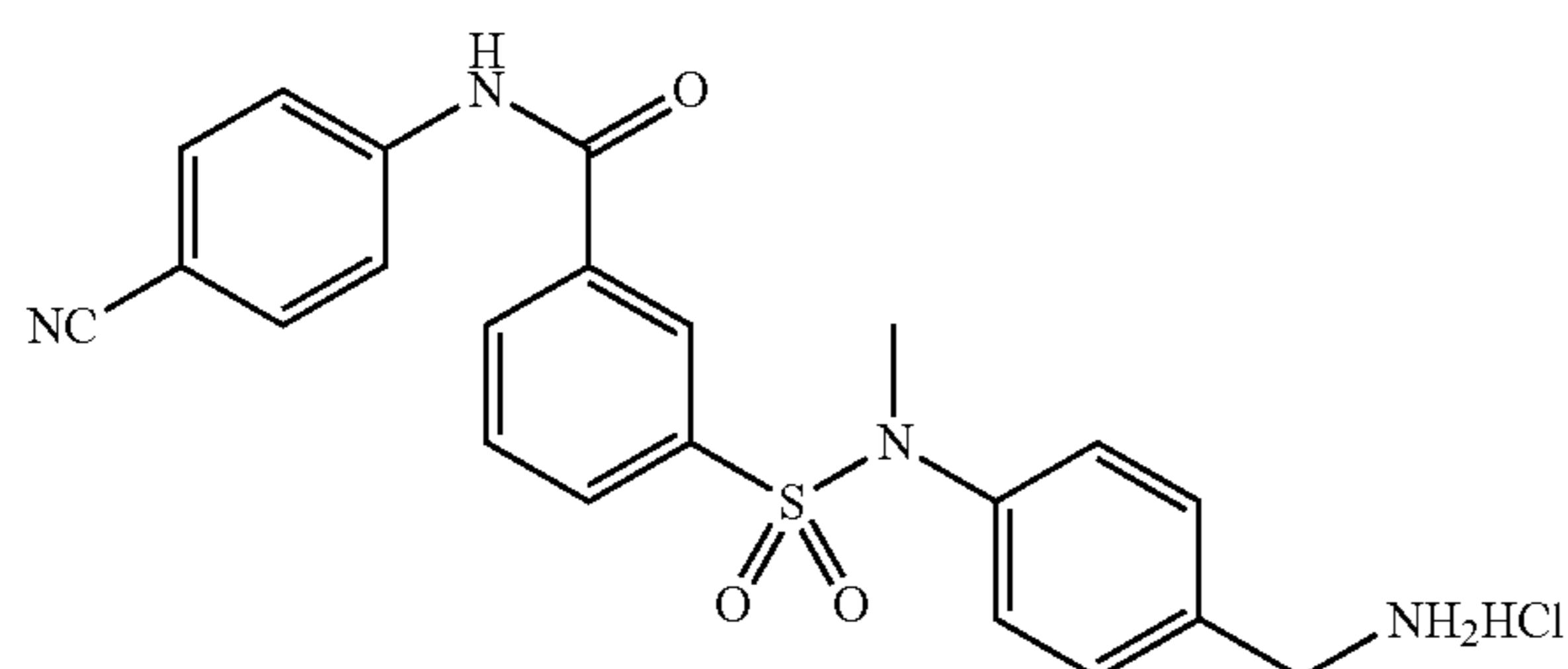
3-(N-(4-(aminomethyl)phenyl)-N-methylsulfamoyl)-N-(4-cyanophenyl)benzamide hydrochloride (203Af)
