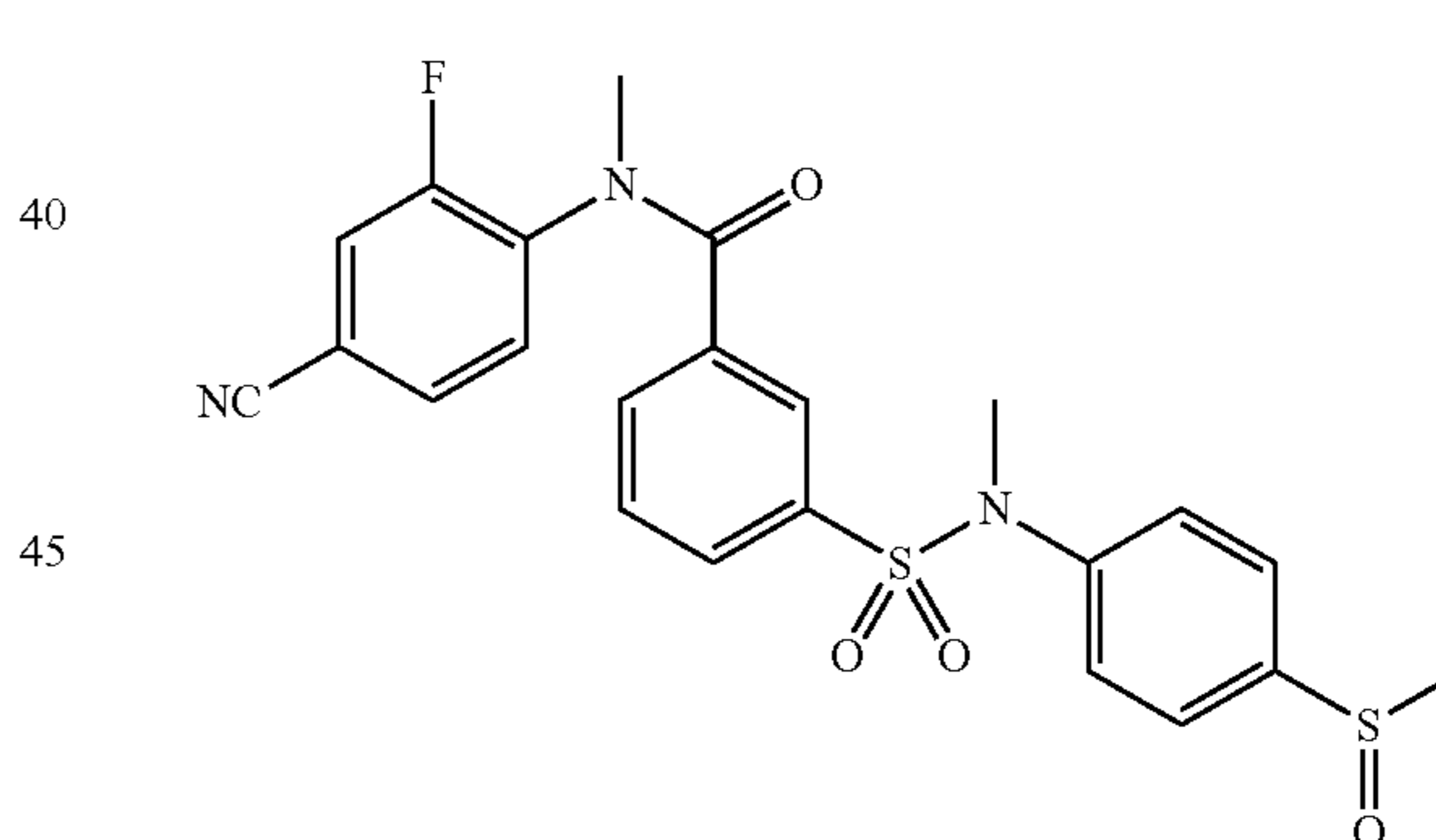
N-(4-cyano-2-fluorophenyl)-N-methyl-3-(N-methyl-N-(4-(methylsulfinyl)phenyl)sulfamoyl)benzamide (203Al)
