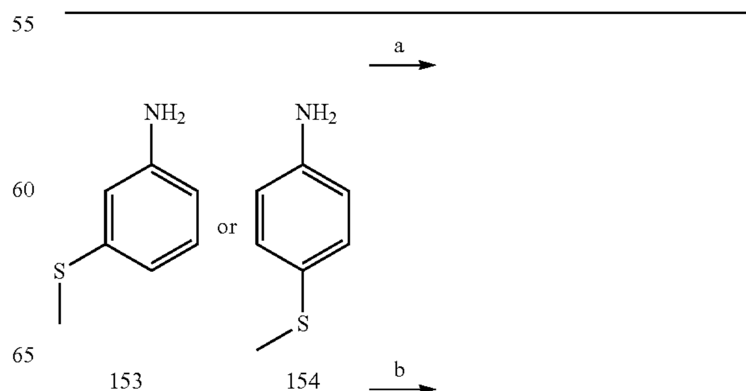
Scheme 2 a . Oxidation of aminothioanisole to generate the corresponding sulfoxide and sulfone derivatives
