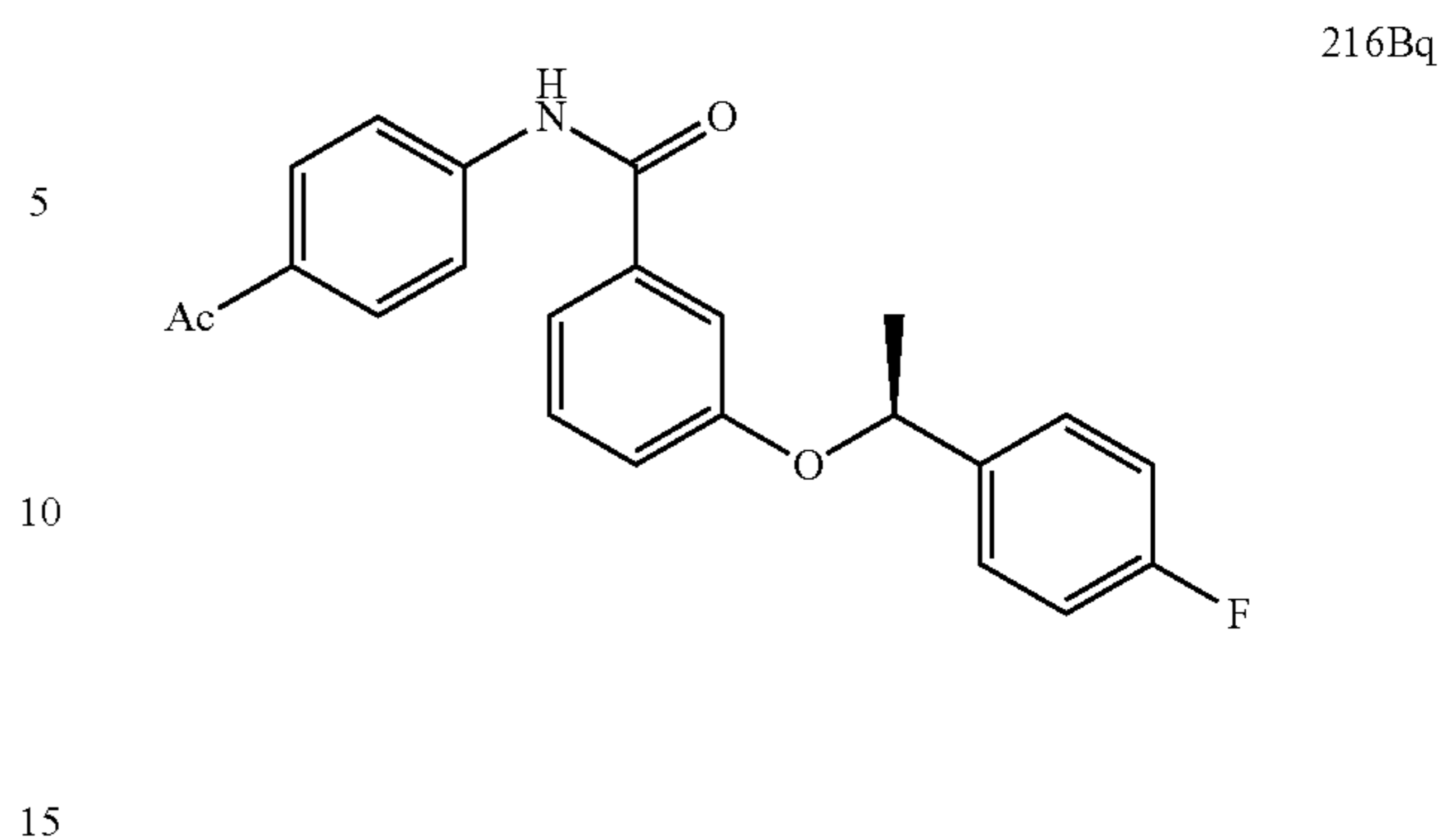
(S)—N-(4-acetylphenyl)-3-(1-(4-fluorophenyl)ethoxy)benzamide (216Bq)
