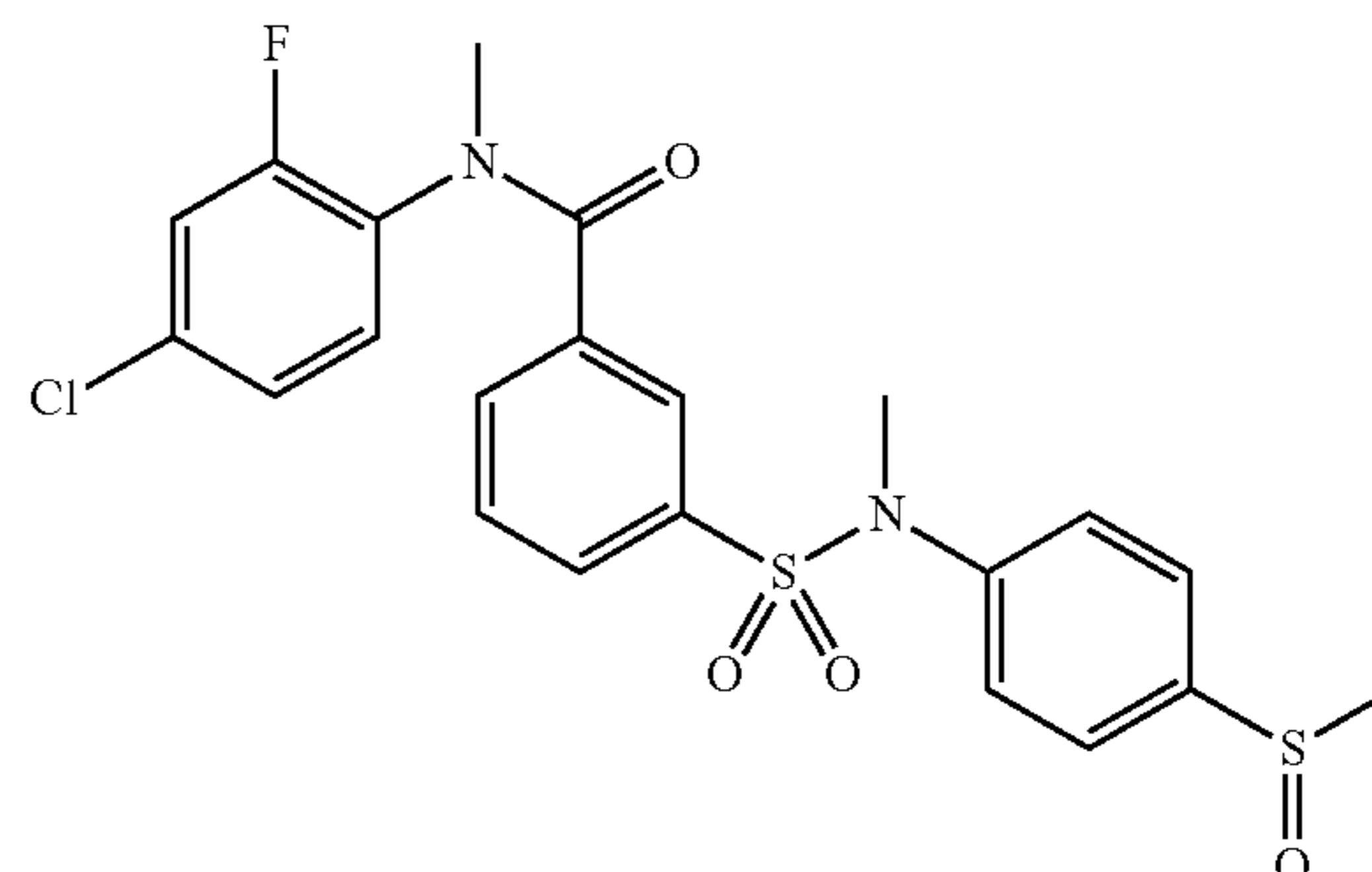
N-(4-chloro-2-fluorophenyl)-N-methyl-3-(N-methyl-N-(4-(methylsulfonyl)phenyl)sulfamoyl)benzamide (203Ag)
