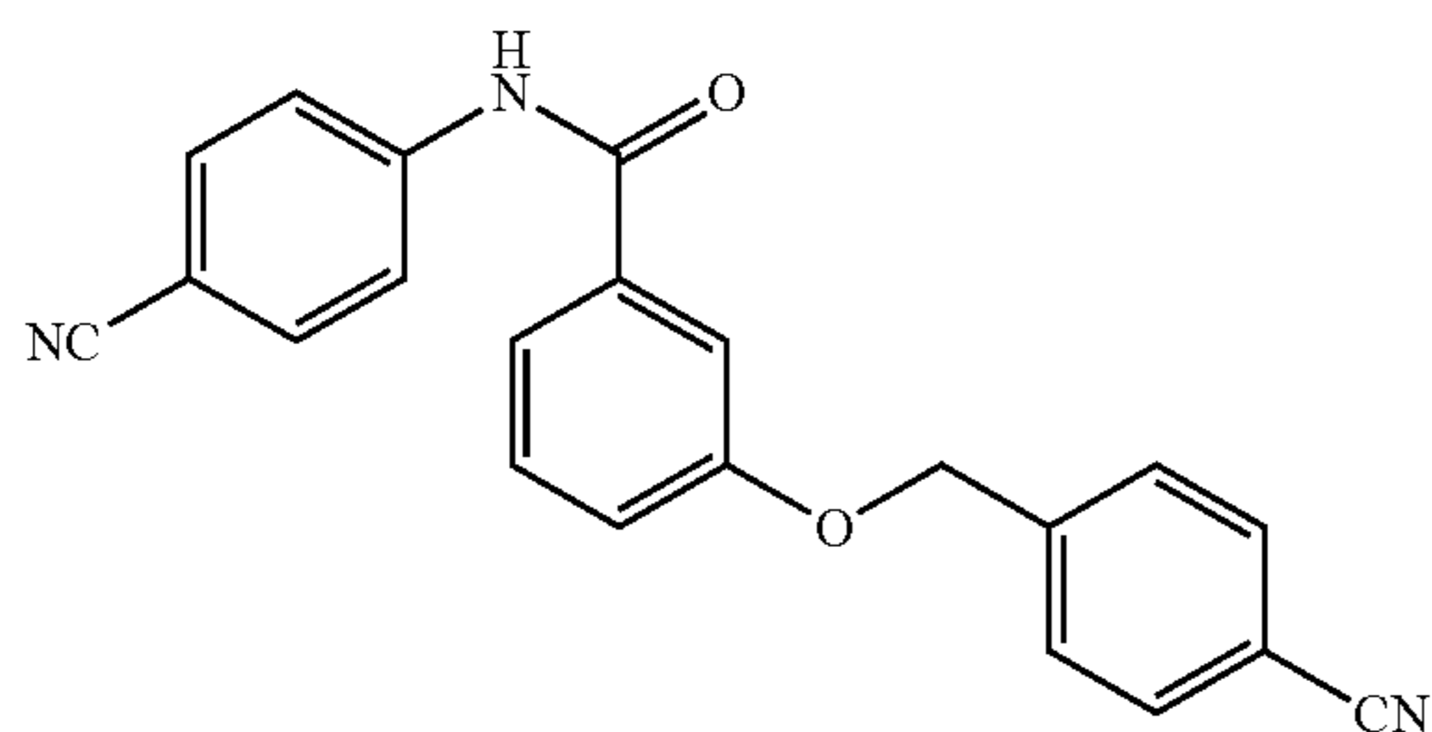
3-((4-cyanobenzyl)oxy)-N-(4-cyanophenyl)benzamide (216q)
