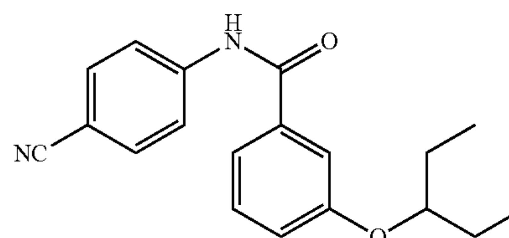
N-(4-cyanophenyl)-3-(pentan-3-yloxy)benzamide (216Ao)
