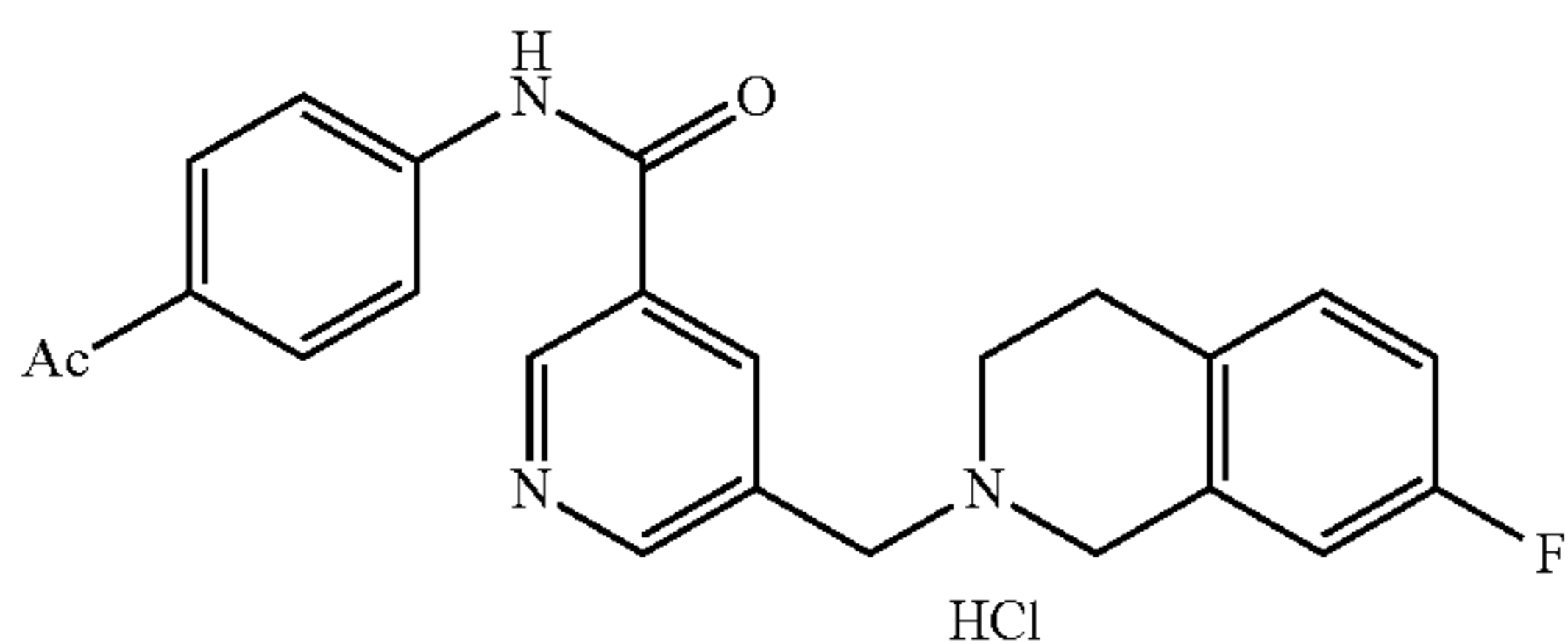
N-(4-acetylphenyl)-5-((7-fluoro-3,4-dihydroisoquinolin-2(1H)-yl)methyl)-nicotinamide hydrochloride (225Af)
