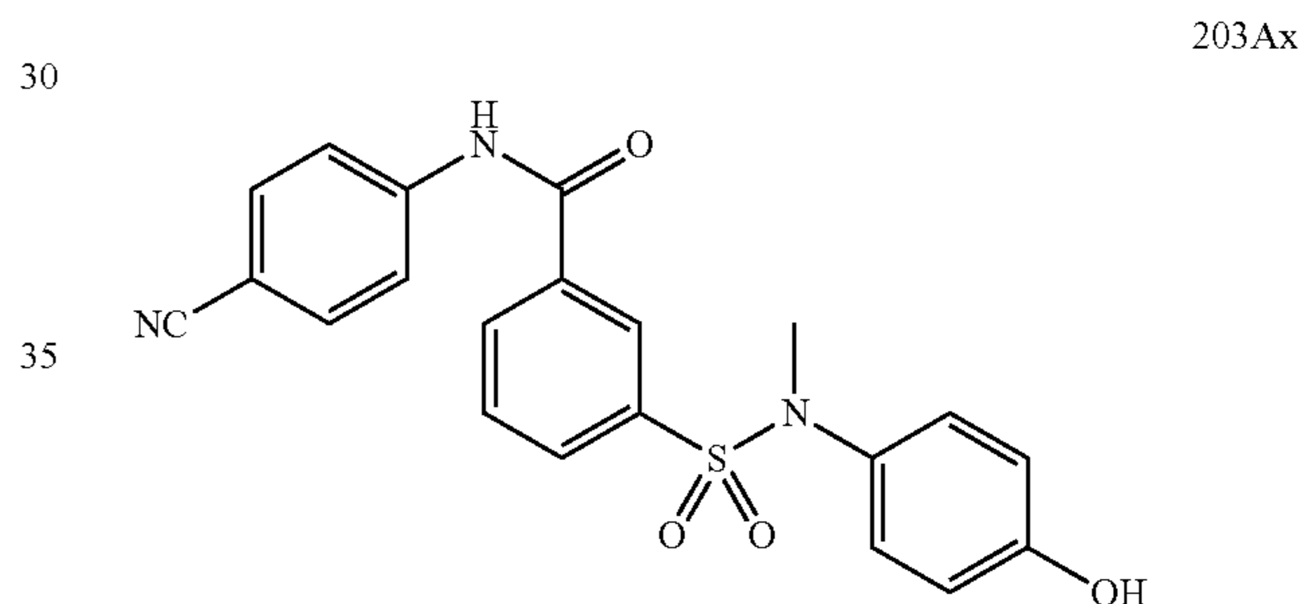
N-(4-cyanophenyl)-3-(N-(4-hydroxyphenyl)-N-methylsulfamoyl)benzamide (203Ax)
