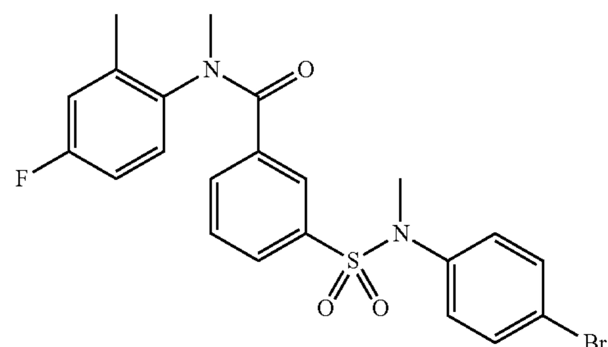
3-(N-(4-bromophenyl)-N-methylsulfamoyl)-N-(4-fluoro-2-methylphenyl)-N-methylbenzamide (203m)
