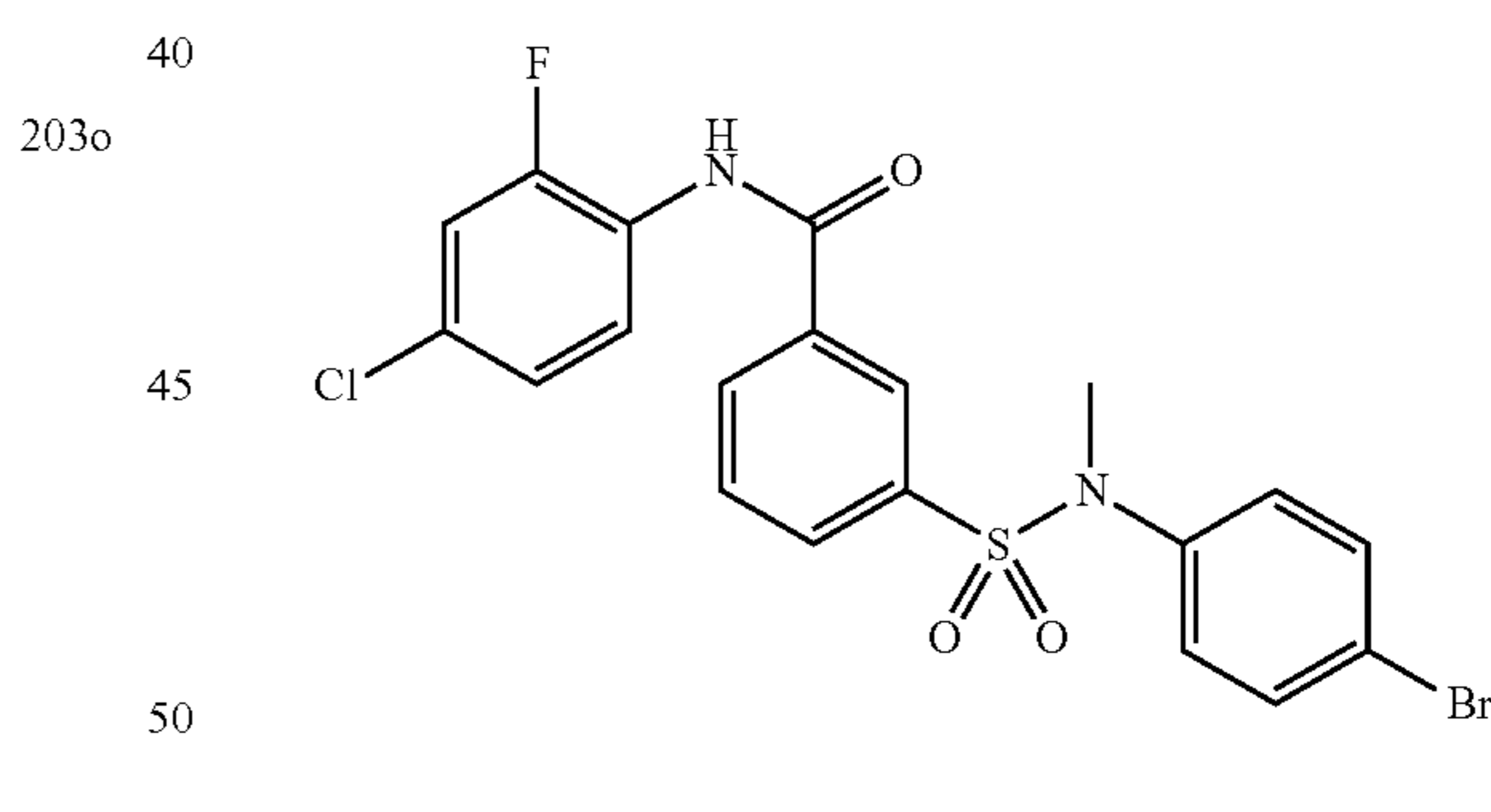
3-(N-(4-bromophenyl)-N-methylsulfamoyl)-N-(4-chloro-2-fluorophenyl)benzamide (203q)
