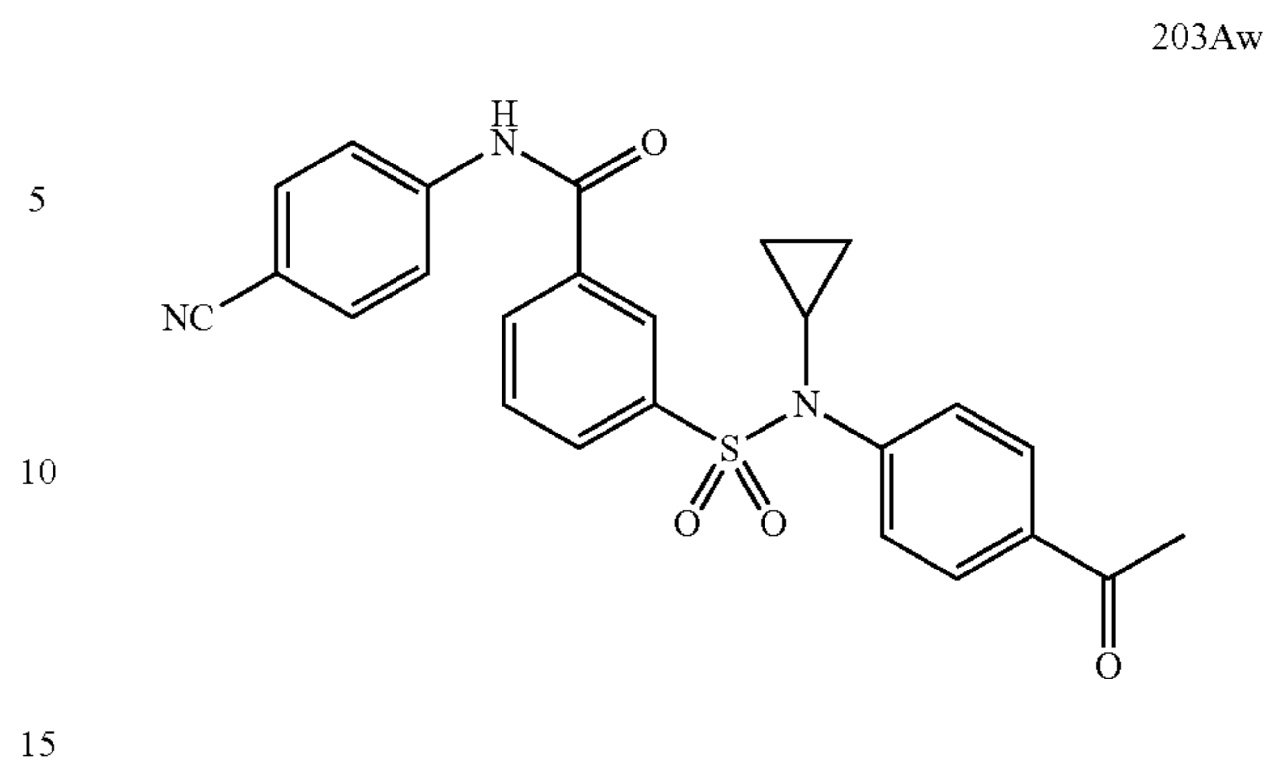
3-(N-(4-acetylphenyl)-N-cyclopropylsulfamoyl)-N-(4-cyanophenyl)benzamide (203Aw)
