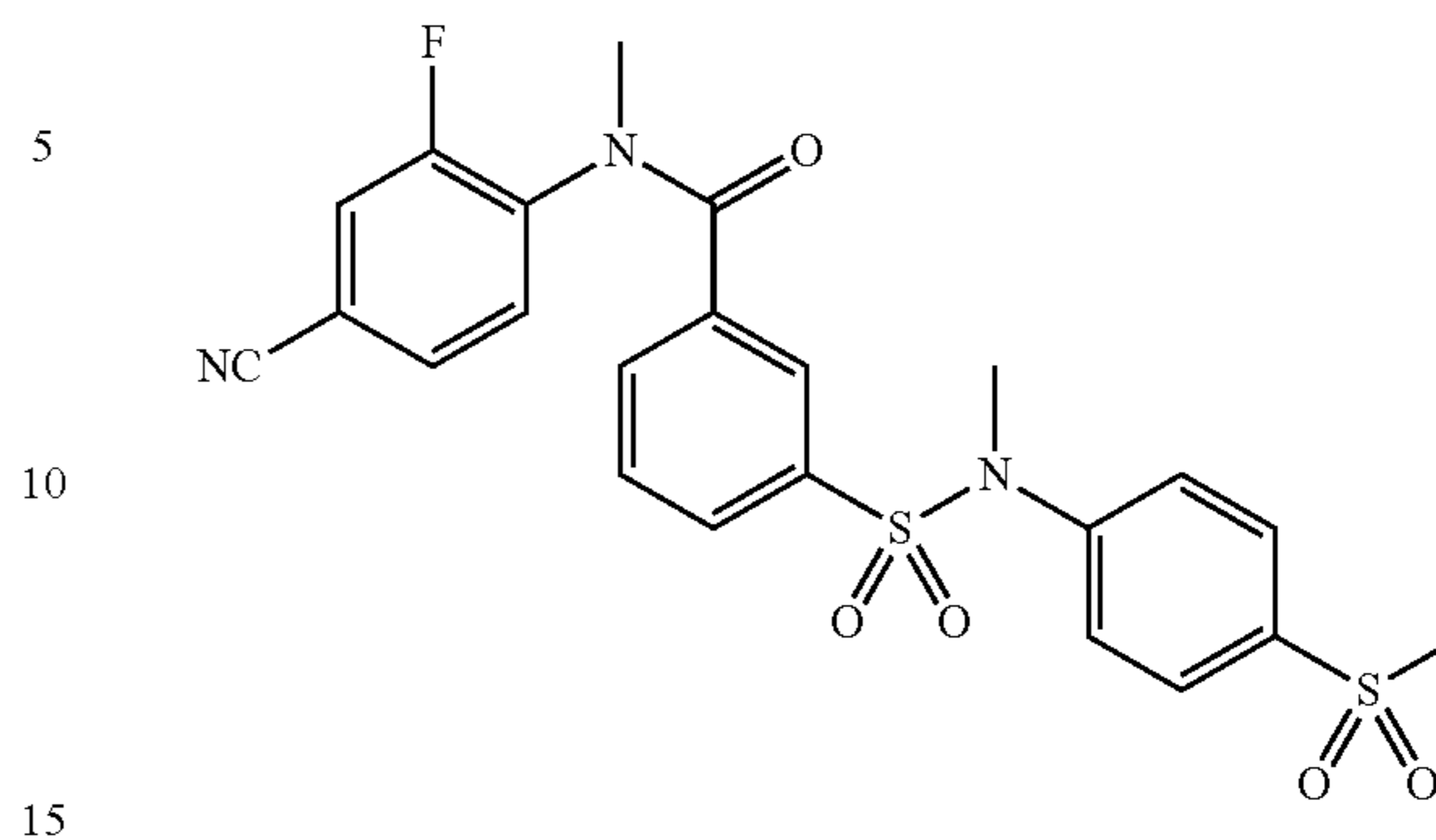
N-(4-cyano-2-fluorophenyl)-N-methyl-3-(N-methyl-N-(4-(methylsulfonyl)phenyl)sulfamoyl)benzamide (203Ak)
