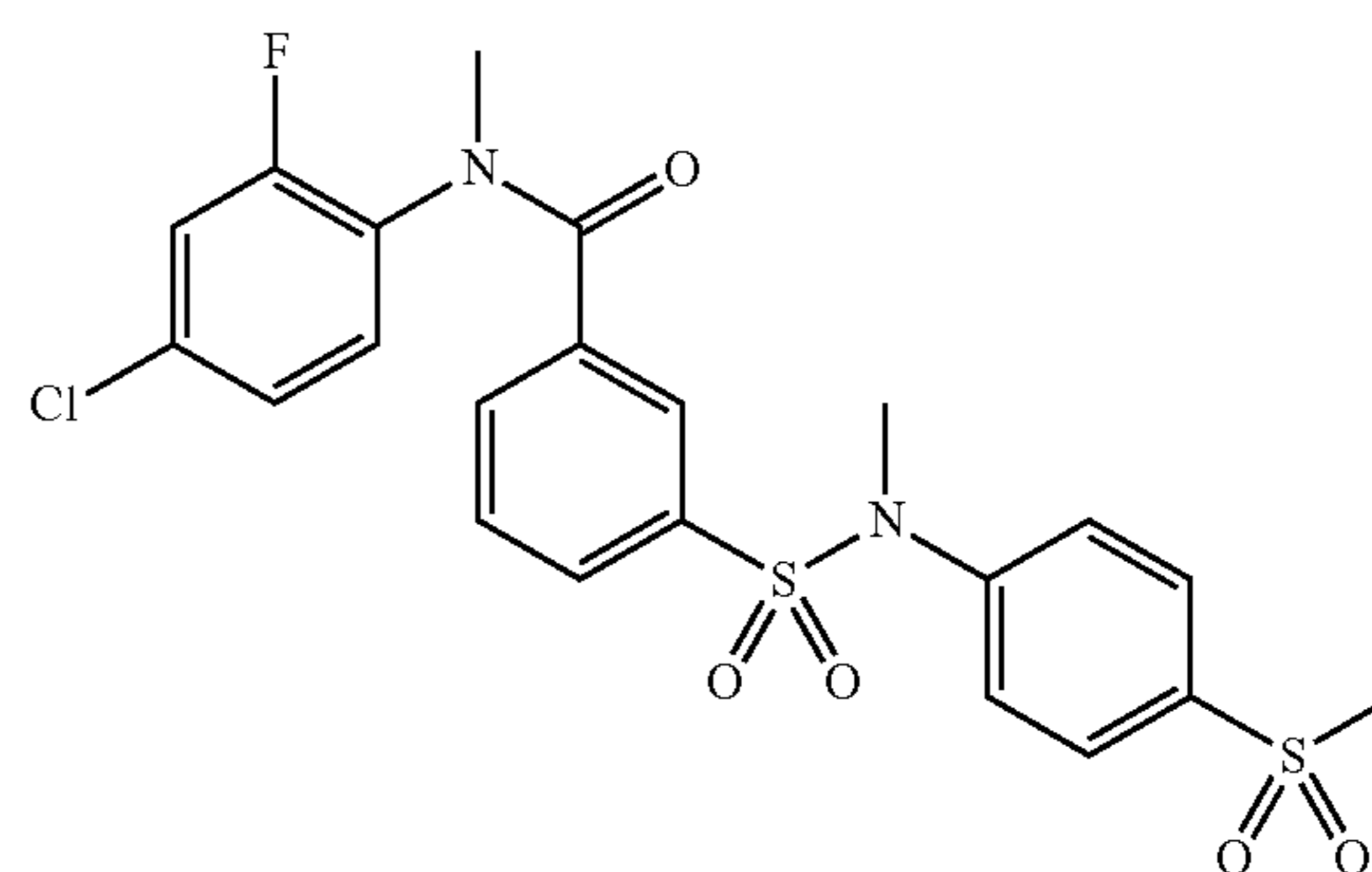
N-(4-chloro-2-fluorophenyl)-N-methyl-3-(N-methyl-N-(4-(methylsulfonyl)phenyl)sulfamoyl)benzamide (203Ah)
