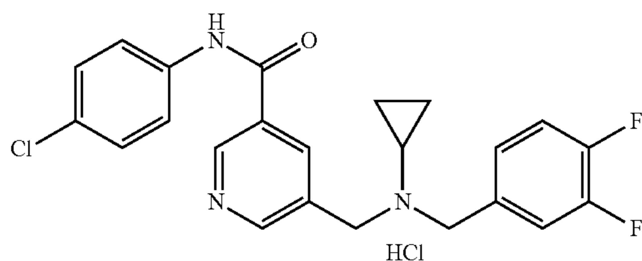
N-(4-chlorophenyl)-5-((cyclopropyl(3,4-difluorobenzyl)amino)methyl)nicotinamide hydrochloride (225t)
