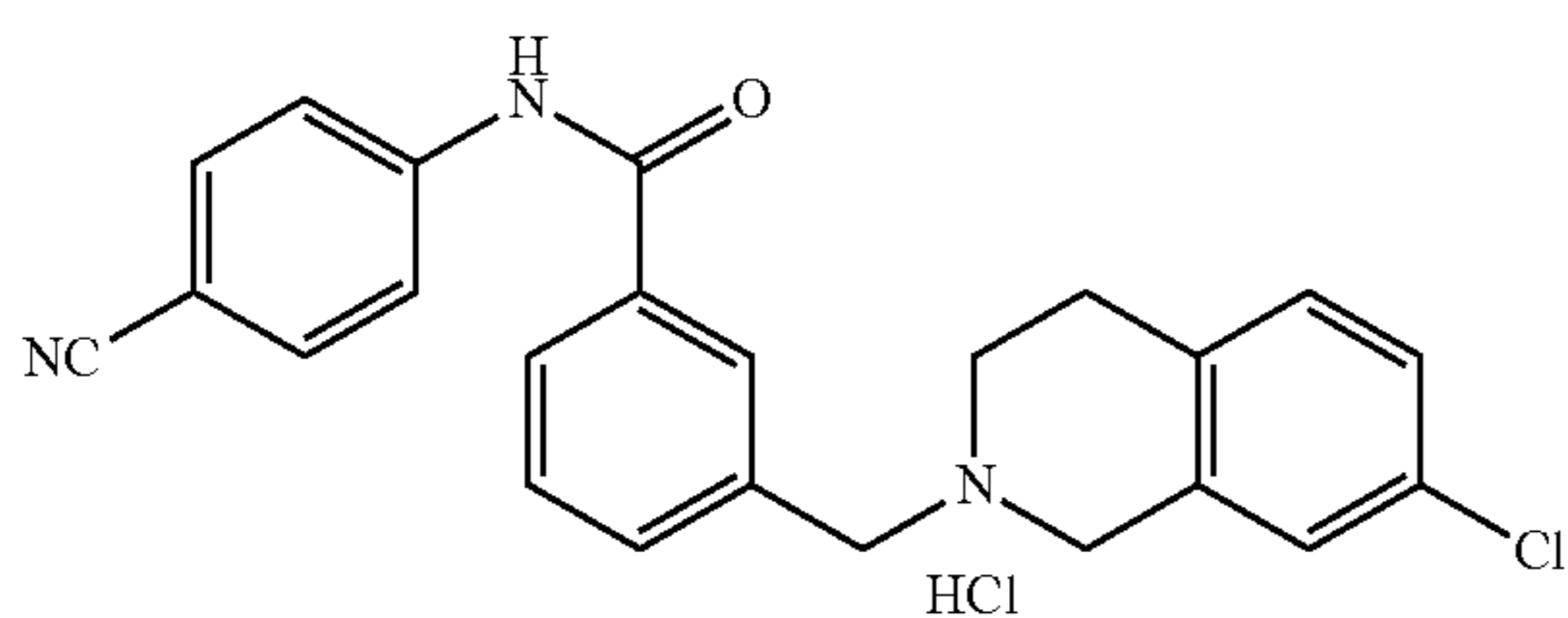
3-((7-chloro-3,4-dihydroisoquinolin-2(1H)-yl)methyl)-N-(4-cyanophenyl)benzamide hydrochloride (225Ag)
