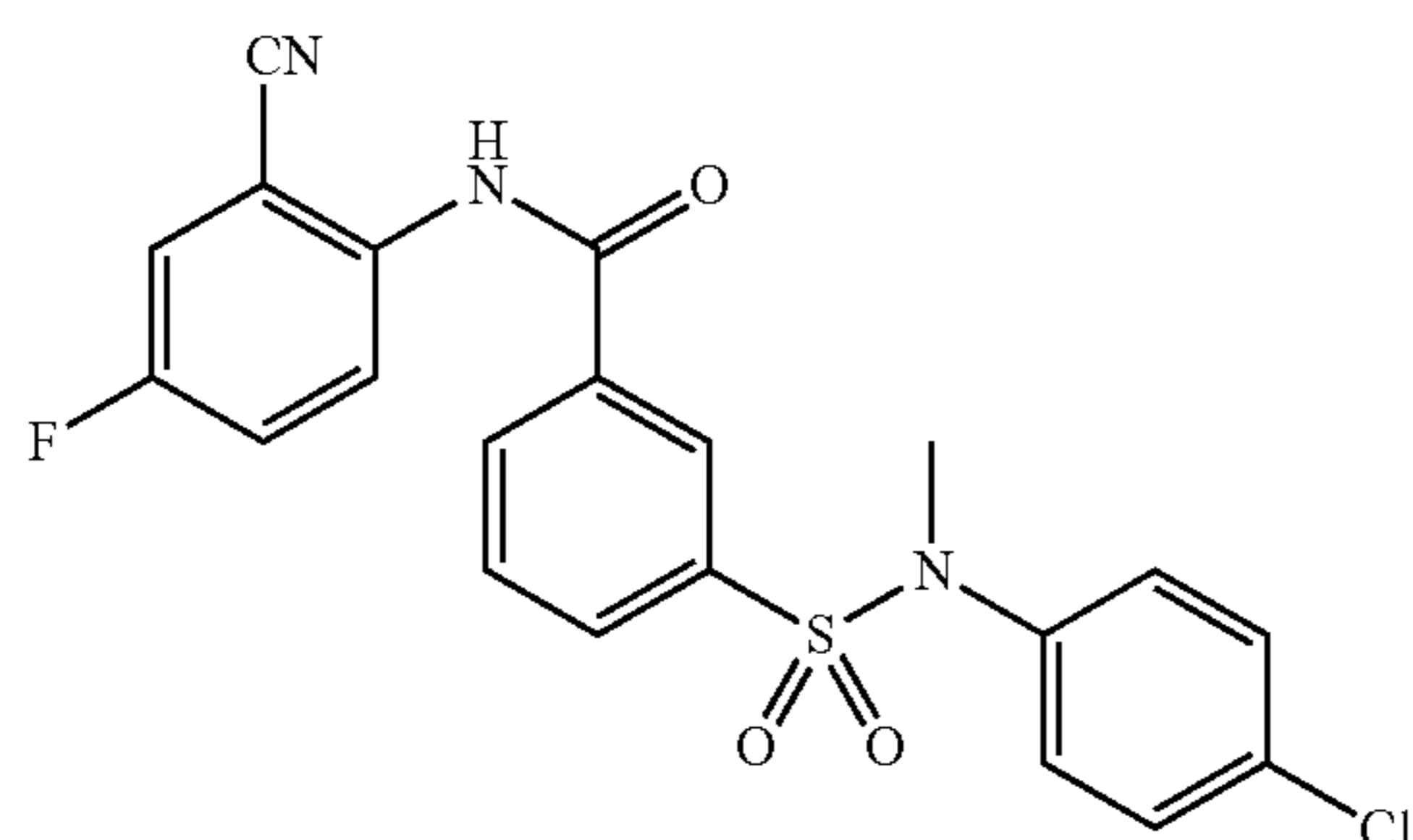
3-(N-(4-chlorophenyl)-N-methylsulfamoyl)-N-(2-cyano-4-fluorophenyl)benzamide (203z)
