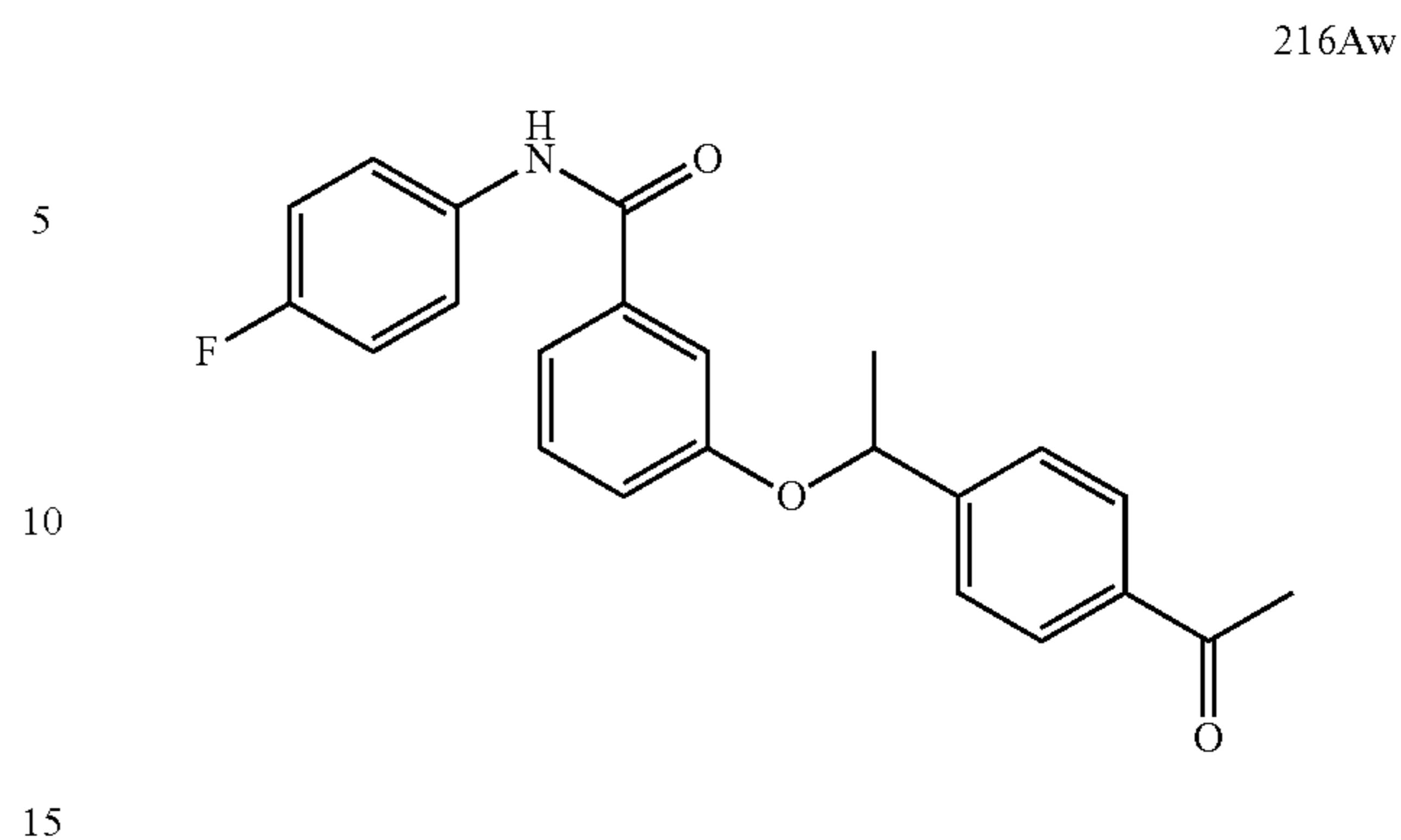
3-(1-(4-acetylphenyl)ethoxy)-N-(4-fluorophenyl)benzamide (216Aw)
