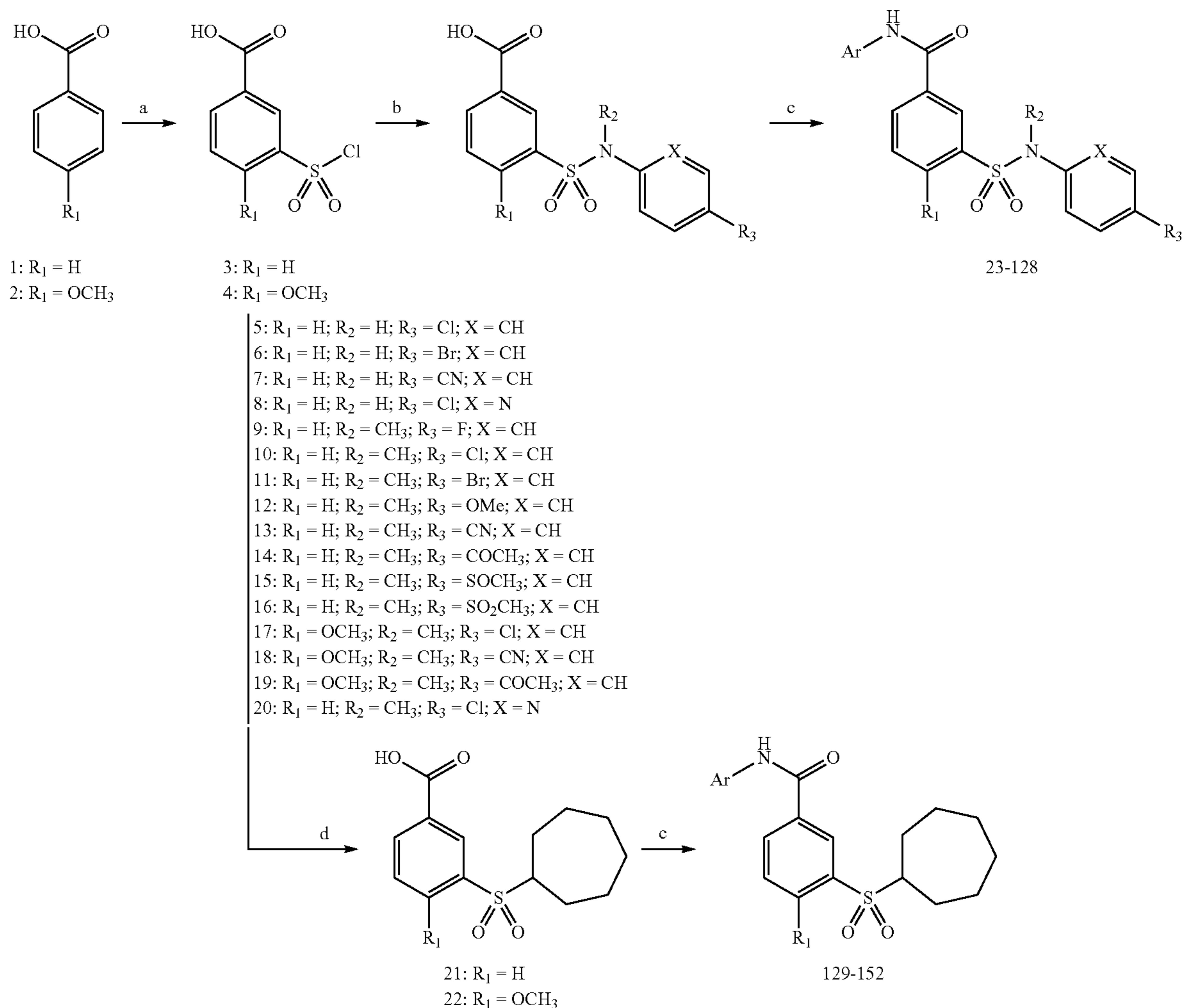
Scheme 1. General synthetic routes to new analogs of C2-8, AK-1, and AK-7
