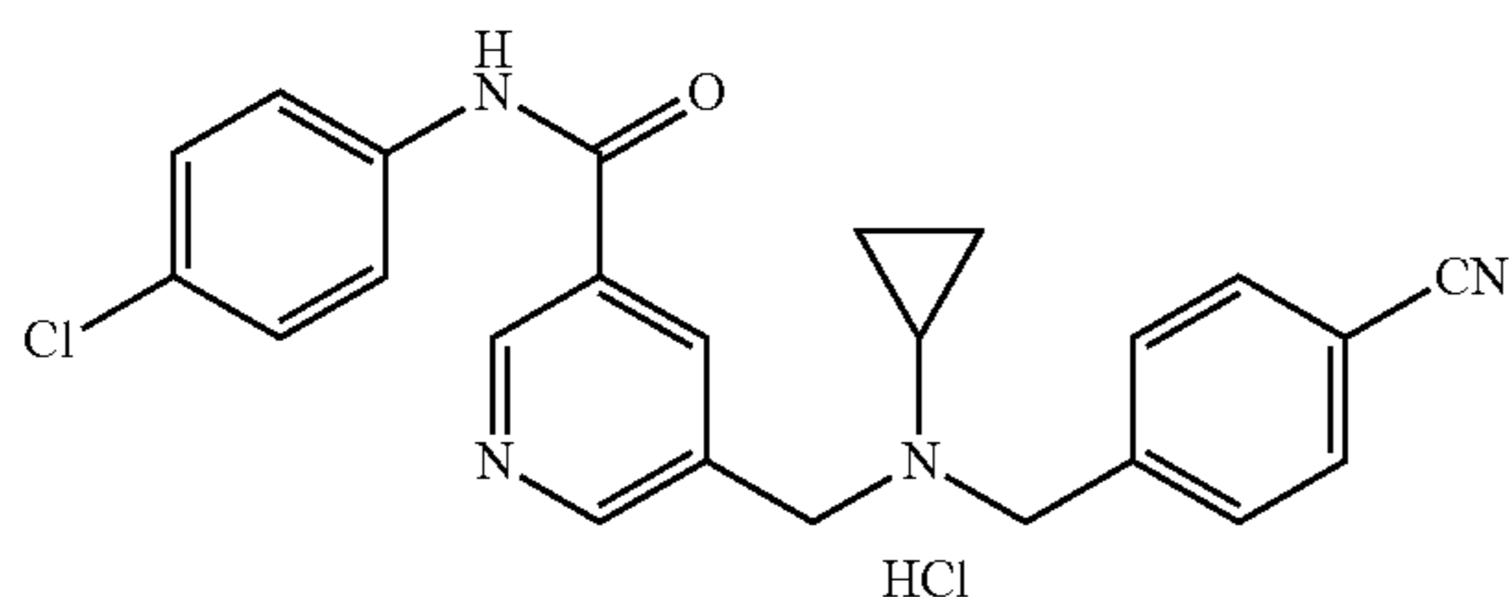
N-(4-chlorophenyl)-5-(((4-cyanobenzyl)(cyclopropyl)amino)methyl)nicotinamide hydrochloride (225o)
