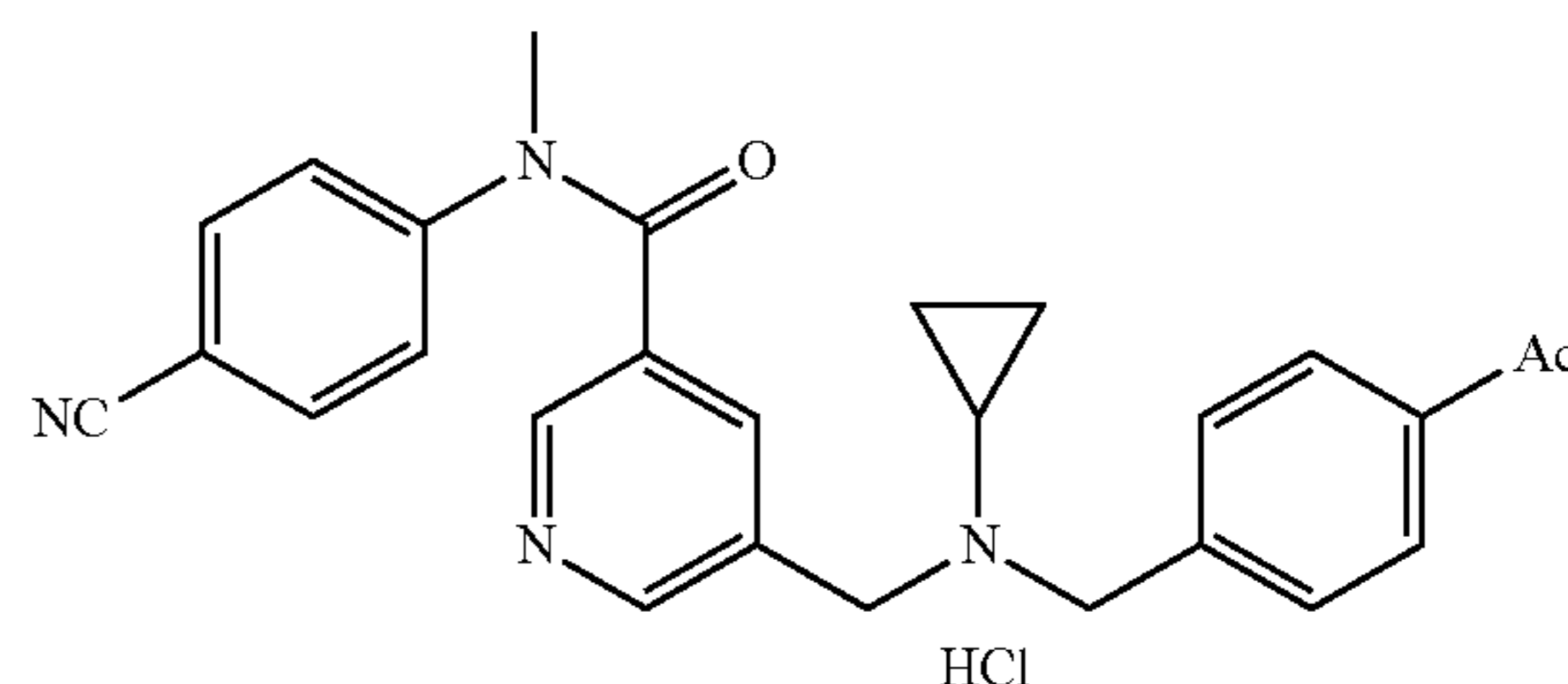
5-(((4-acetylbenzyl)(cyclopropyl)amino)methyl)-N-(4-cyanophenyl)-N-methylnicotinamide hydrochloride (225s)
