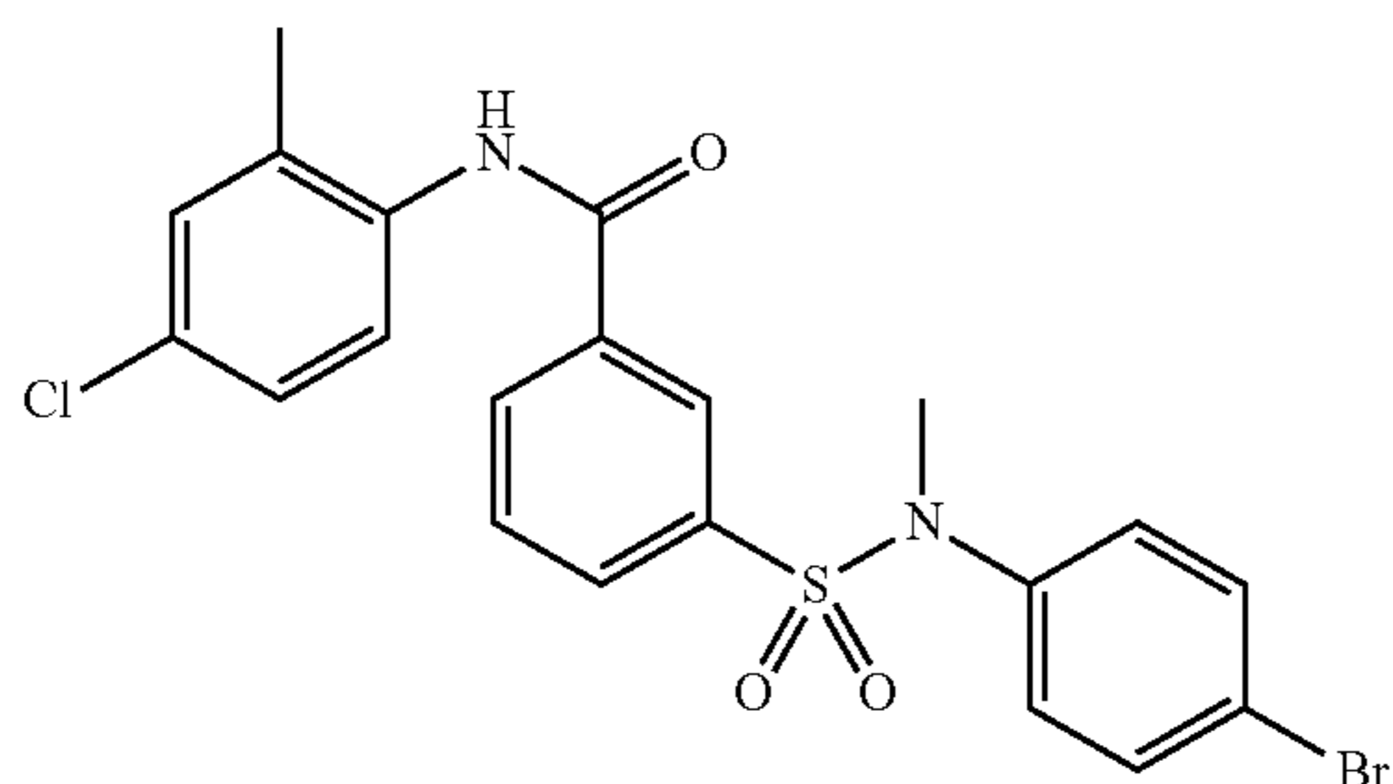
3-(N-(4-bromophenyl)-N-methylsulfamoyl)-N-(4-chloro-2-methylphenyl)benzamide (203n)
