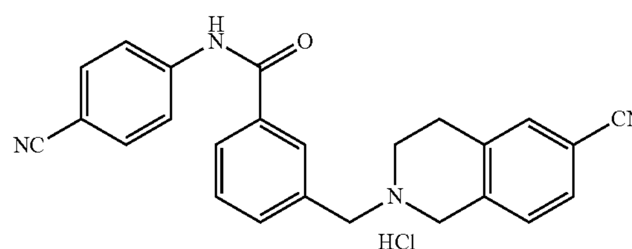
3-((6-cyano-3,4-dihydroisoquinolin-2(1H)-yl)methyl)-N-(4-cyanophenyl)benzamide hydrochloride (225Ai)
