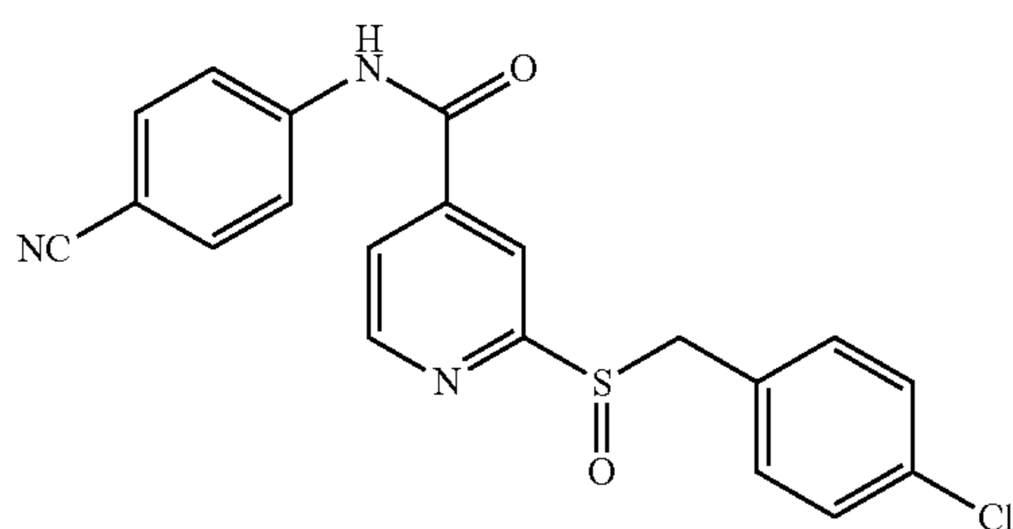
2-((4-chlorobenzyl)sulfinyl)-N-(4-cyanophenyl)isonicotinamide (235a)
