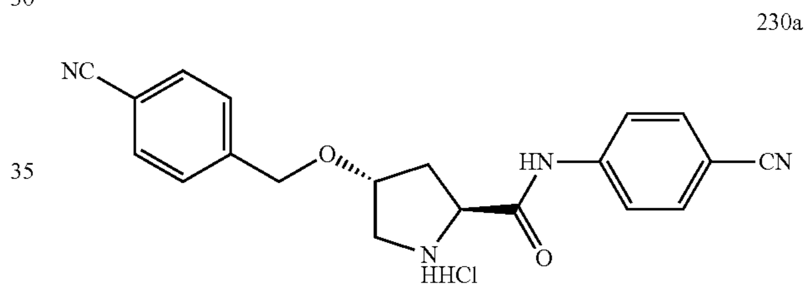
(2S,4R)-4-((4-cyanobenzyl)oxy)-N-(4-cyanophenyl)pyrrolidine-2-carboxamide hydrochloride (230a)
