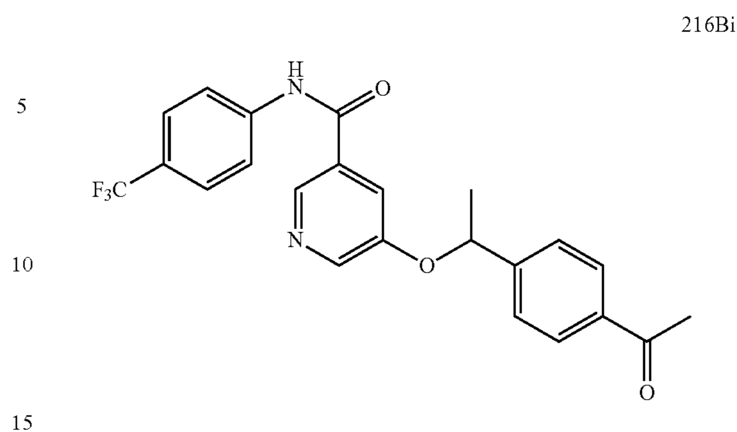
5-(1-(4-acetylphenyl)ethoxy)-N-(4-(trifluoromethyl) phenyl)nicotinamide (216Bi)
