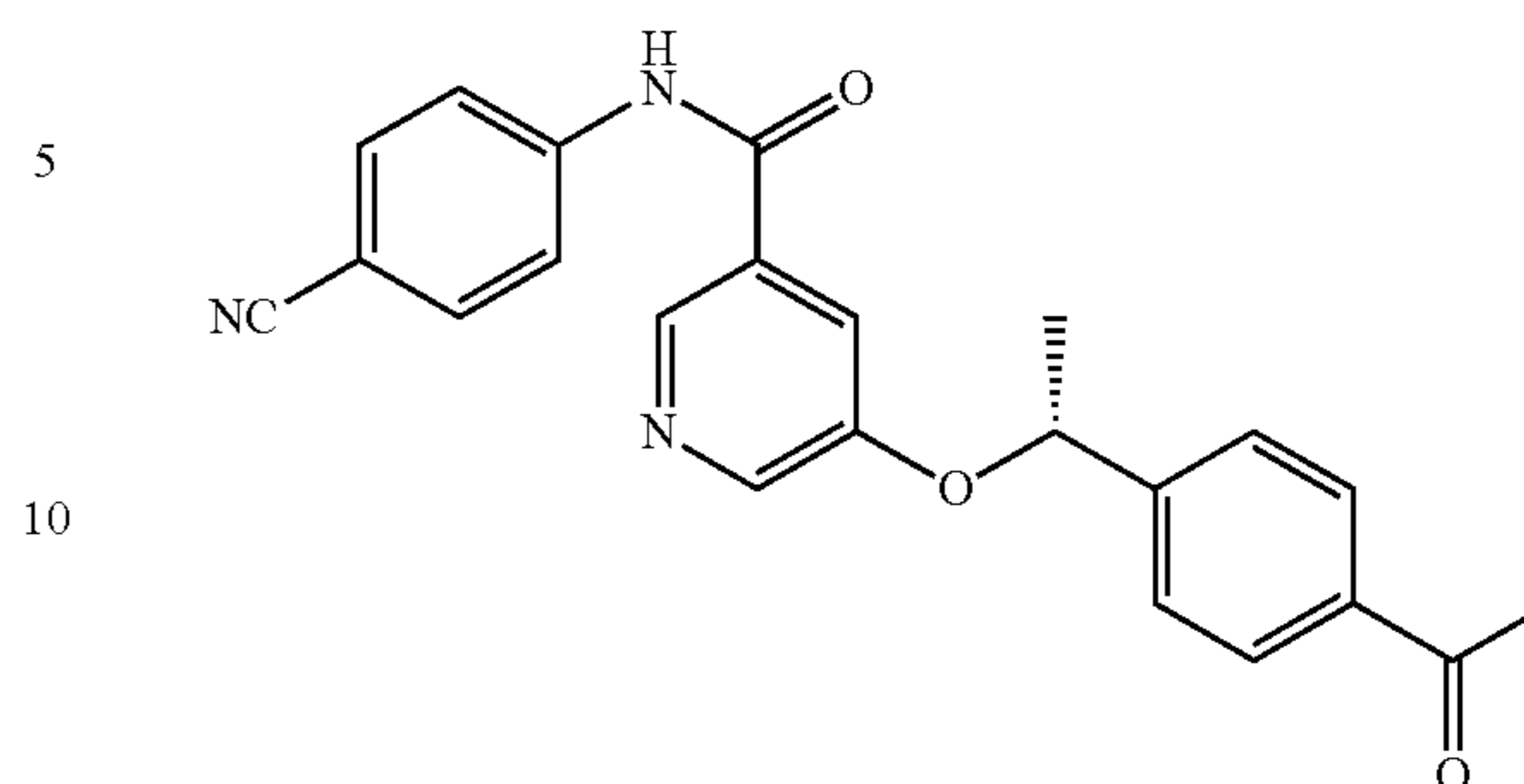
(R)-5-(1-(4-acetylphenyl)ethoxy)-N-(4-cyanophenyl)nicotinamide (216An)
