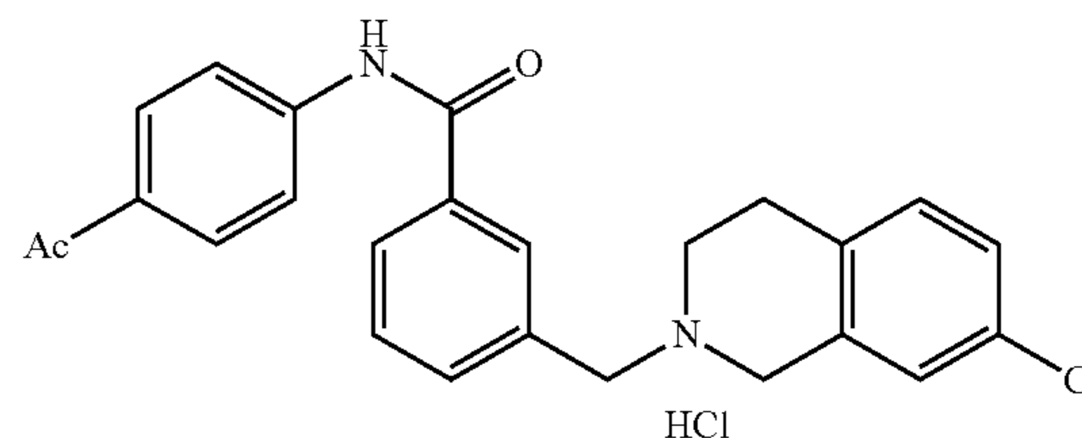
N-(4-acetylphenyl)-3-((7-chloro-3,4-dihydroisoquinolin-2(1H)-yl)methyl)benzamide hydrochloride (225Ah)
