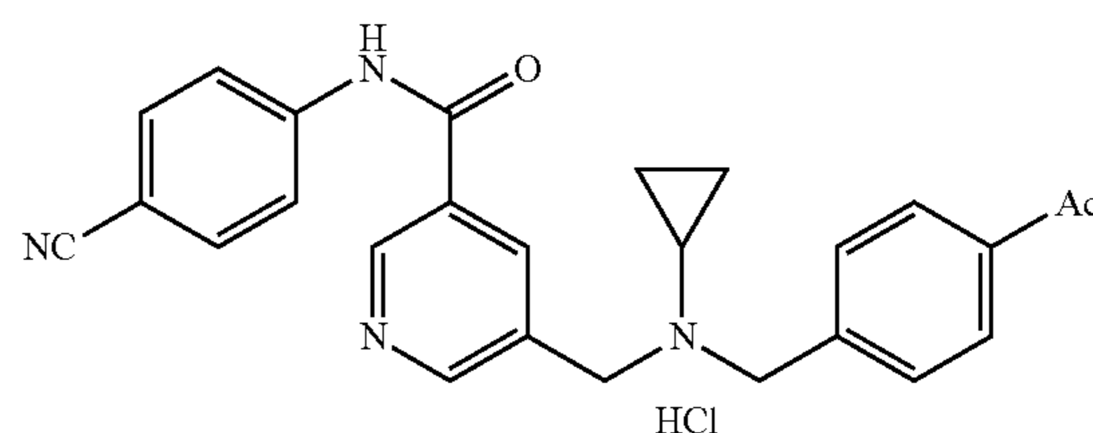
5-(((4-acetylbenzyl)(cyclopropyl)amino)methyl)-N-(4-cyanophenyl)nicotinamide hydrochloride (225r)
