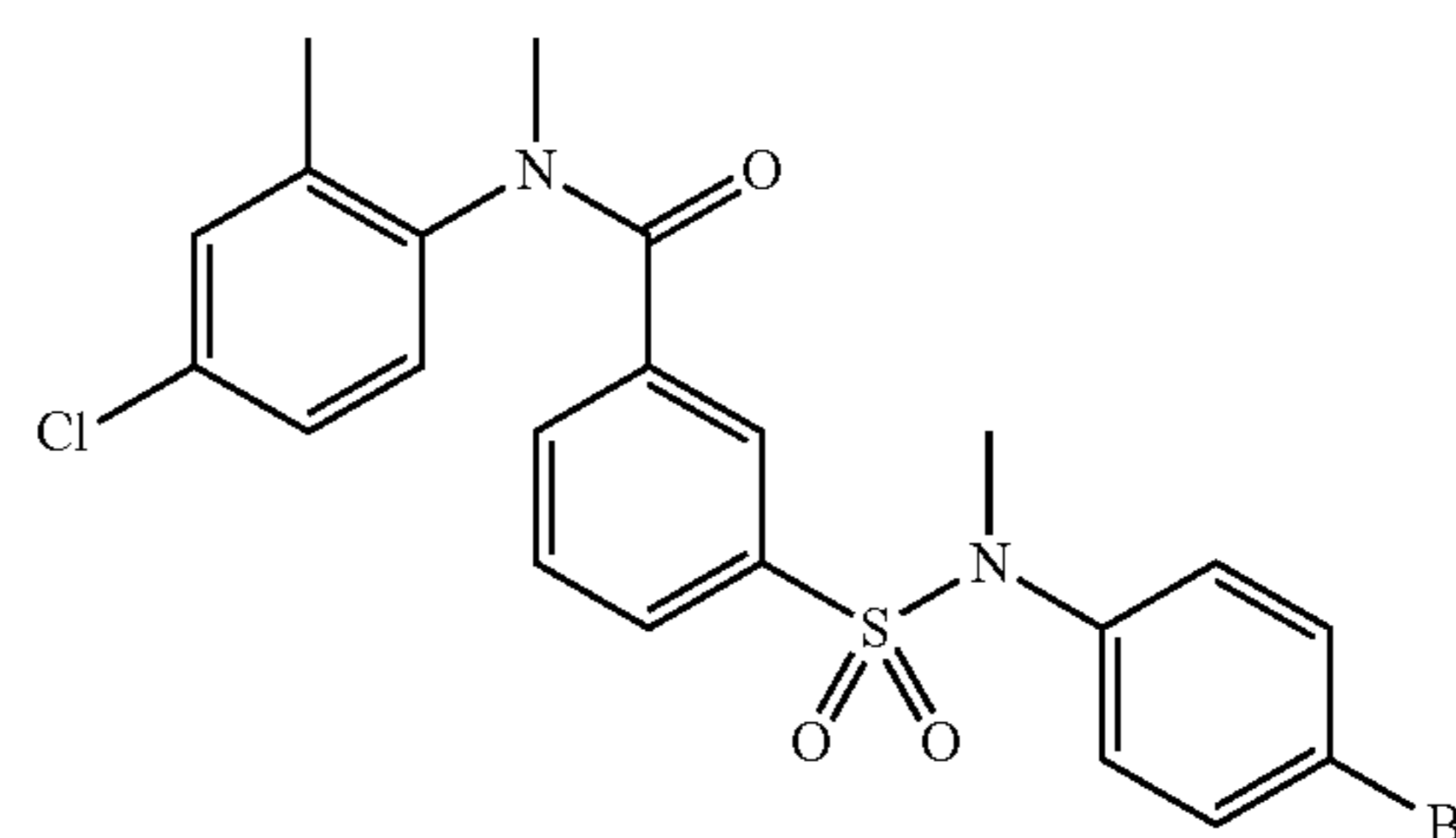
3-(N-(4-bromophenyl)-N-methylsulfamoyl)-N-(4-chloro-2-methylphenyl)-N-methylbenzamide (203l)
