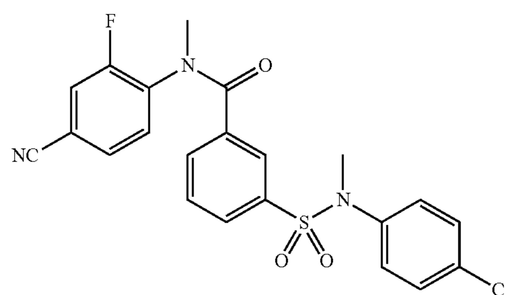
3-(N-(4-chlorophenyl)-N-methylsulfamoyl)-N-(4-cyano-2-fluorophenyl)-N-methylbenzamide (203Ac)
