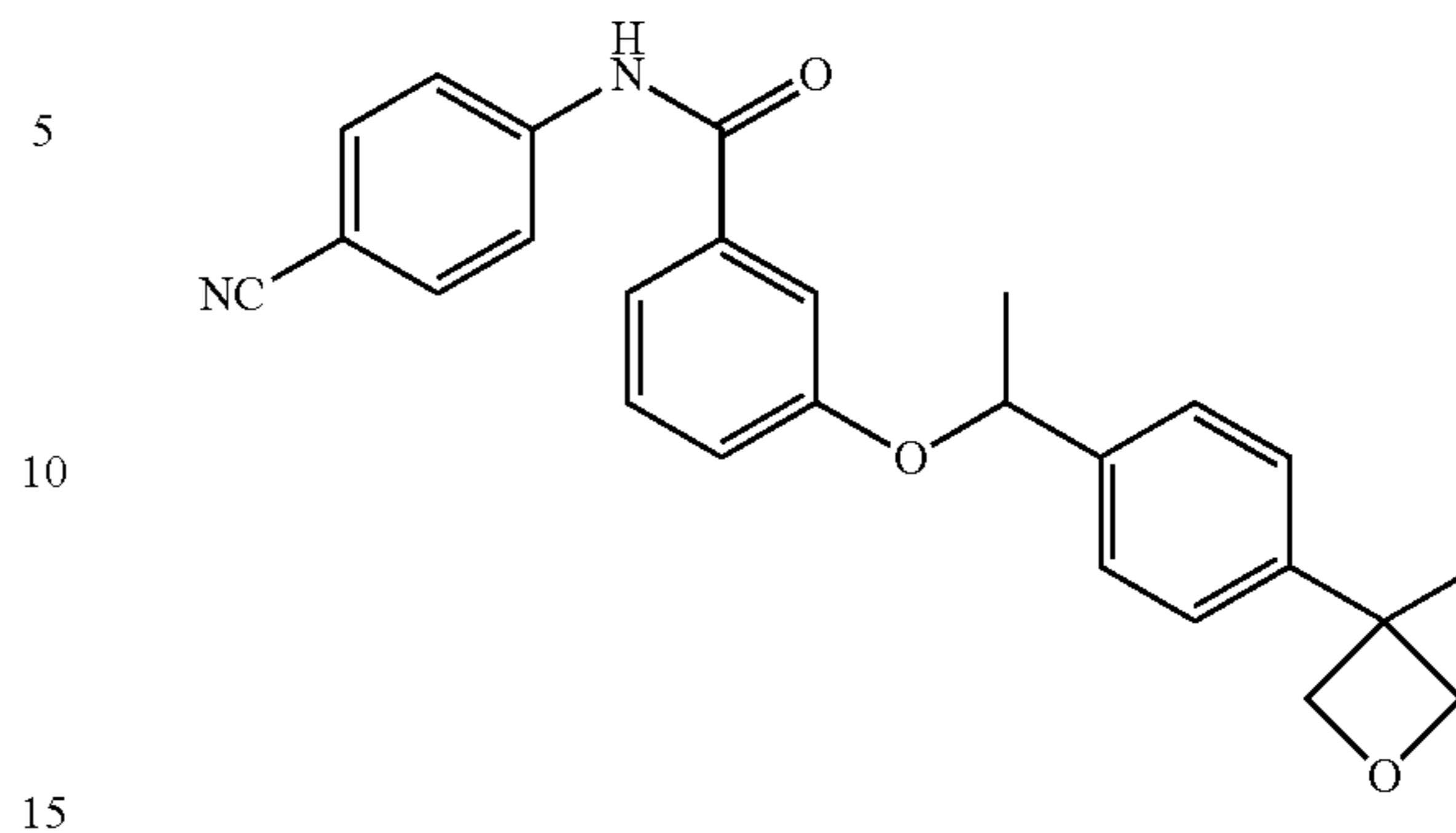
N-(4-cyanophenyl)-3-(1-(4-(3-methyloxetan-3-yl)phenyl)ethoxy)benzamide (216Aj)
