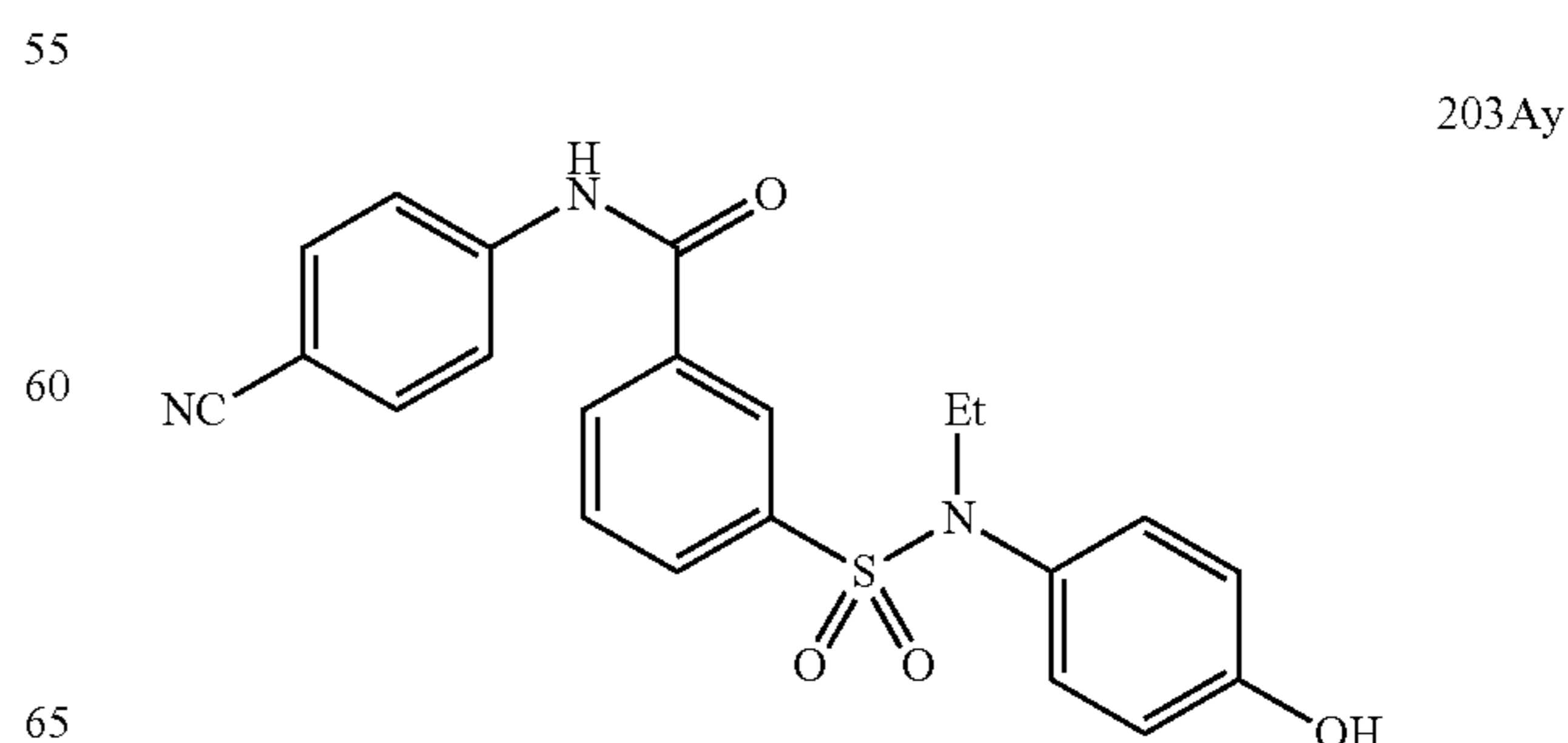
3-(N-(4-chlorophenyl)-N-cyclopropylsulfamoyl)-N-(4-cyanophenyl)benzamide (203Av)
