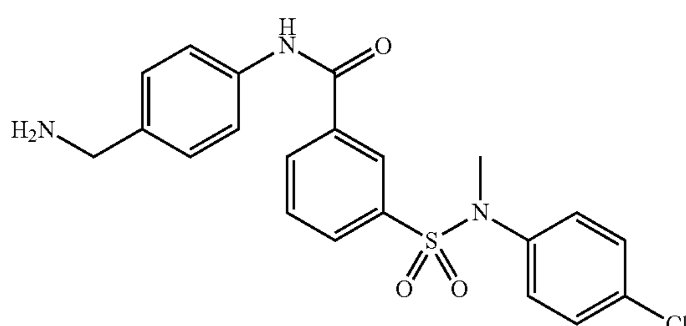
N-(4-(aminomethyl)phenyl)-3-(N-(4-chlorophenyl)-N-methylsulfamoyl)benzamide (203Aa)
