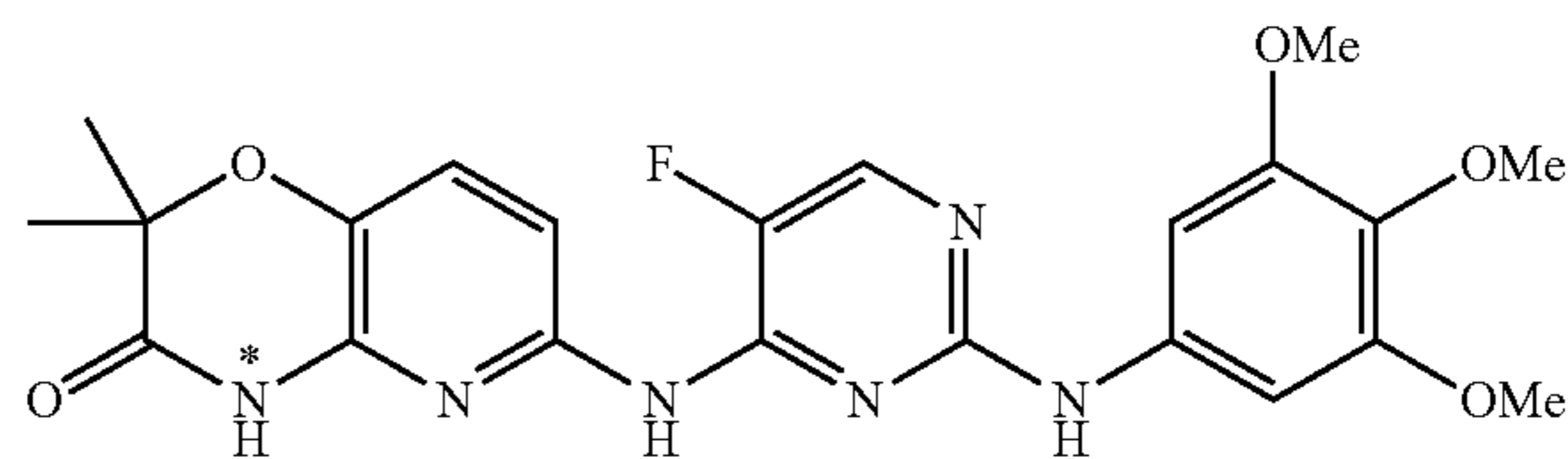
Compound 1
