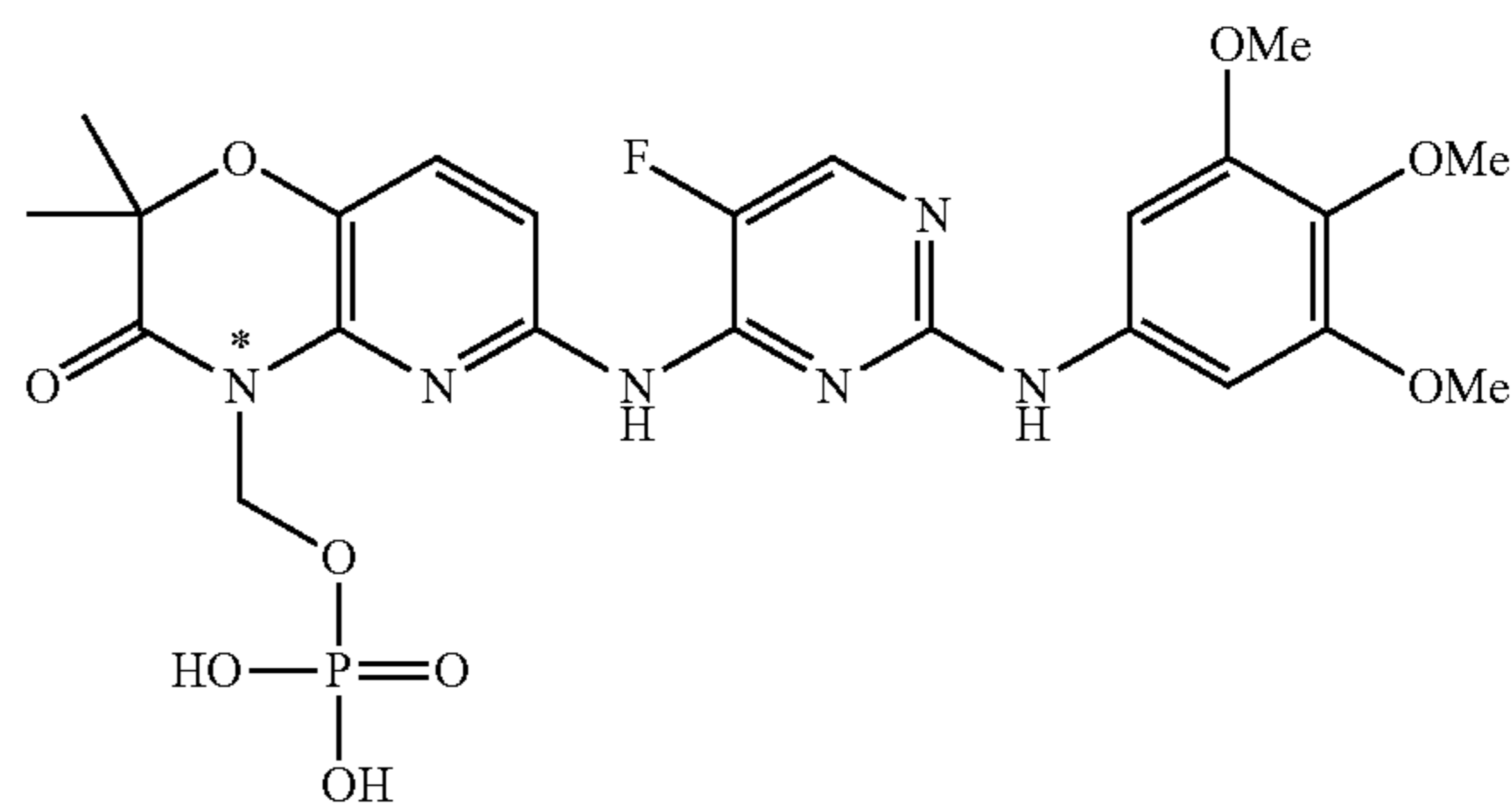
Compound 4
