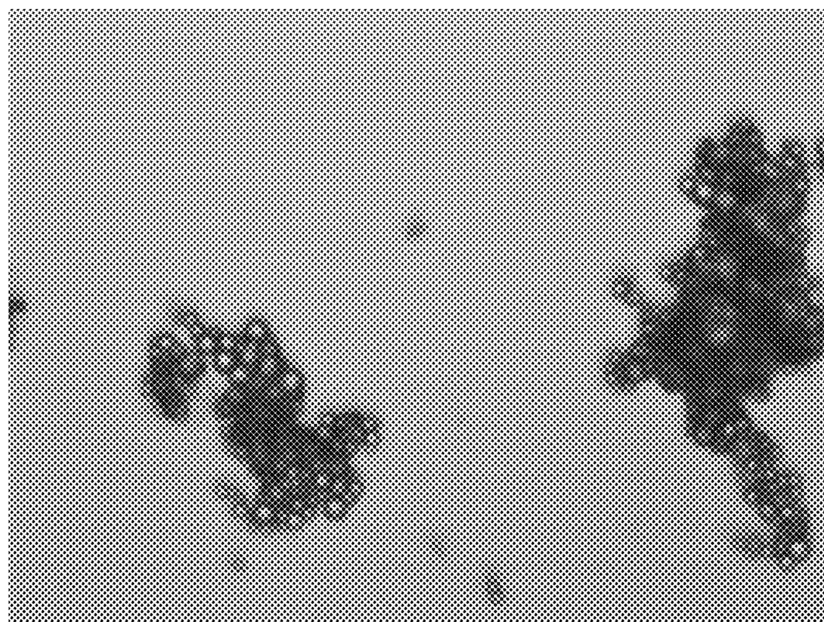
Figure 6: Optical microscopy image of cocoamidopropylamine oxide special-treated silica capsules, 4 days after drying on glass slide.
