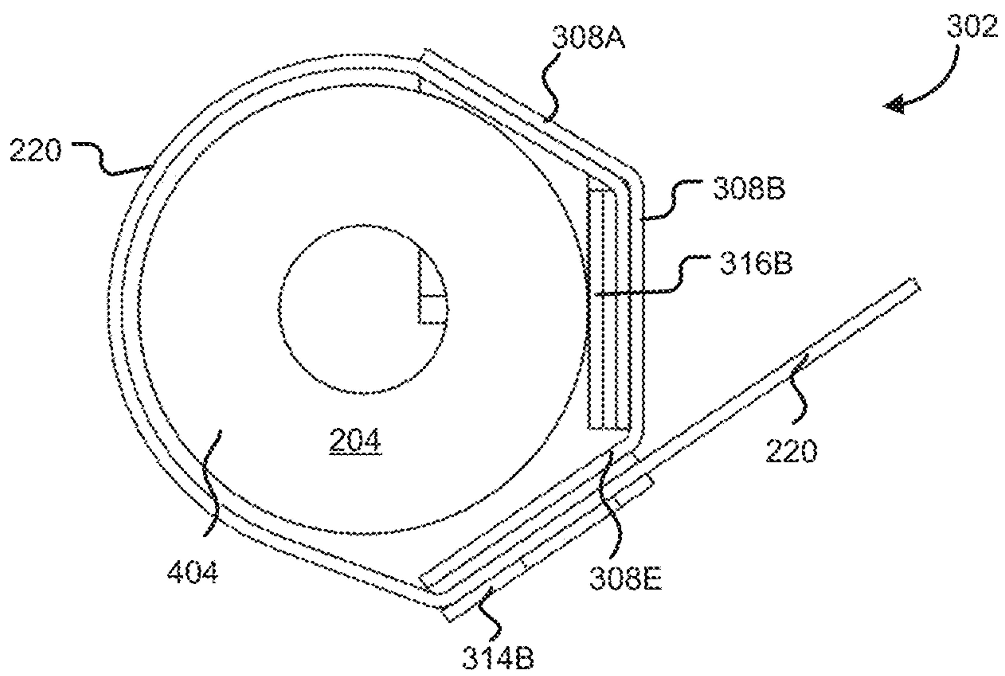
Section C-C
