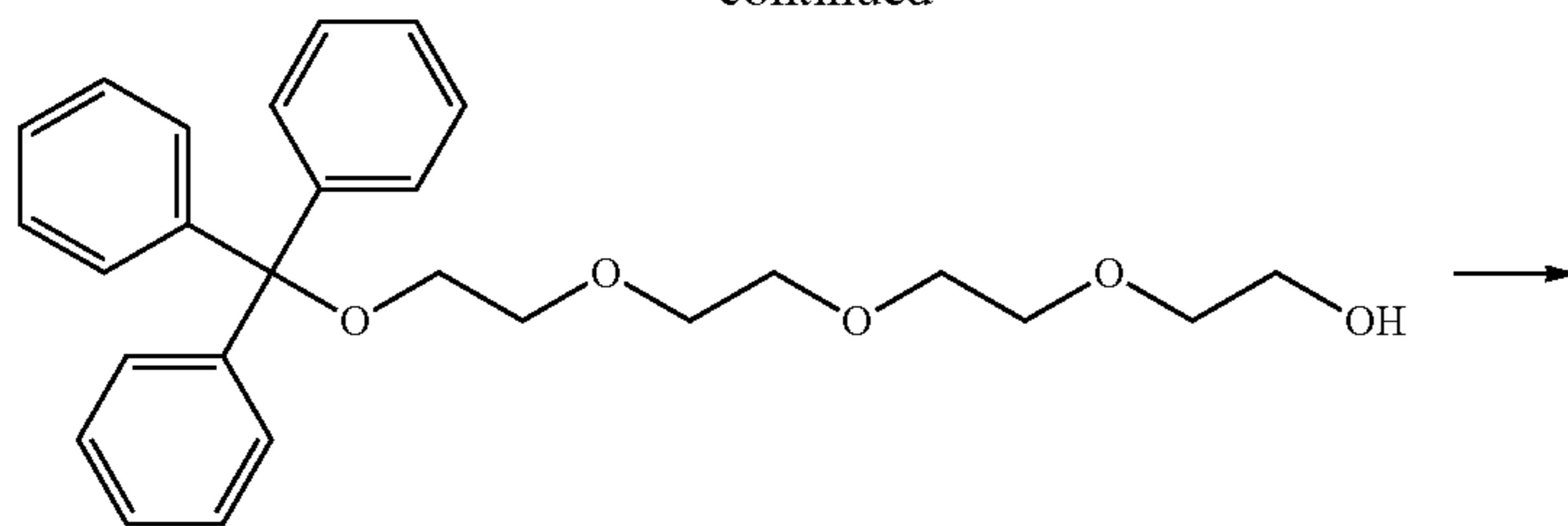
Compound 2
