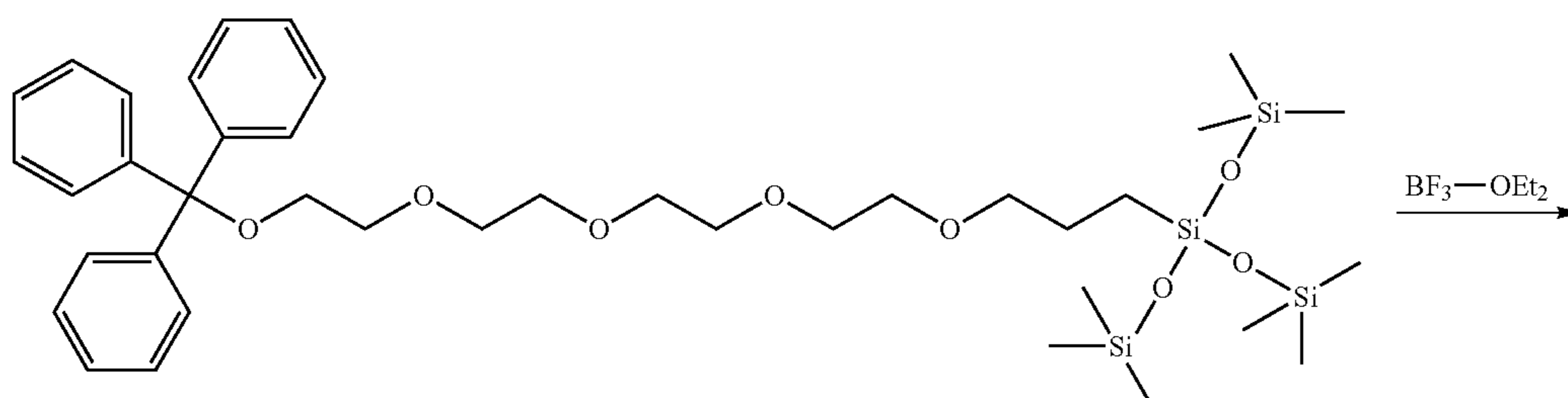
Compound 4
