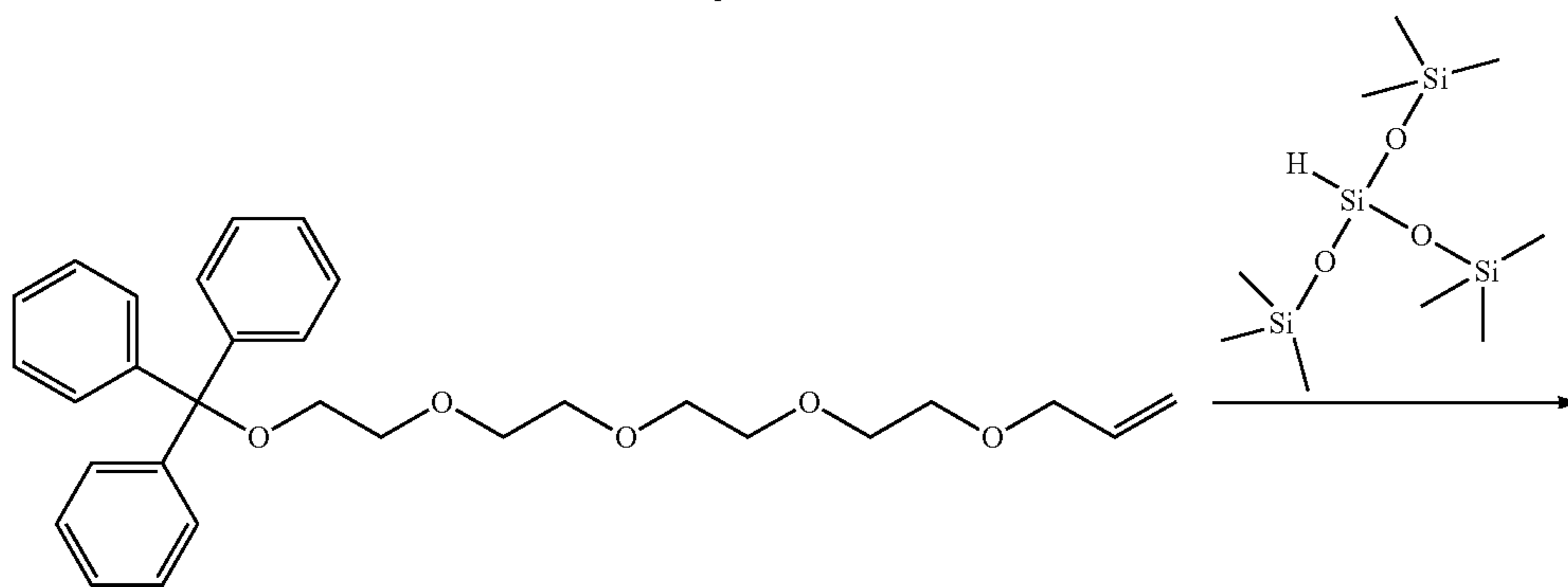
Compound 3
