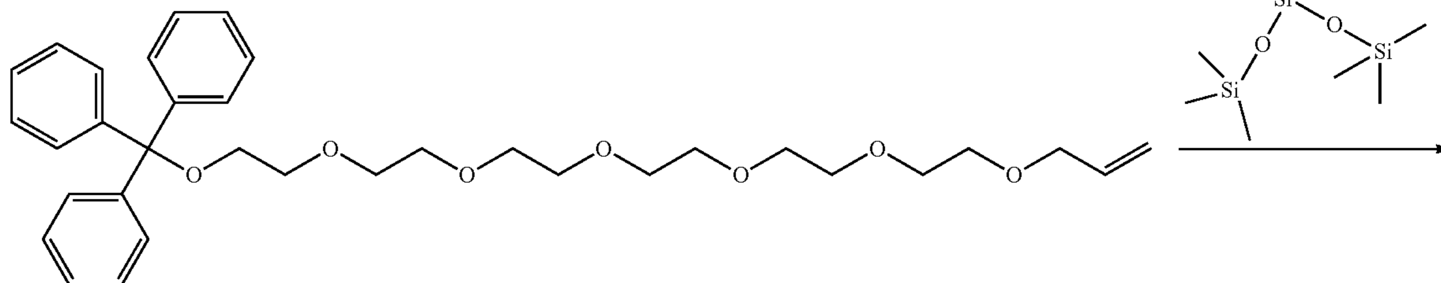
Compound 8
