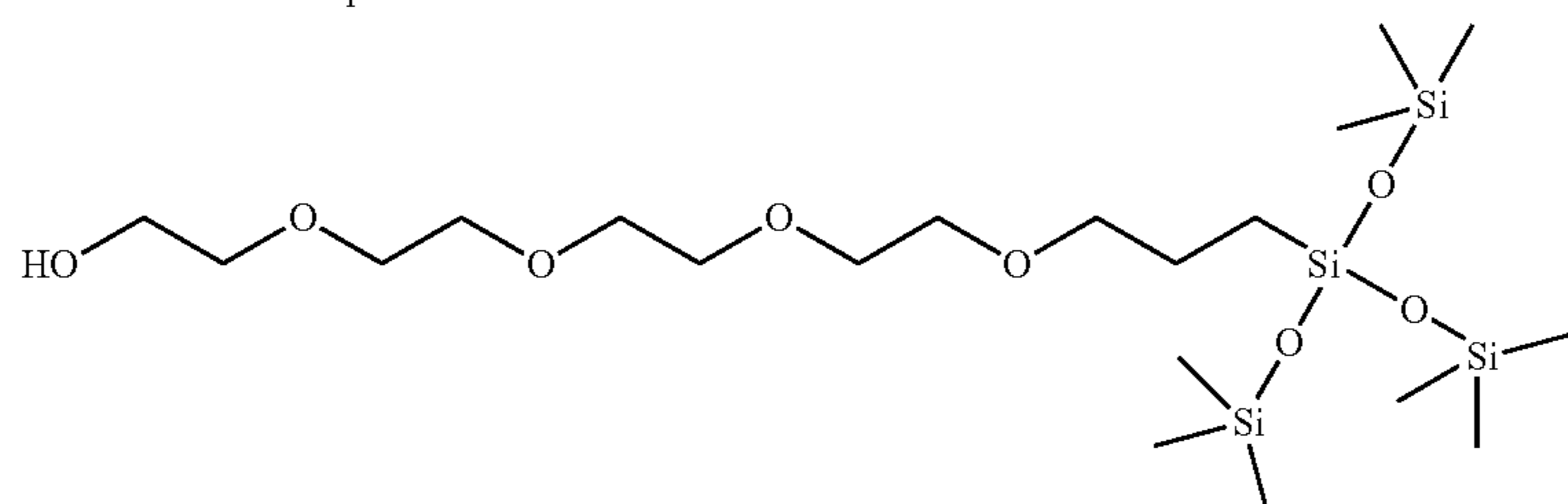
Compound 5
