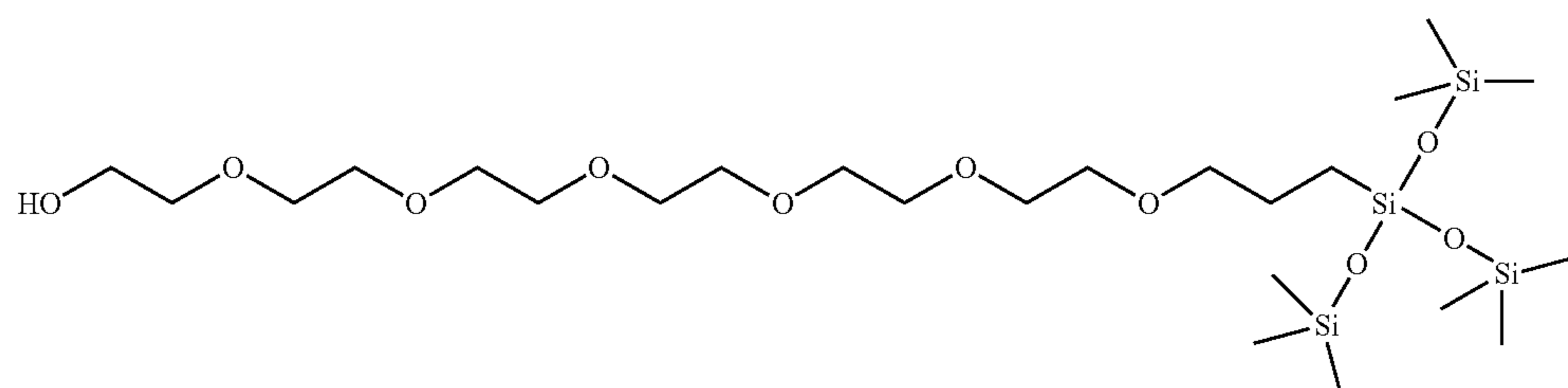
Compound 10
