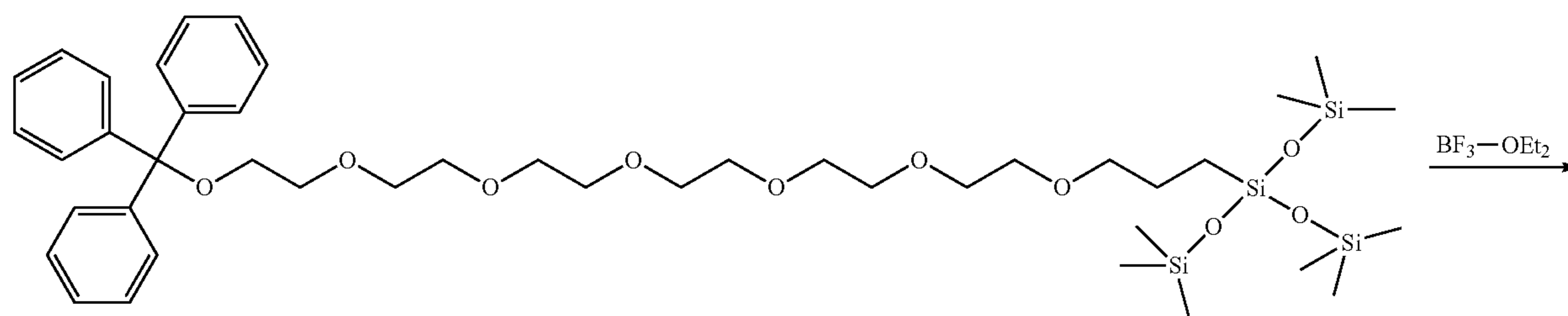
Compound 9
