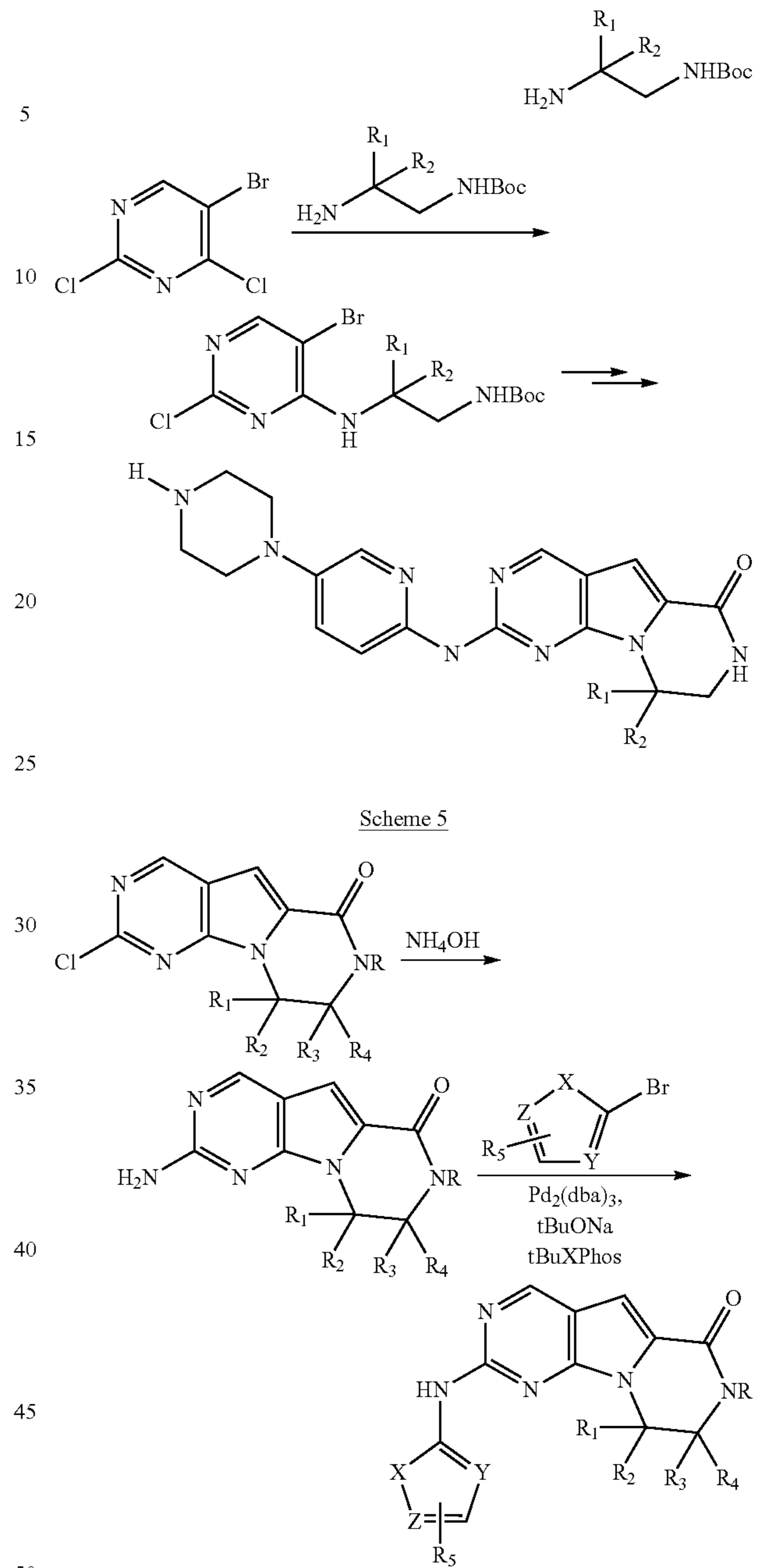
Scheme 6
