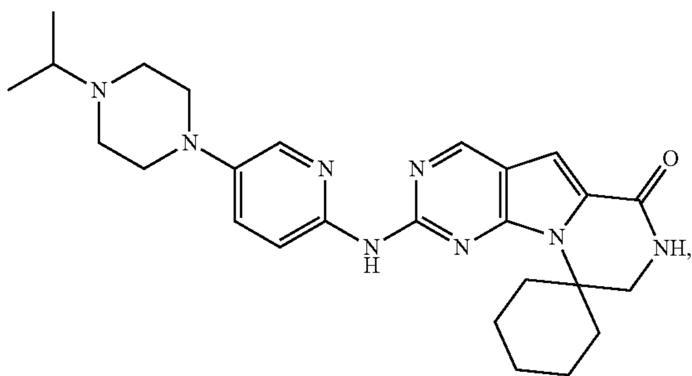
Compound GG
