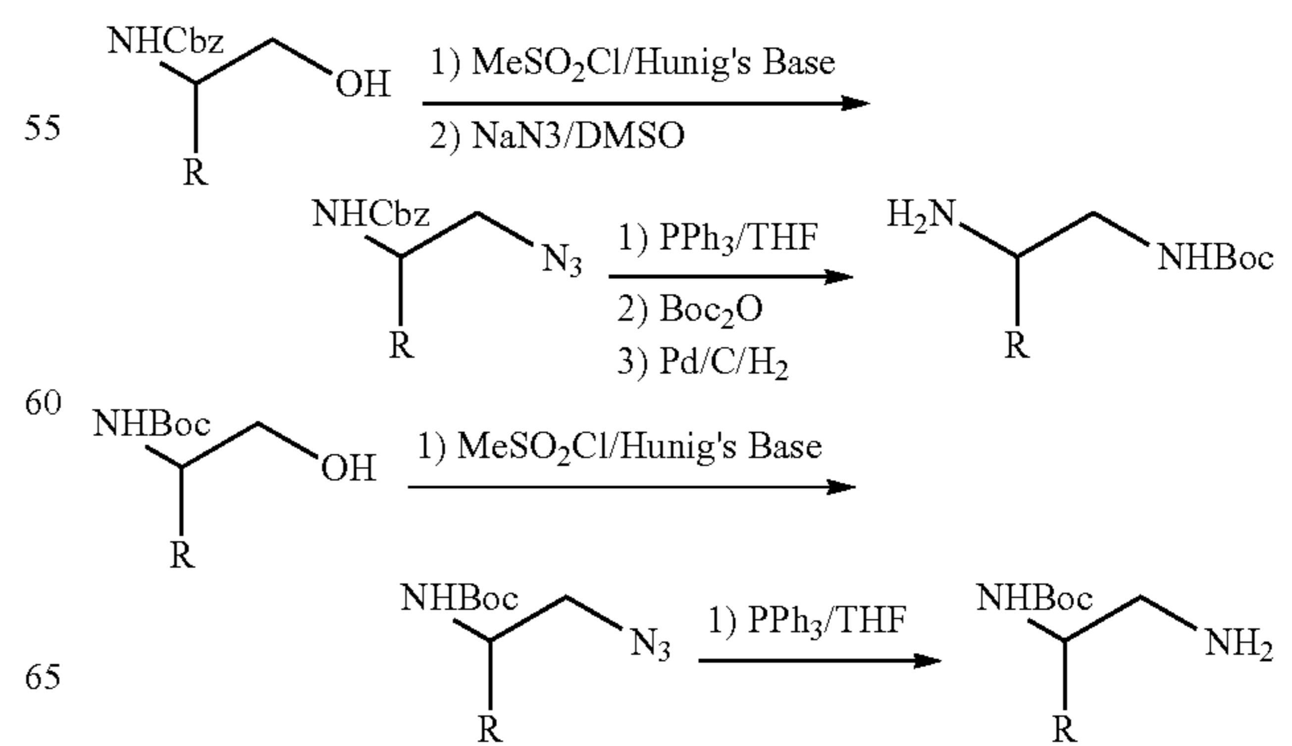
Scheme 6
