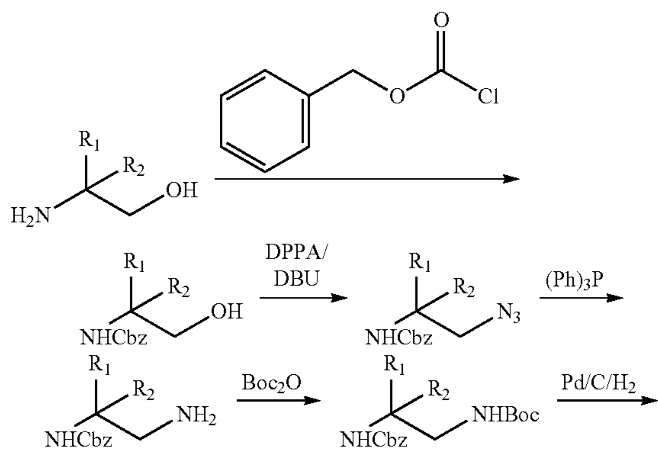
Scheme 4
