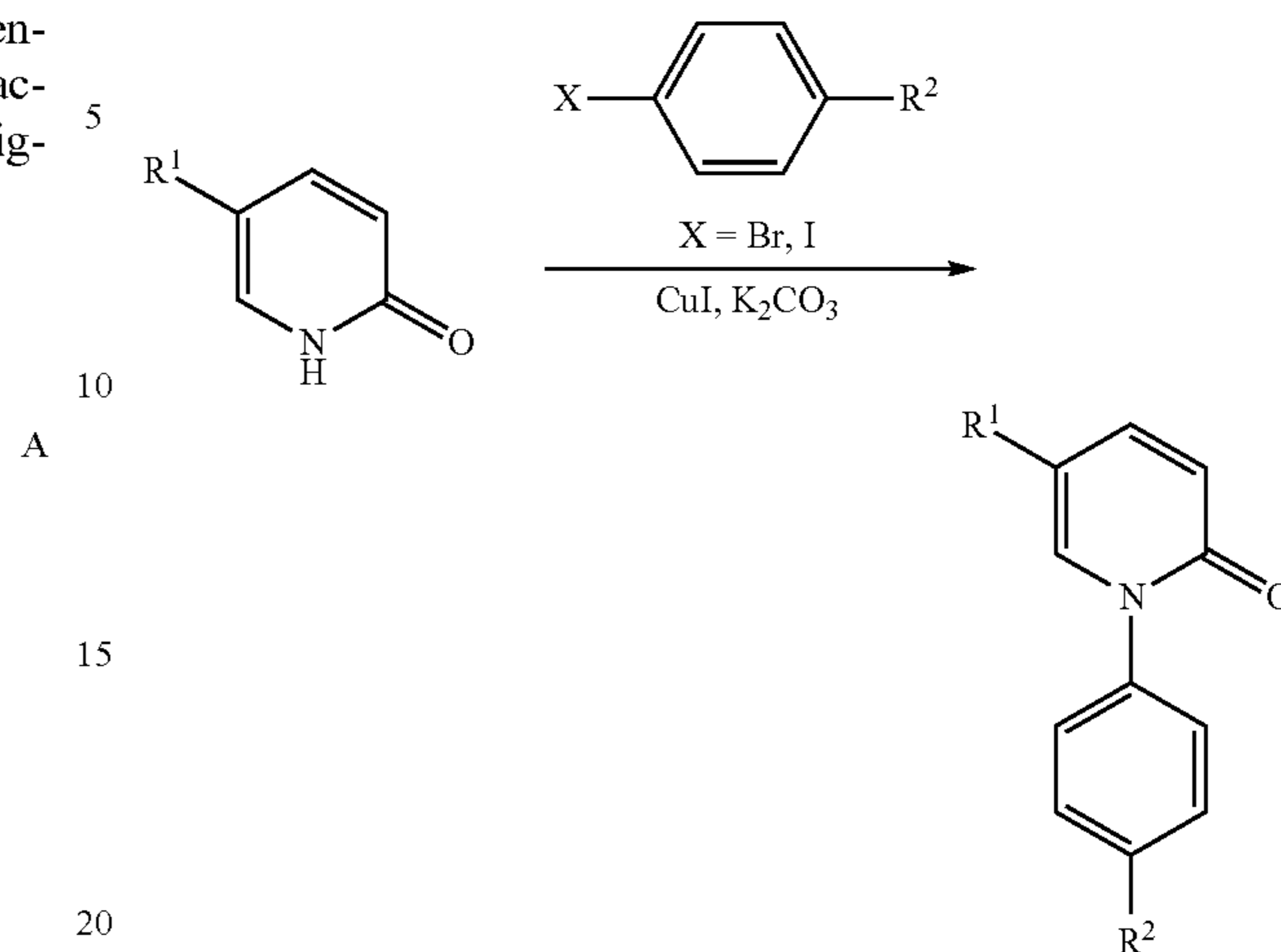
Synthetic Scheme 2
