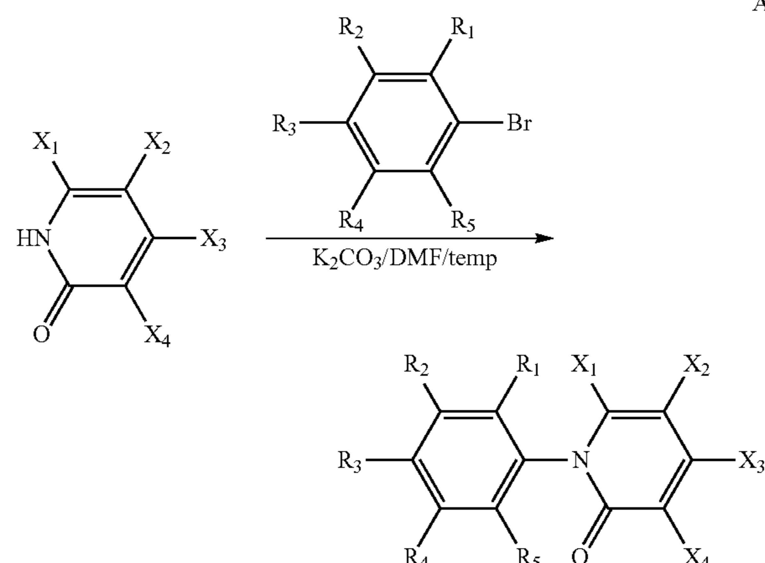
Synthetic Scheme 1
