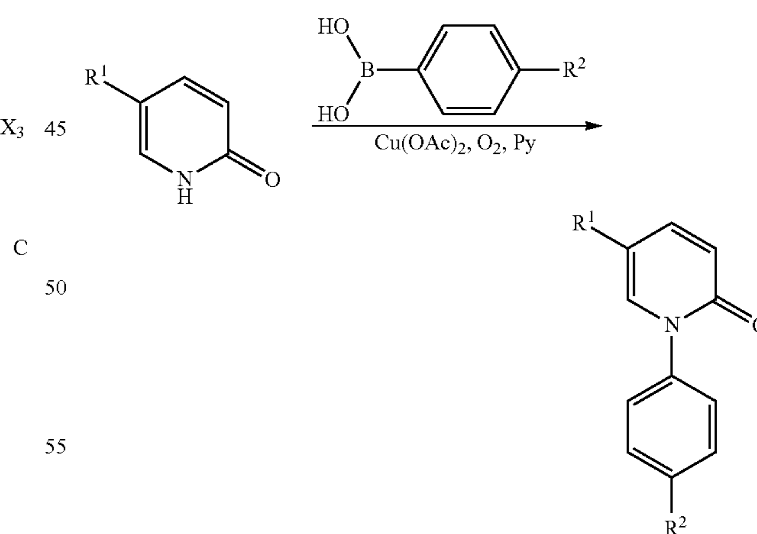
Synthetic Scheme 3
