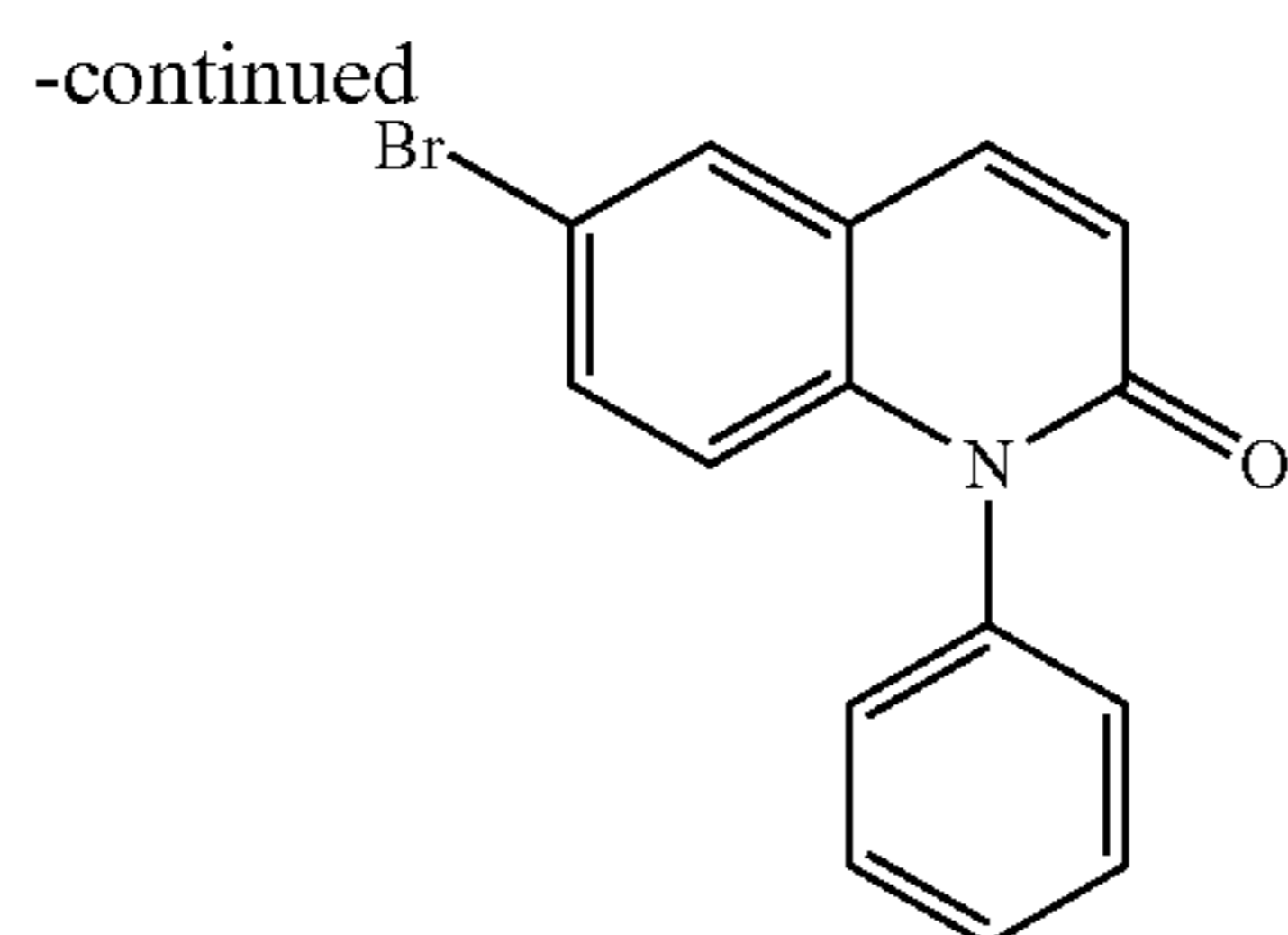
Compound 33
