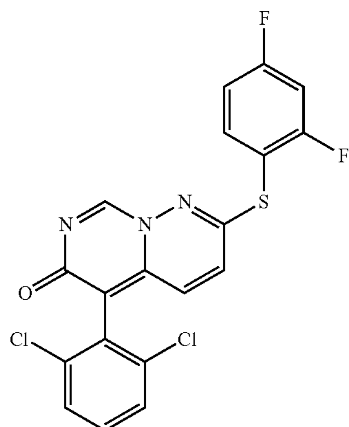
P8 VX-745
