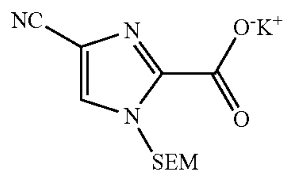
a) 1H-Imidazole-4-carbonitrile
