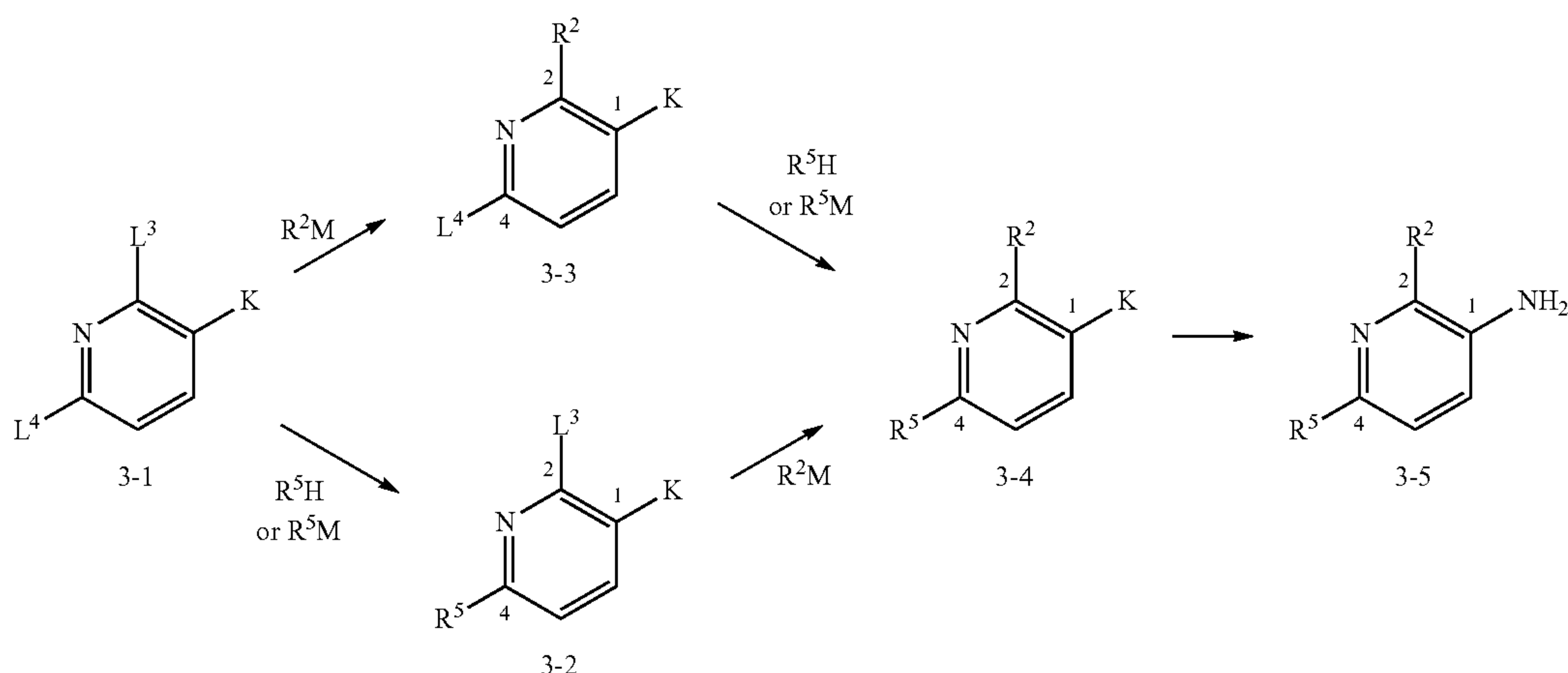
Scheme 3
