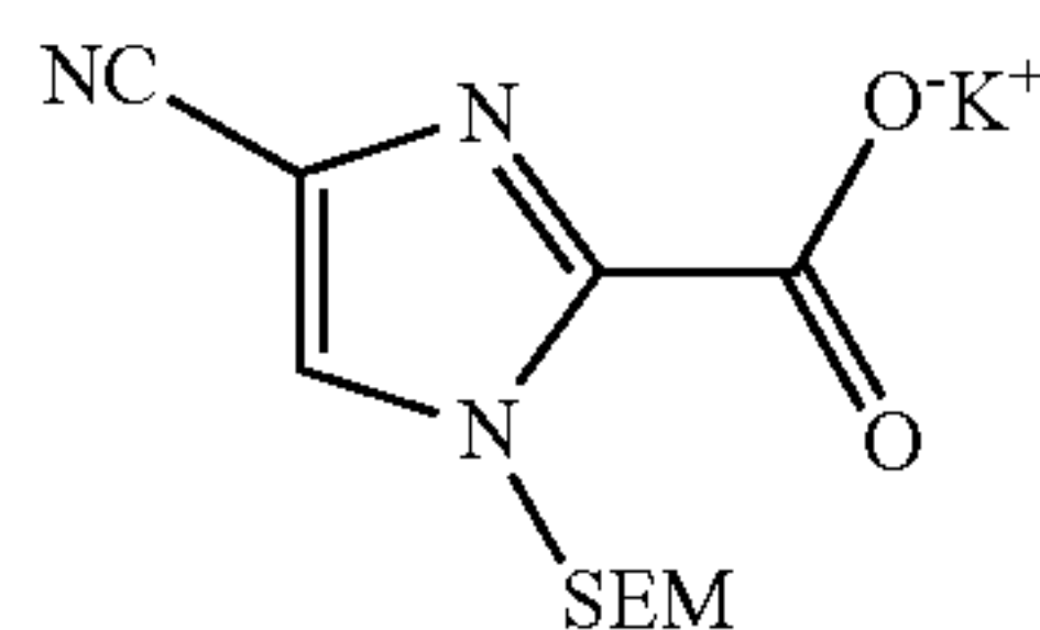
a) 1H-Imidazole-4-carbonitrile
