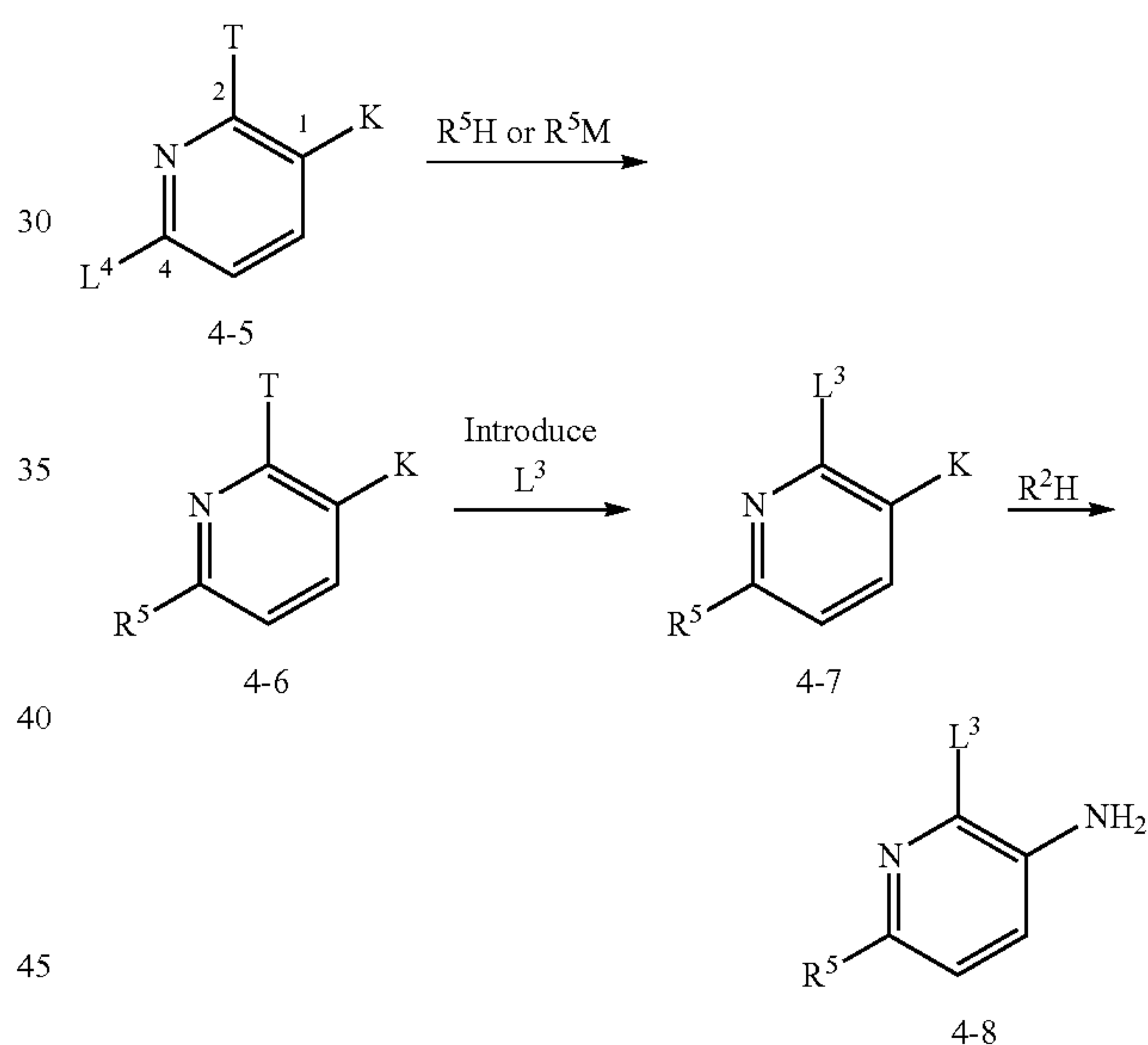
Scheme 4b
