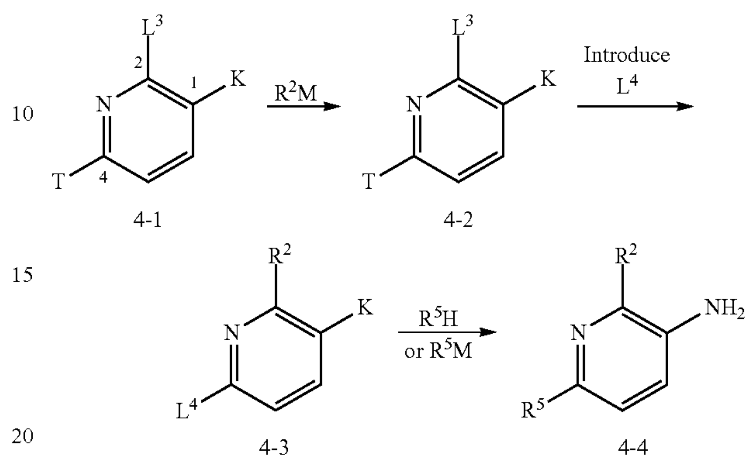
Scheme 4a
