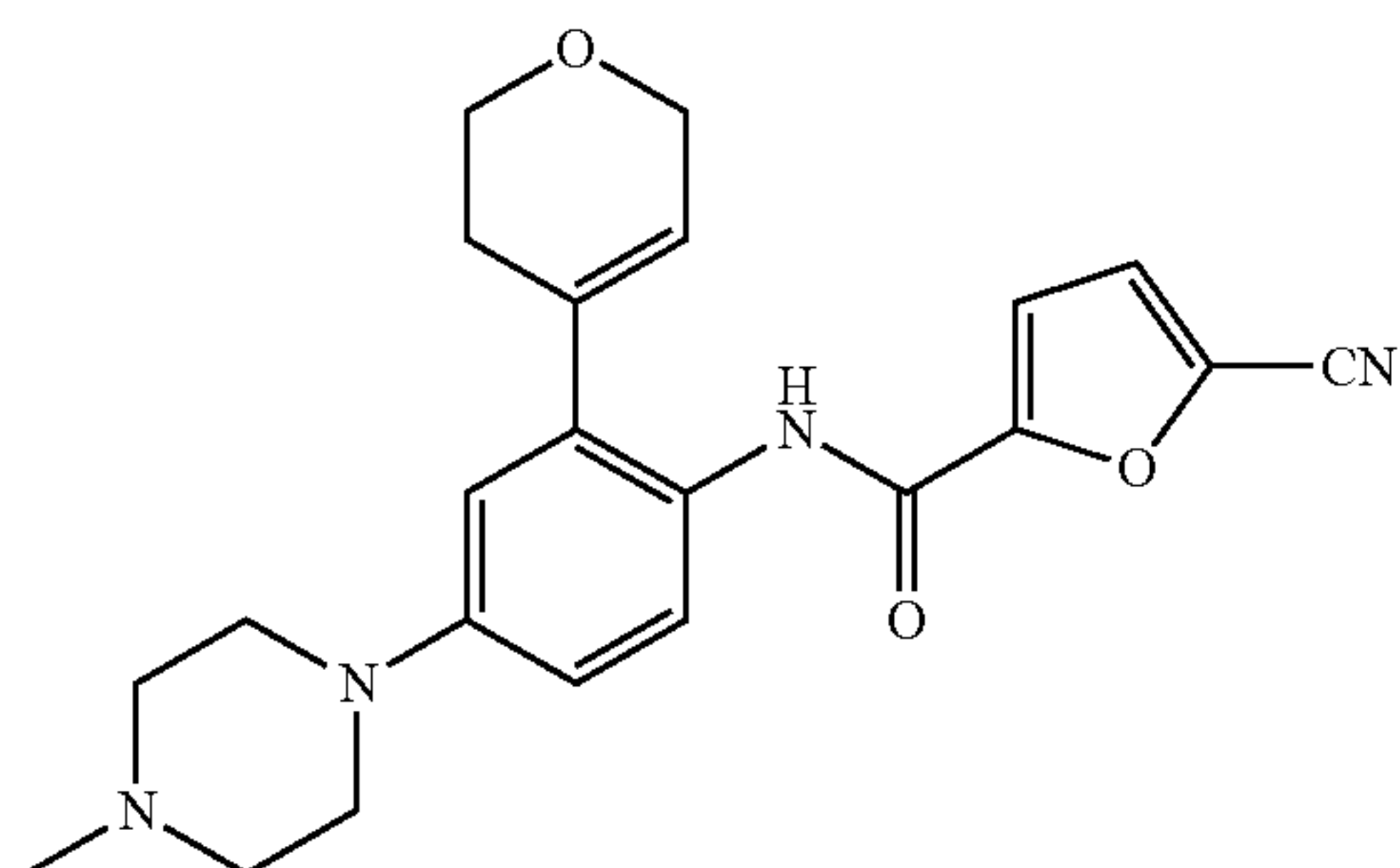
a) 1-[3-(3,6-Dihydro-2H-pyran-4-yl)-4-nitro-phenyl]-4-methyl-piperazine
