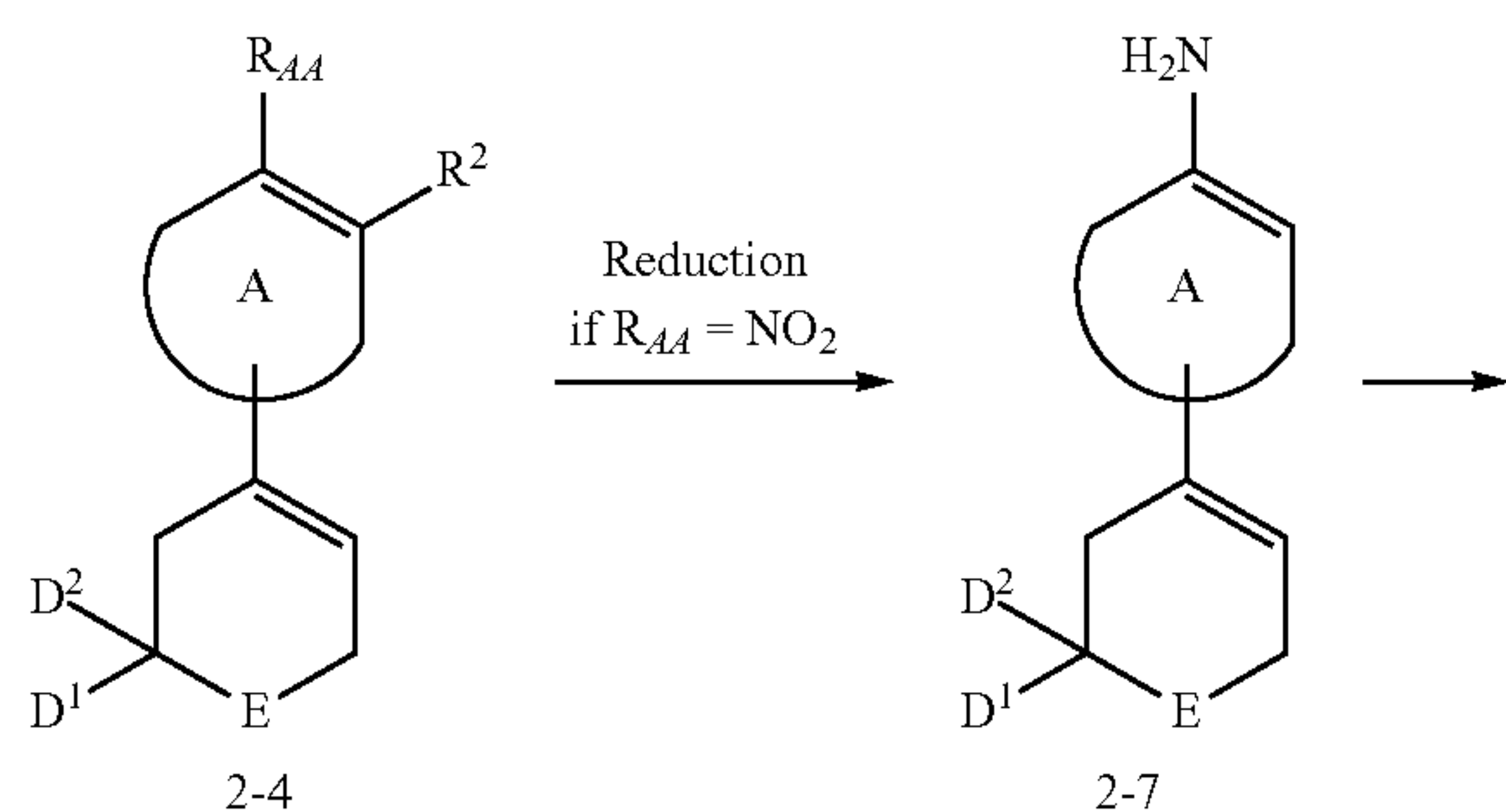
Scheme 2b
