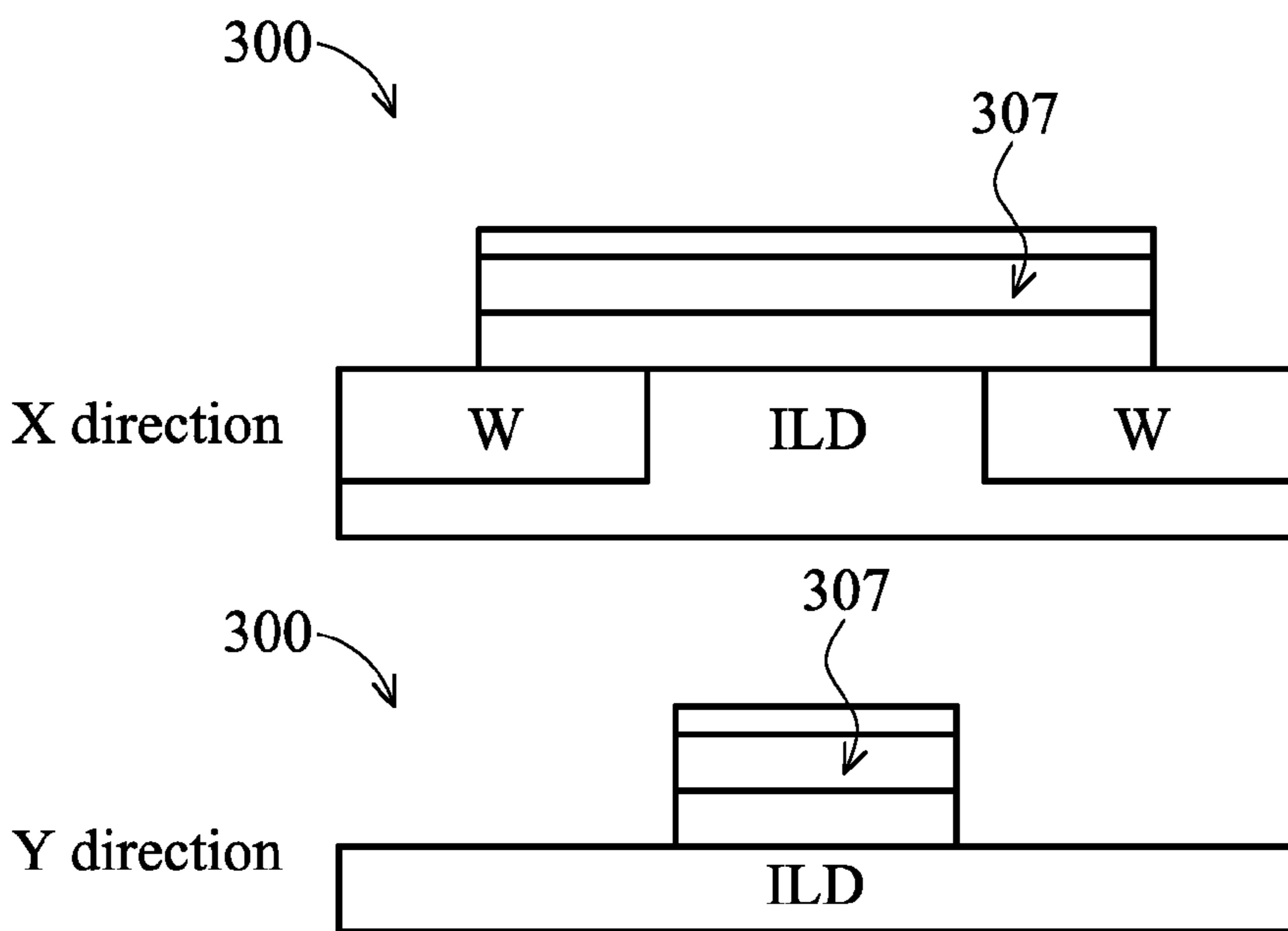
Fig. 3C (PRIOR ART)
