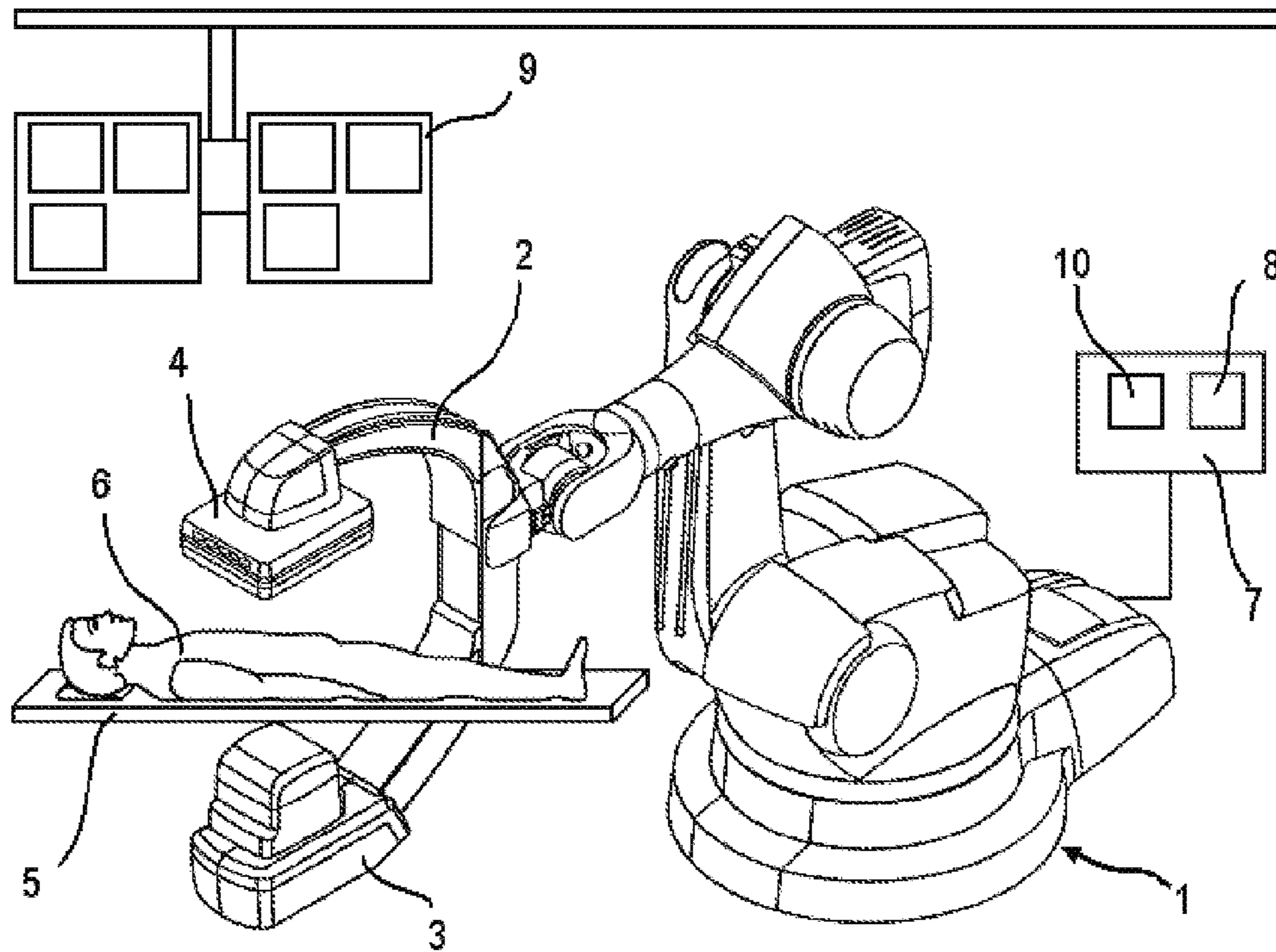
FIG 1 (Prior Art)
