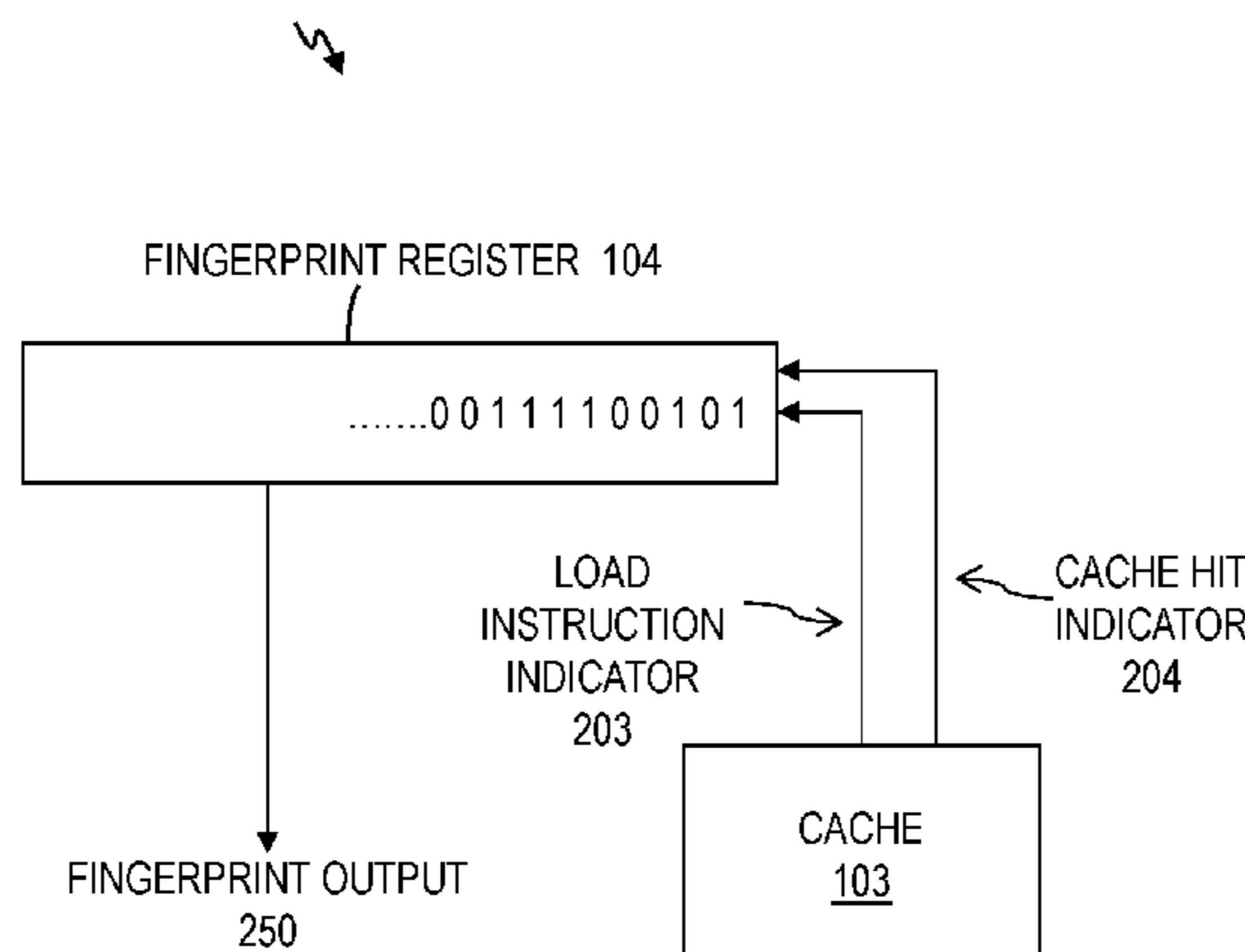
FINGERPRINT CIRCUIT 110
