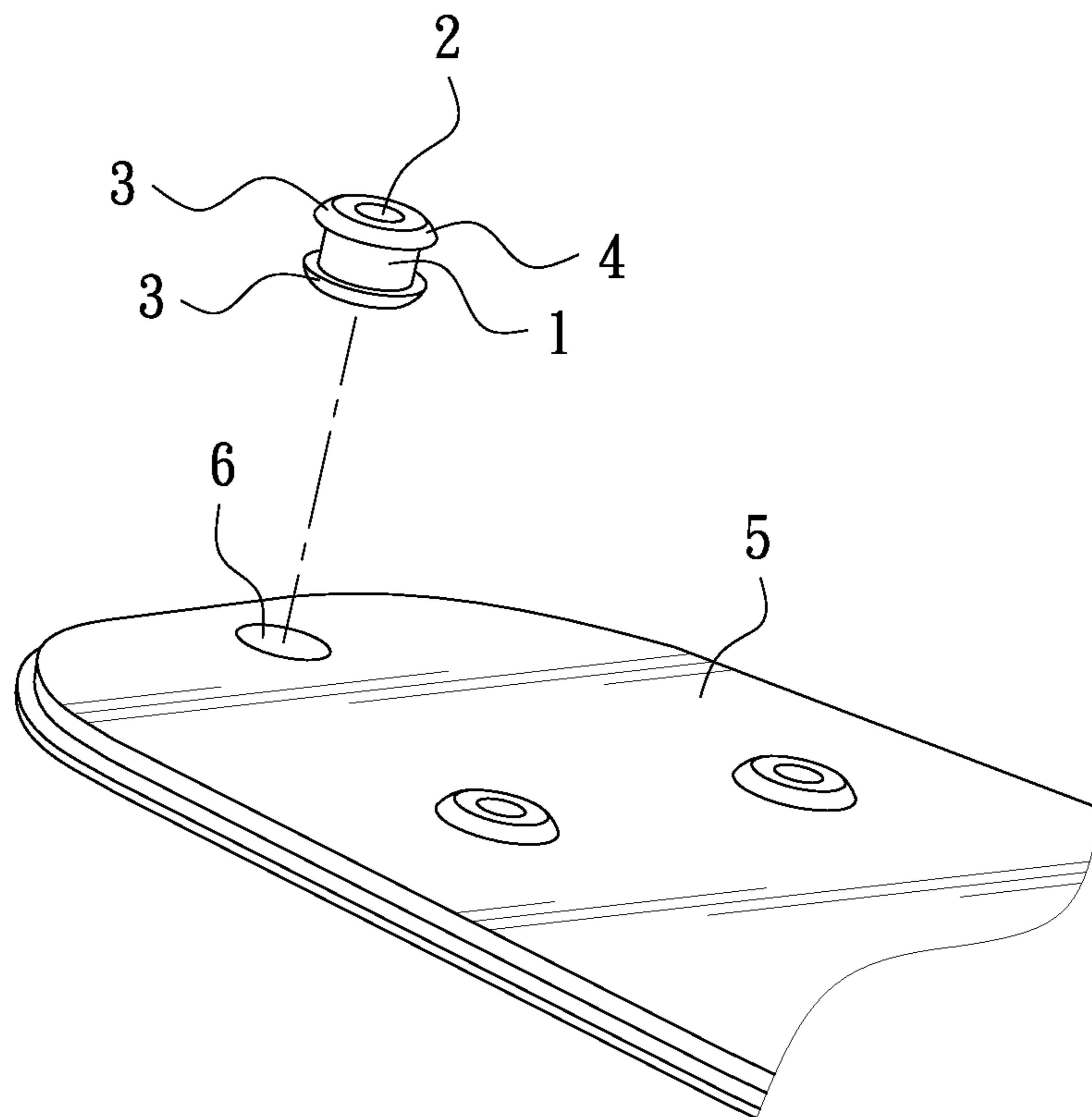
FIG. 1 PRIOR ART
