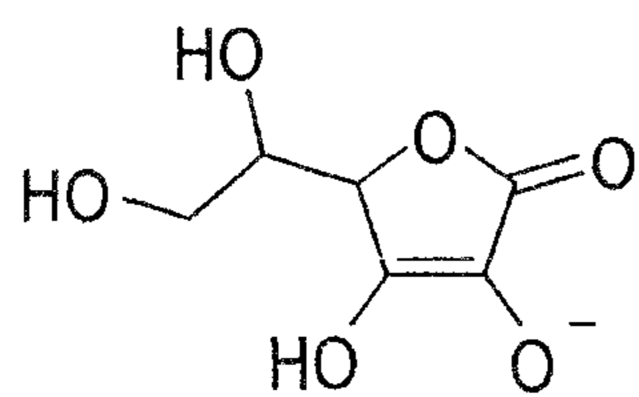
Ascorbate anion
