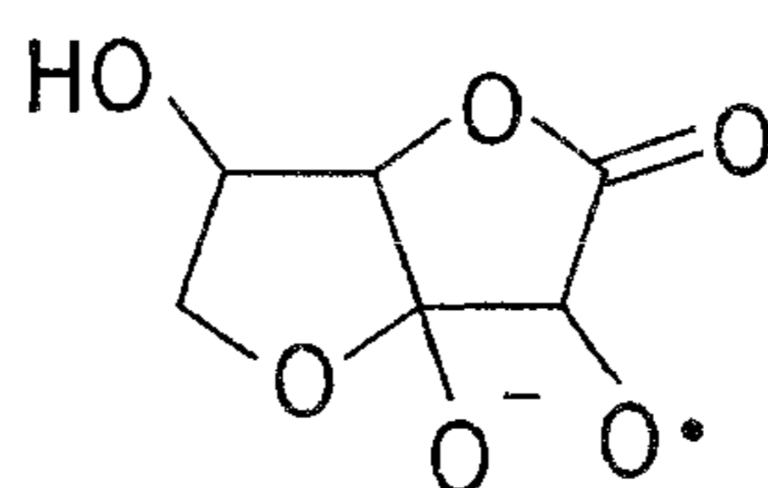
Ascorbate radical
