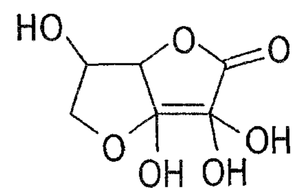
Dehydroascorbic acid
