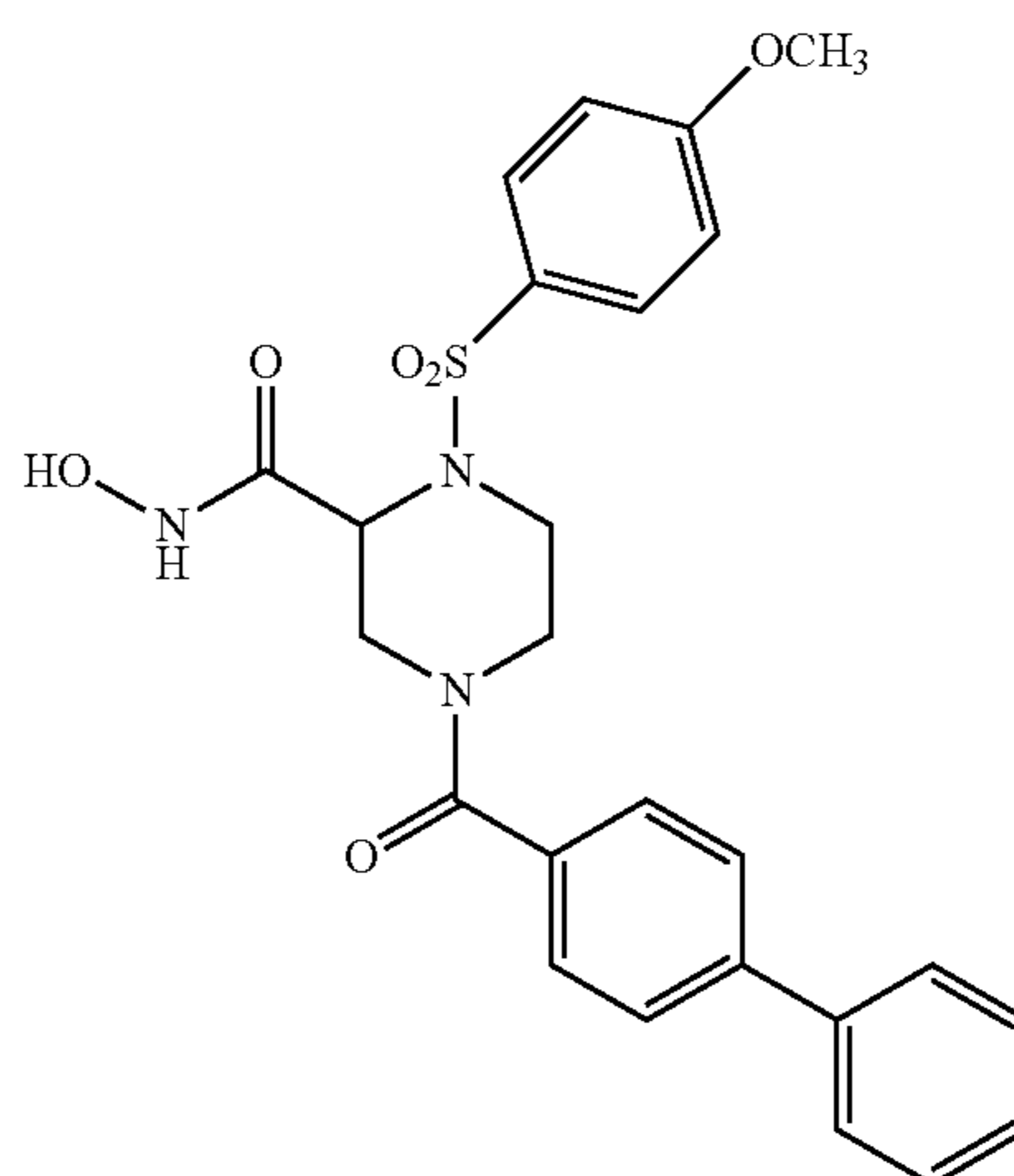
N-Hydroxy-1-(4-methoxyphenyl)sulfonyl-4-(40 biphenylcarbonyl)piperazine-2-carboxamide
