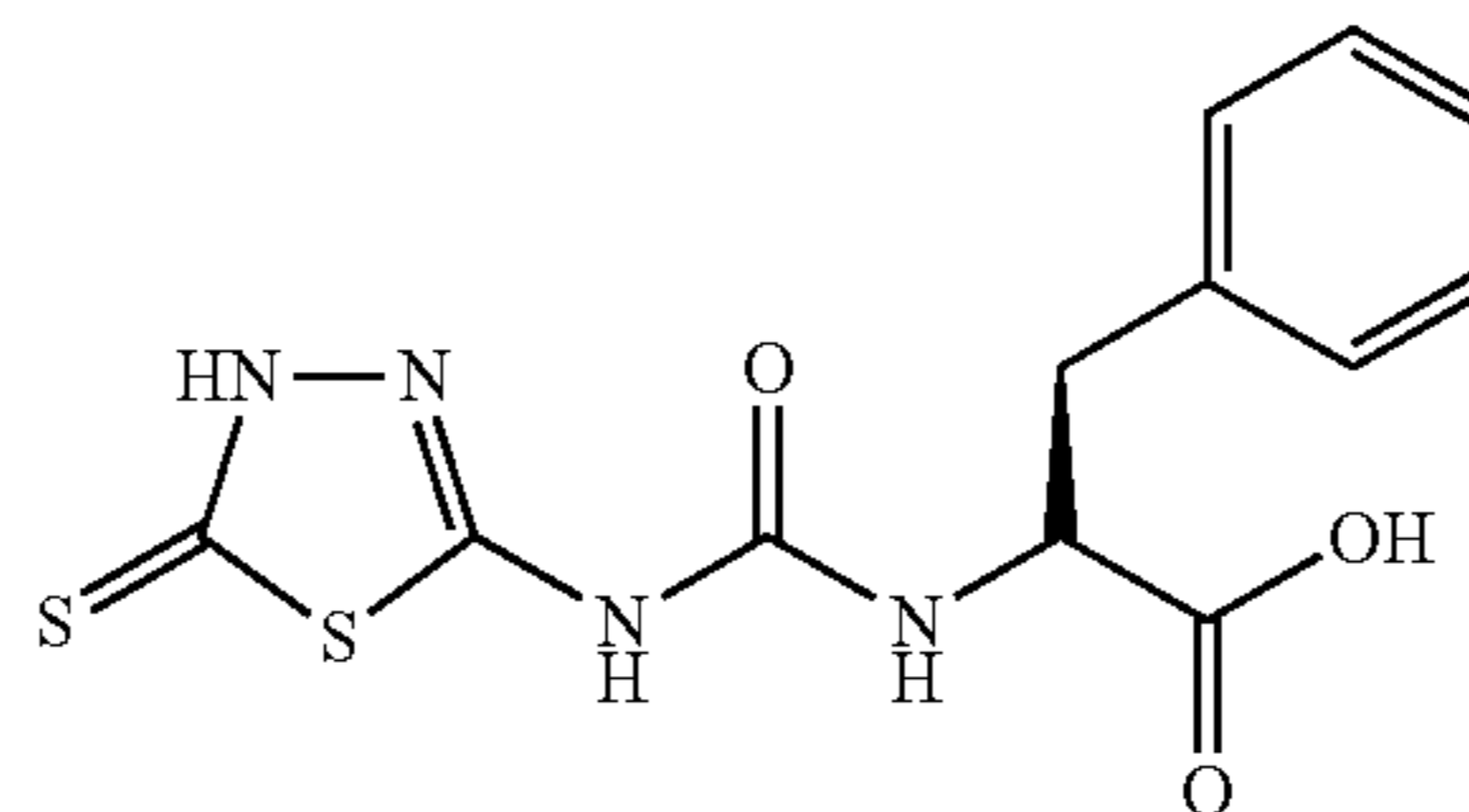
N-[[4,5-Dihydro-5-thioxo-1,3,4-thiadiazol-2-yl]amino]carbonyl]-L-phenylalanine
