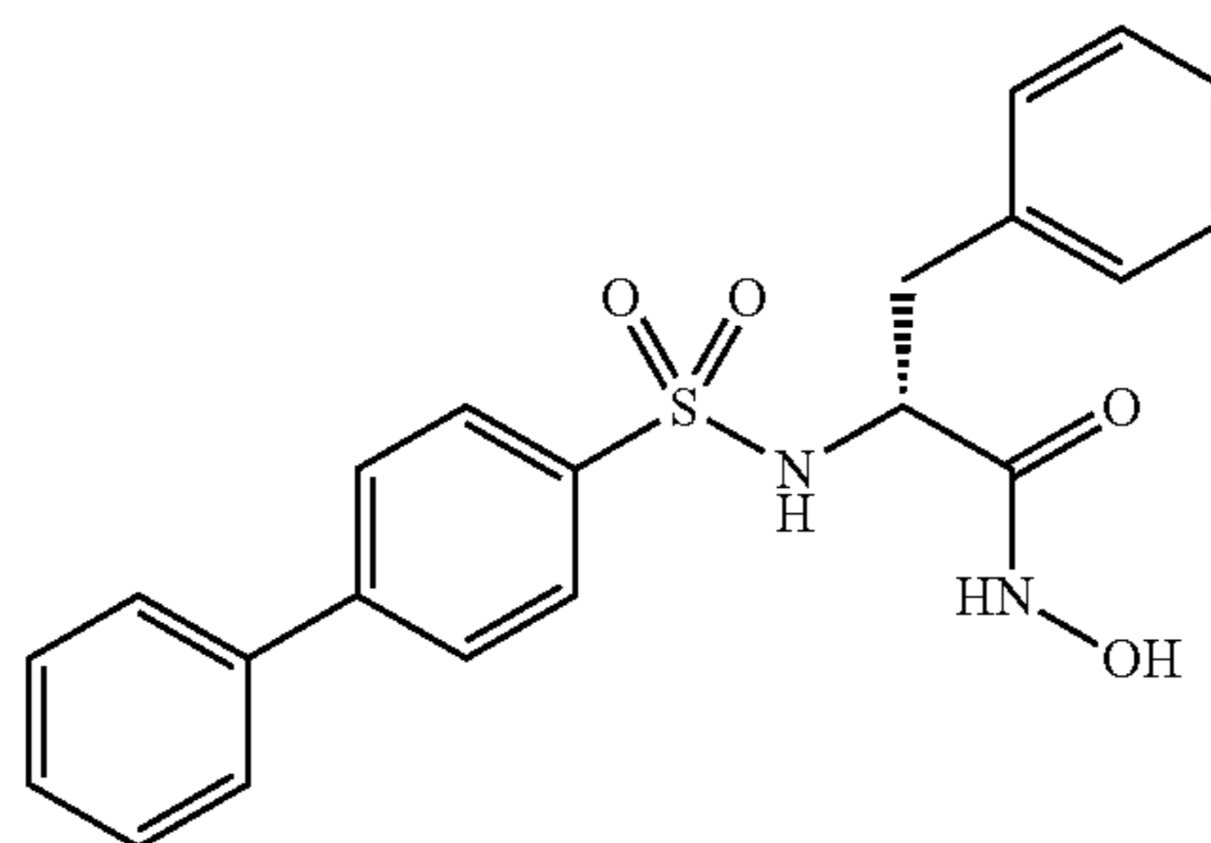
(2R)-[(4-Biphenylsulfonyl)amino]-N-hydroxy-3-phenylpropionamide
