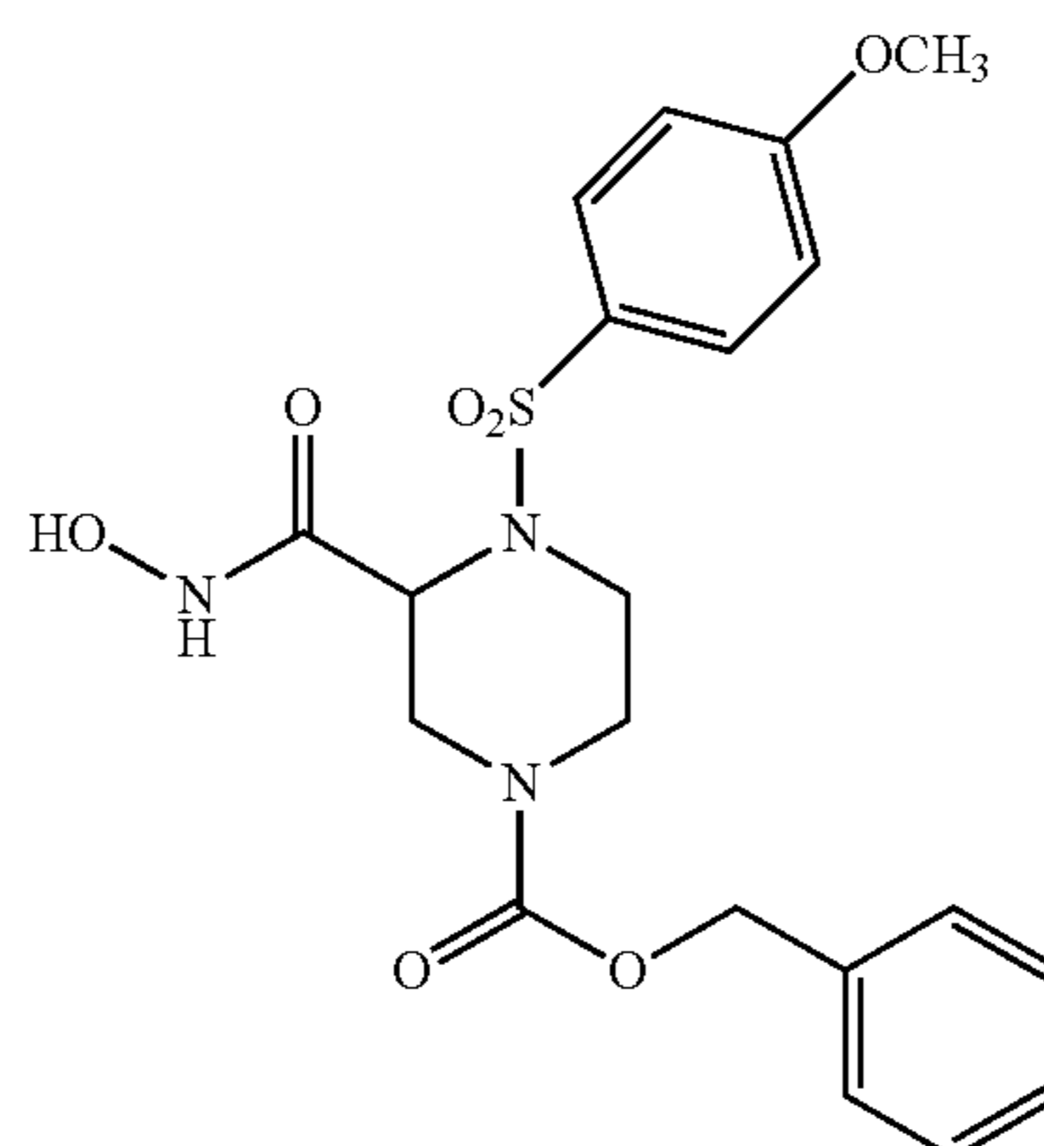
N-Hydroxy-1-(4-methoxyphenyl)sulfonyl-4-benzyloxycarbonylpiperazine-2-carboxamide
