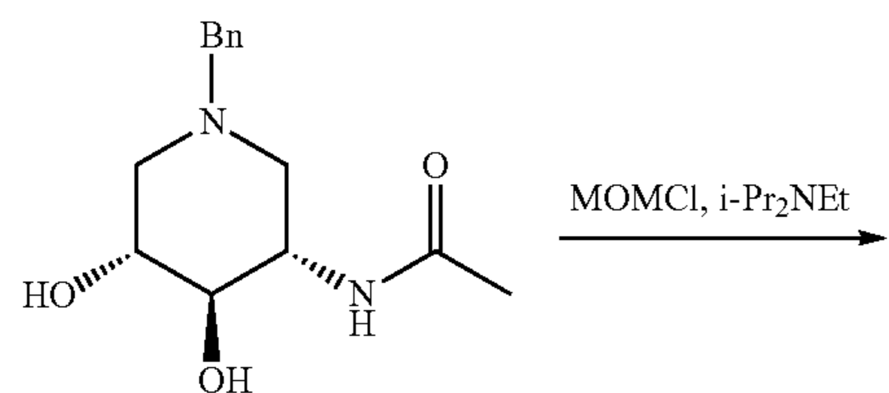
Scheme 8
