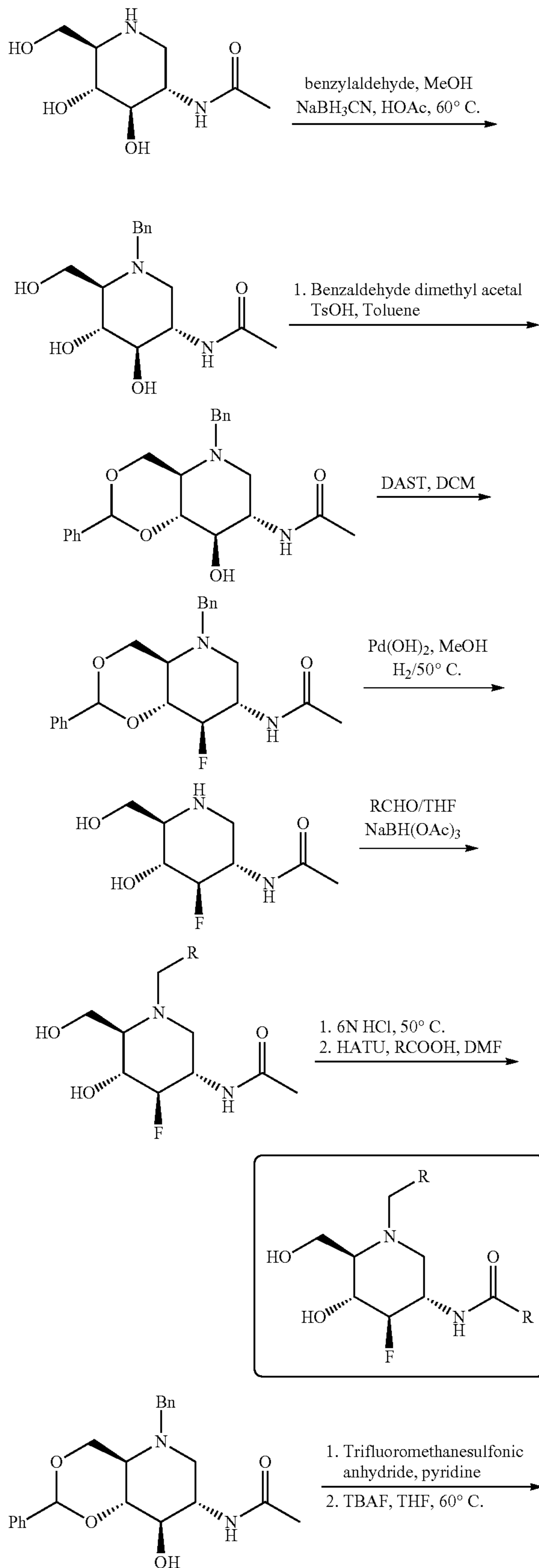
Scheme 2
