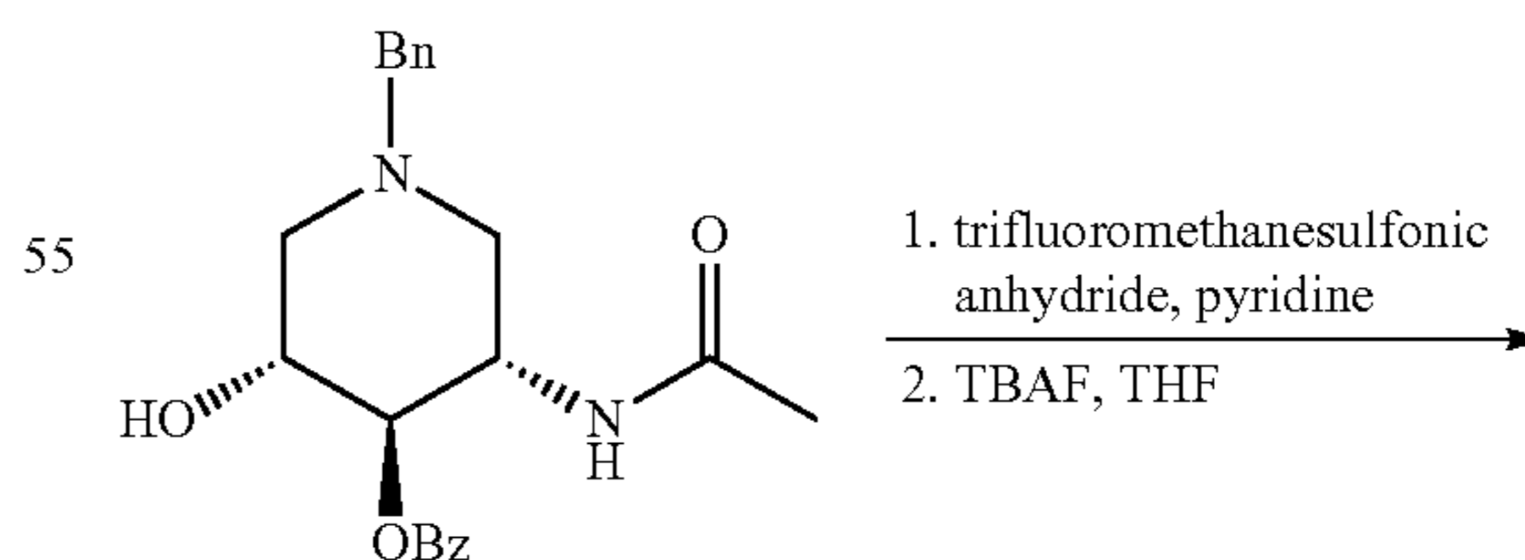
Scheme 9
