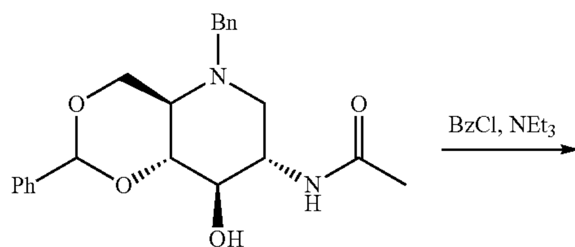
Scheme 3
