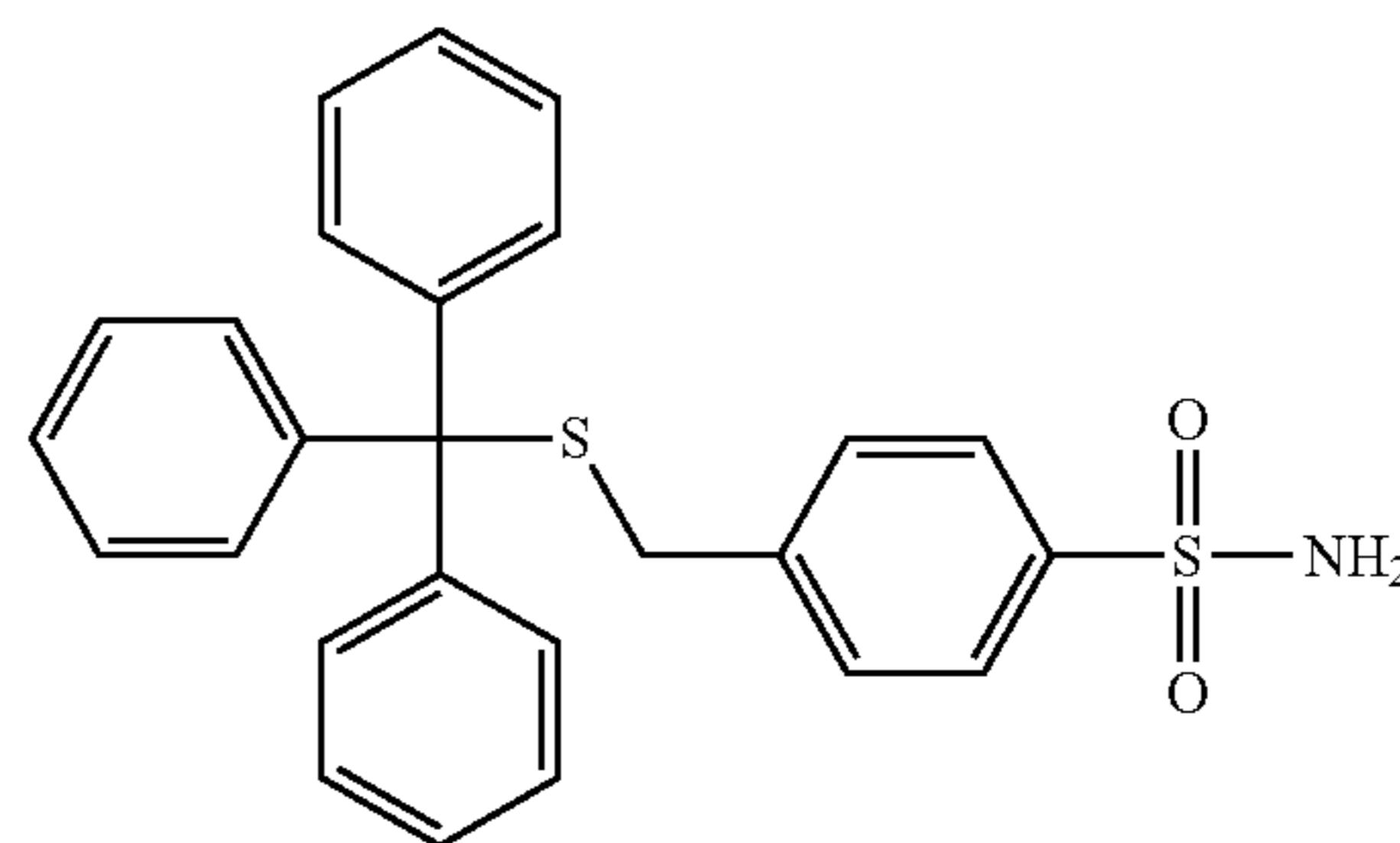
4-(tritylthiomethyl)benzenesulfonamide
