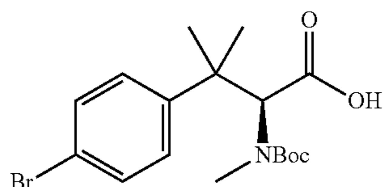
(S)-3-(4-bromophenyl)-2-(tert-butoxycarbonyl(methyl)amino)-3-methylbutanoic acid
