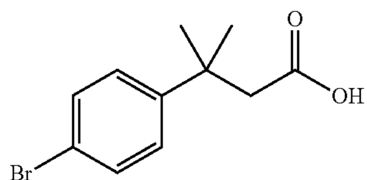
3-methyl-3-(4-bromophenyl)butanoic acid
