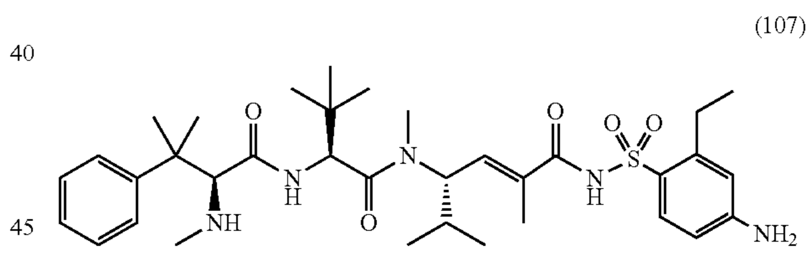
(S,E)-N-(4-amino-2-ethylphenylsulfonyl)-2,5-dimethyl-4-((S)-N,3,3-trimethyl-2-((S)-3-methyl-2-(methylamino)-3-phenylbutanamido)butanamido)hex-2-enamide
