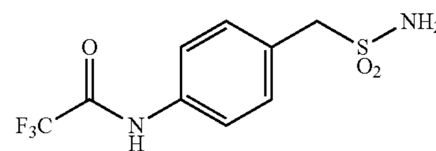
2,2,2-trifluoro-N-(4-(sulfamoylmethyl)phenyl)acetamide
