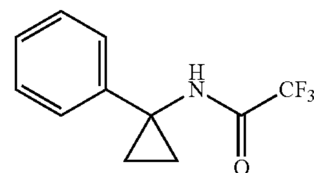
2,2,2-trifluoro-N-(1-phenylcyclopropyl)acetamide
