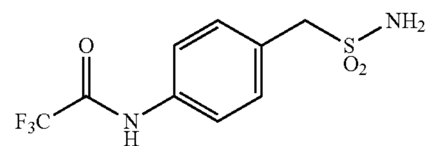
2,2,2-trifluoro-N-(4-(sulfamoylmethyl)phenyl)acetamide
