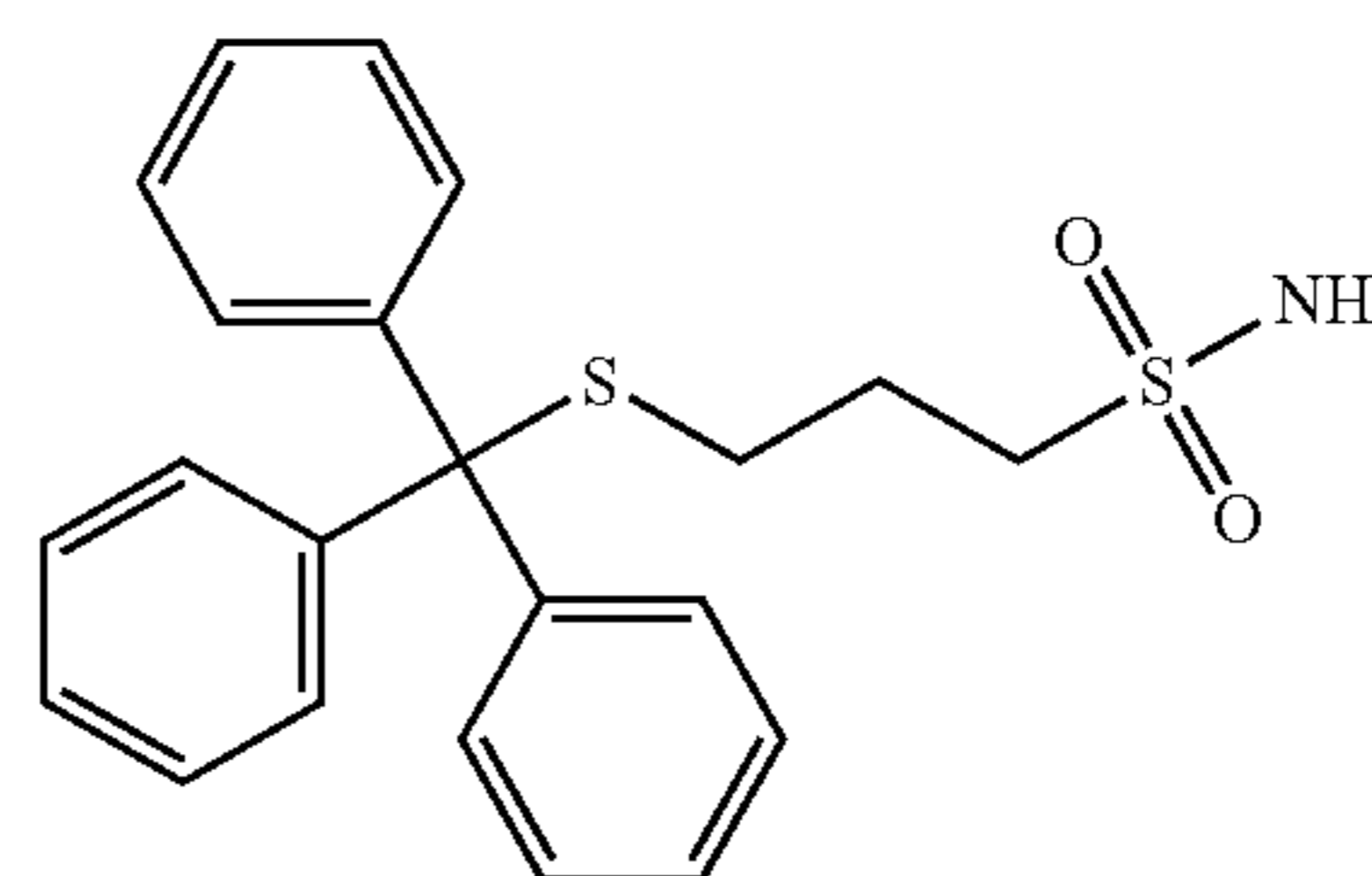
3-(tritylthio)propane-1-sulfonamide
