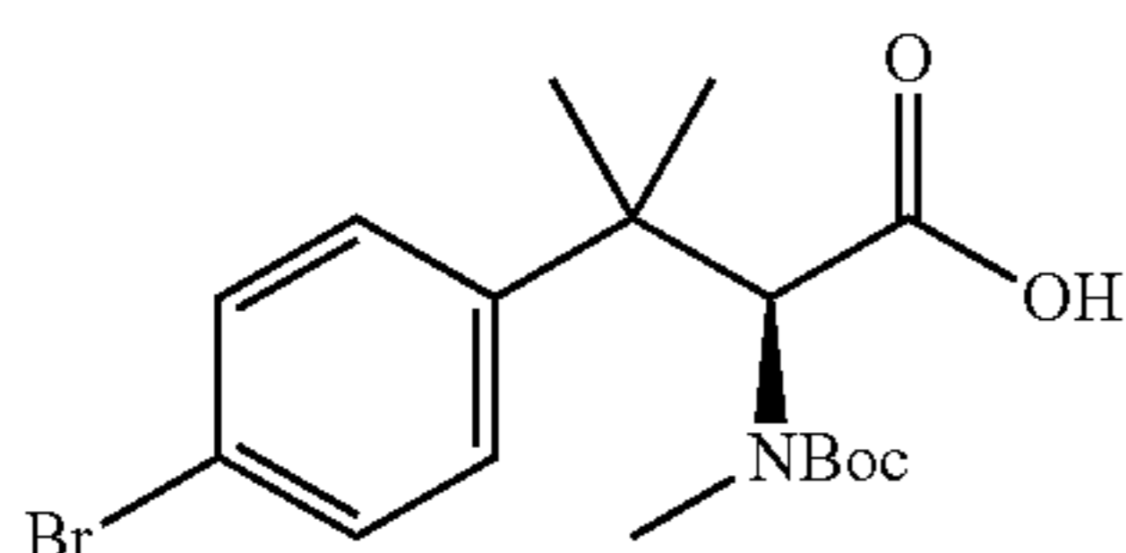
(S)-3-(4-bromophenyl)-2-(tert-butoxycarbonyl(methyl)amino)-3-methylbutanoic acid
