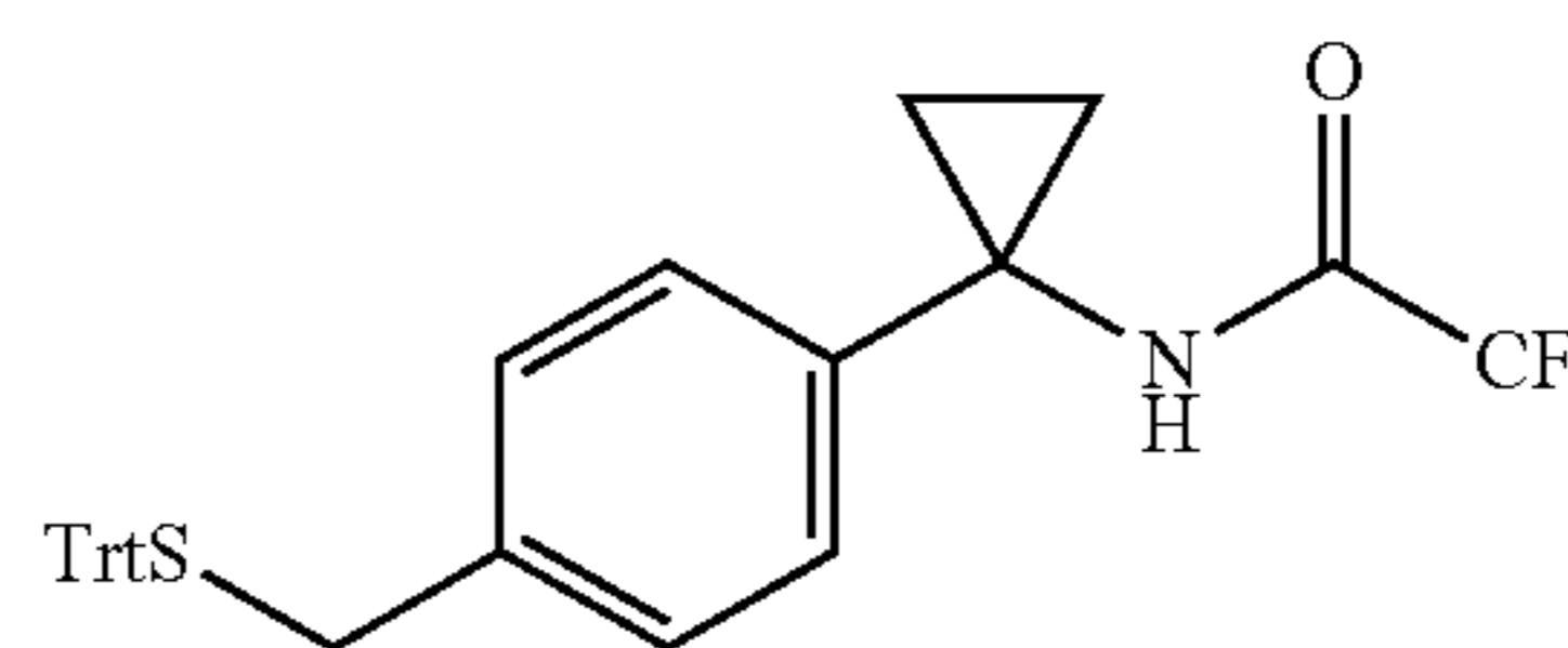
2,2,2-trifluoro-N-(1-(4-(tritylthiomethyl)phenyl)cyclopropyl)acetamide
