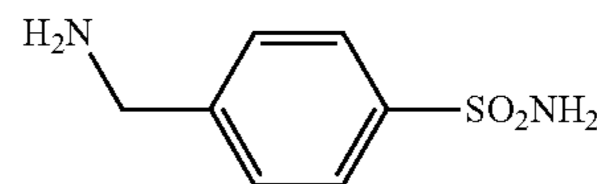
4-(aminomethyl)benzenesulfonamide
