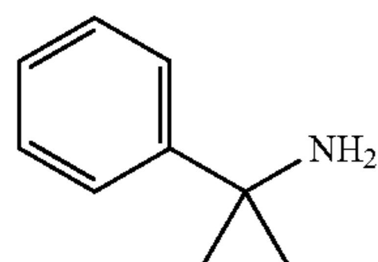
1-phenylcyclopropanamine
