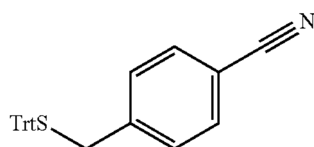
4-(tritylthiomethyl)benzonitrile
