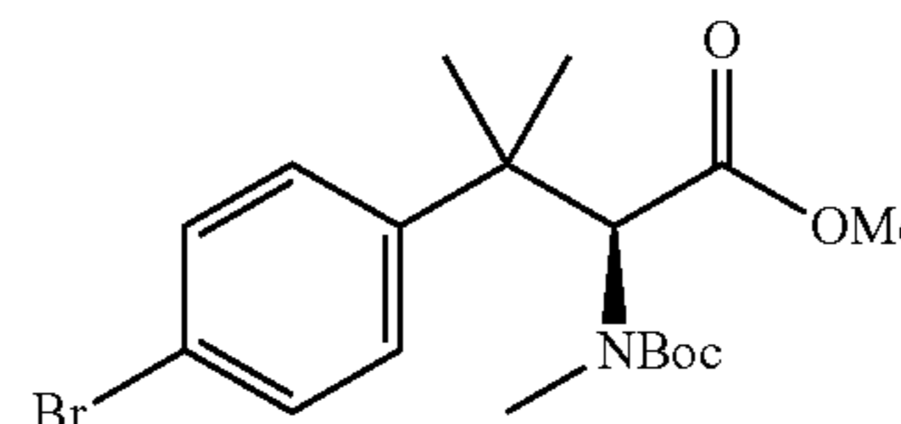
(S)-methyl 3-(4-bromophenyl)-2-(tert-butoxycarbonyl(methyl)amino)-3-methylbutanoate
