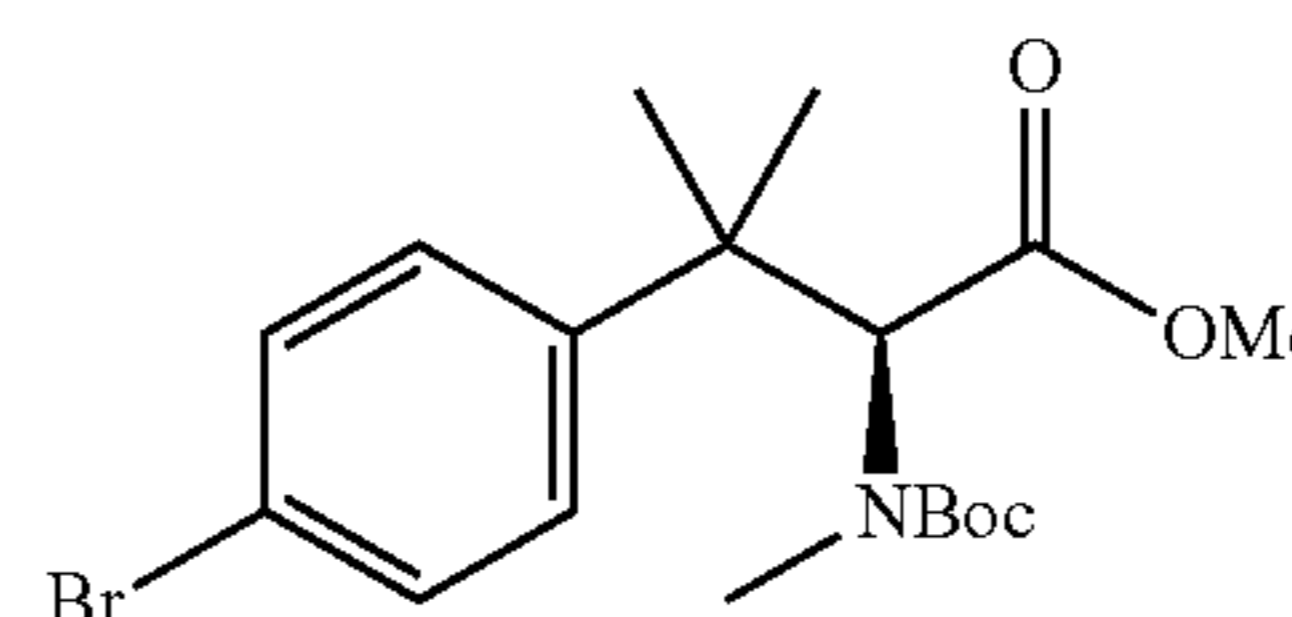
(S)-methyl 3-(4-bromophenyl)-2-(tert-butoxycarbonyl(methyl)amino)-3-methylbutanoate
