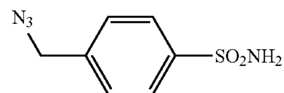
4-(azidomethyl)benzenesulfonamide
