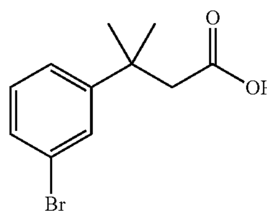
3-methyl-3-(3-bromophenyl)butanoic acid
