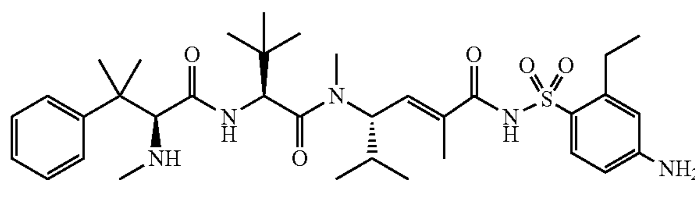
(S,E)-N-(4-amino-2-ethylphenylsulfonyl)-2,5-dimethyl-4-((S)-N,3,3-trimethyl-2-((S)-3-methyl-2-(methylamino)-3-phenylbutanamido)butanamido)hex-2-enamide
