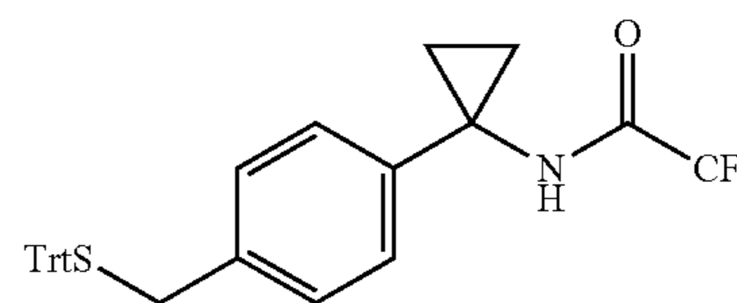
2,2,2-trifluoro-N-(1-(4-(tritylthiomethyl)phenyl)cyclopropyl)acetamide
