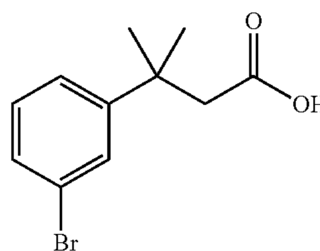
3-methyl-3-(3-bromophenyl)butanoic acid
