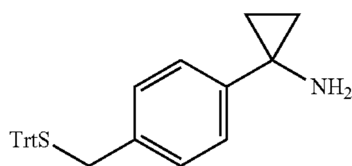
1-(4-(tritylthiomethyl)phenyl)cyclopropanamine
