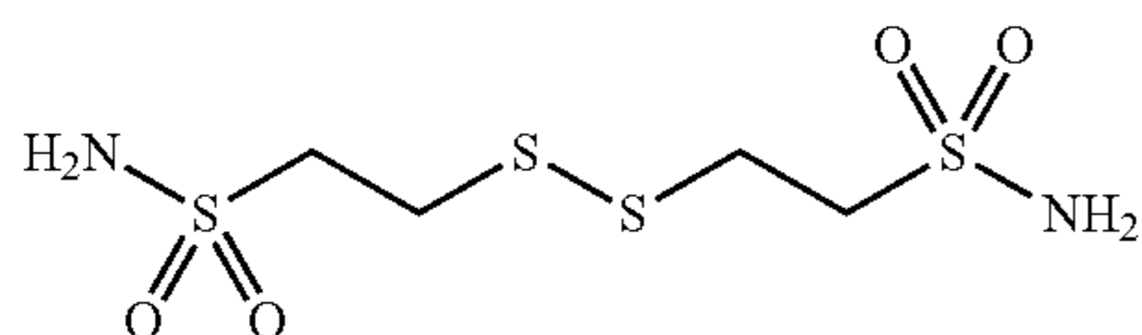
2,2'-disulfanediyldiethanesulfonamide
