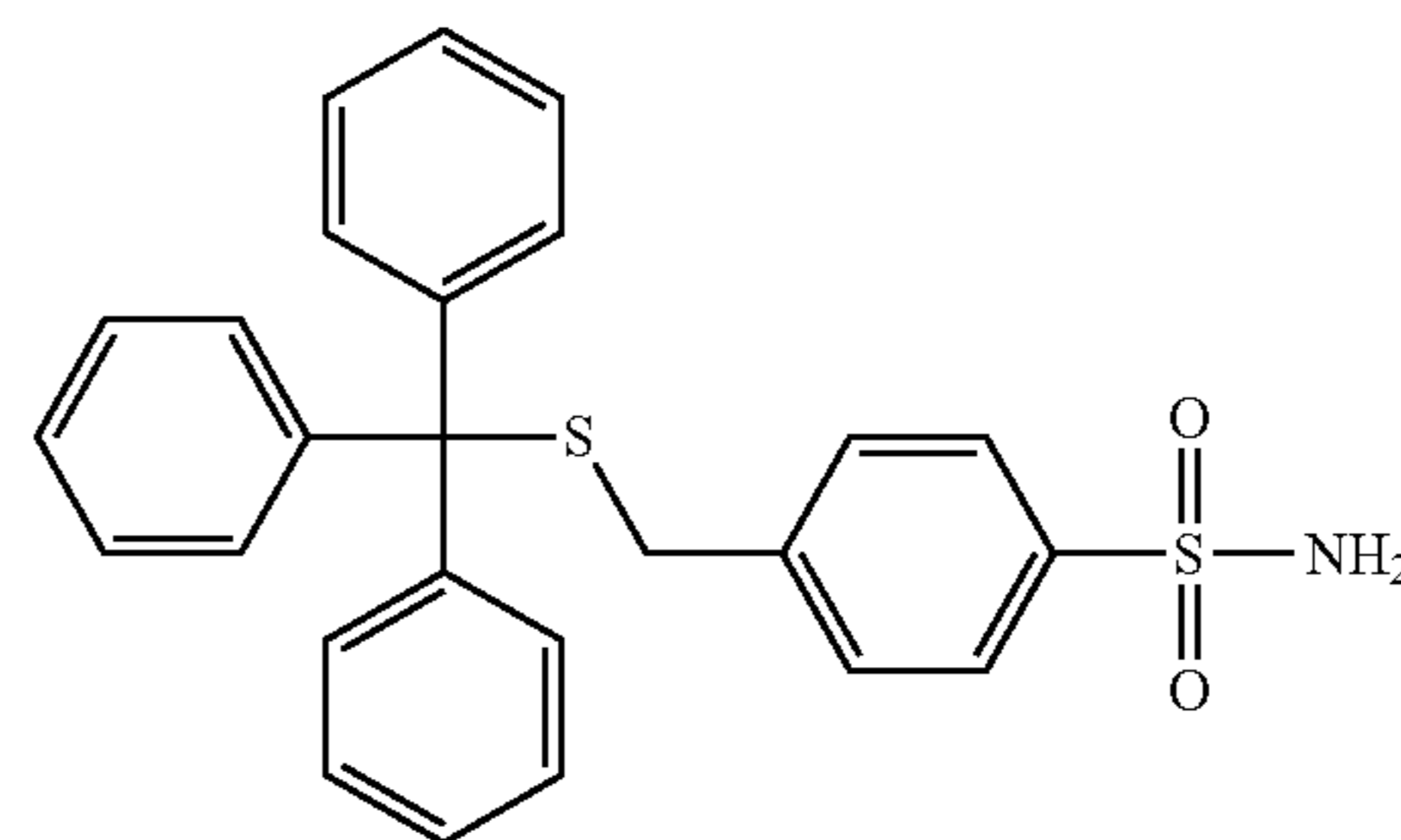
4-(tritylthiomethyl)benzenesulfonamide
