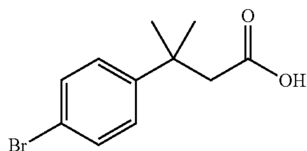
3-methyl-3-(4-bromophenyl)butanoic acid
