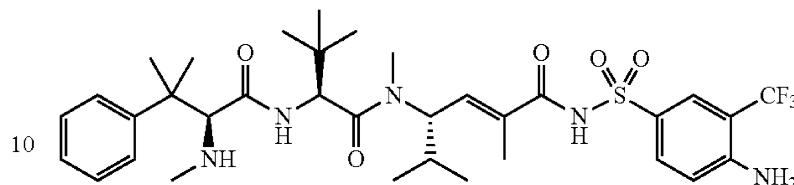
(S,E)-N-(4-amino-3-(trifluoromethyl)phenylsulfonyl)-2,5-dimethyl-4-((S)-N,3,3-trimethyl-2-((S)-3-methyl-2-(methylamino)-3-phenylbutanamido)butanamido)hex-2-enamide
