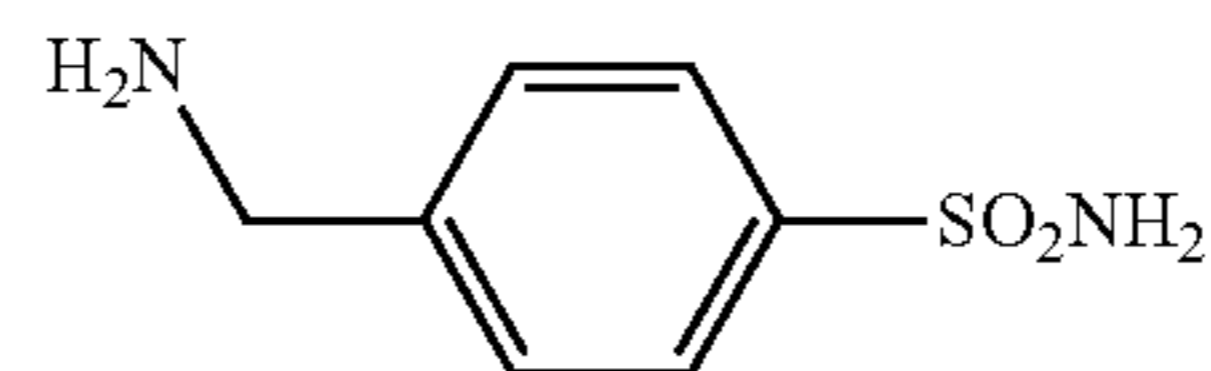
4-(aminomethyl)benzenesulfonamide
