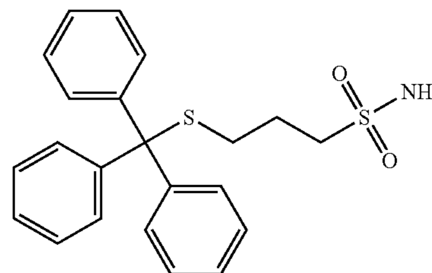
3-(tritylthio)propane-1-sulfonamide
