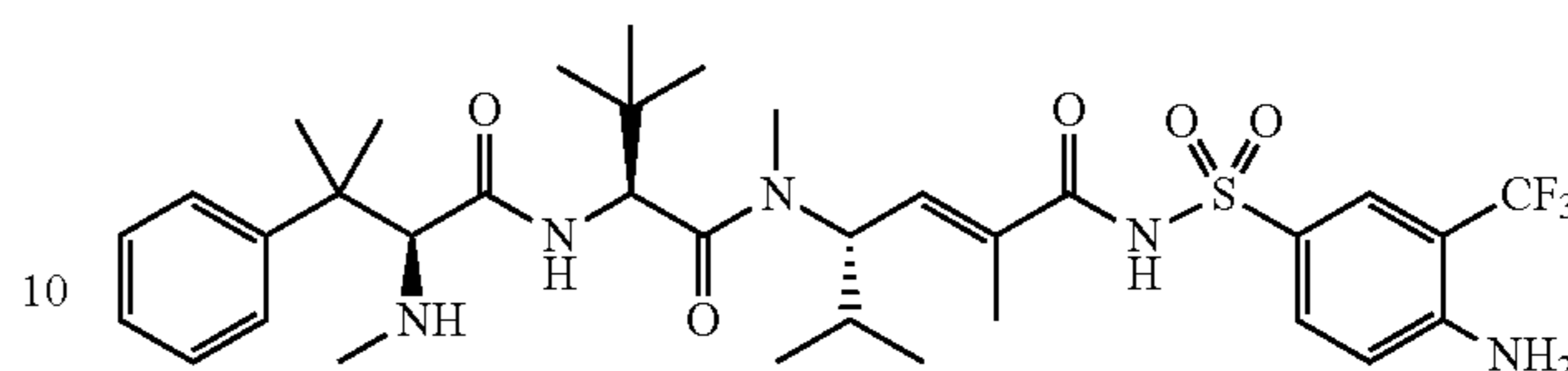
(S,E)-N-(4-amino-3-(trifluoromethyl)phenylsulfonyl)-2,5-dimethyl-4-((S)-N,3,3-trimethyl-2-((S)-3-methyl-2-(methylamino)-3-phenylbutanamido)butanamido)hex-2-enamide
