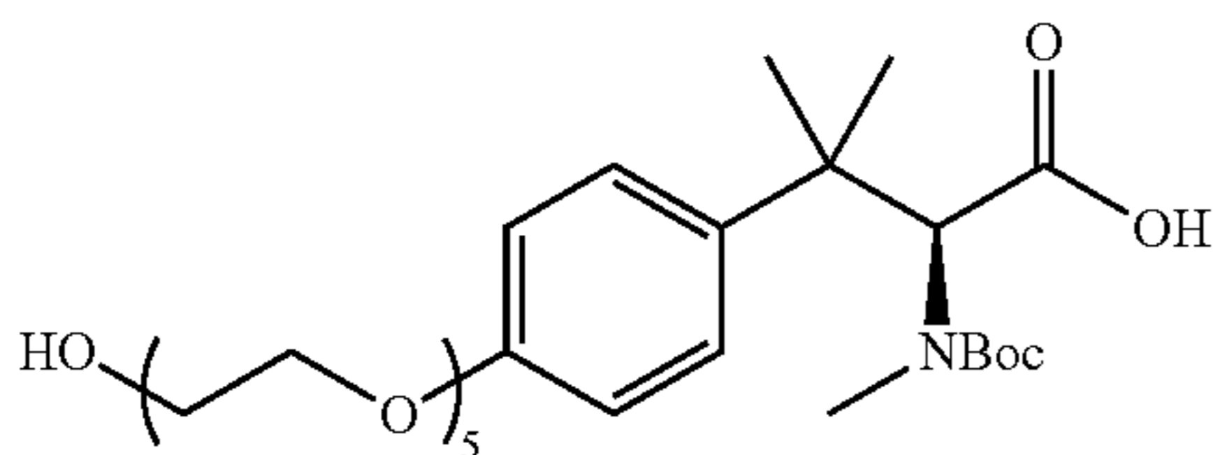
(S)-2-(((tert-butoxycarbonyl)(methyl)amino)-3-(4-((14-hydroxy-3,6,9,12-tetraoxatetradecyl)oxy)phenyl)-3-methylbutanoic acid
