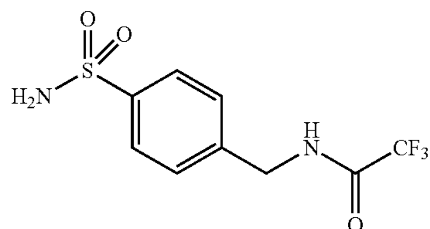
2,2,2-trifluoro-N-(4-sulfamoylbenzyl)acetamide
