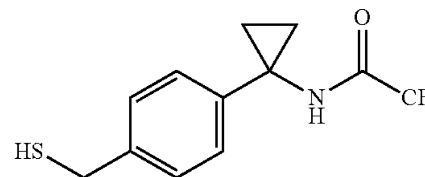
2,2,2-trifluoro-N-(1-(4-(mercaptomethyl)phenyl)cyclopropyl)acetamide
