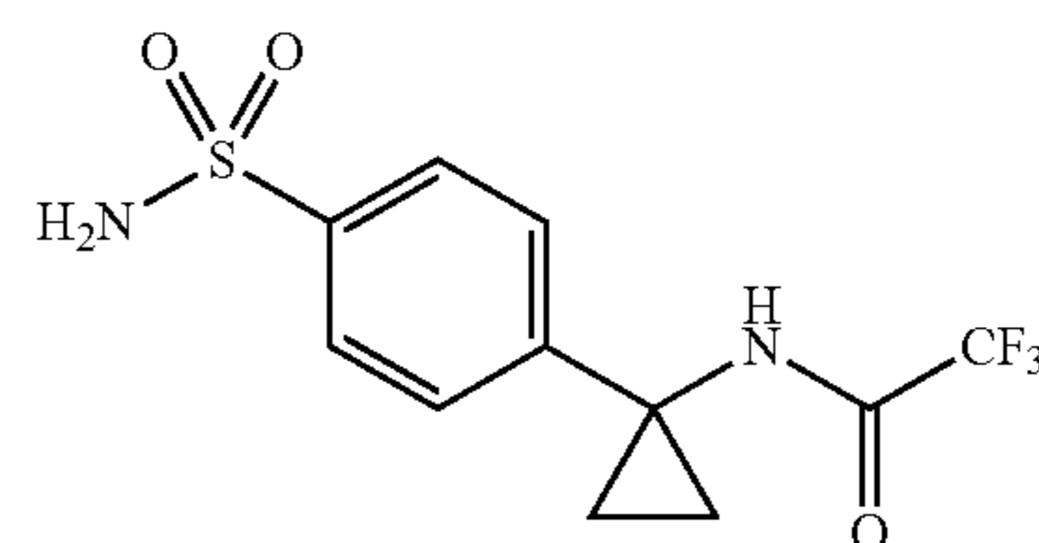
2,2,2-trifluoro-N-(1-(4-sulfamoylphenyl)cyclopropyl)acetamide
