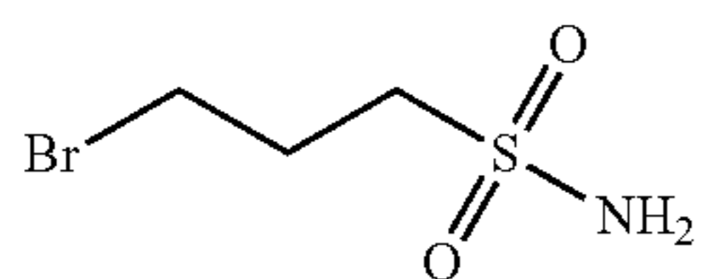
3-bromopropane-1-sulfonamide
