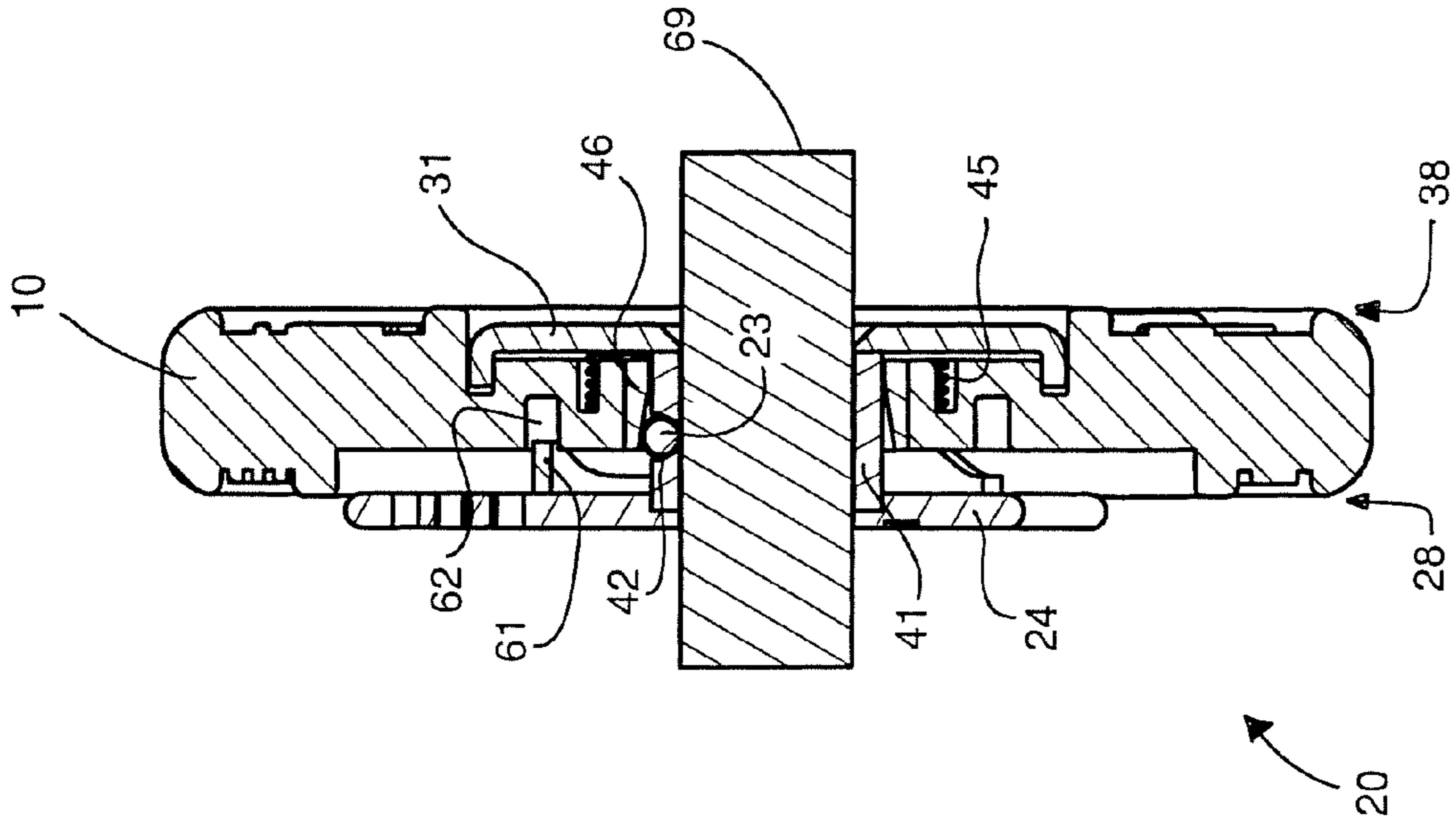
SECTION B-B
