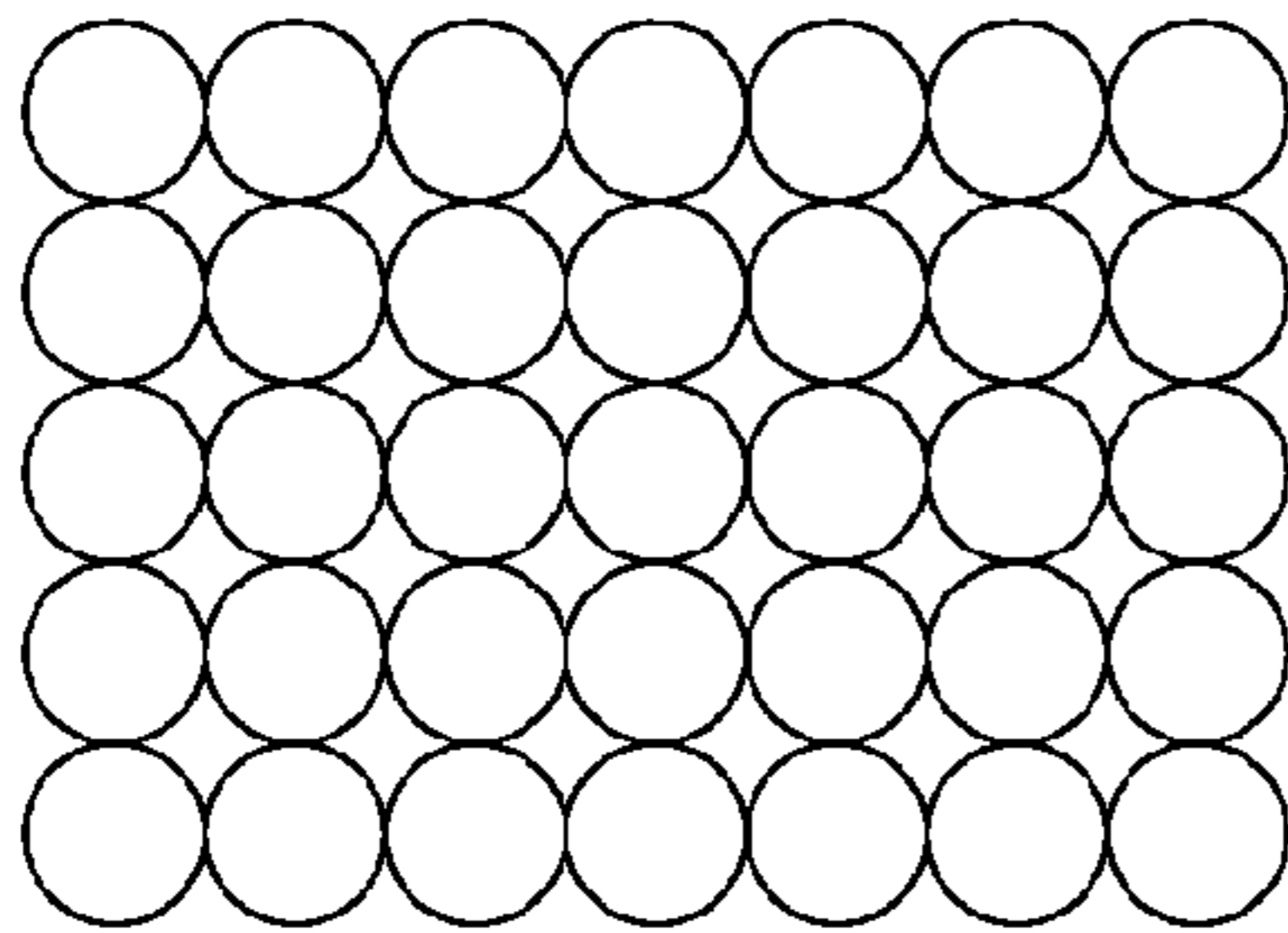
square packing
