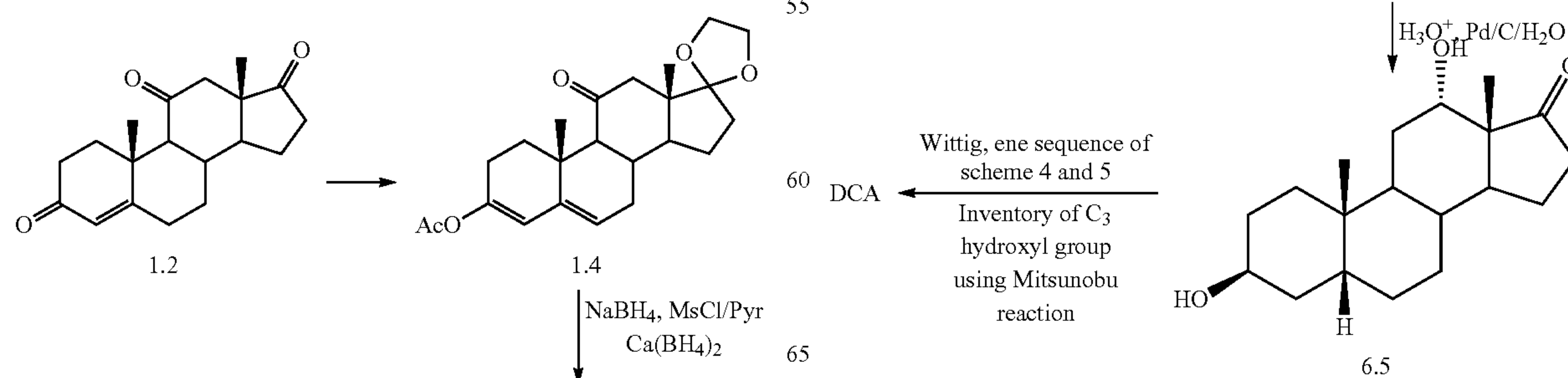
Scheme 6. Protection of A-B-ring system by formation of the i-steroid (i.e., 3,5-cyclosterol)
