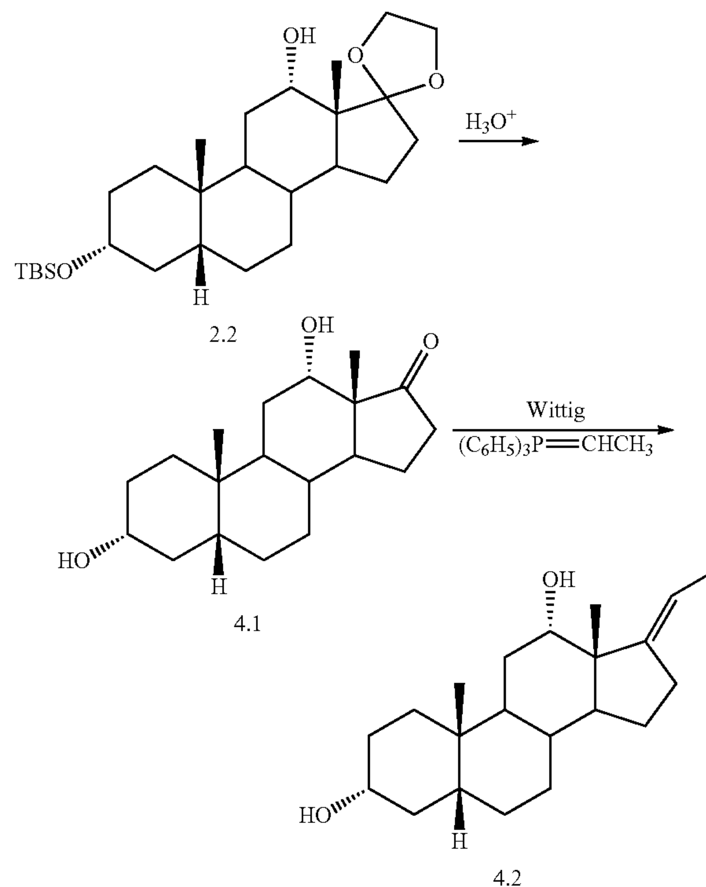
Scheme 4. Deprotection and Wittig Reaction
