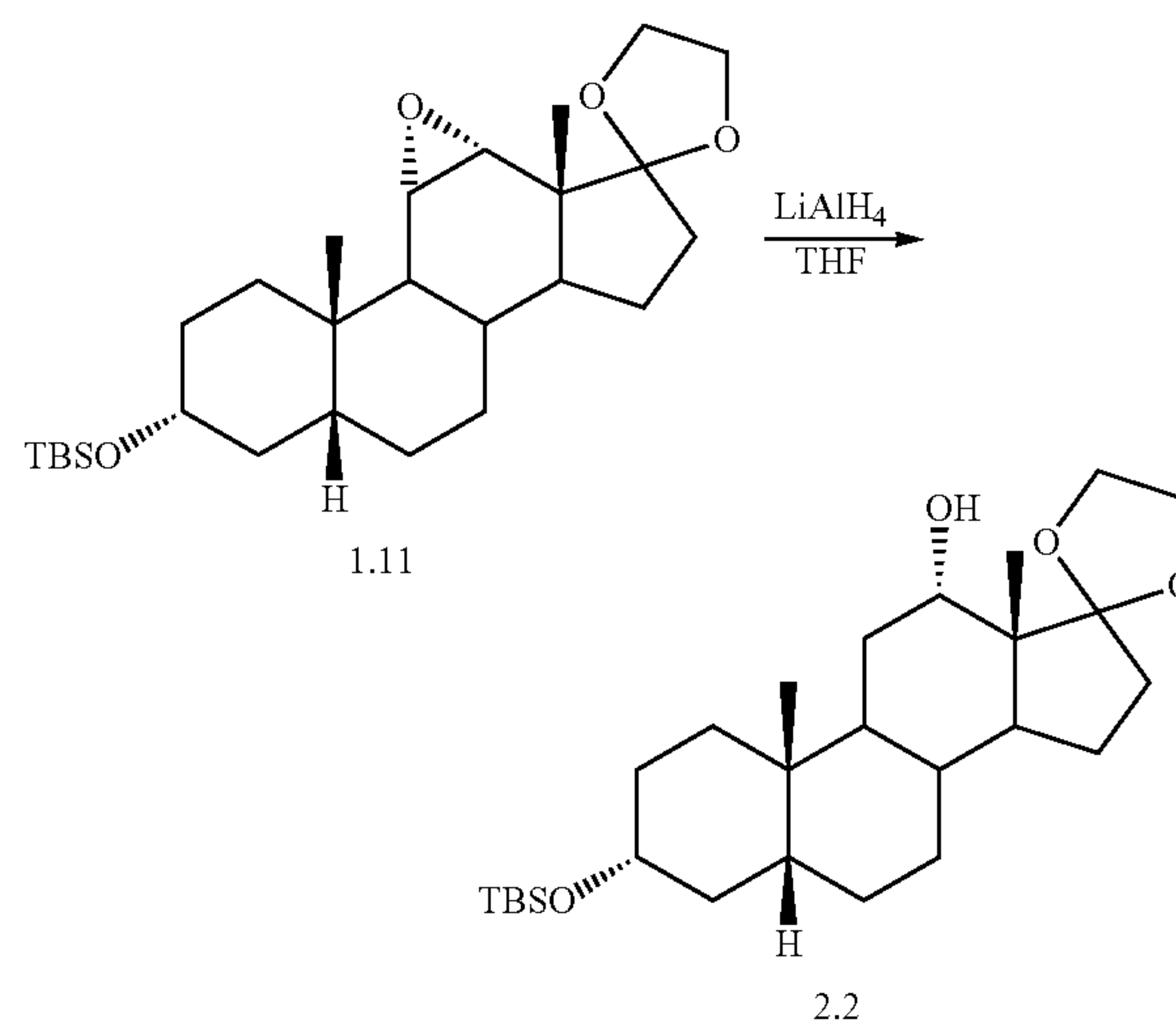
Scheme 3. Stereoselective Reduction of C 11 -C 12 epoxide.
