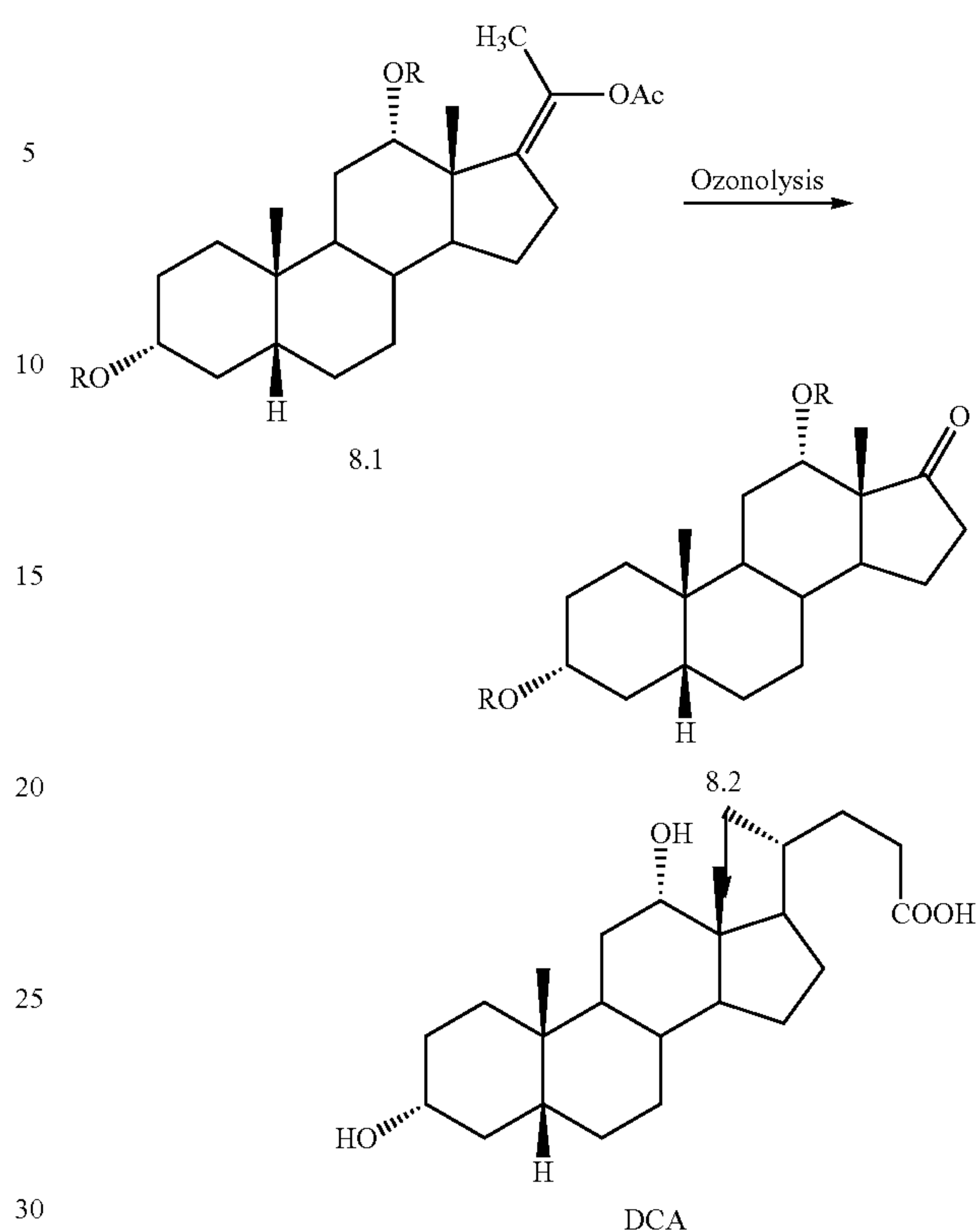
Scheme 8. Side-chain introduction
