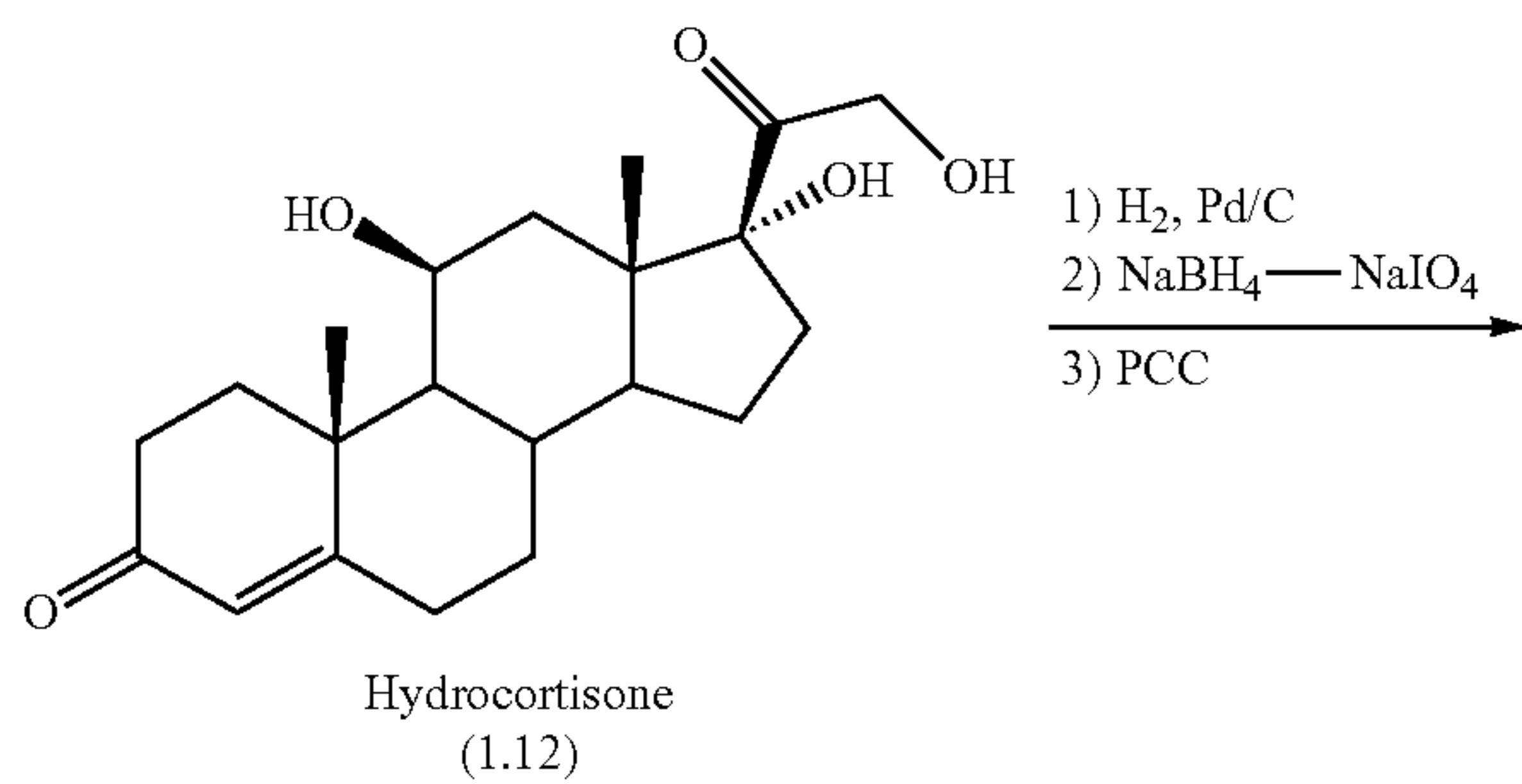
Scheme 1B. Synthesis of DCA from Hydrocortisone
