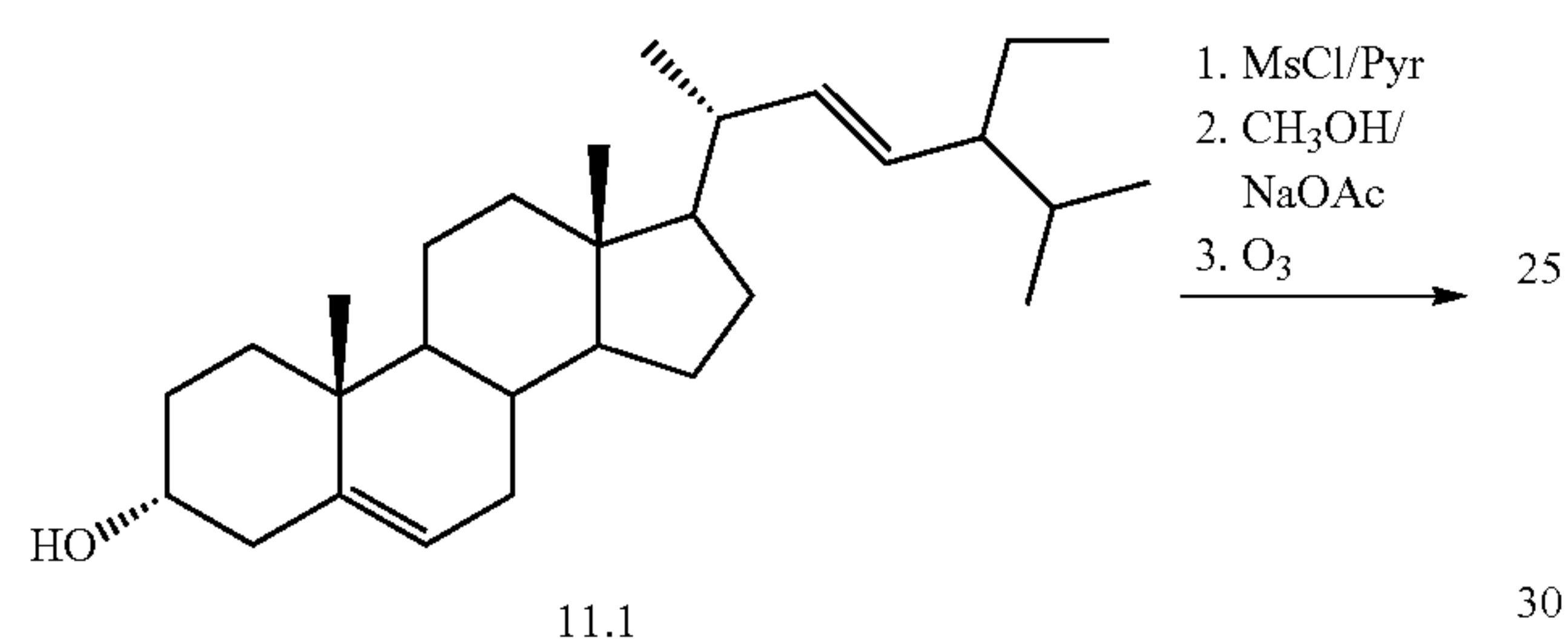
Scheme 11. Ozonolysis of i-steroid and side chain reduction
