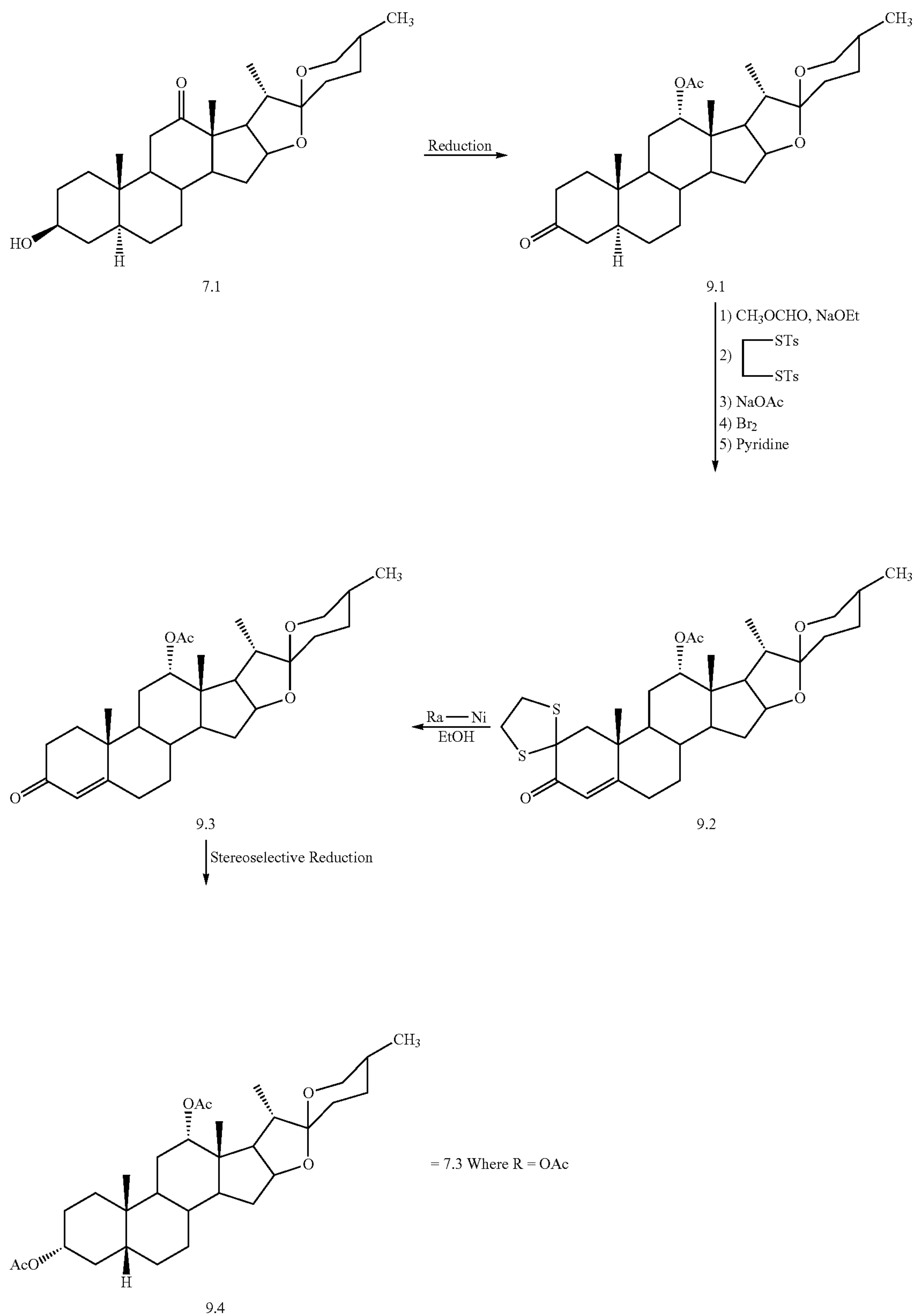
Scheme 9. Dithioethane route to 3-keto-4-ene
