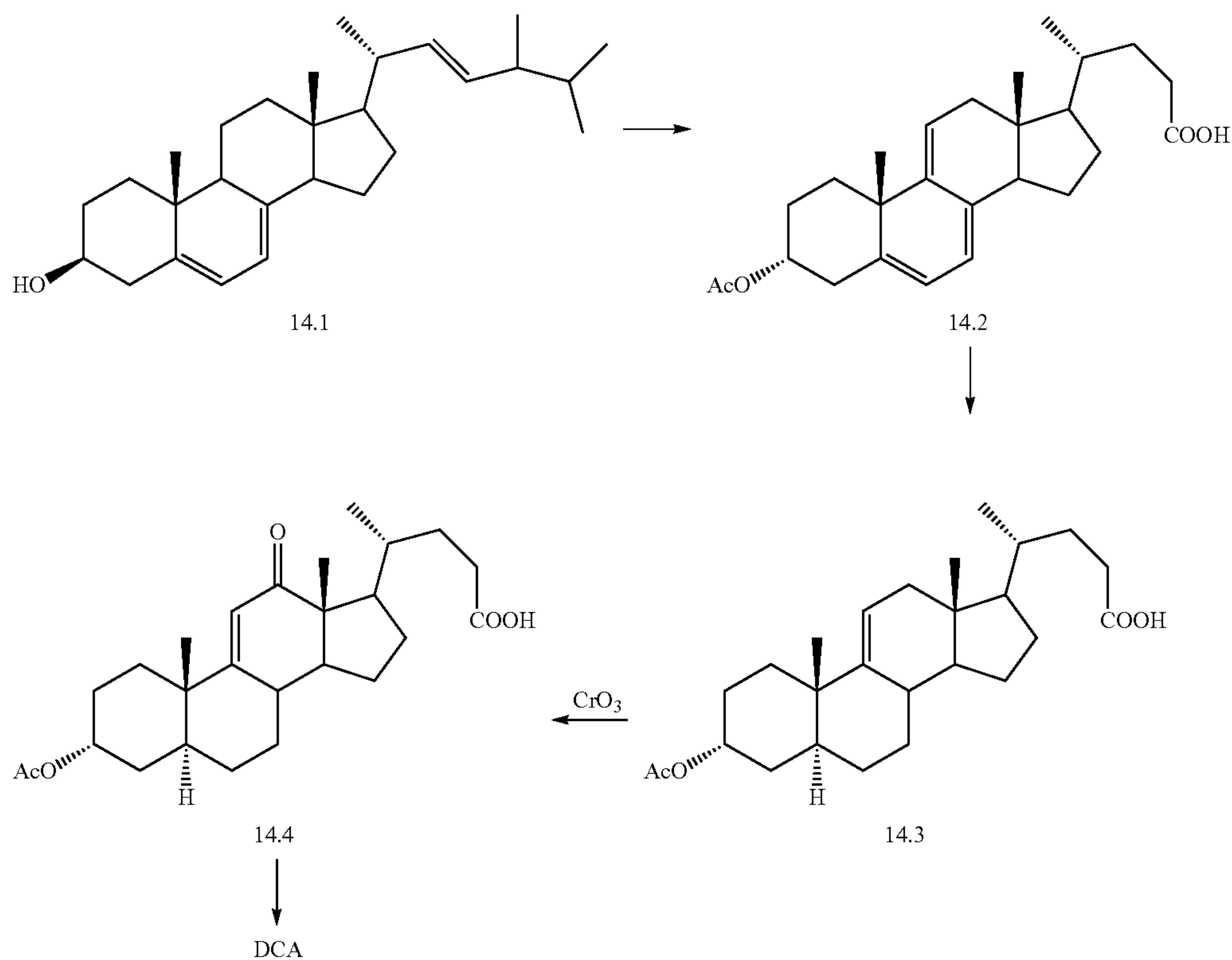
Scheme 14. Triene formation from Ergosterol
