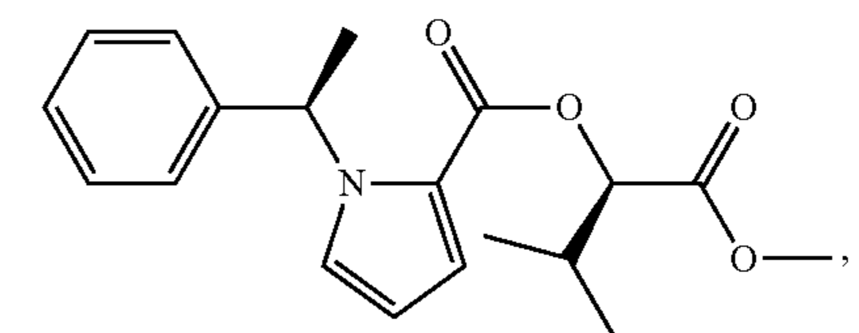
(R-isopropyl-MOC-carbometomidate)
