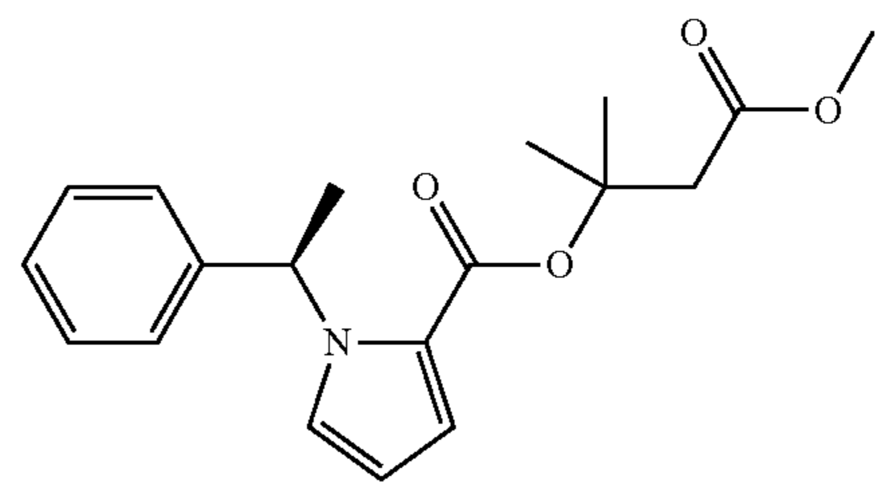
(β-dimethyl-MOC-carboetomidate)
