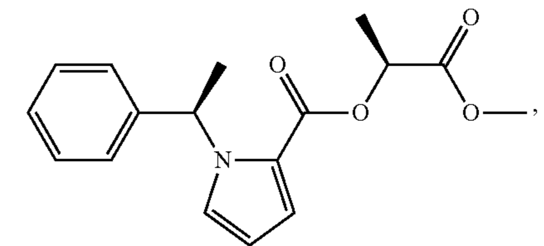
(R-methyl-MOC-carbometomidate)
