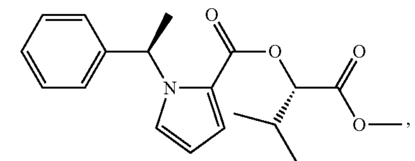
(S-isopropyl-MOC-carbometomidate)
