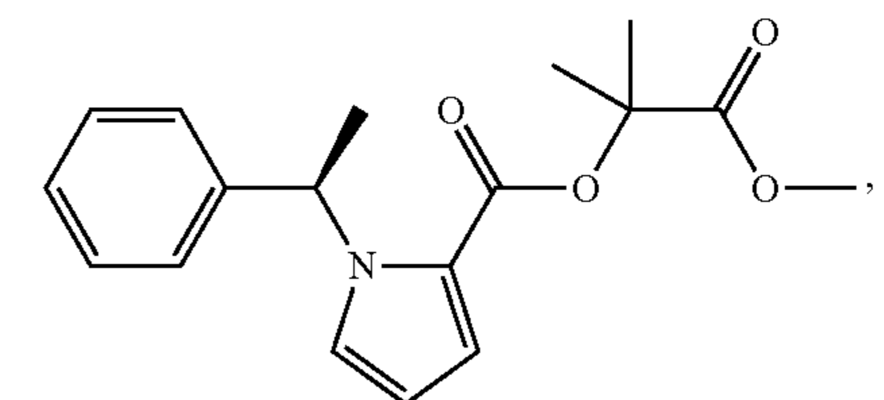
(dimethyl-MOC-carbometomidate)
