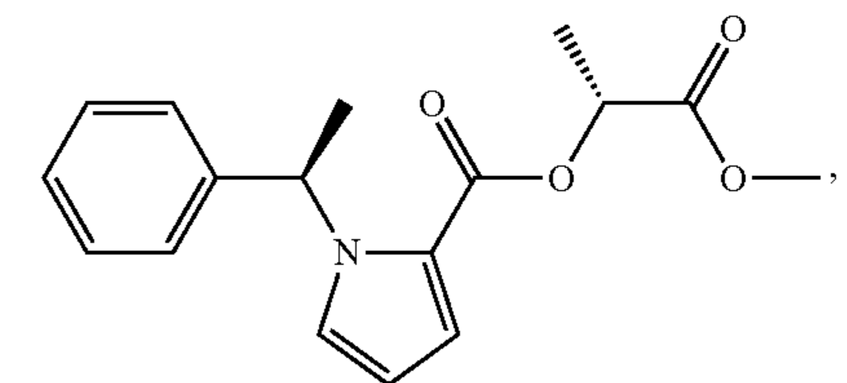
(S-methyl-MOC-carbometomidate)
