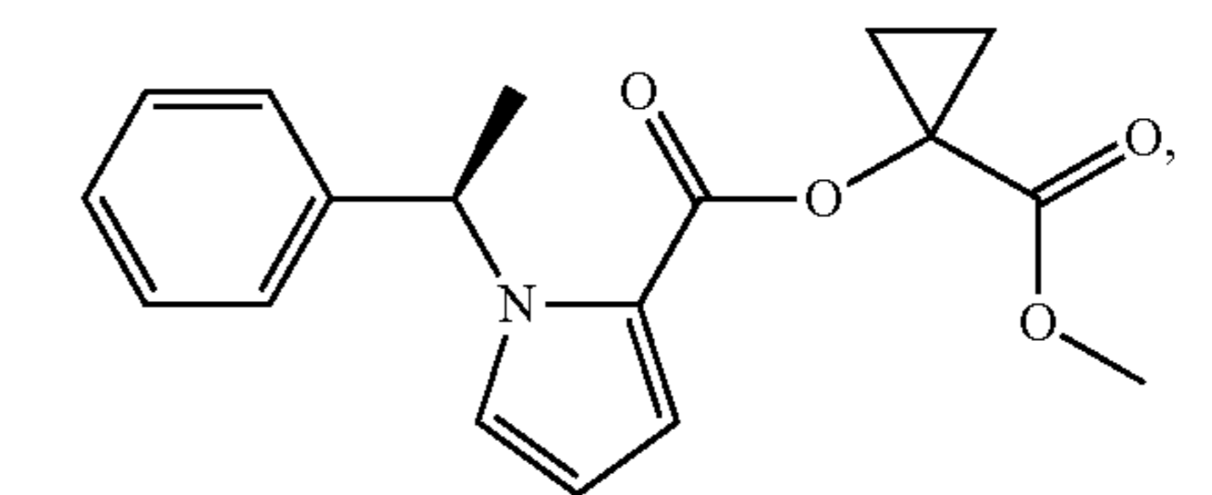
(cyclopropyl-MOC-carbometomidate)
