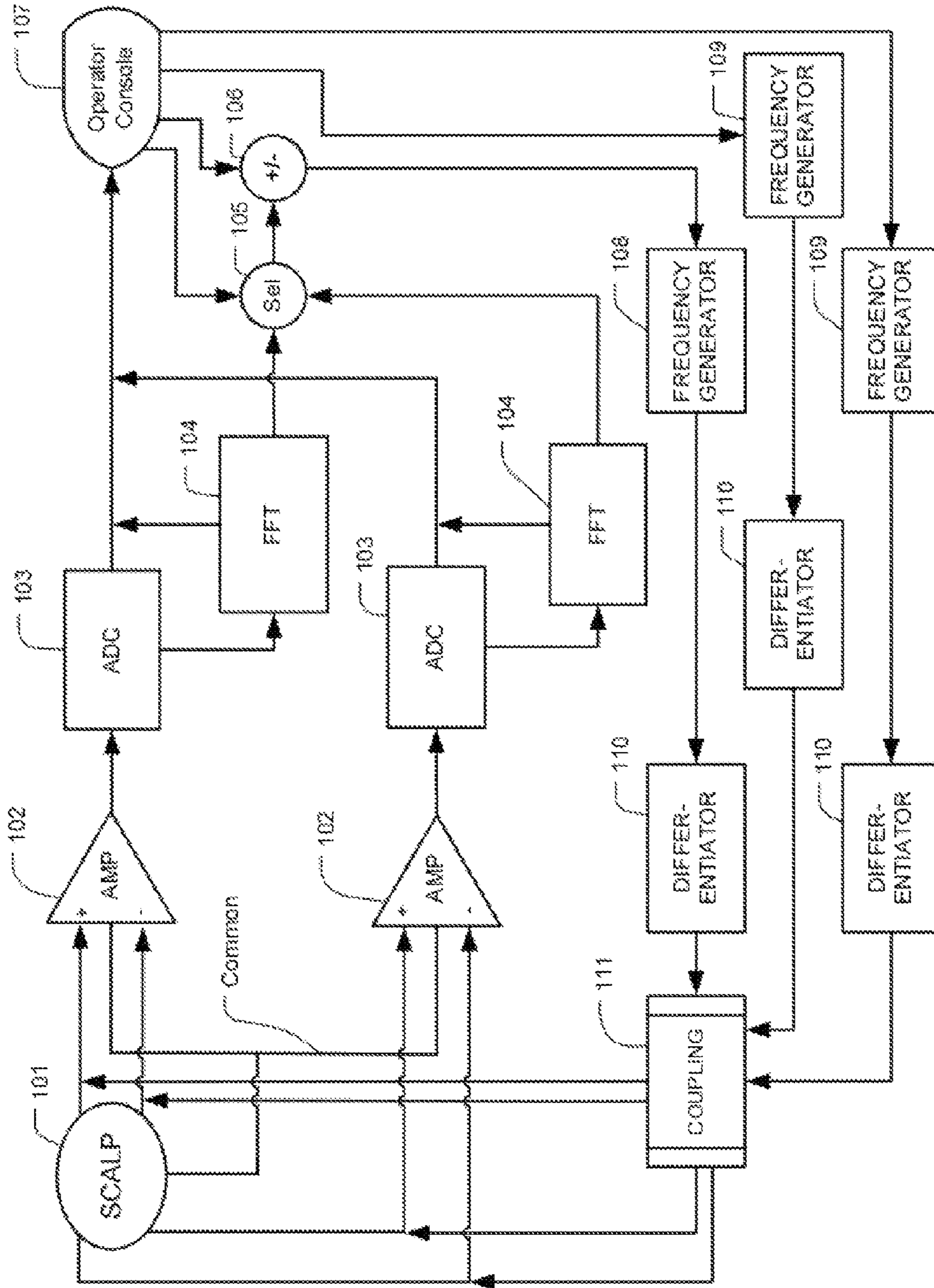
ULTRA LOW POWER DIRECT ELECTRICAL STIMULATION FEEDBACK, EMBODIMENT #1 BLOCK DIAGRAM - FIGURE 1
