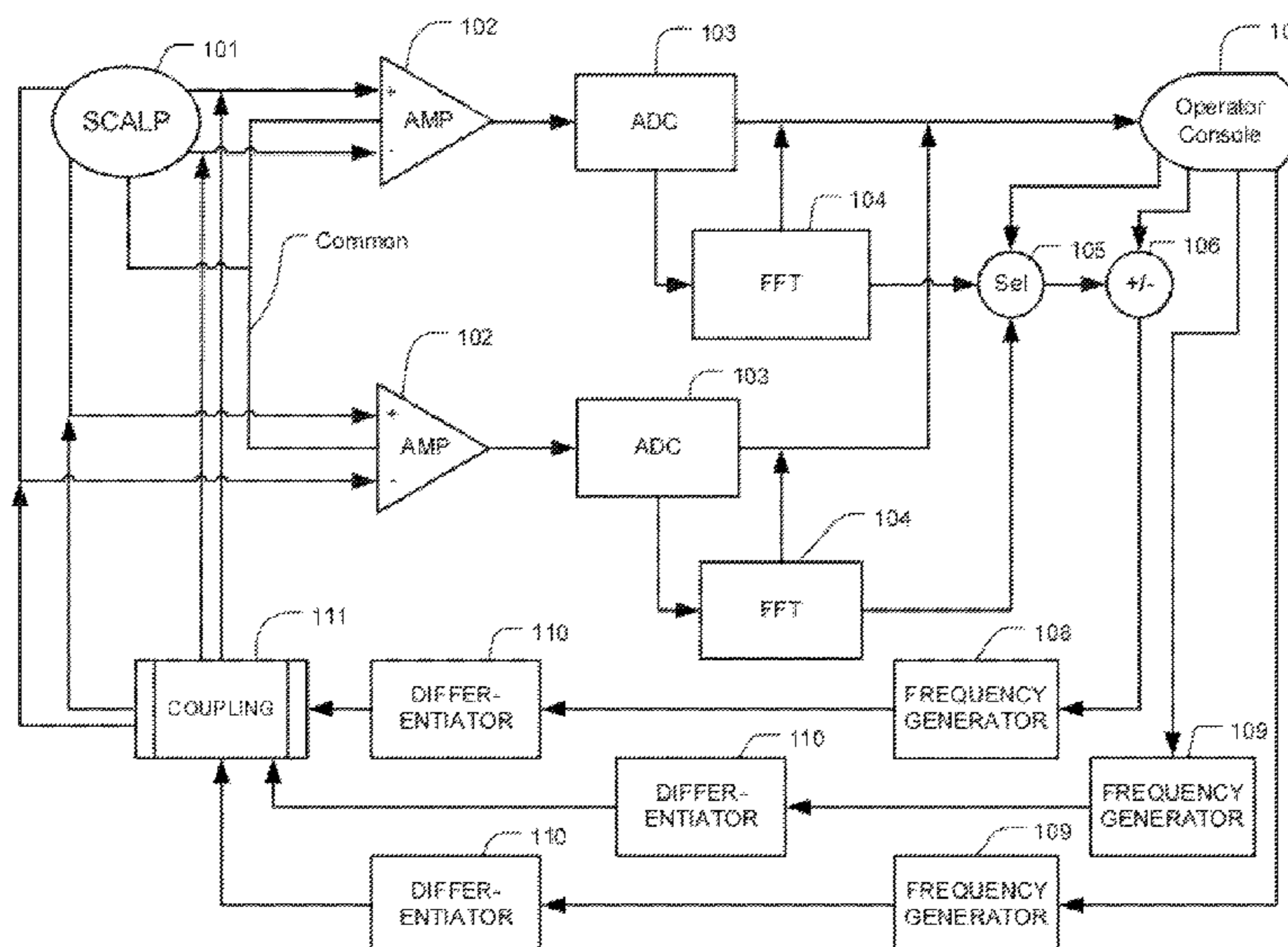
ULTRA LOW POWER DIRECT ELECTRICAL STIMULATION FEEDBACK, EMBODIMENT #1 BLOCK DIAGRAM
