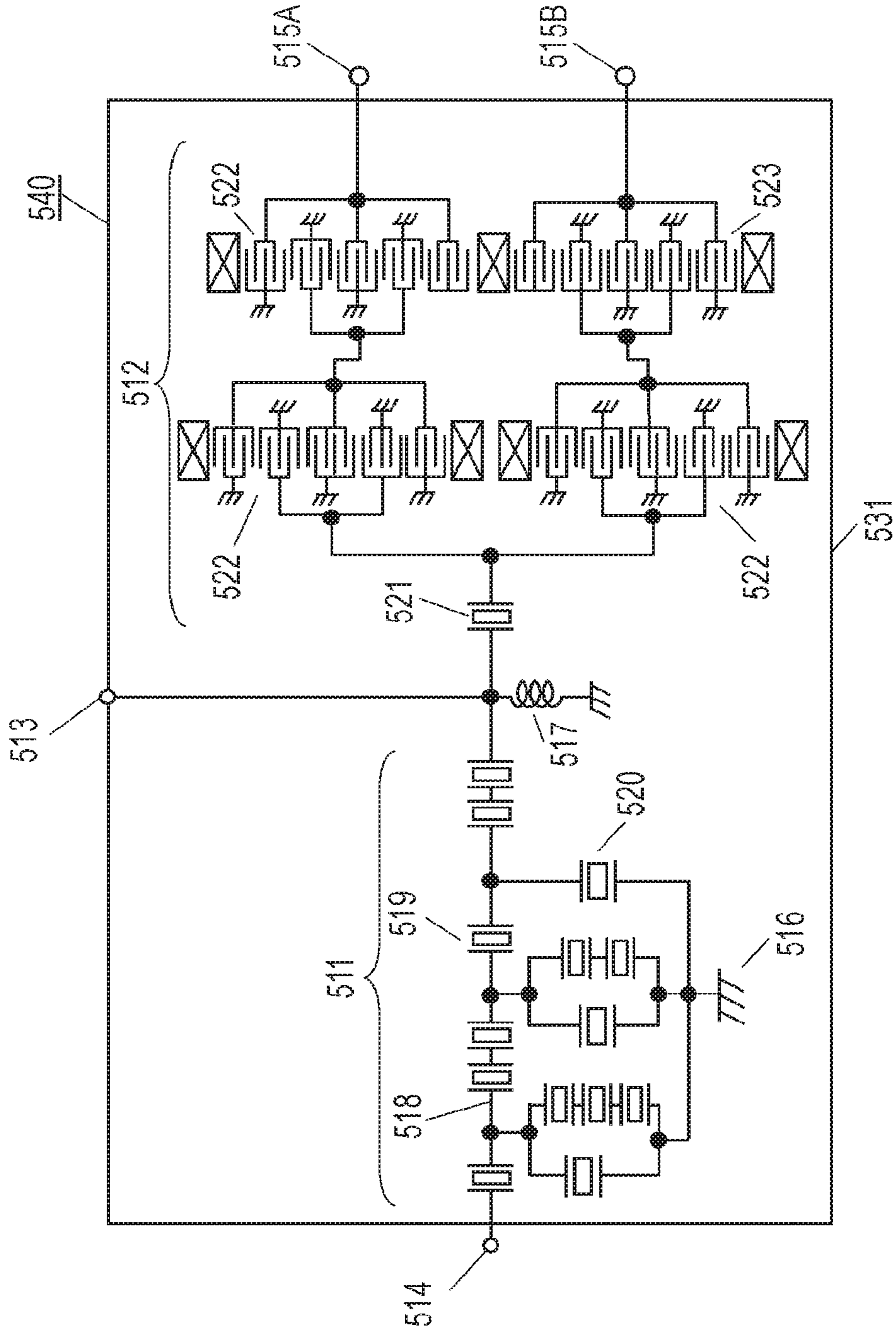
Fig. 31 PRIOR ART
