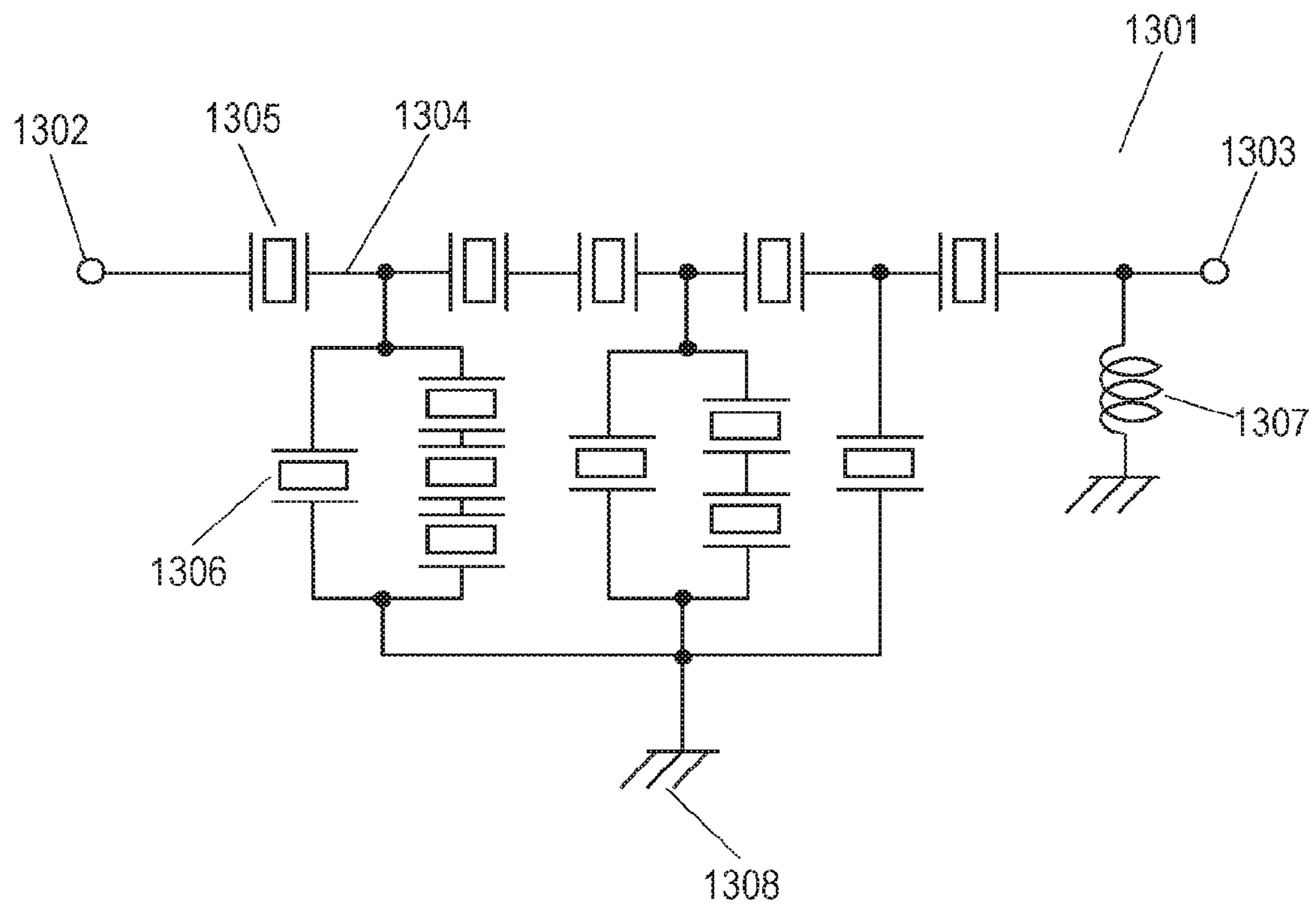
Fig. 28 PRIOR ART
