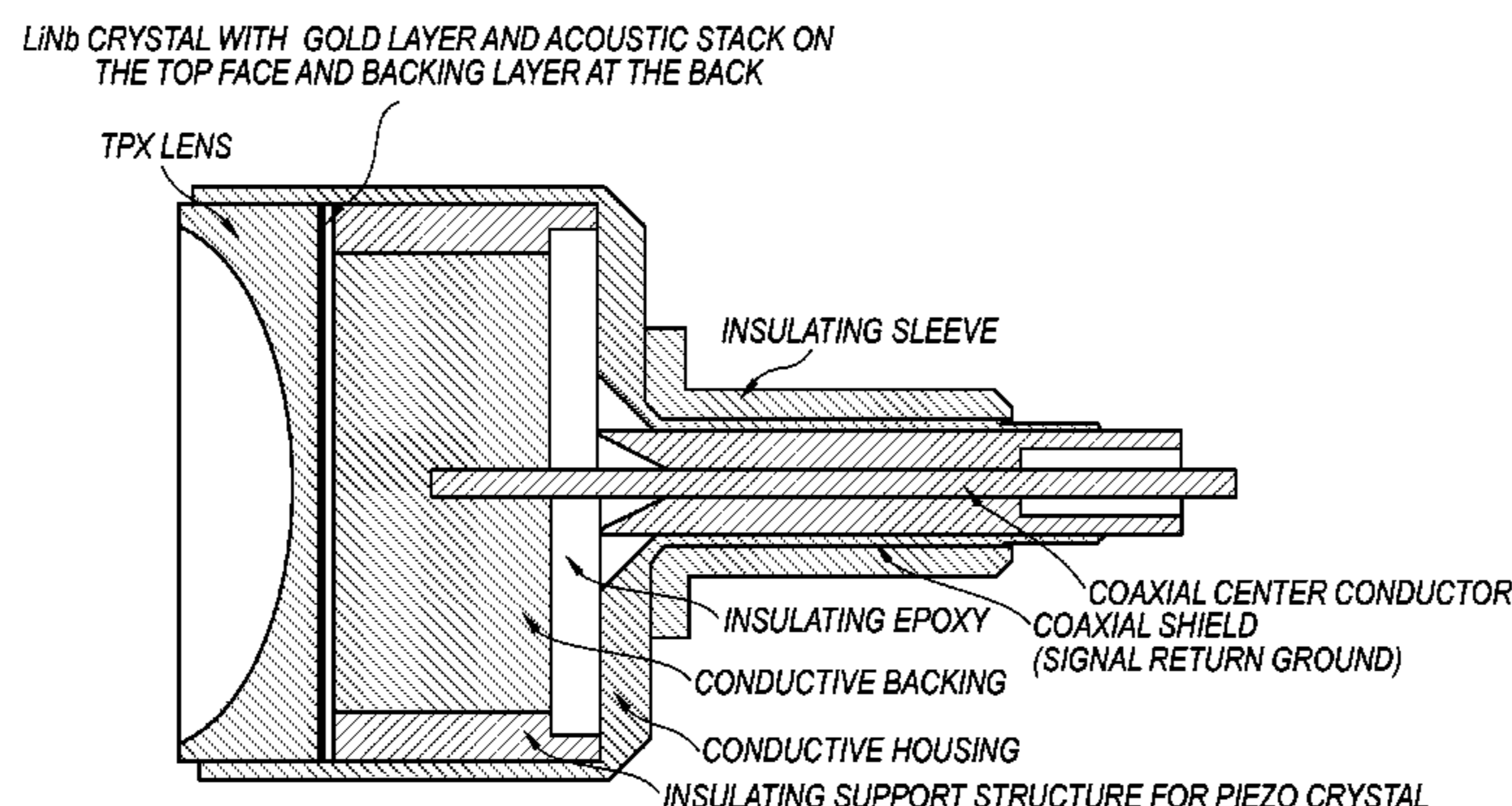
A GROUND CONNECTION IS MADE BETWEEN THE CONDUCTIVE HOUSING AND THE GOLD LAYER ON THE FACE OF THE LiNbO3 CRYSTAL
