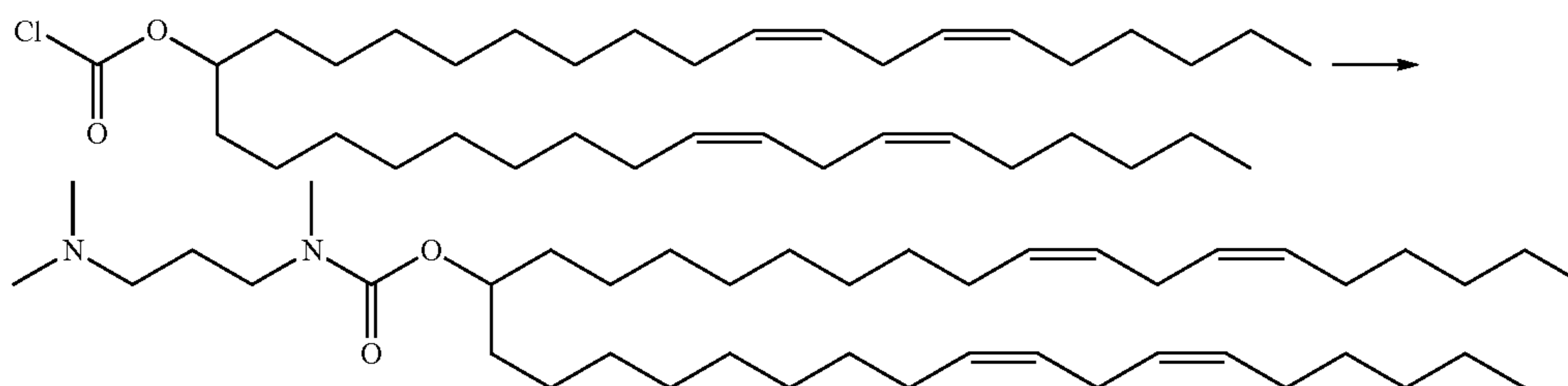
Scheme 5
