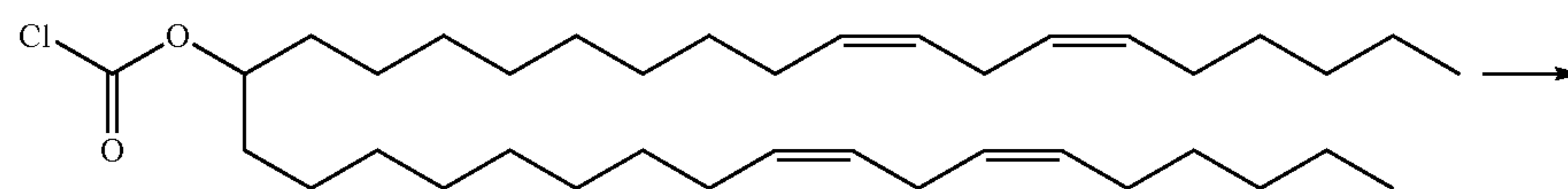
Scheme 7
