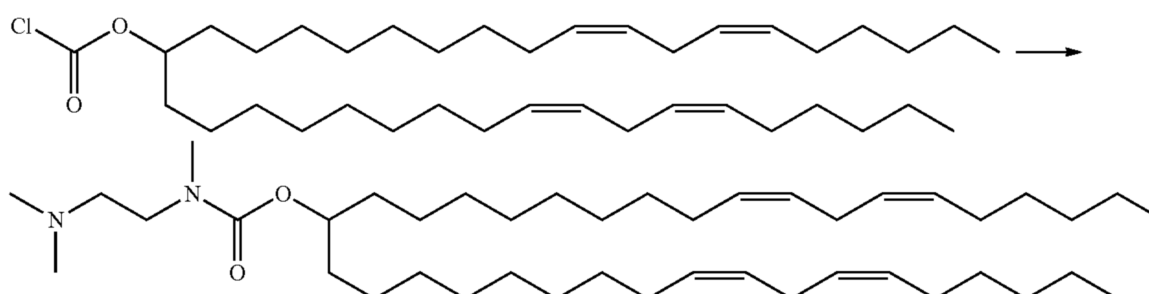
Scheme 6
