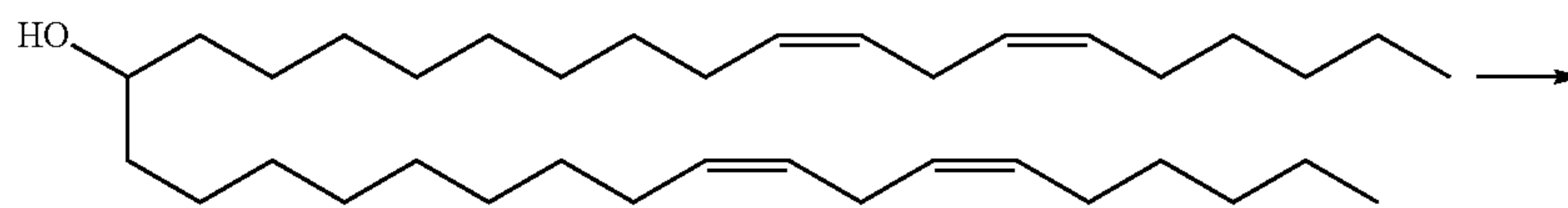
Scheme 8
