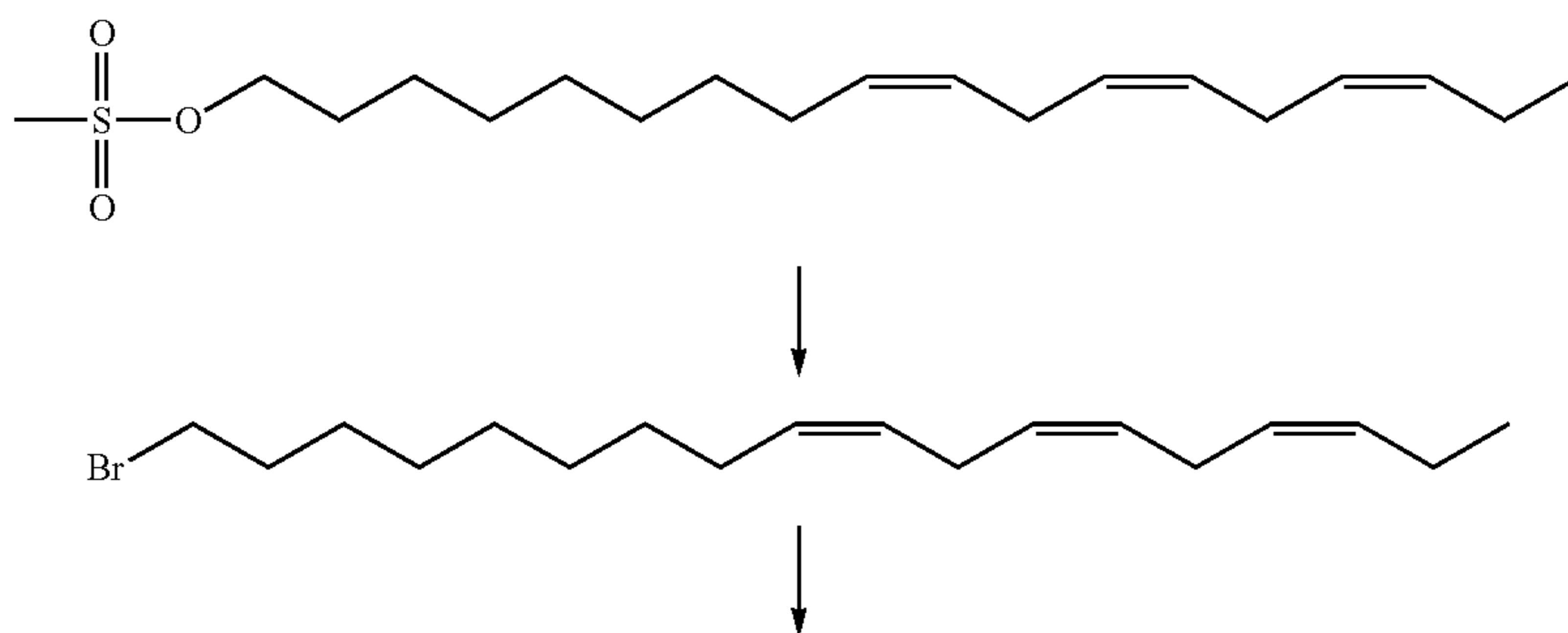
Scheme 2
