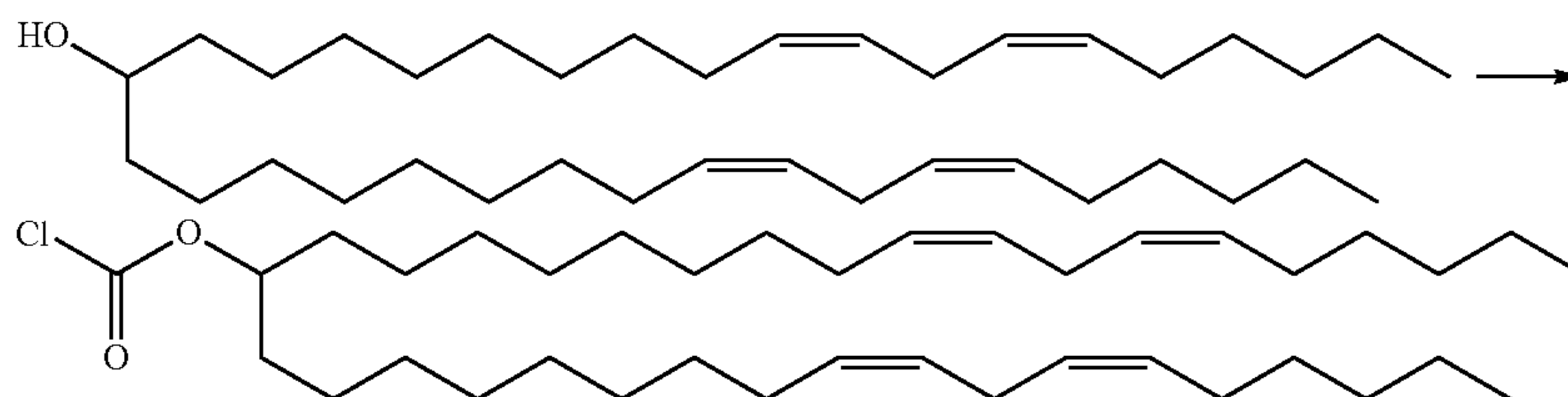
Scheme 4
