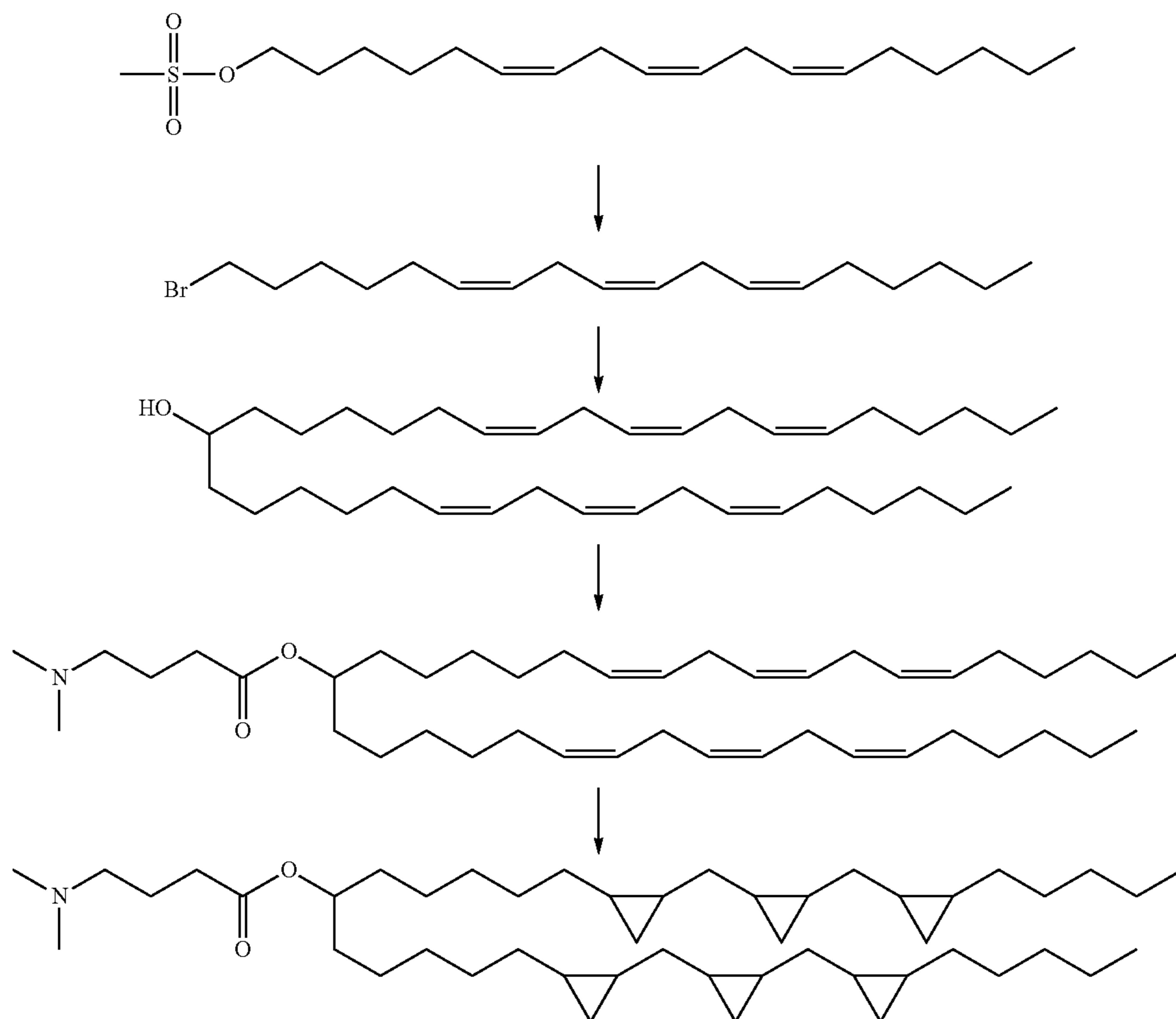
Scheme 3
