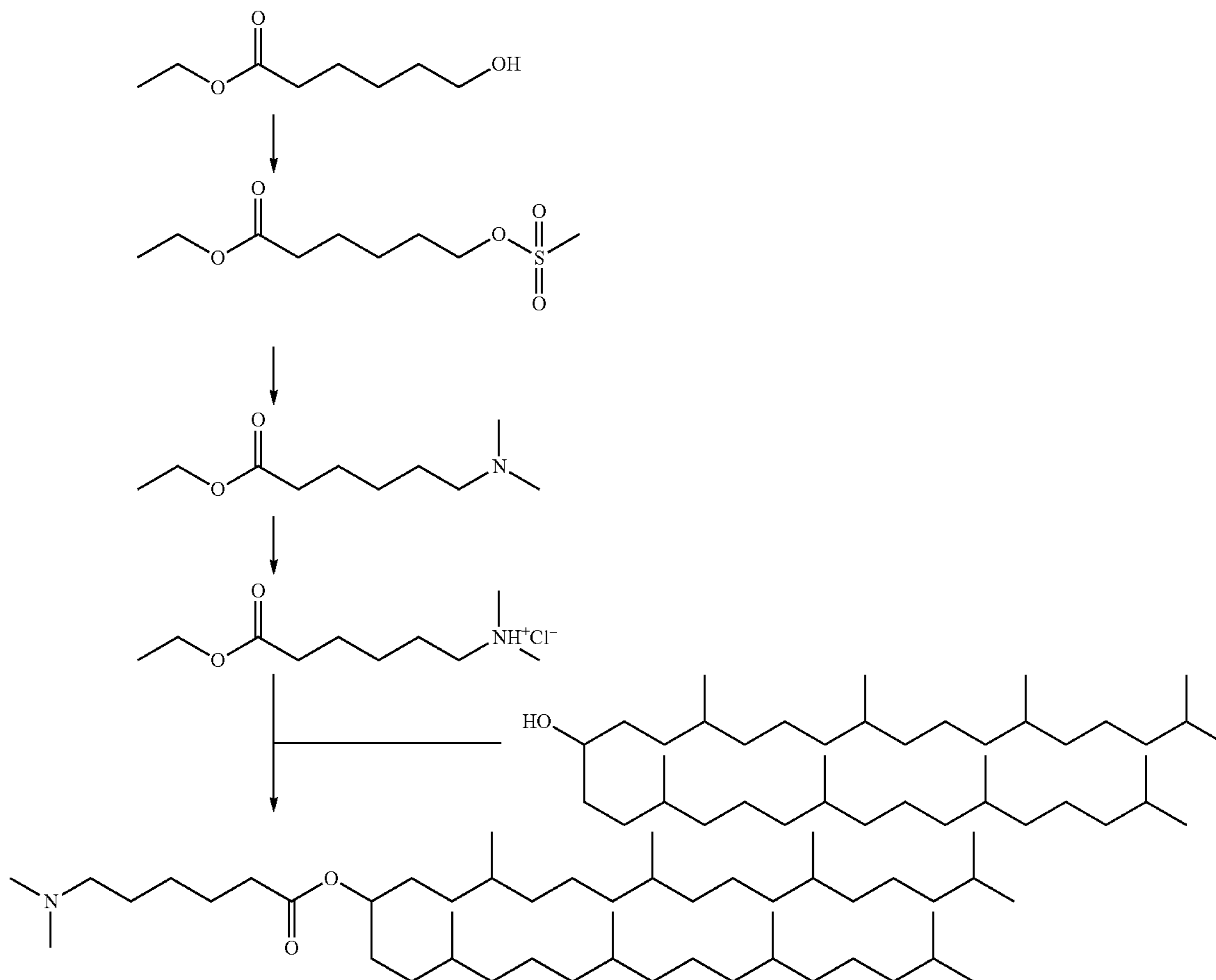
Scheme 14
