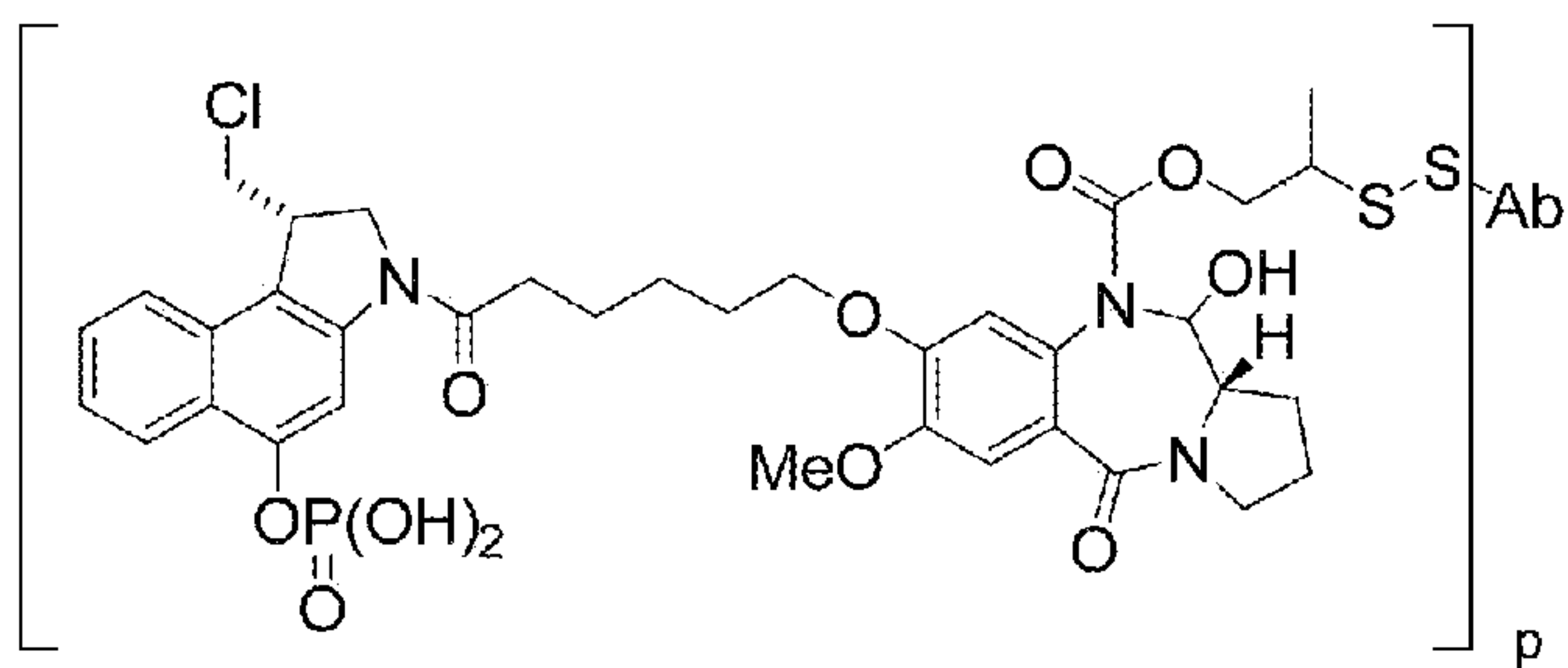
FIG. 12F: thio-hu7C2-LC-K149C-disulfide-CBI-PBD (phosphate)
