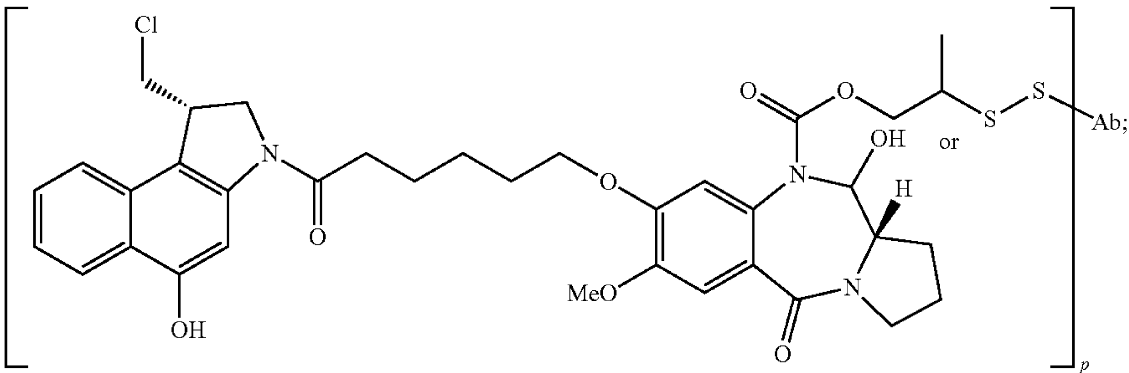
CBI-PBD-disulfide-Ab
