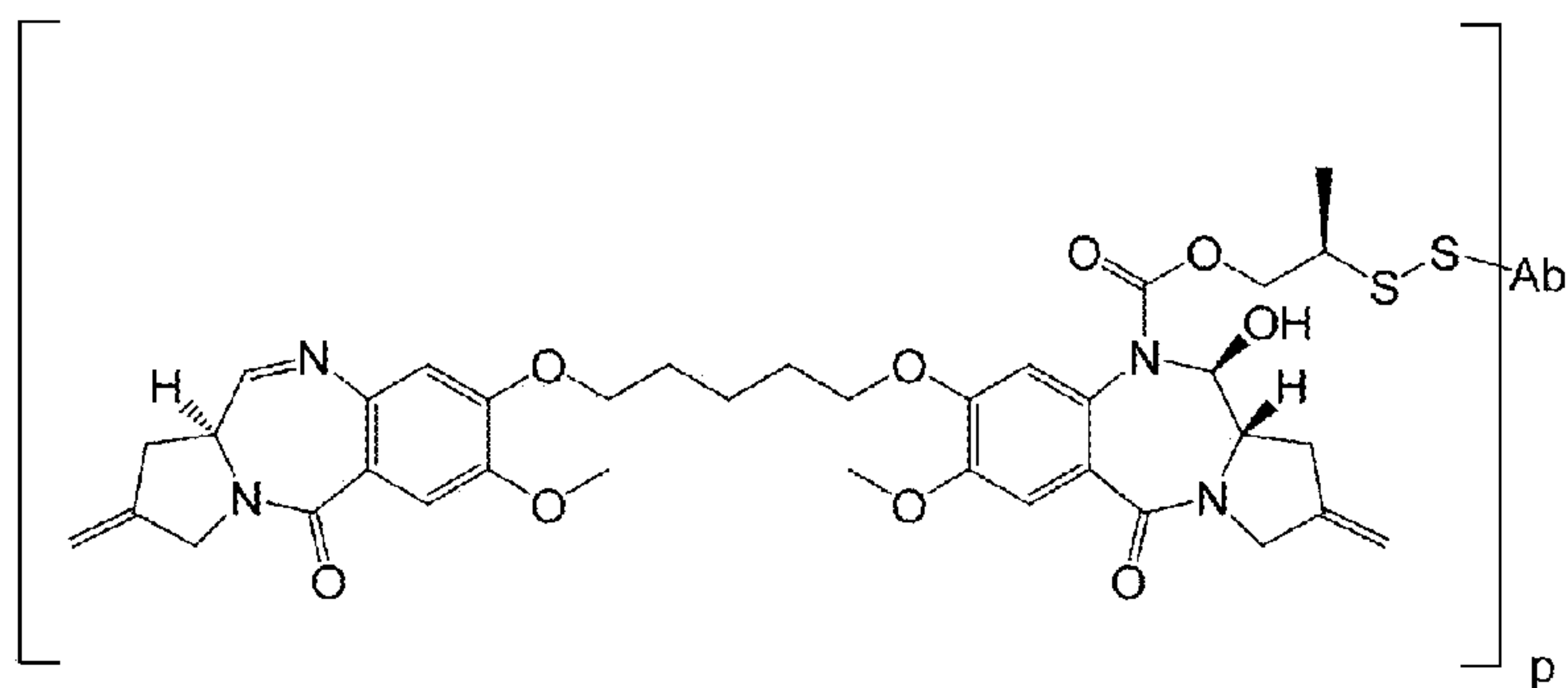
FIG. 12A: thio-hu7C2-HC-A118C-disulfide-PBD and thio-hu7C2-LC-K149C-disulfide-PBD
