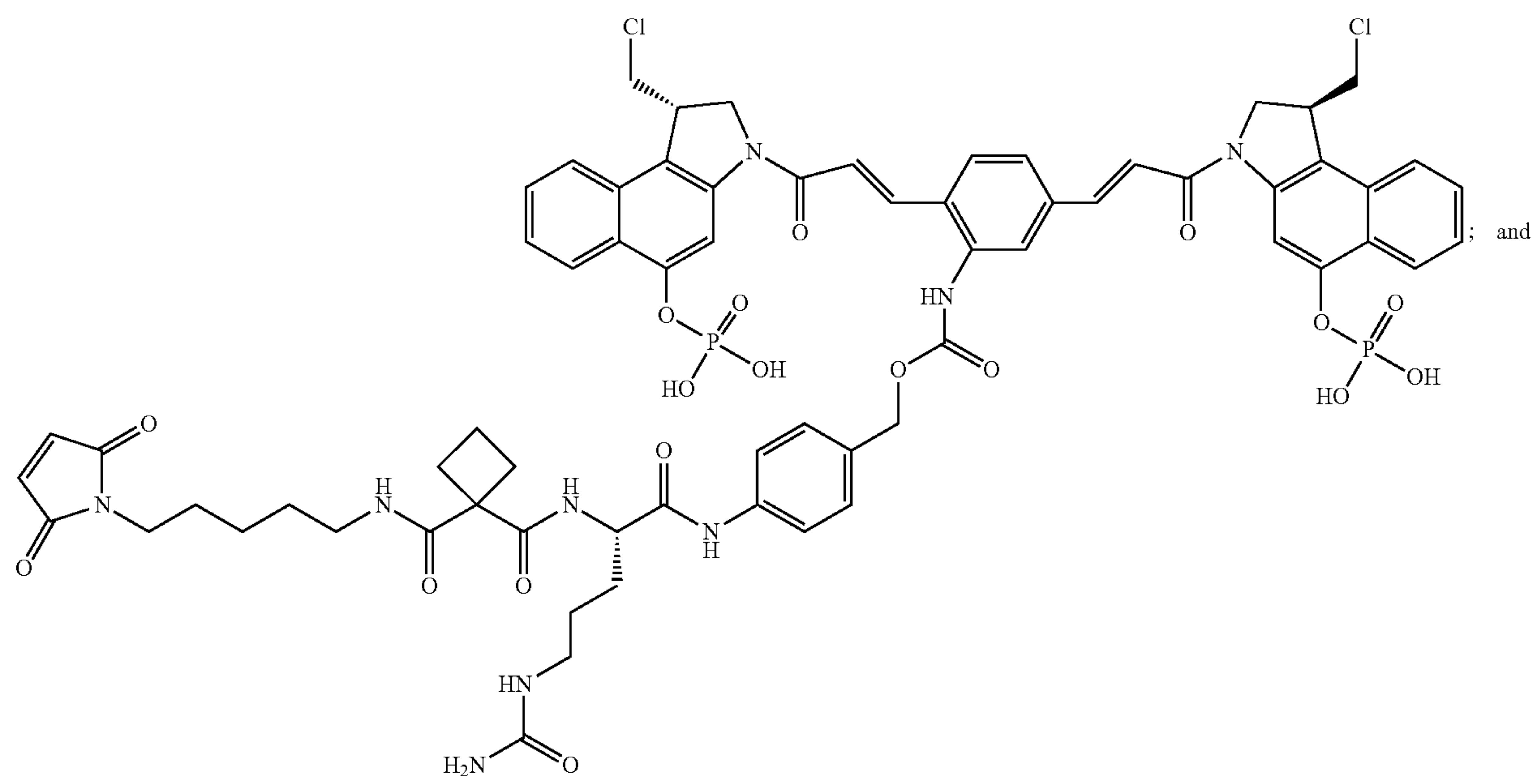
CBI-CBI (phosphate)-peptidomimetic PAB linker 89
