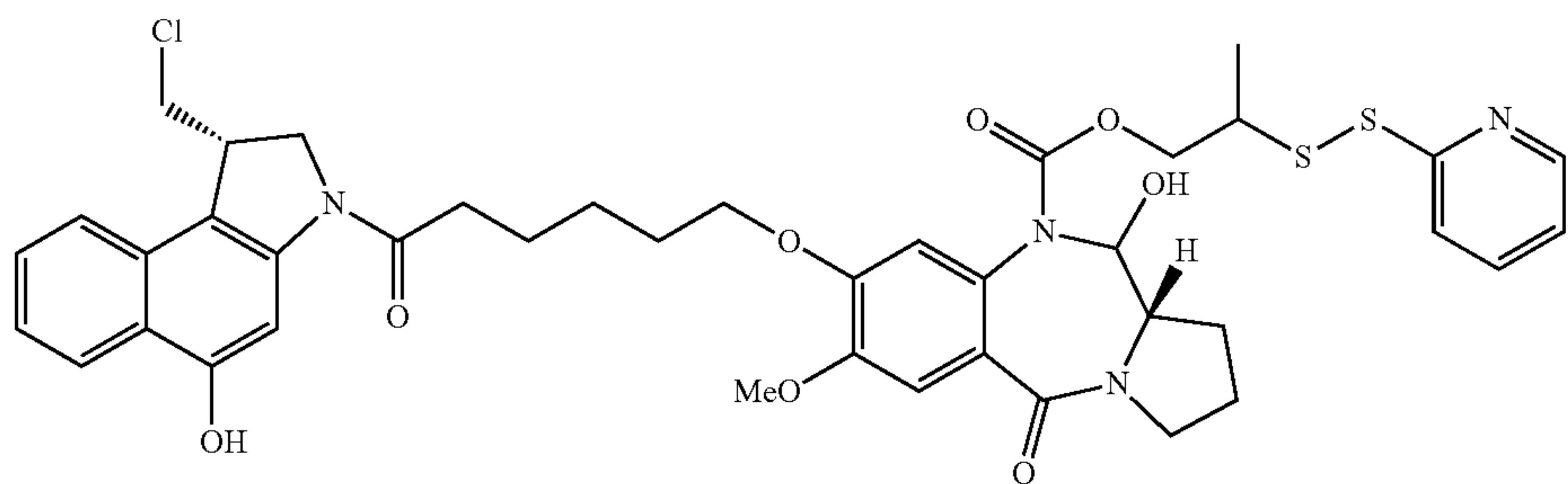
CBI-PBD-2-propyl pyridyl disulfide
