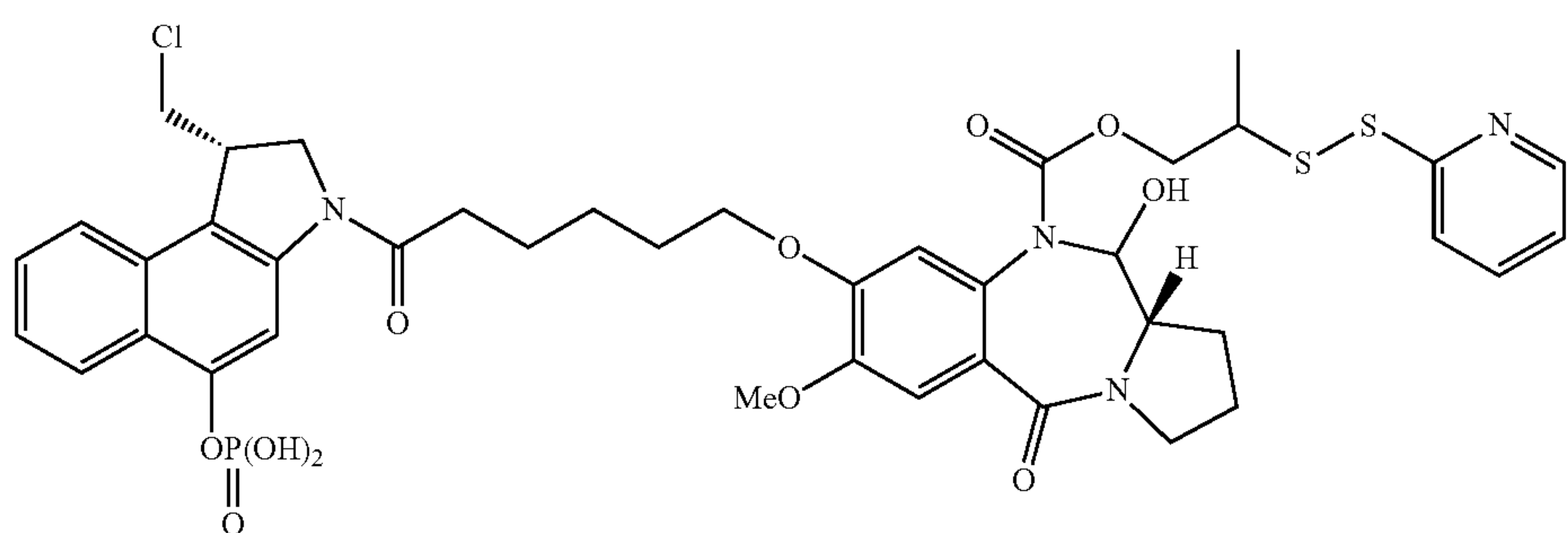
CBI-PBD (phosphate)-2-propyl pyridyl disulfide
