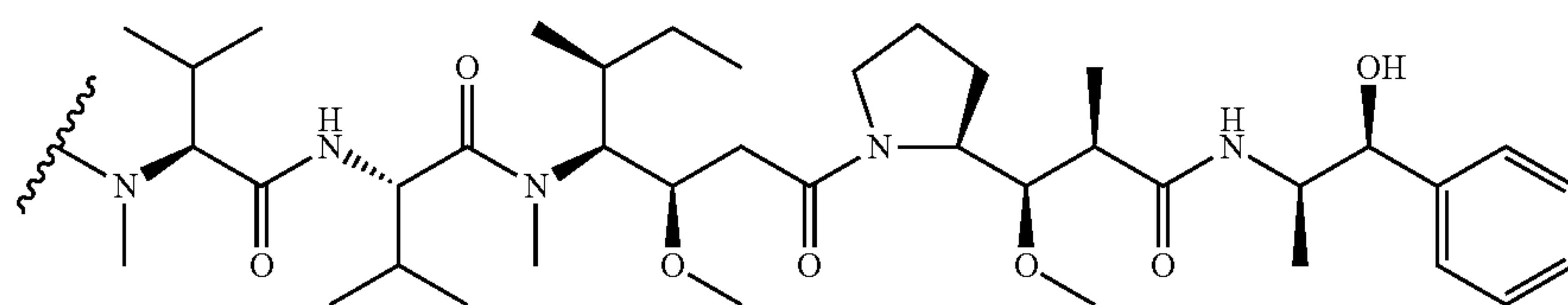
MMAE
