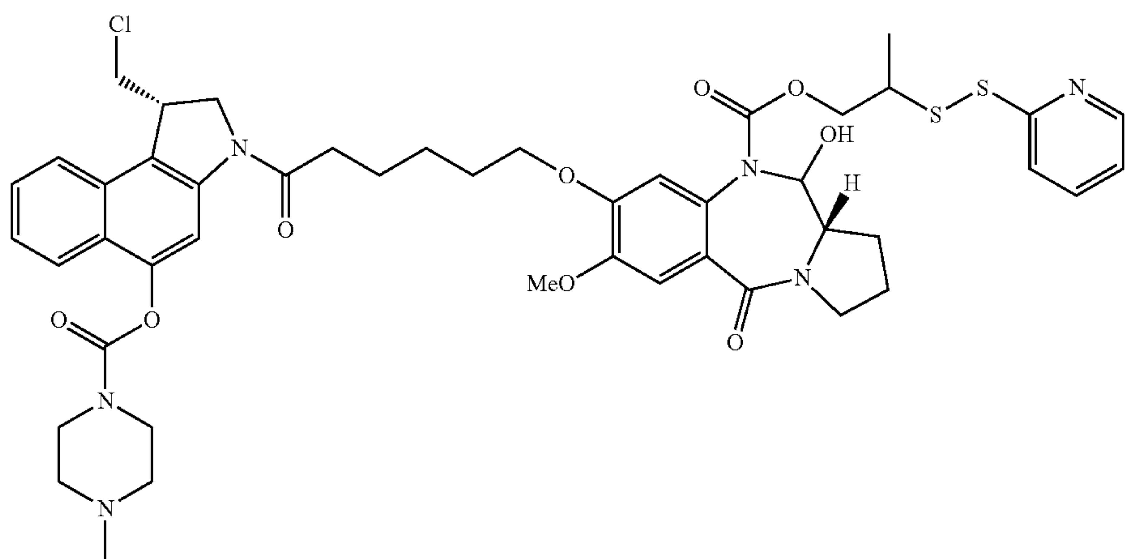
CBI-PBD (piperazine-carbamate prodrug)-2-propyl pyridyl disulfide
