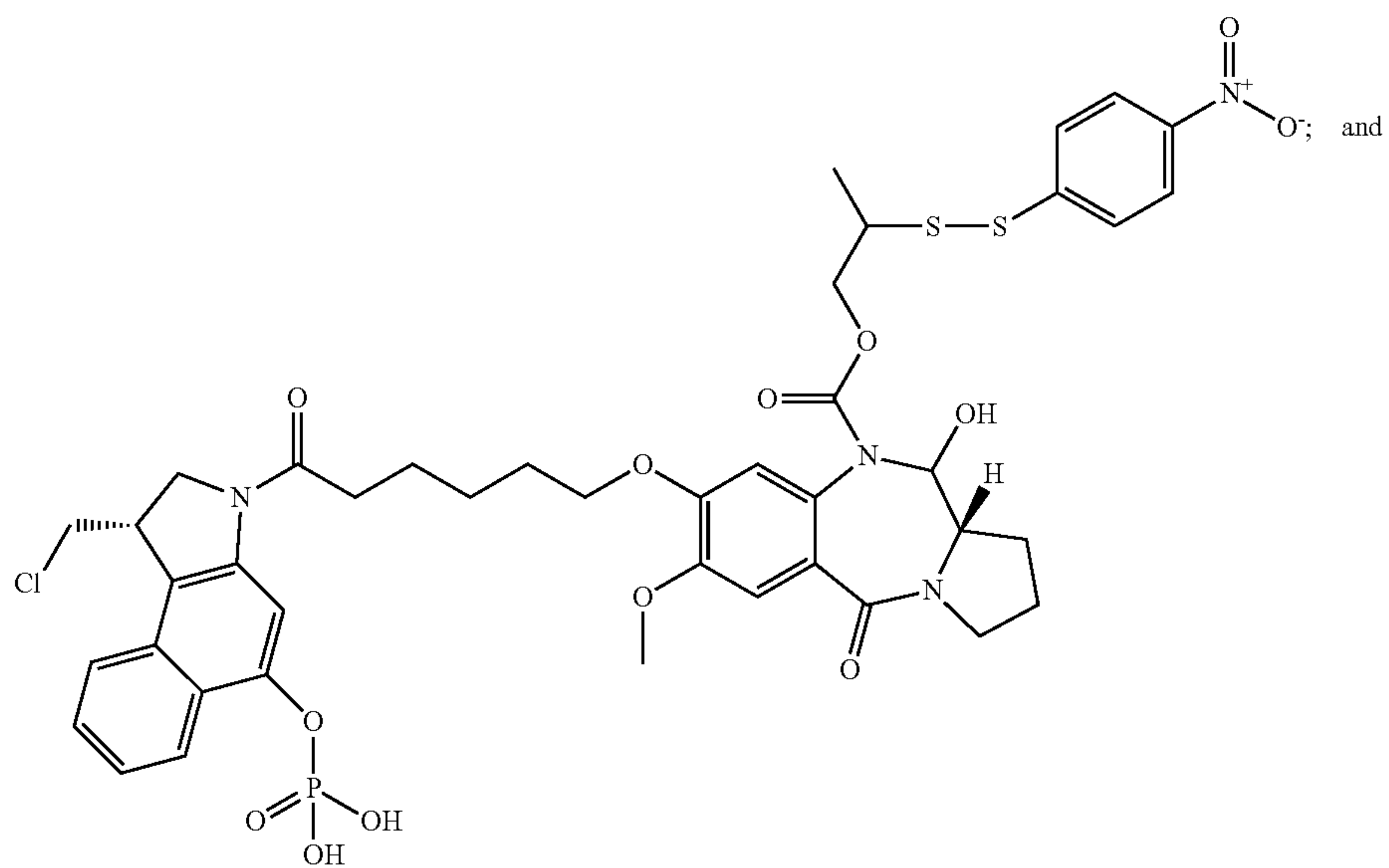
CBI-PBD-(phosphate)-2-propyl, nitropyridyl disulfide
