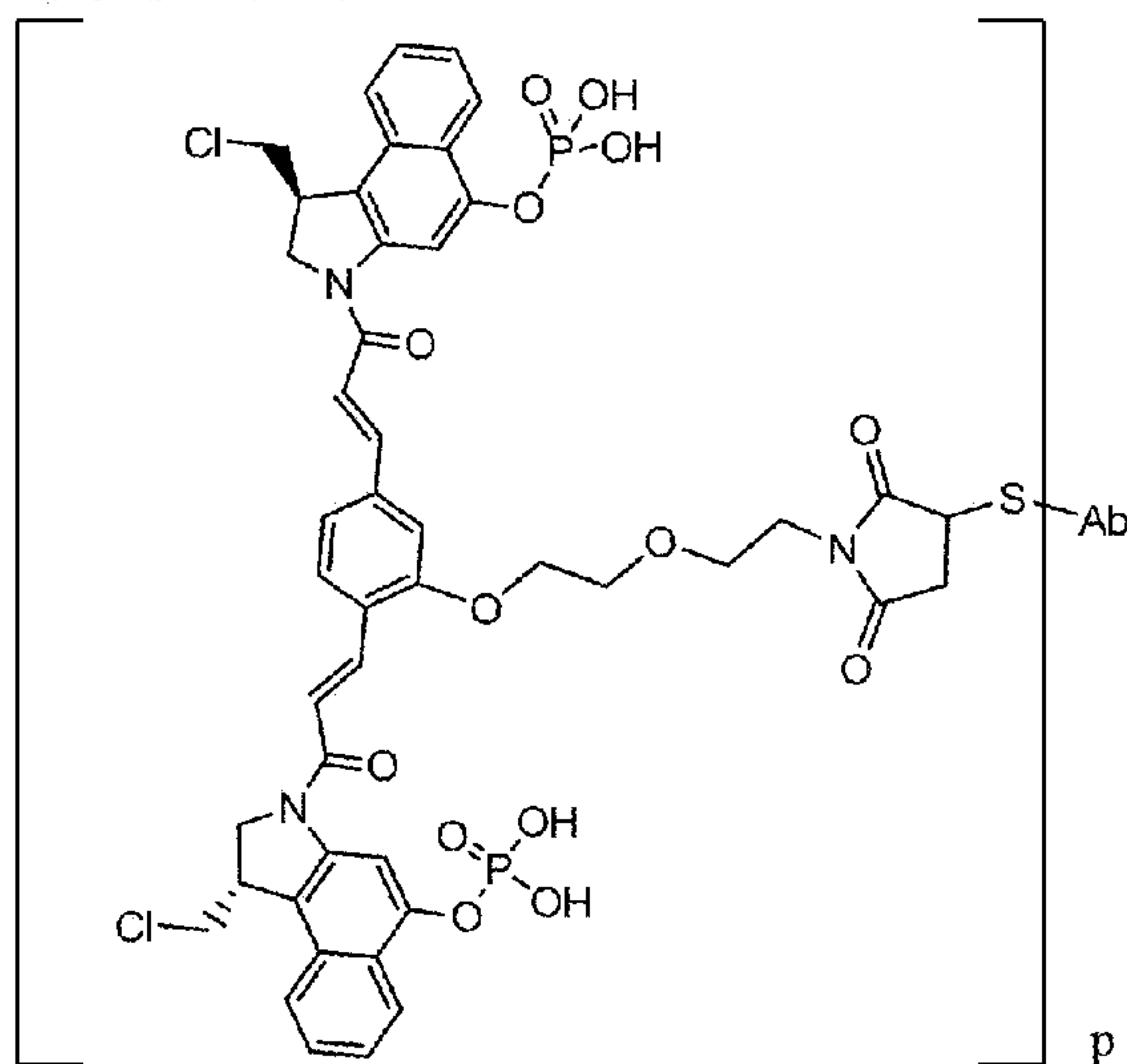
FIG. 12B: thio-hu7C2-LC-K149C-CBI dimer
