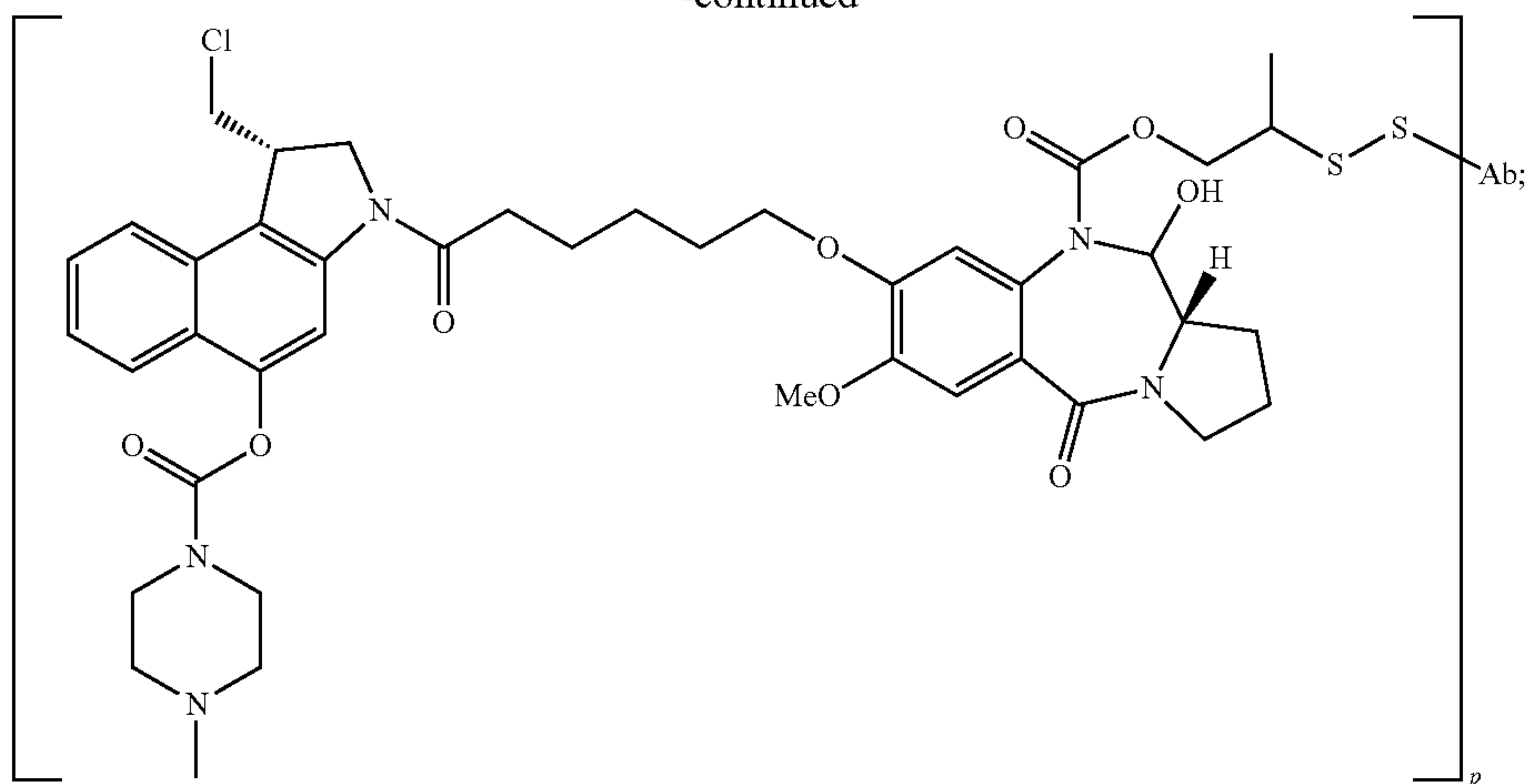
CBI-PBD (piperazine-carbamate prodrug)-disulfide-Ab;
