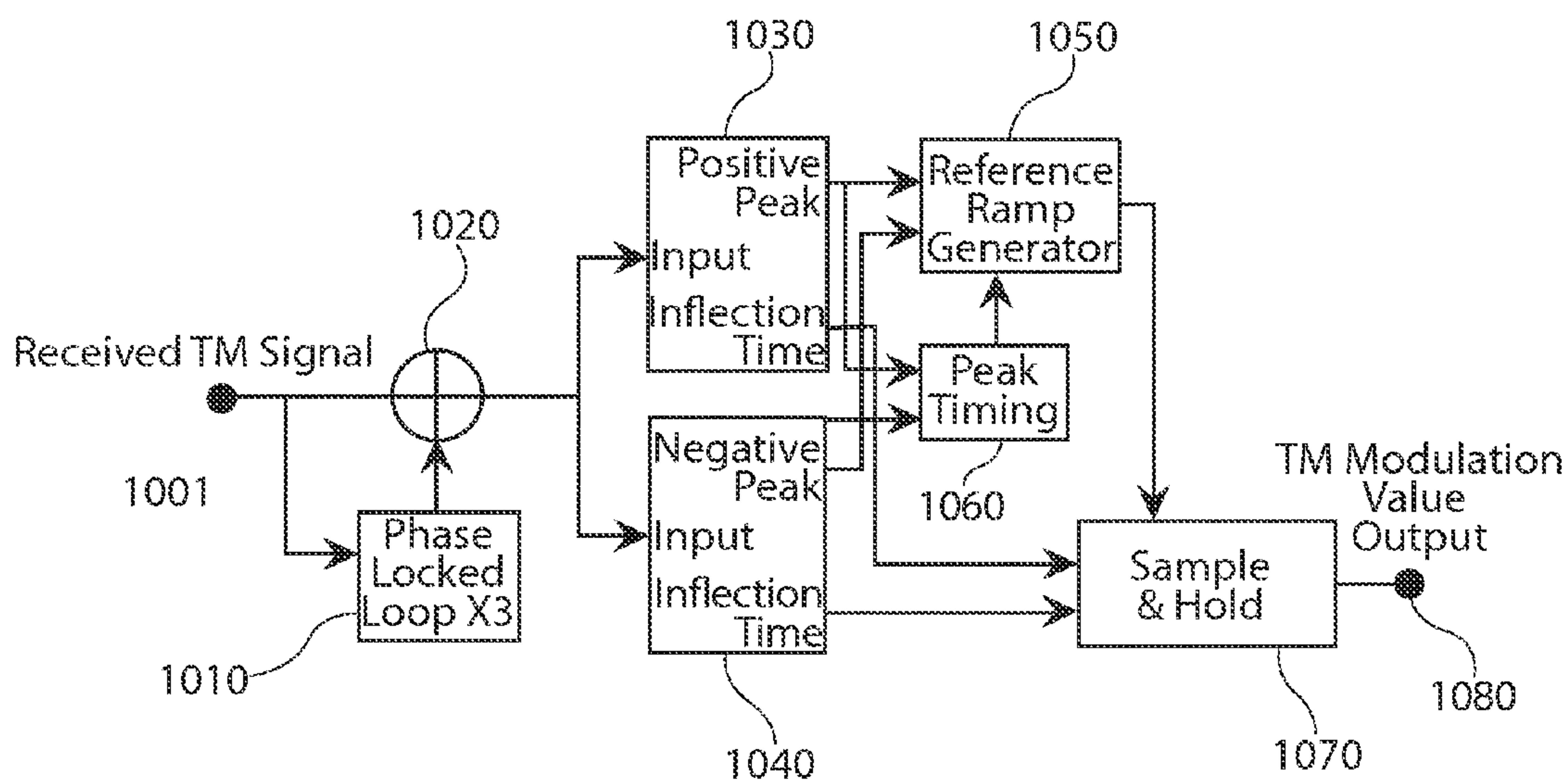
The Sub-Cycle Calibration method of TM demodulation.
