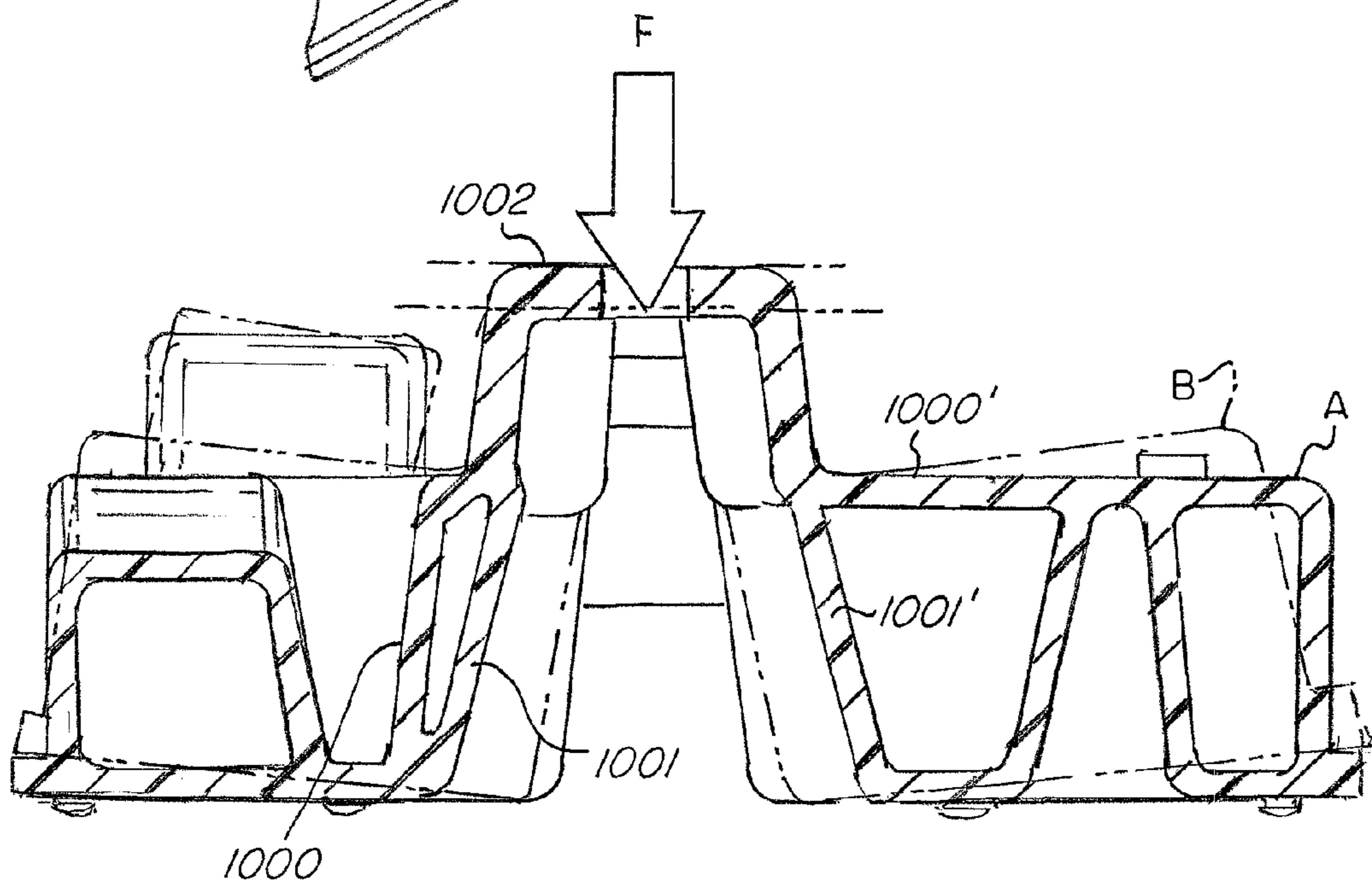
FIG. 10 (PRIOR ART)
