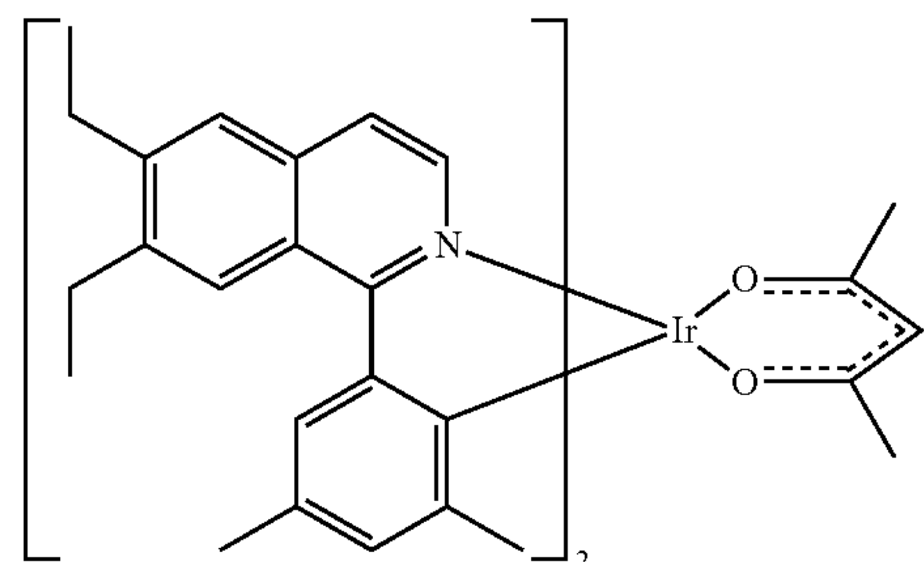
Compound 30
