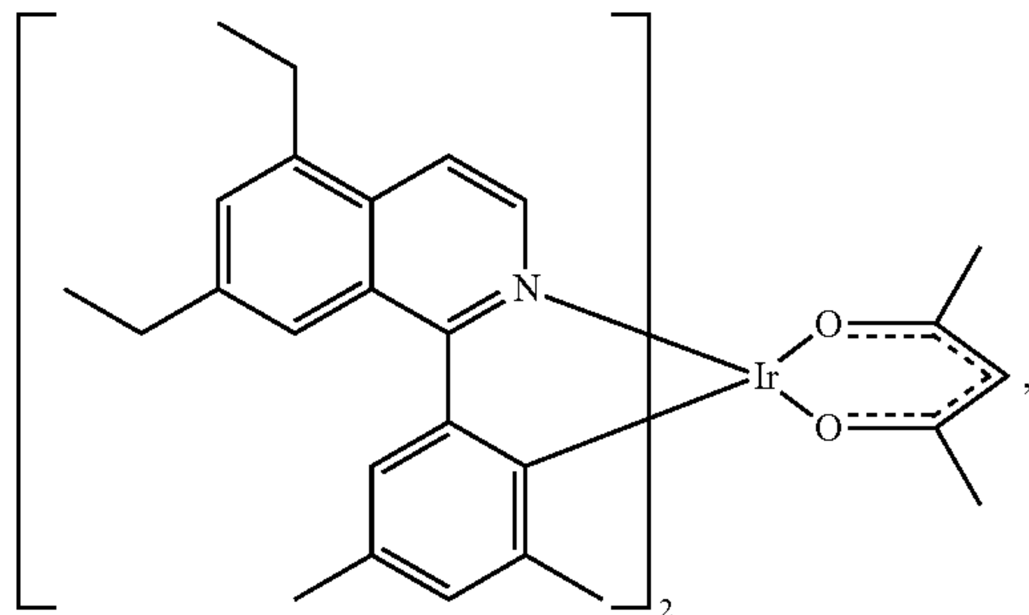
Compound 28
