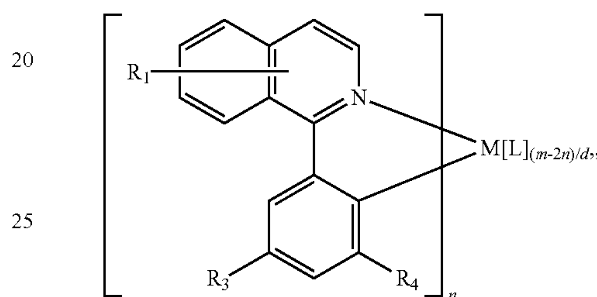
Formula I
