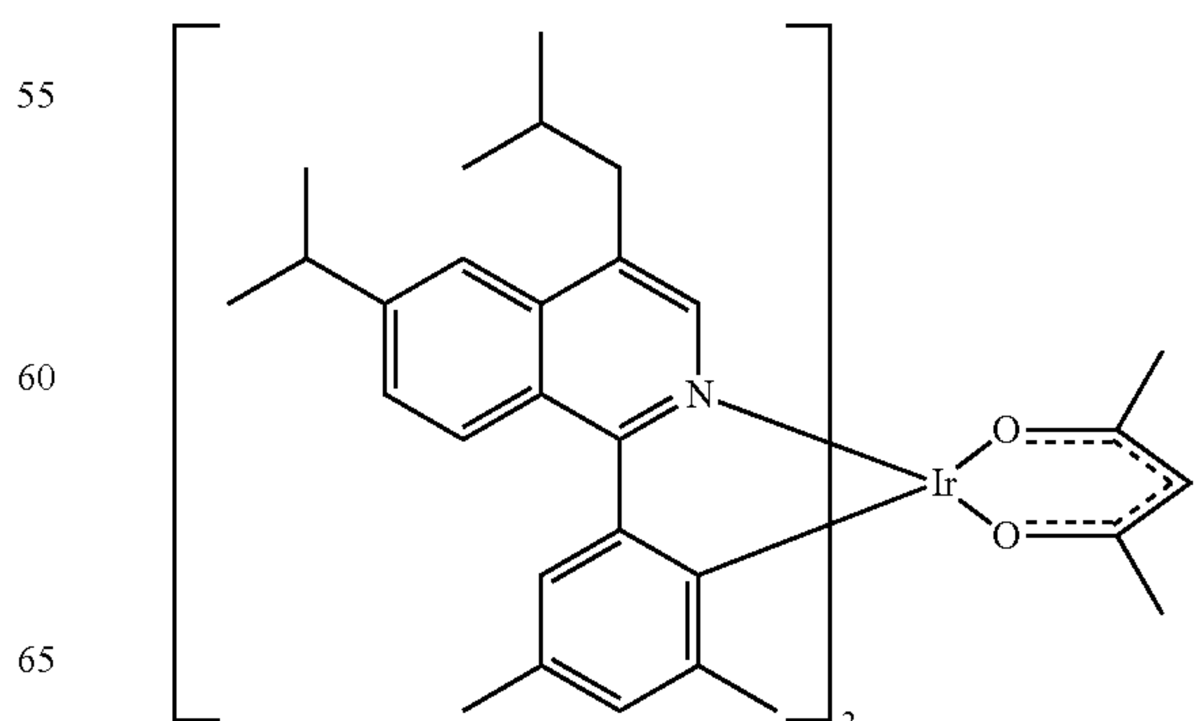
Compound 40
