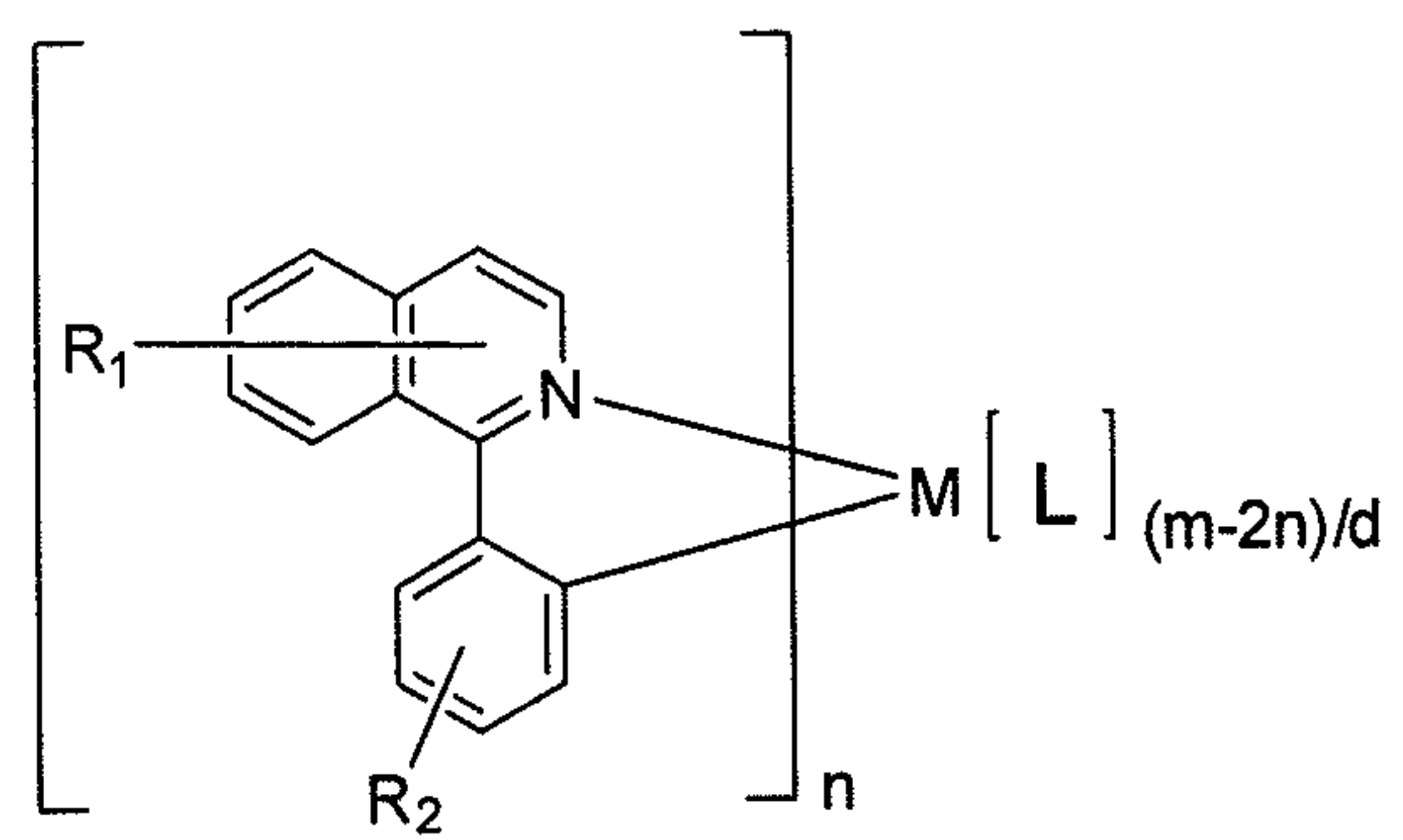
Formula I
