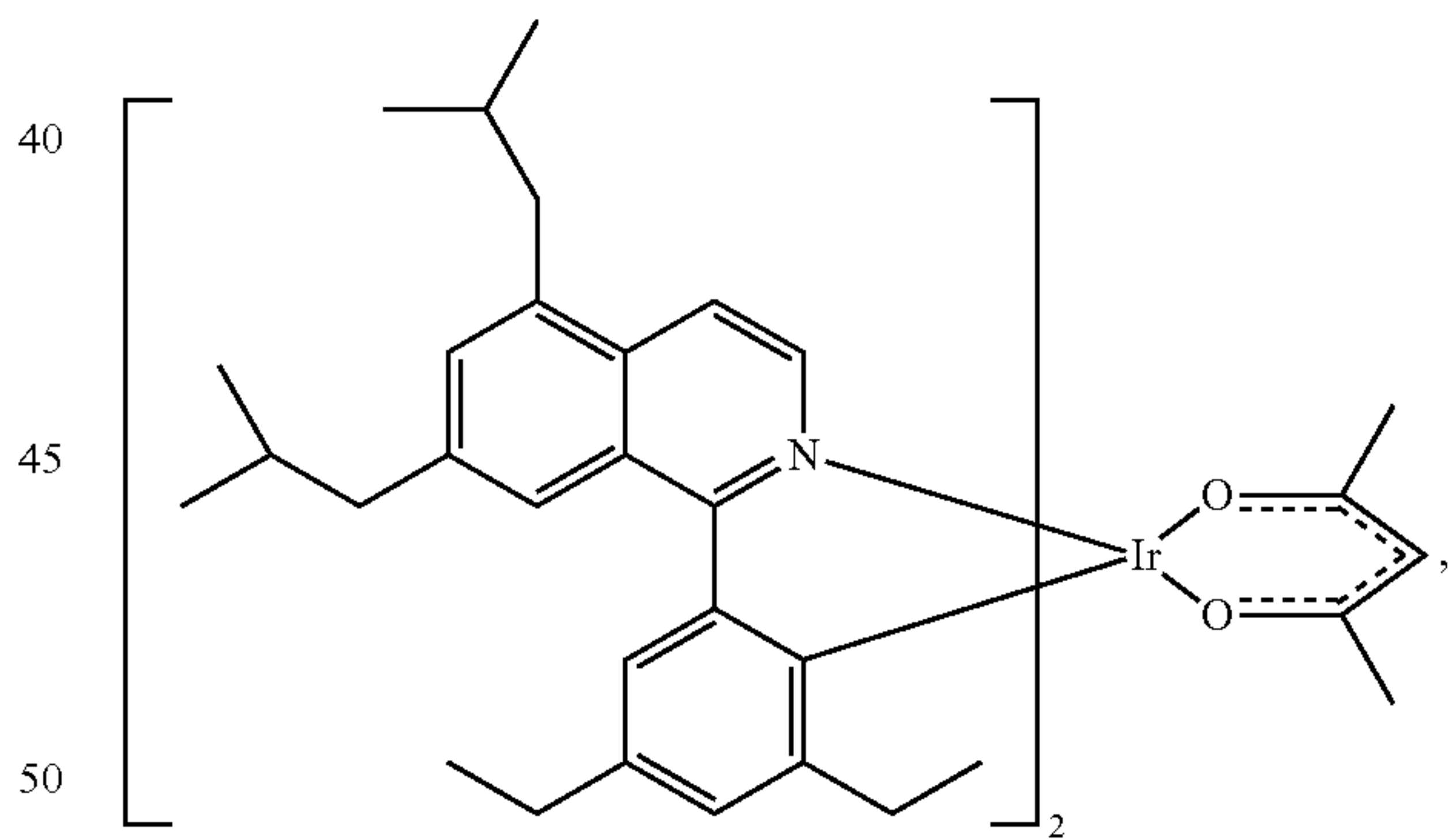
Compound 47
