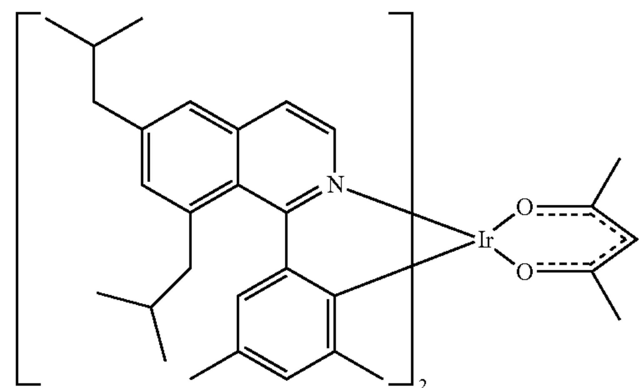
Compound 15
