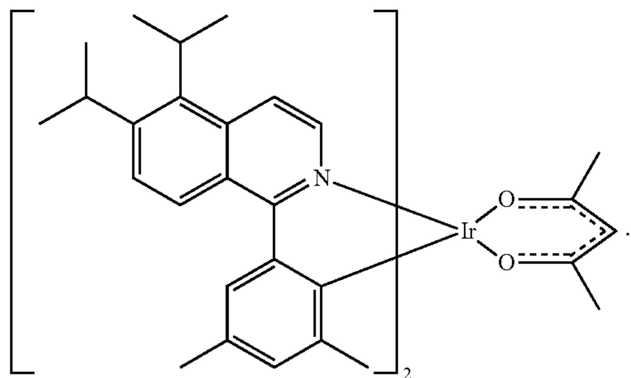
Compound 11
