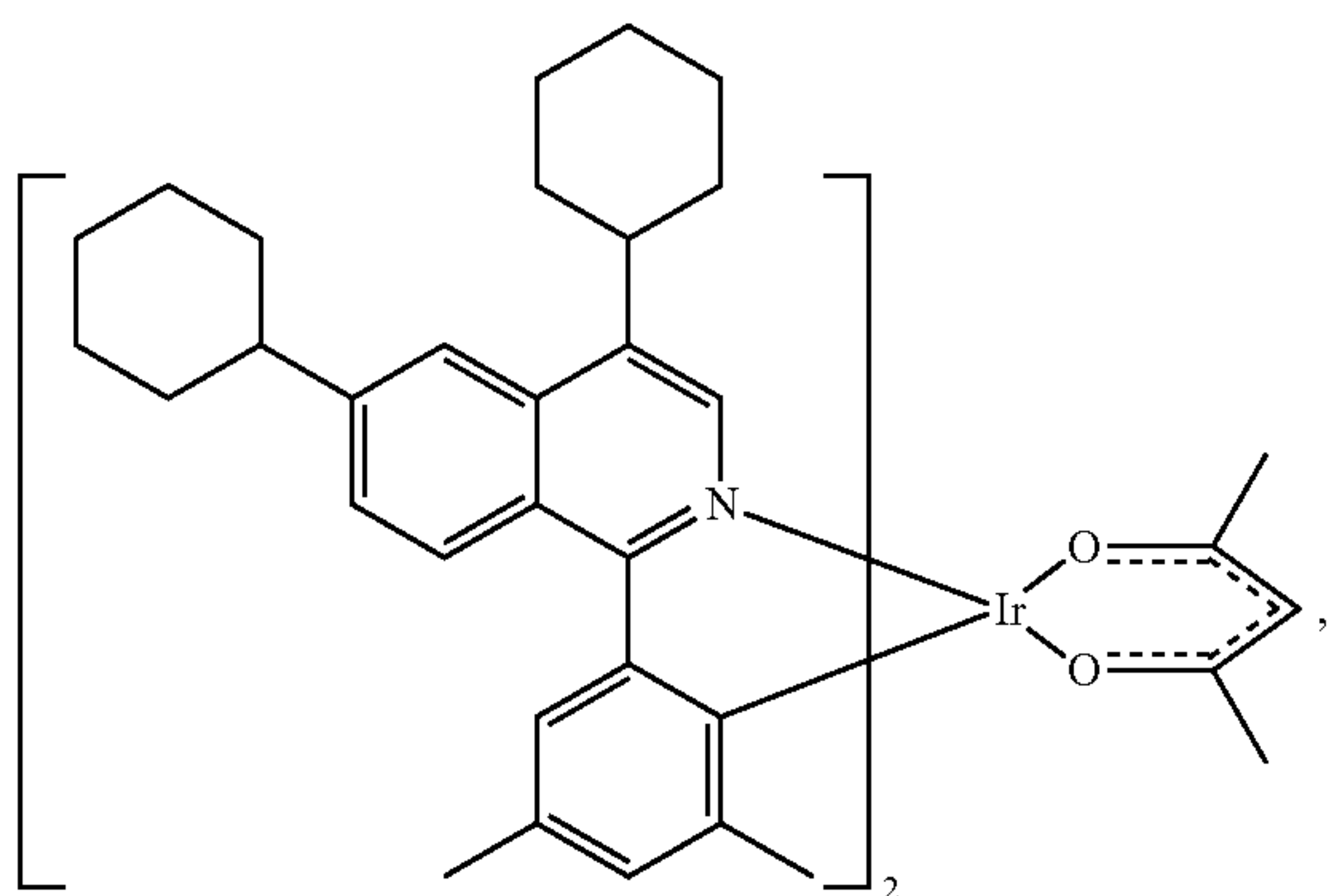
Compound 44
