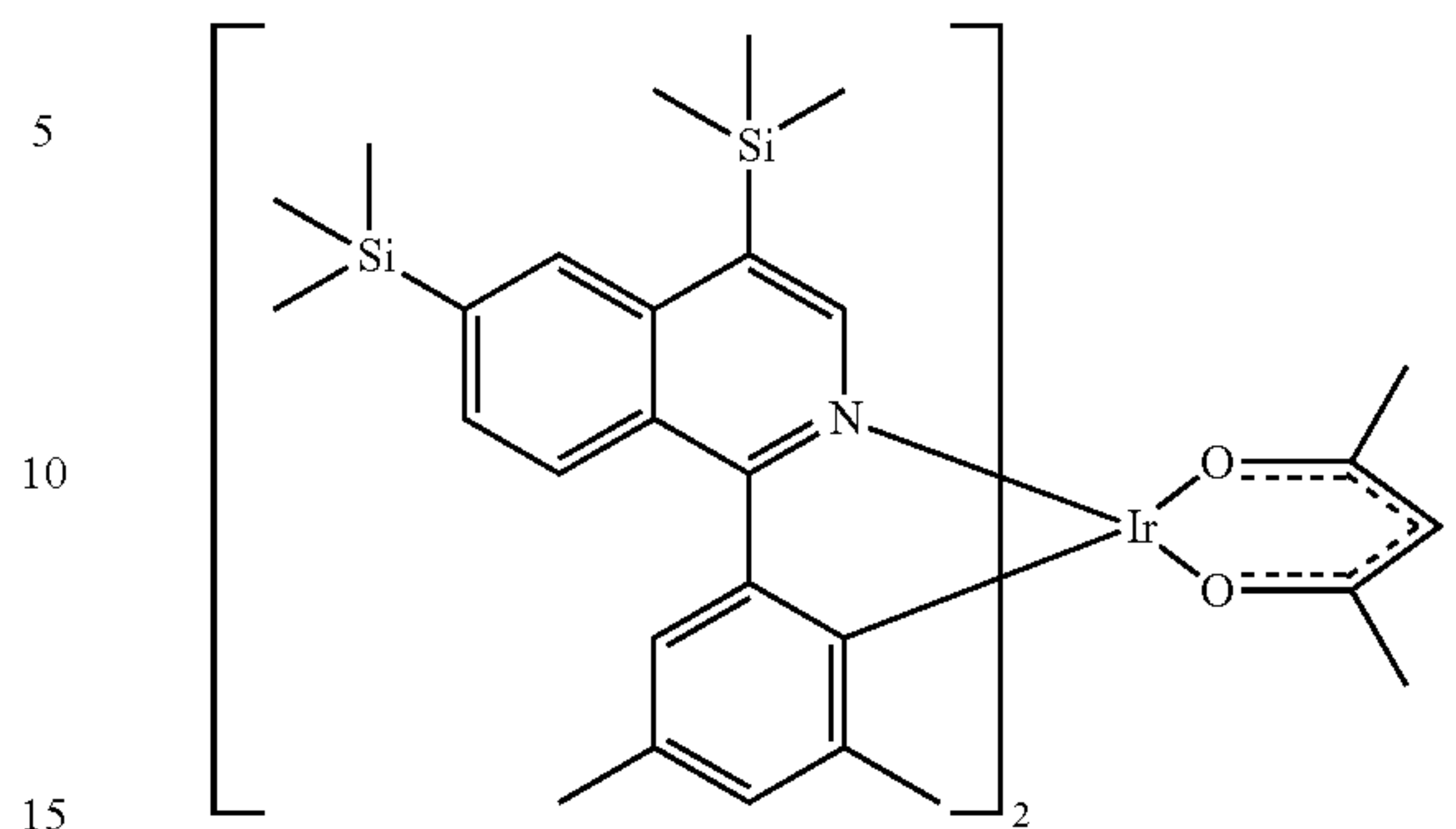
Compound 37
