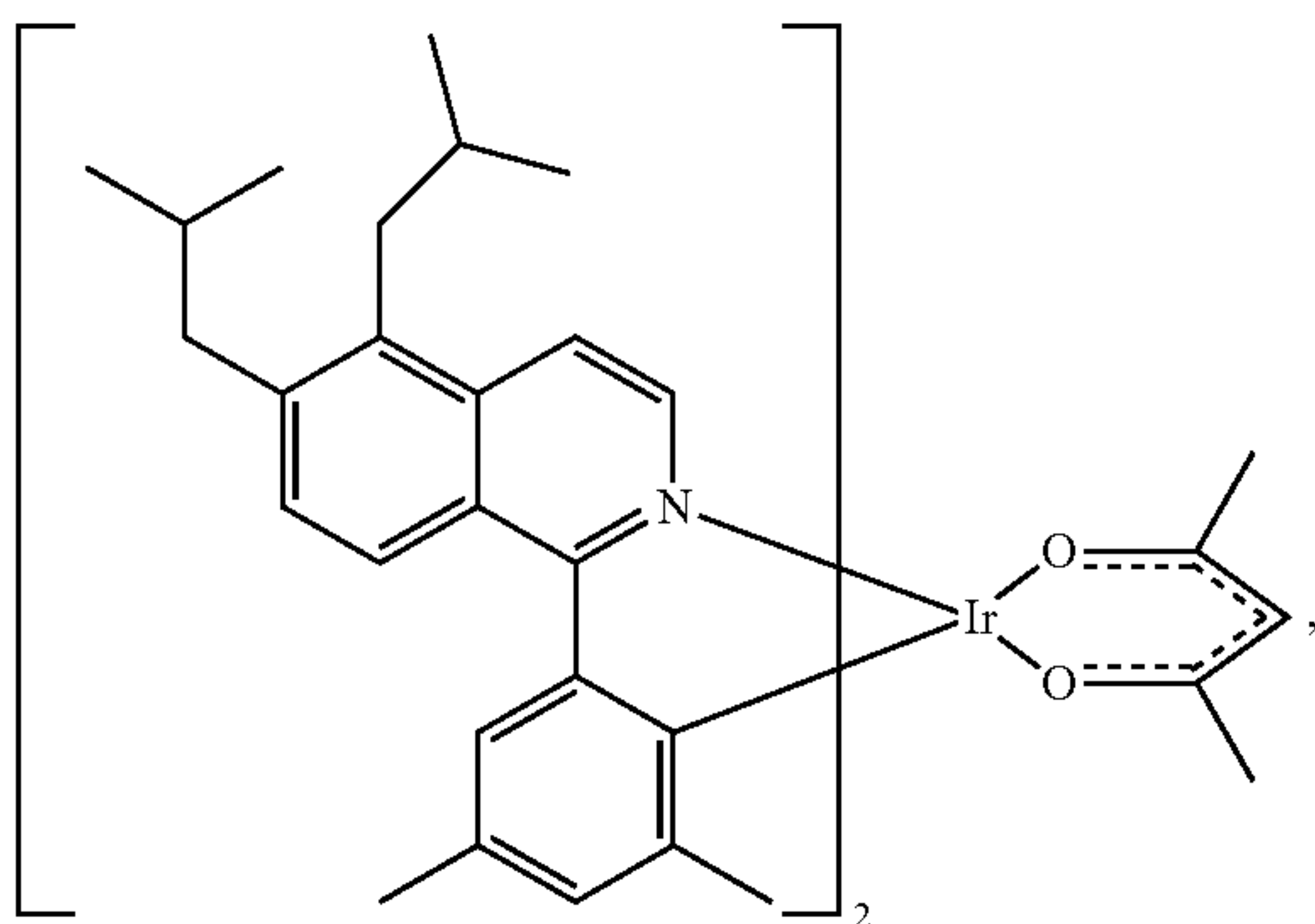
Compound 10
