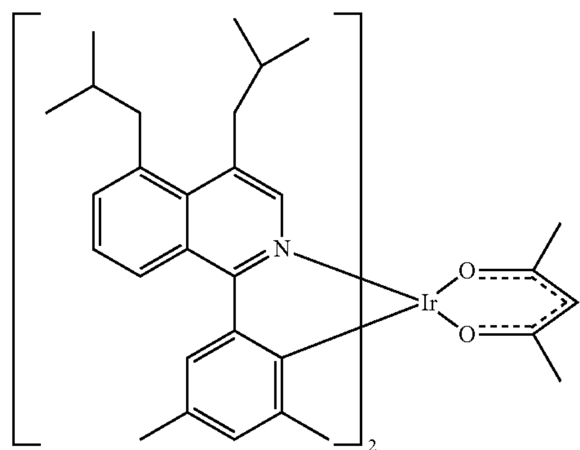
Compound 13
