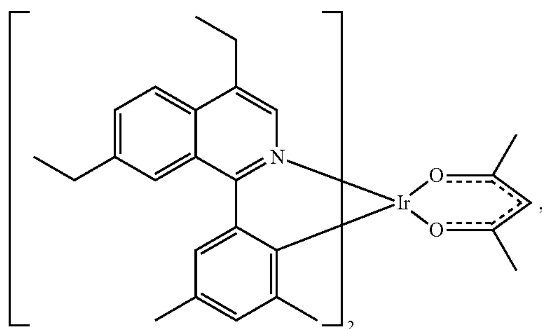
Compound 27
