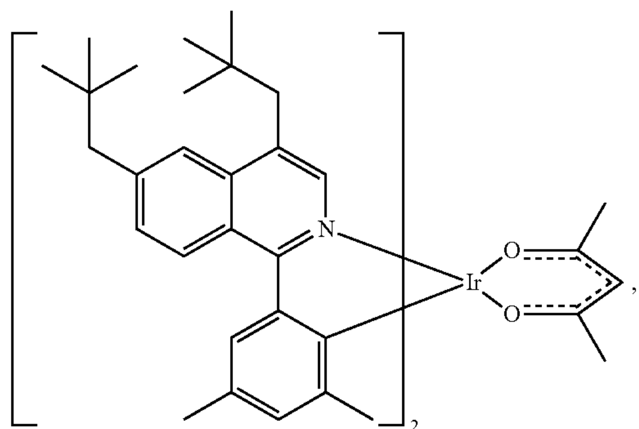
Compound 33
