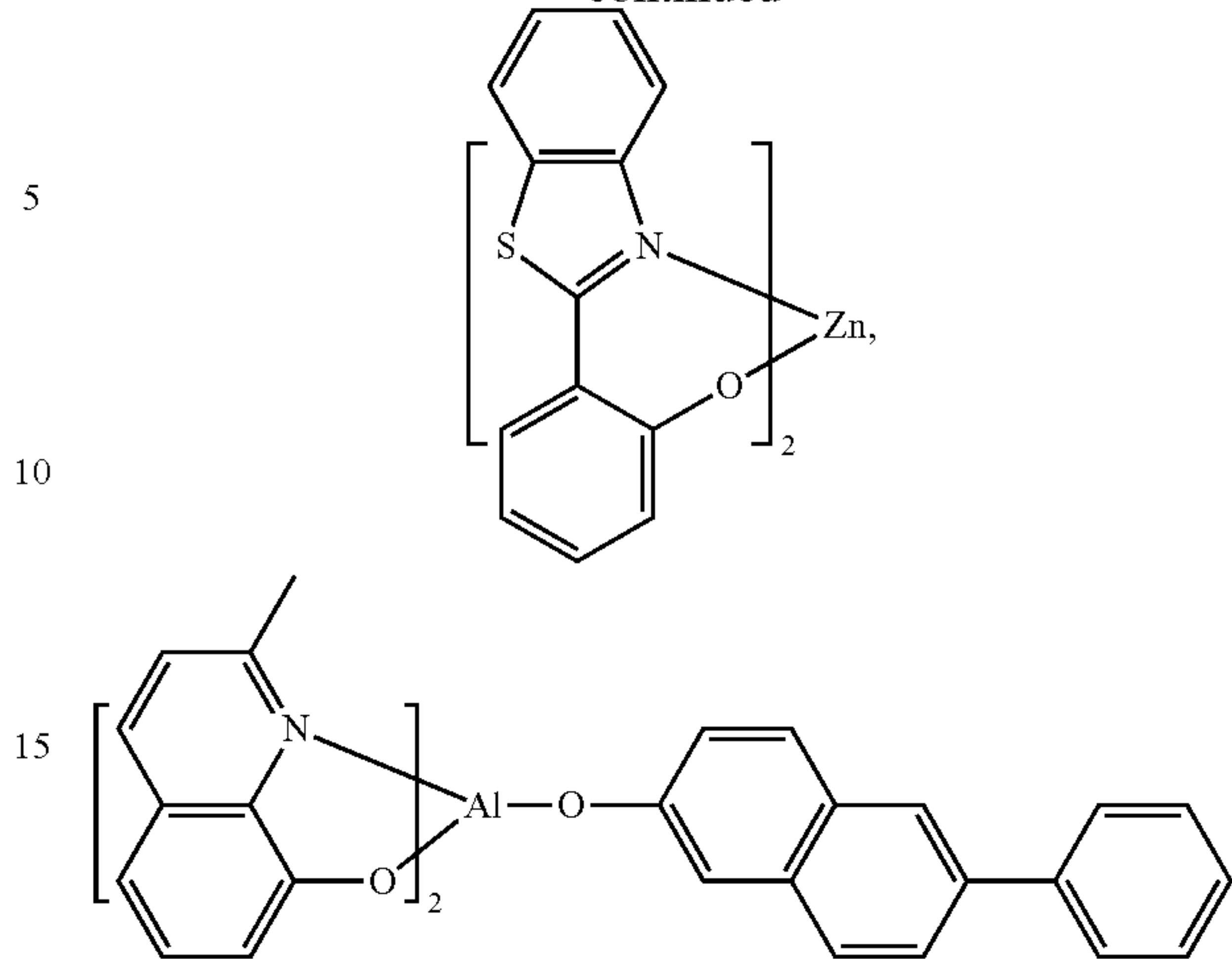
Formula I
