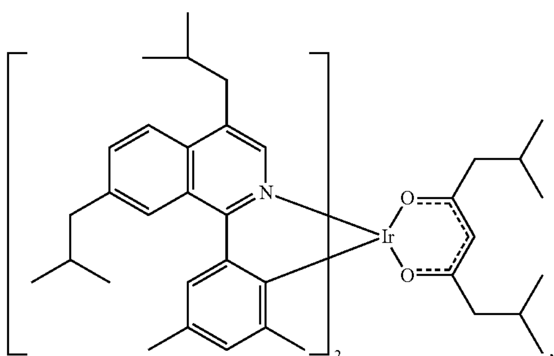
Compound 26
