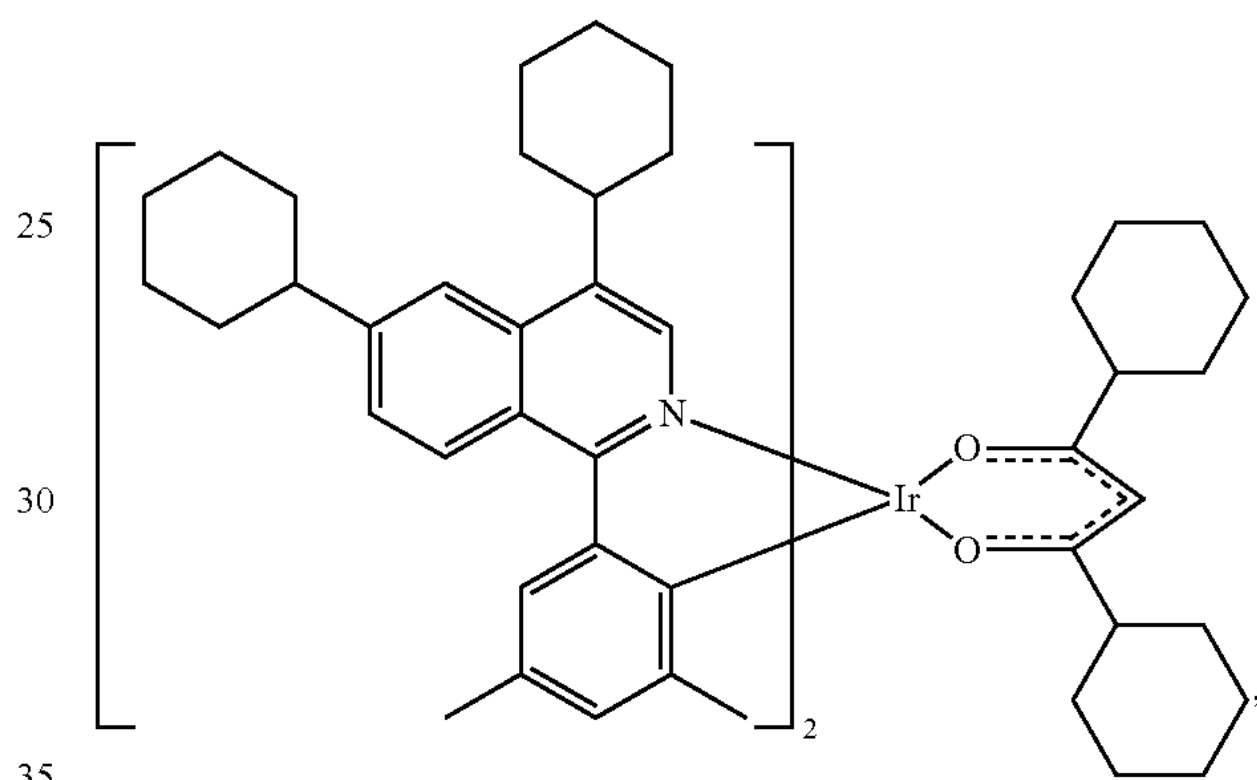
Compound 46
