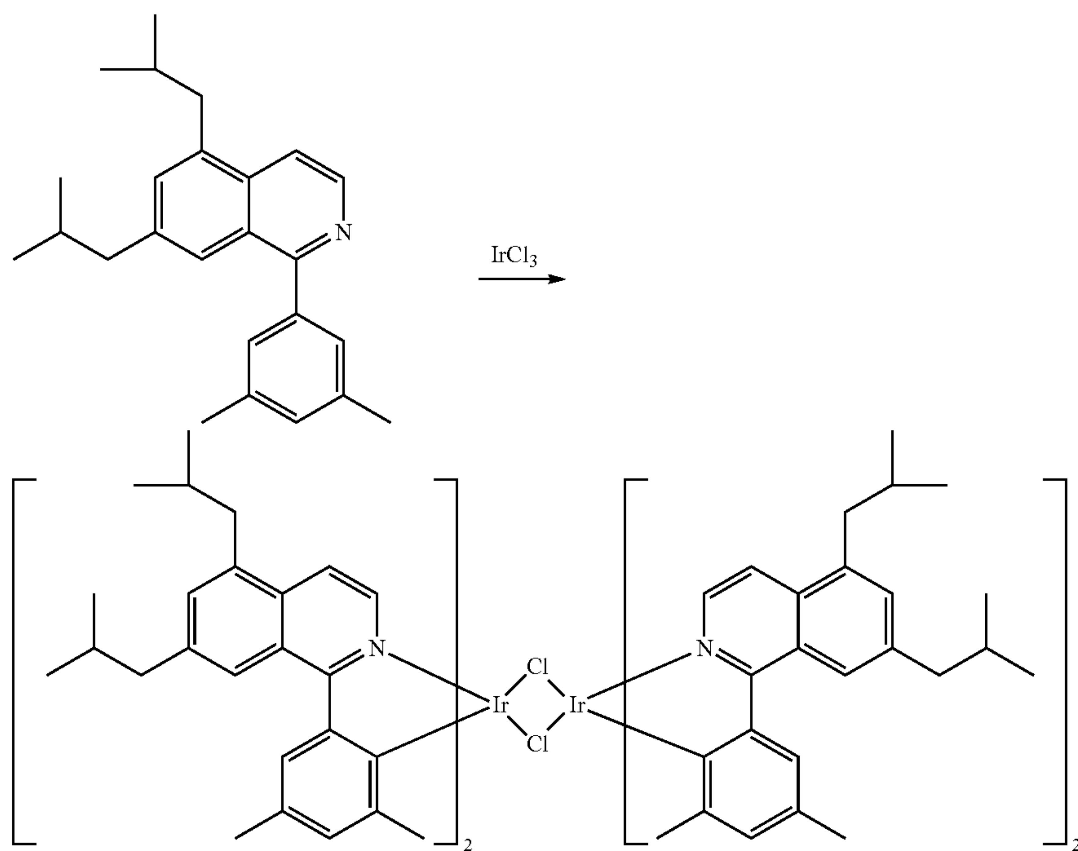
Synthesis of Iridium Dimer
