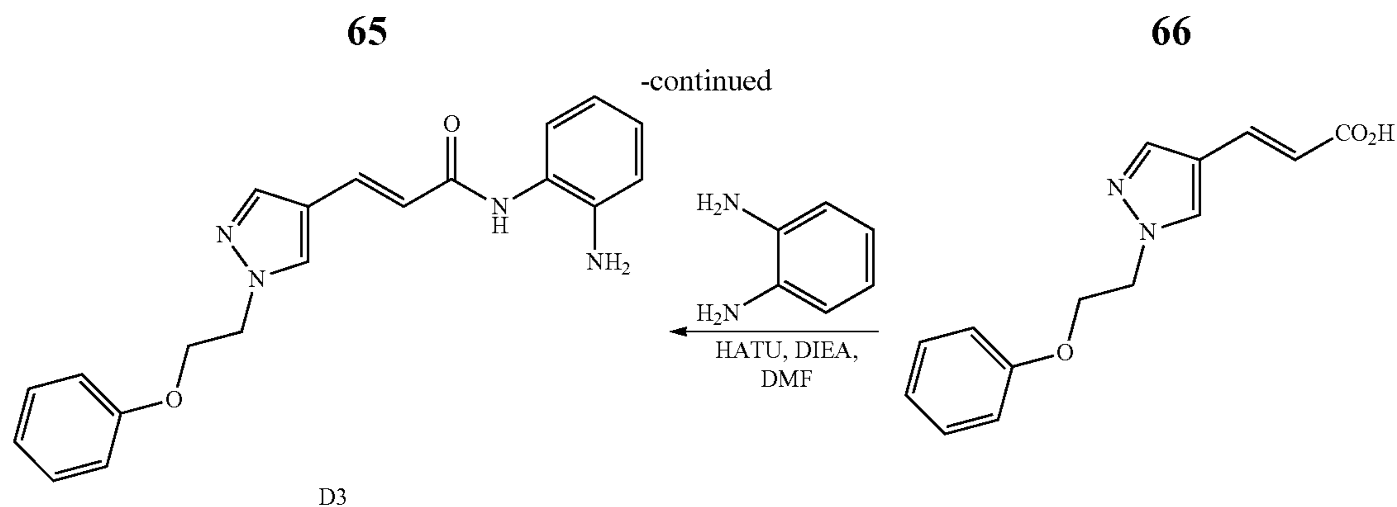
(E)-ethyl 3-(1-(2-phenoxyethyl)-1H-pyrazol-4-yl)acrylate
