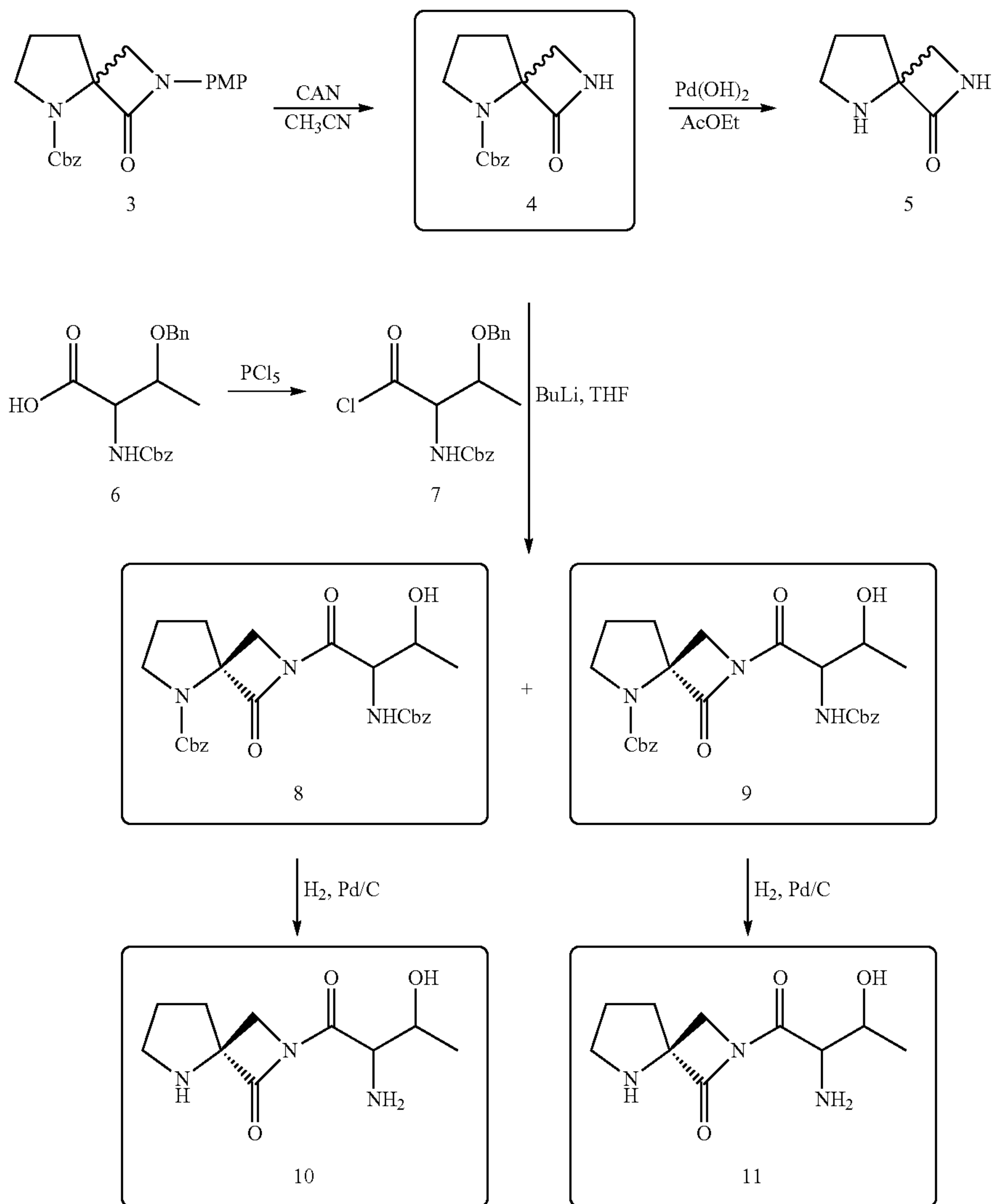
Scheme 1: Preparation of Compounds
