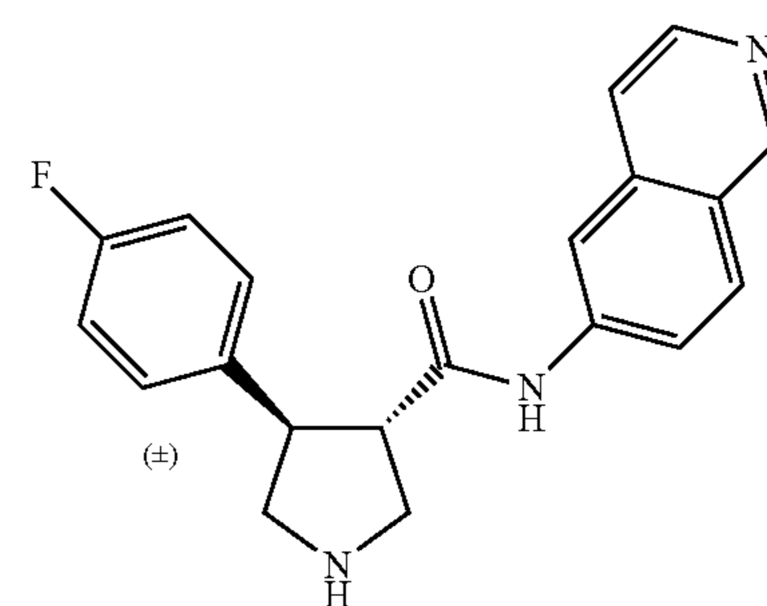
(trans)-4-(4-fluorophenyl)-N-(isoquinolin-6-yl)pyrrolidine-3-carboxamide
