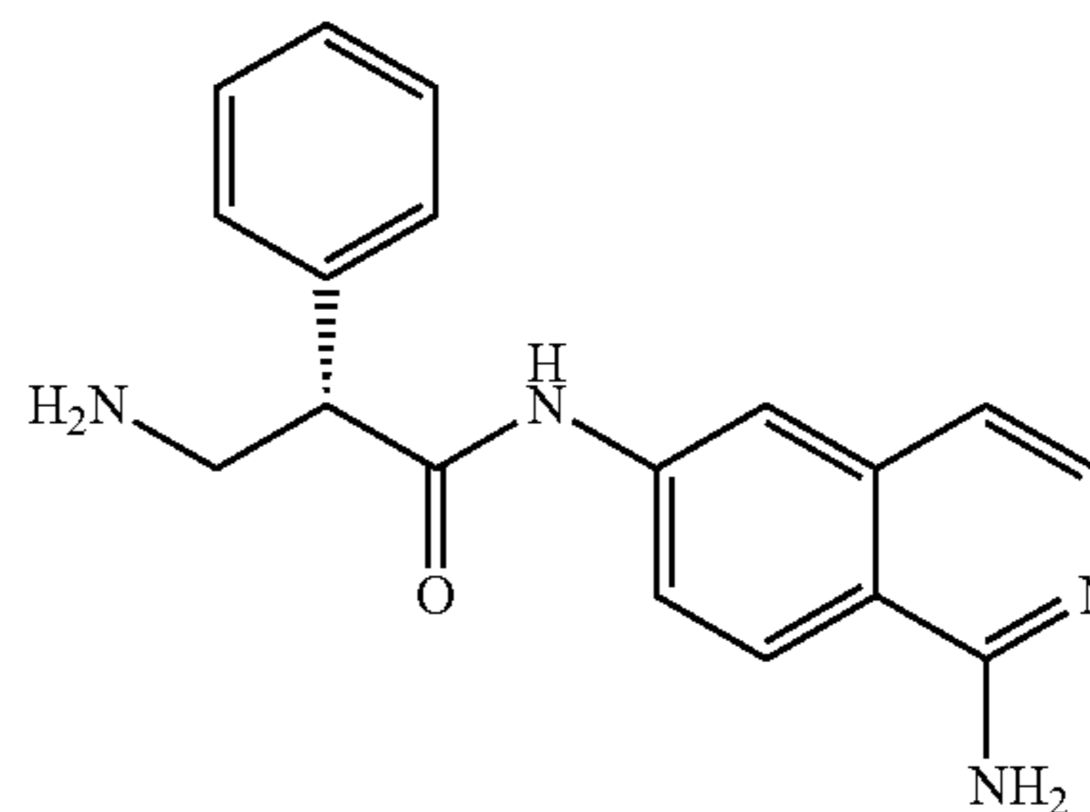
(S)-3-amino-N-(1-aminoisoquinolin-6-yl)-2-phenylpropanamide
