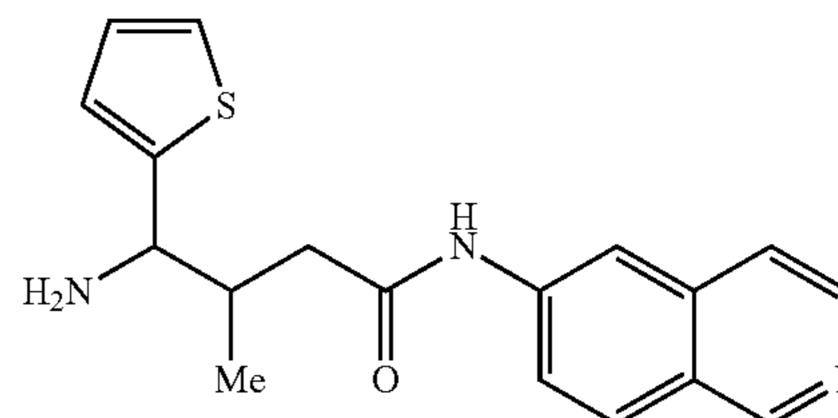
4-amino-N-(isoquinolin-6-yl)-3-methyl-4-(thiopen-2-yl)butanamide
