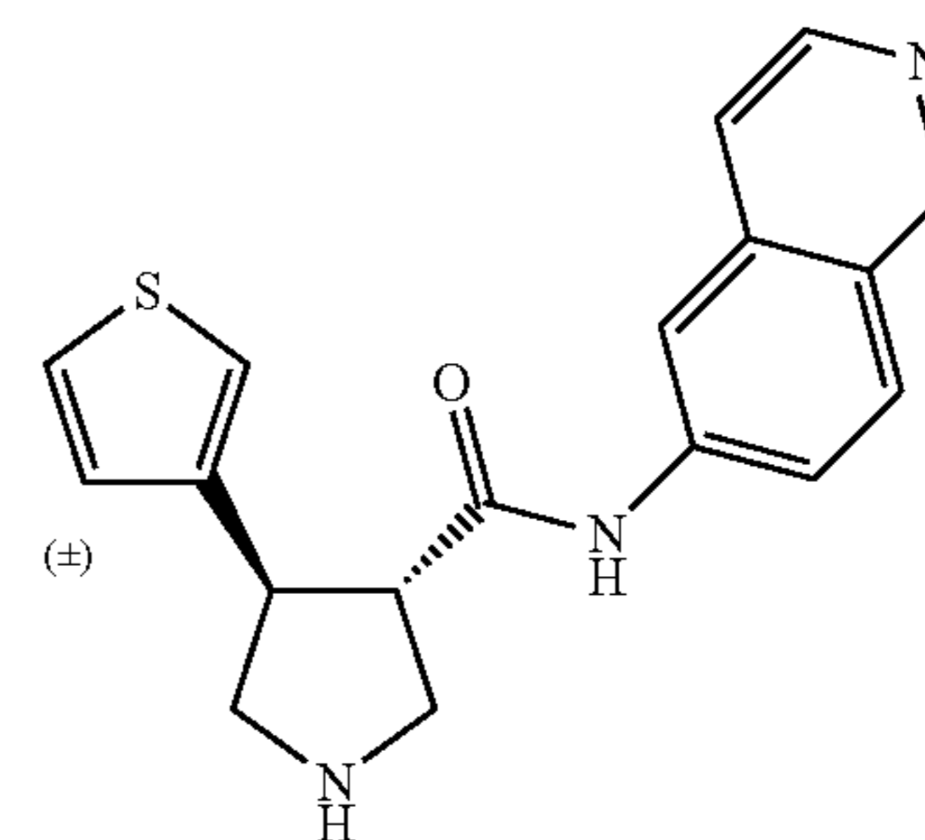
(trans)-N-(isoquinolin-6-yl)-4-(thiophen-3-yl)pyrrolidine-3-carboxamide
