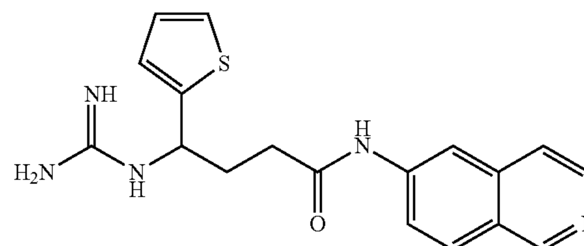
4-guanidino-N-(isoquinolin-6-yl)-4-(thiopen-2-yl)butanamide
