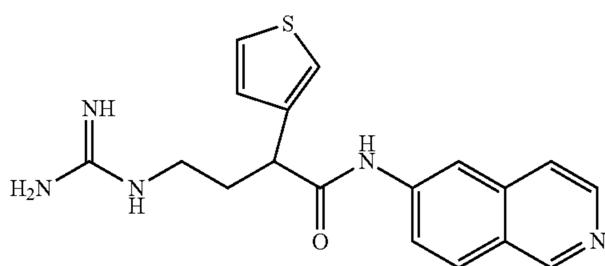
4-guanidino-N-(isoquinolin-6-yl)-2-(thiophen-3-yl)butanamide
