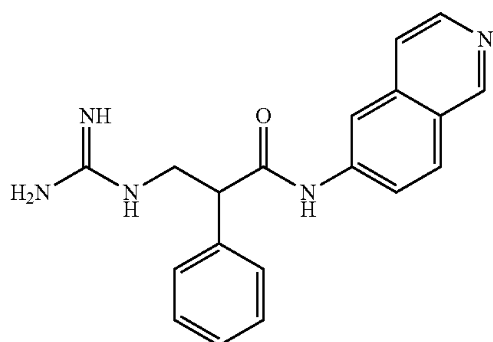
3-guanidino-N-(isoquinolin-6-yl)-2-phenylpropanamide
