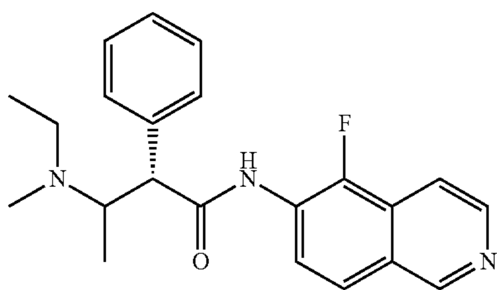
(2S)-3-(ethyl(methyl)amino)-N-(5-fluoroisoquinolin-6-yl)-2-phenylbutanamide
