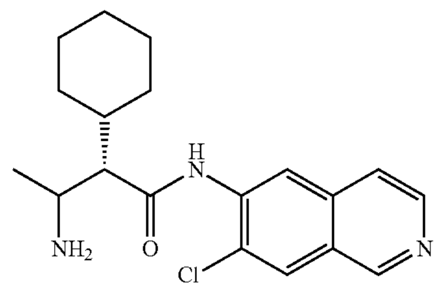
(2S)-3-amino-N-(7-chloroisoquinolin-6-yl)-2-cyclohexylbutanamide
