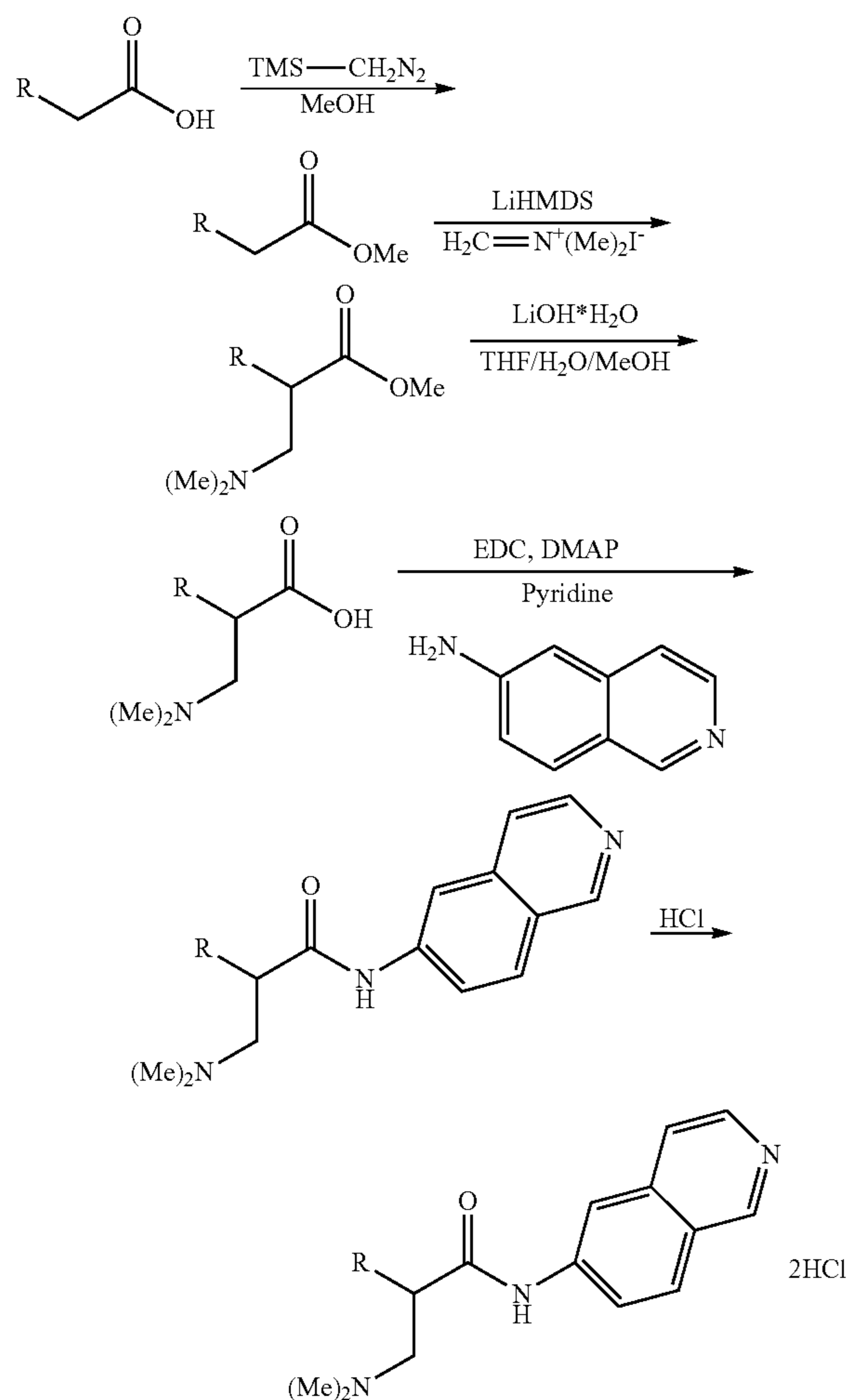
Scheme 4 Scheme 4.
