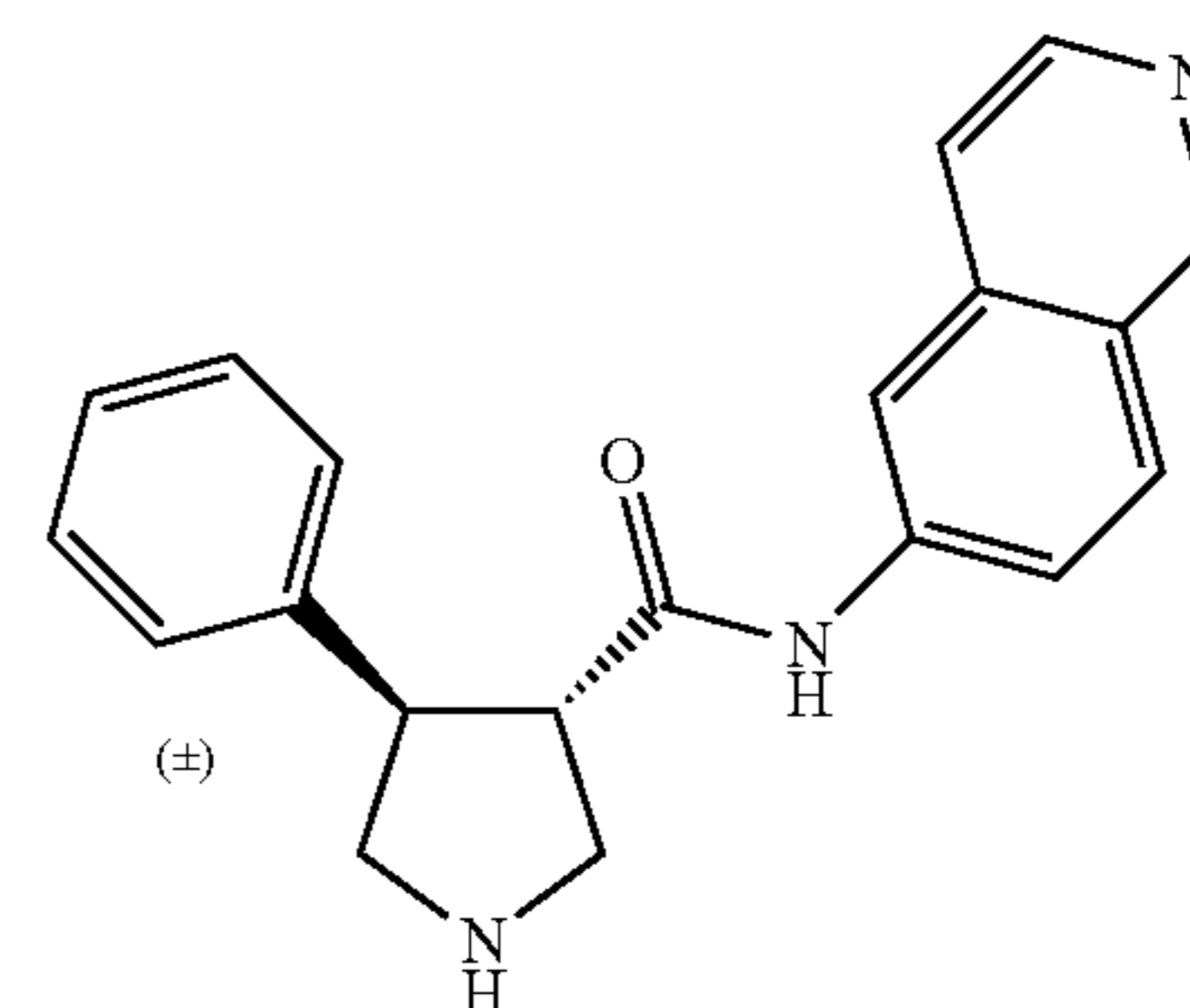
(trans)-N-(isoquinolin-6-yl)-4-phenylpyrrolidine-3-carboxamide
