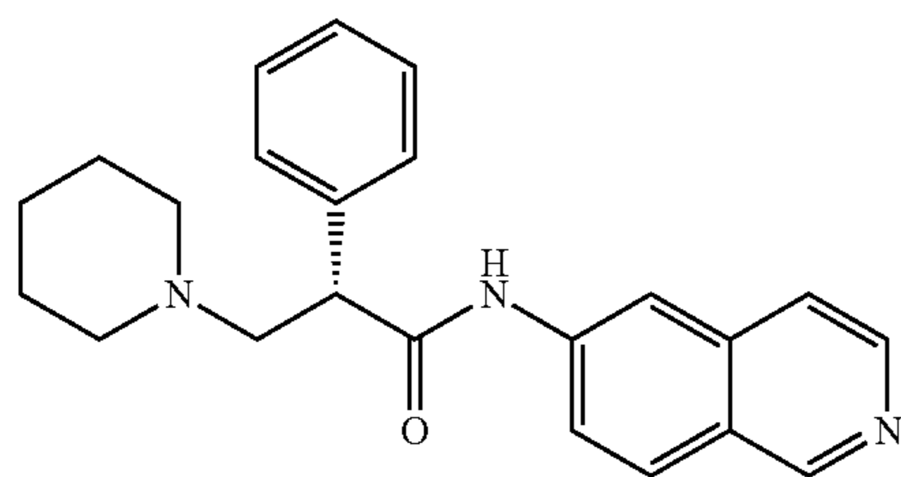
(S)-N-(isoquinolin-6-yl)-2-phenyl-3-(piperidin-1-yl)propanamide
