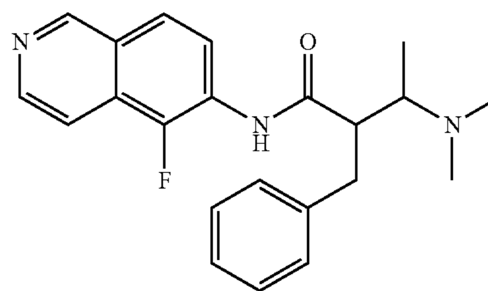
2-benzyl-3-(dimethylamino)-N-(5-fluoroisoquinolin-6-yl)butanamide
