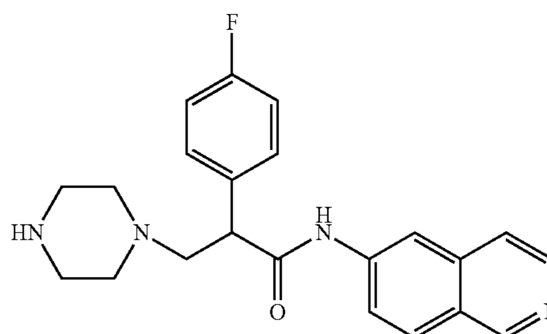
2-(4-fluorophenyl)-N-(isoquinolin-6-yl)-3-(piperazin-1-yl)propanamide
