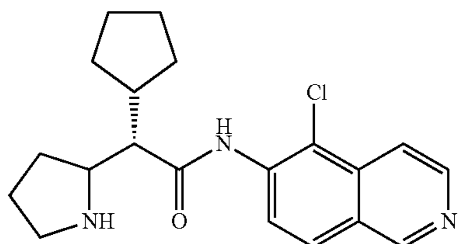
(2S)-N-(5-chloroisoquinolin-6-yl)-2-cyclopentyl-2-(pyrrolidin-2-yl)acetamide
