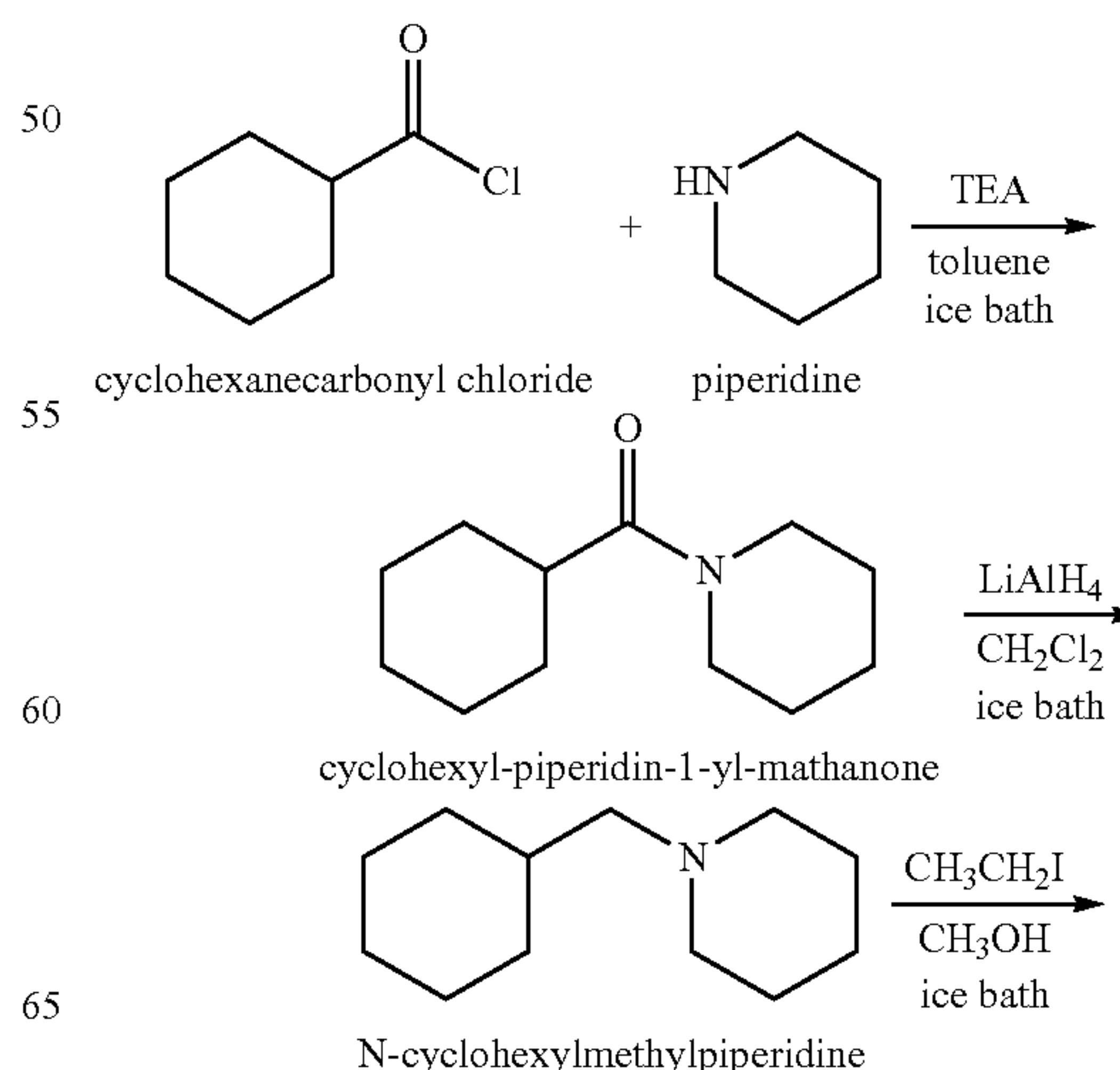
SCHEME 1
