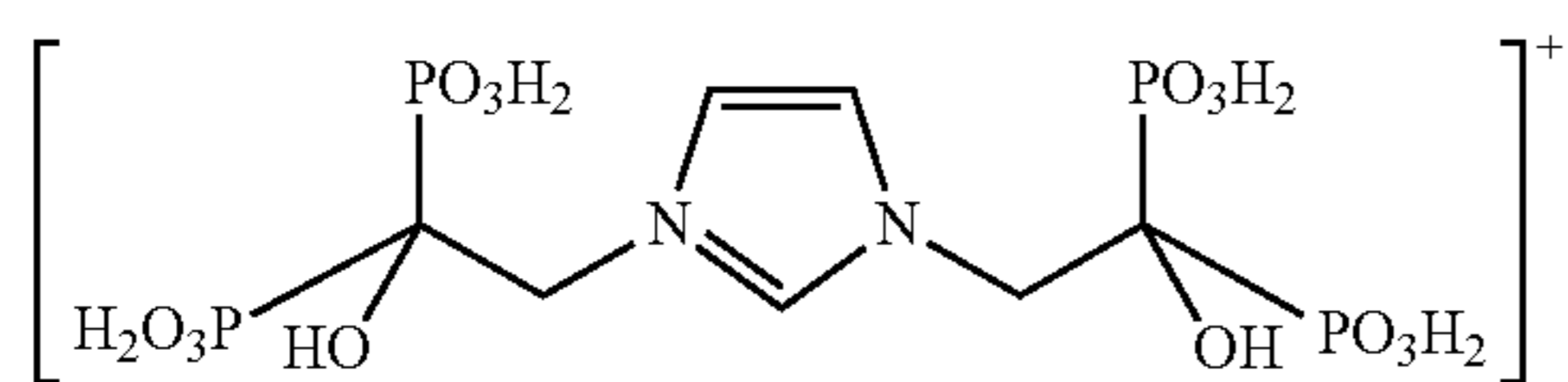
Compound 2
