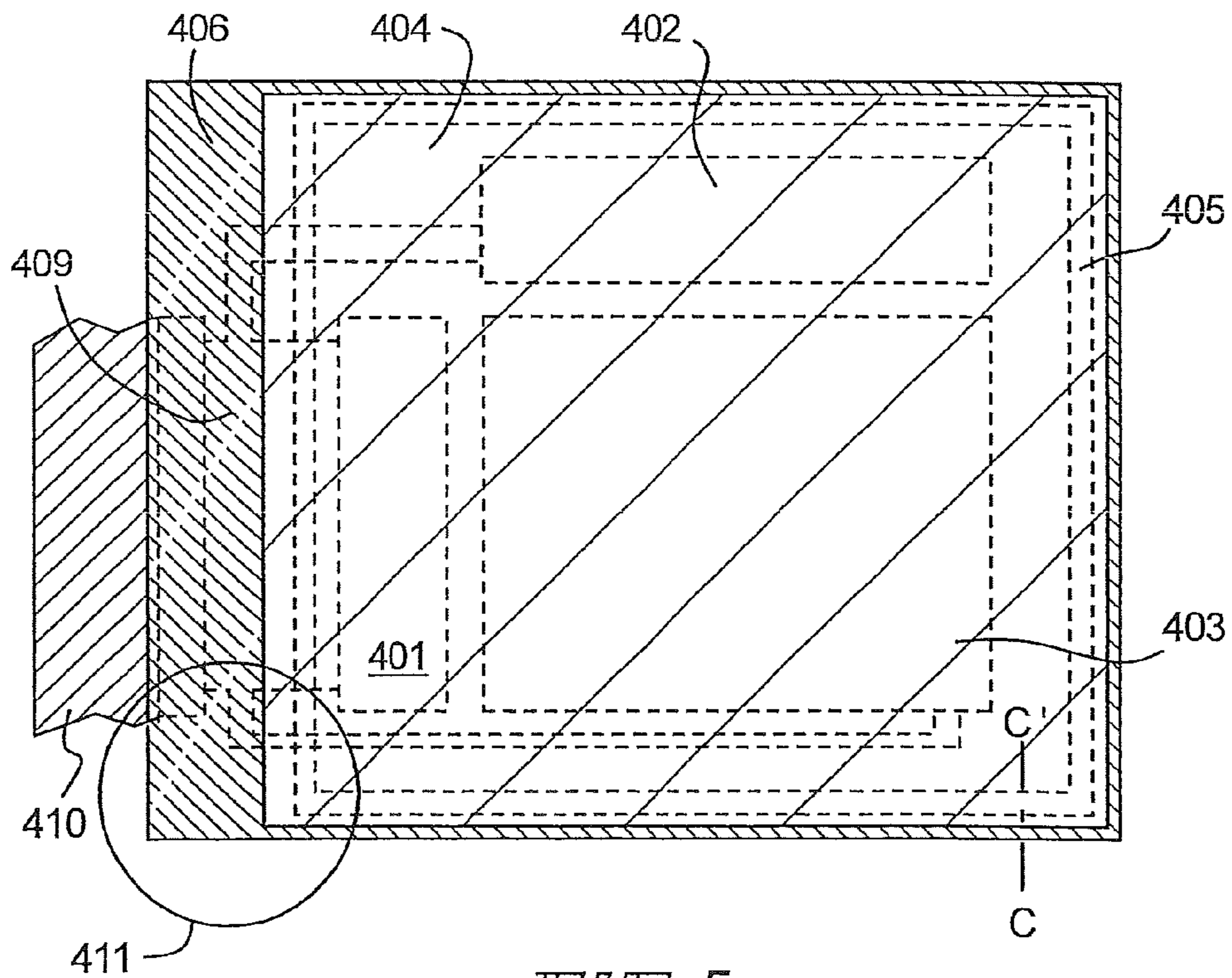
FIG. 5 PRIOR ART
