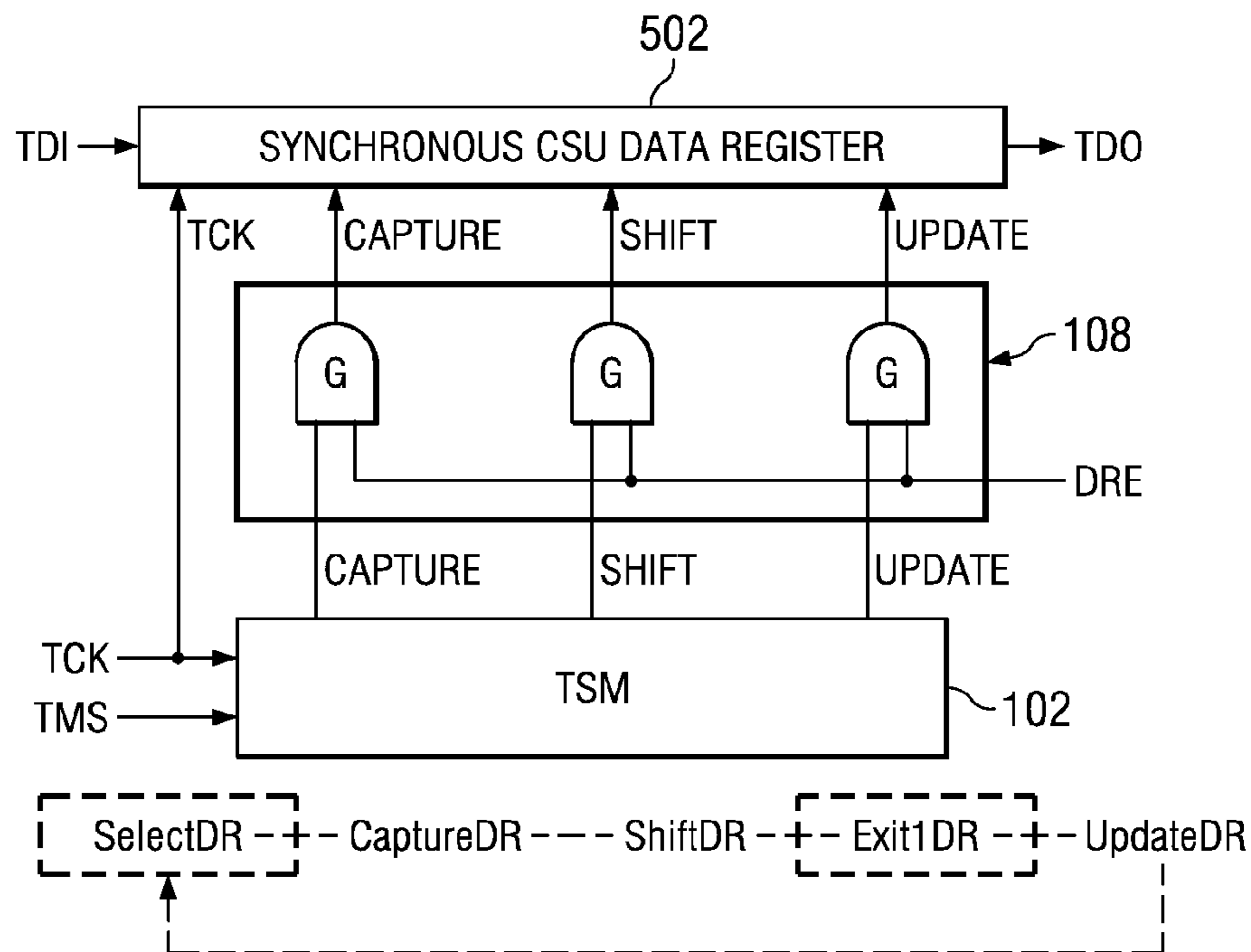
FIG. 5 (PRIOR ART)
