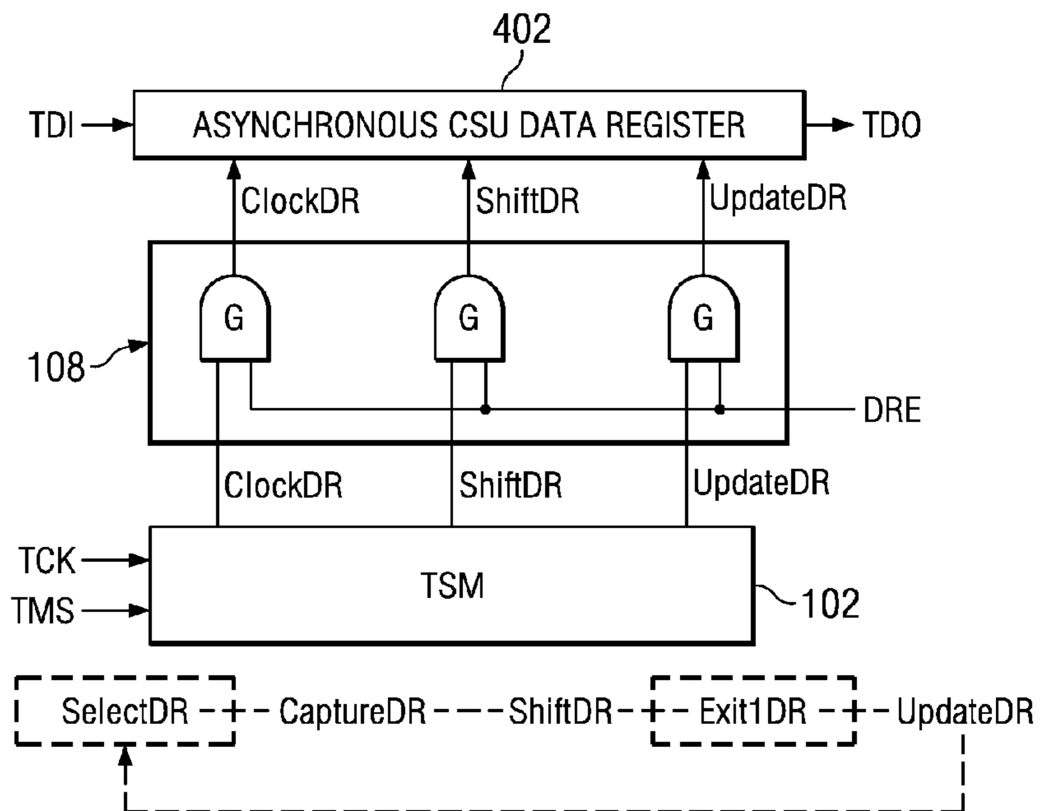
FIG. 4 (PRIOR ART)
