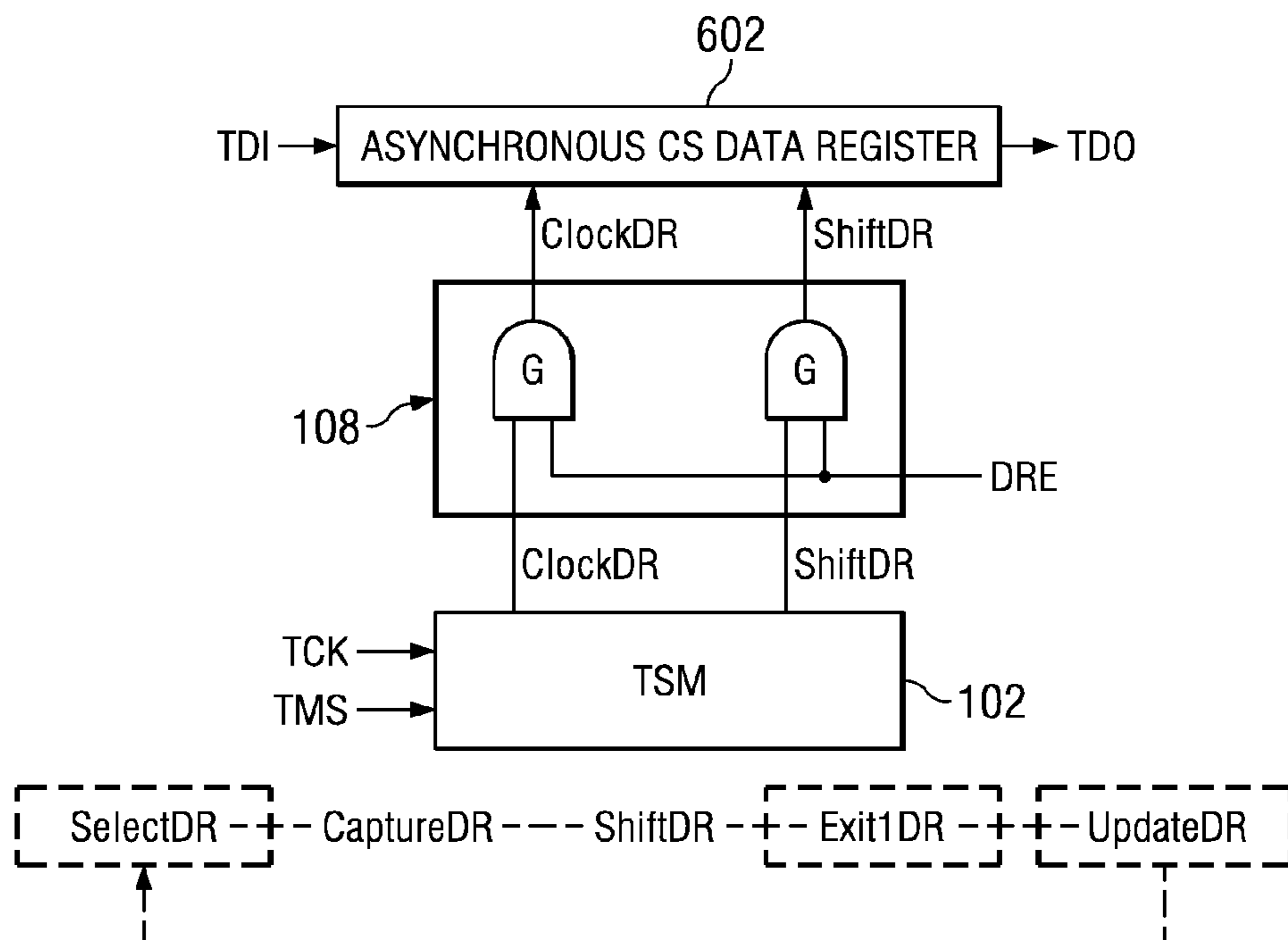
FIG. 6 (PRIOR ART)
