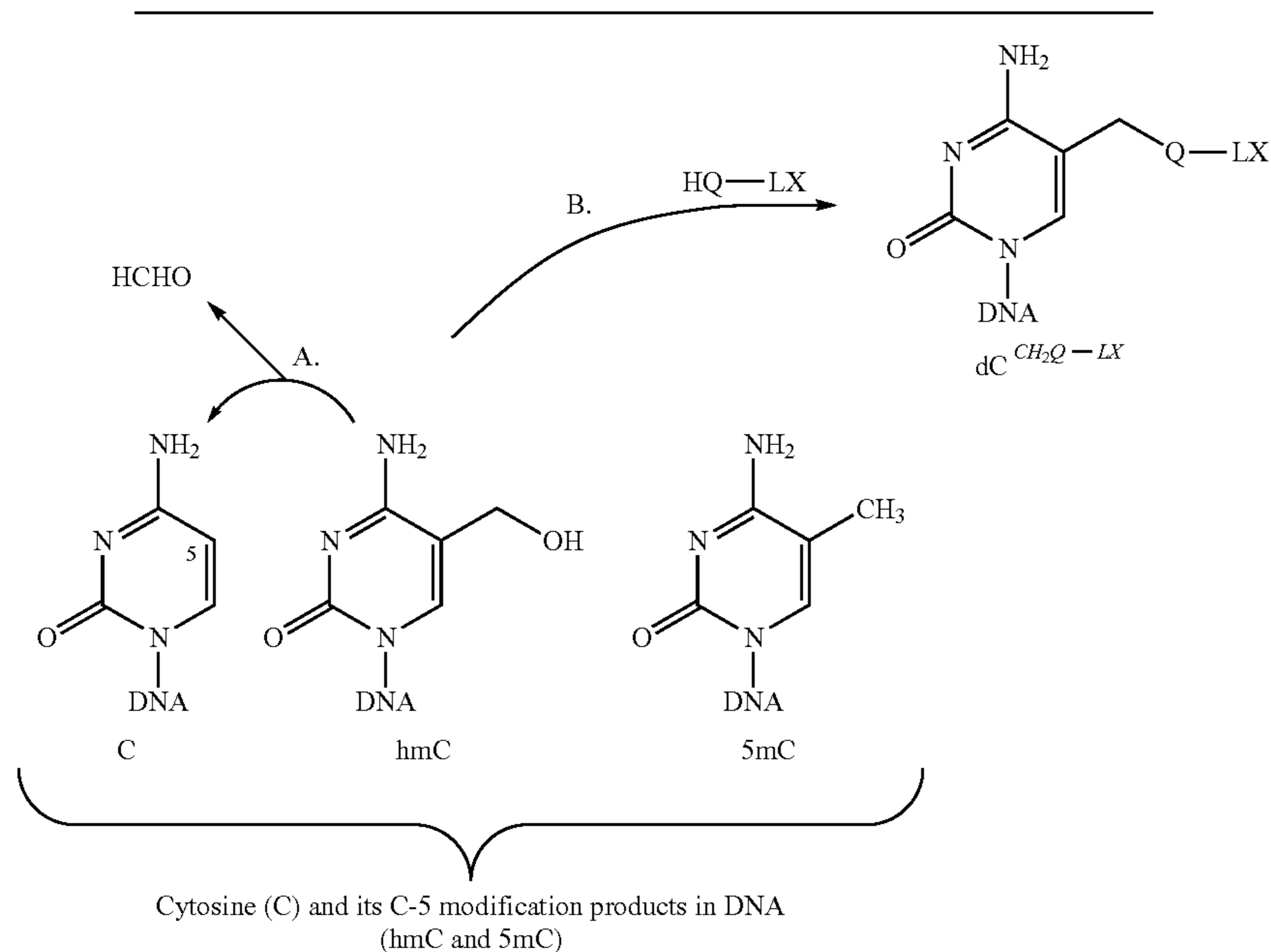
Scheme 3. Sequence specific conversions of natural DNA with DNA methyltransferases according to the present invention for analytical determination of hmC residues. A. conversion of hmC residues to unmodified cytosines; B. derivatization/labeling of hmC residues.
