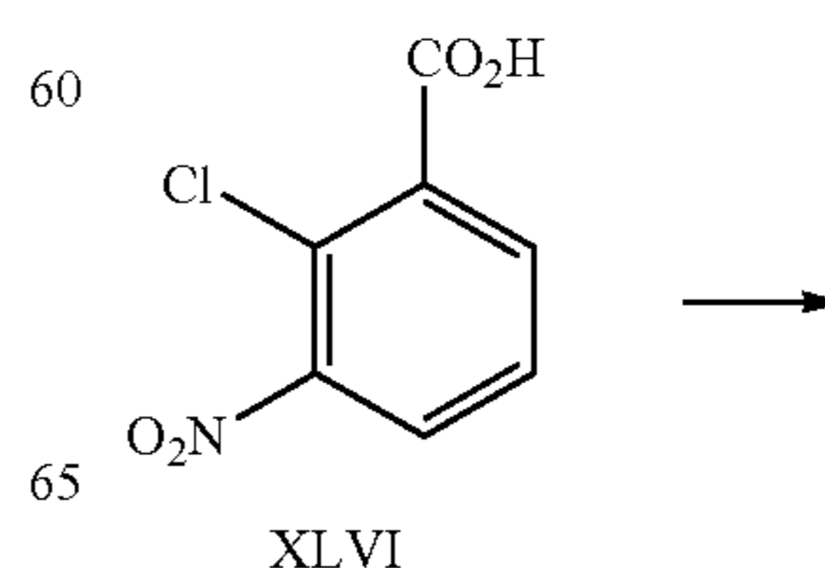
Scheme 13. Synthesis of thioanilines XLIV
