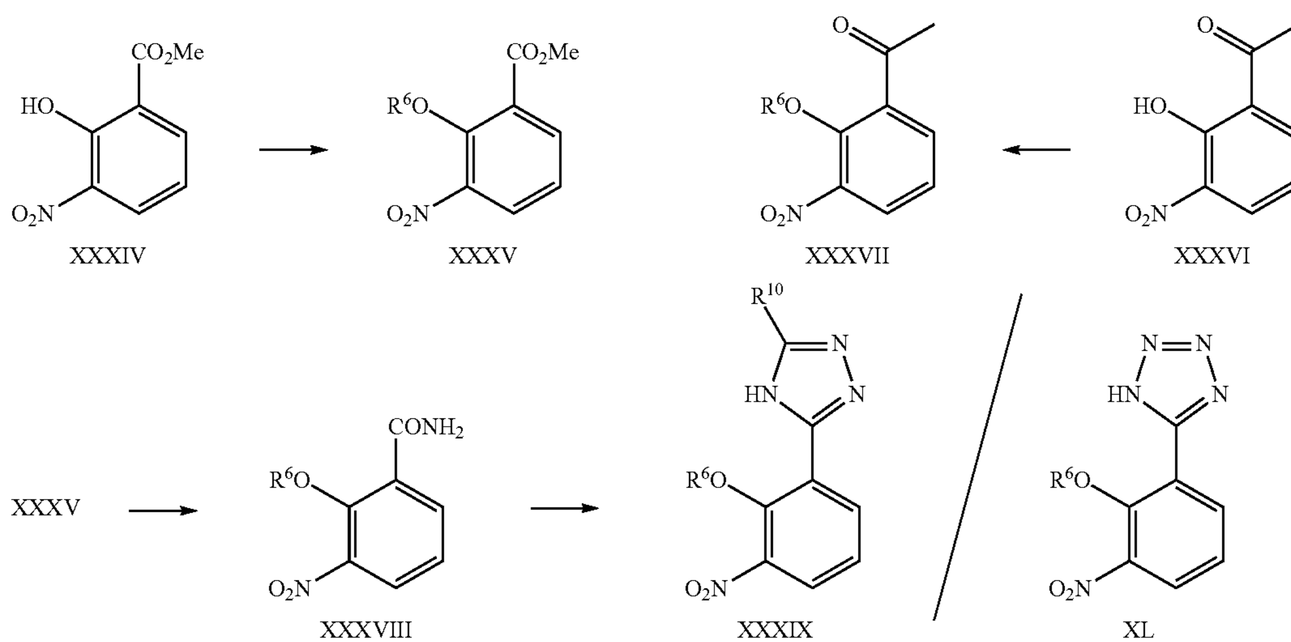
Scheme 12. Alternate synthesis of anilines XII
