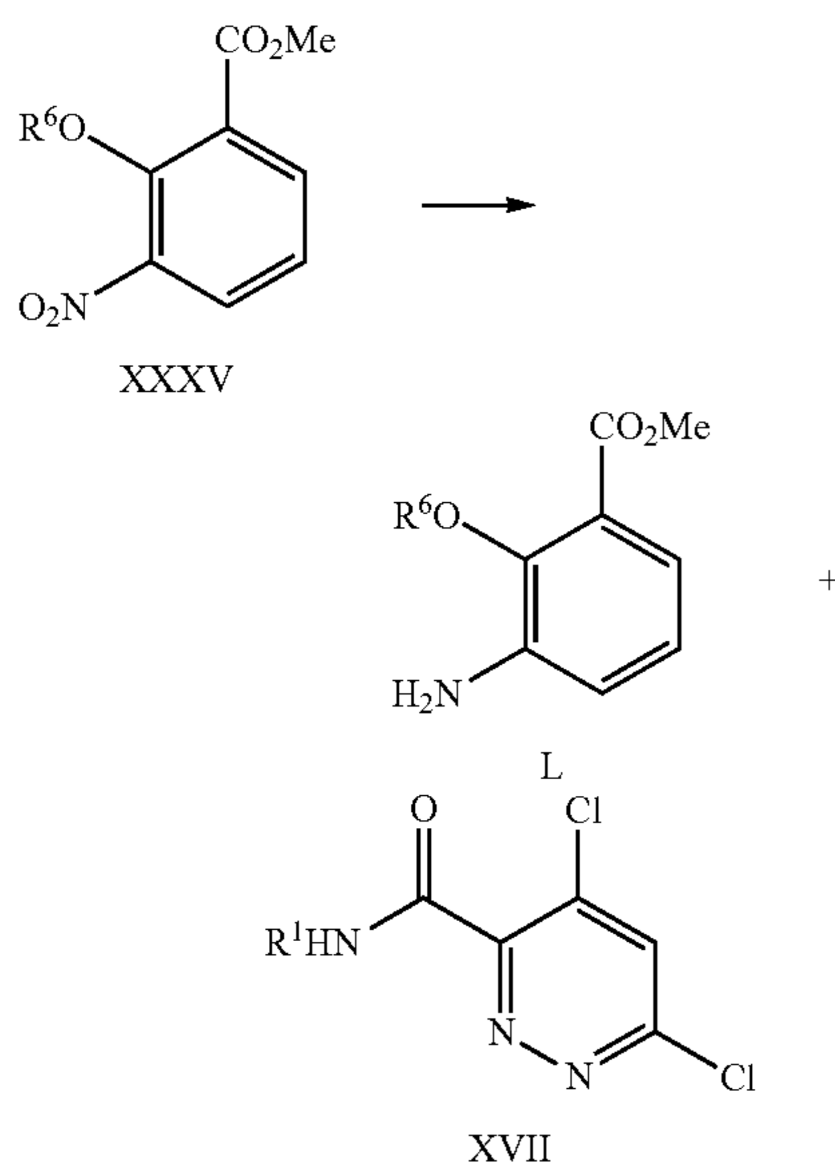
Scheme 14. Synthesis of final compounds LV
