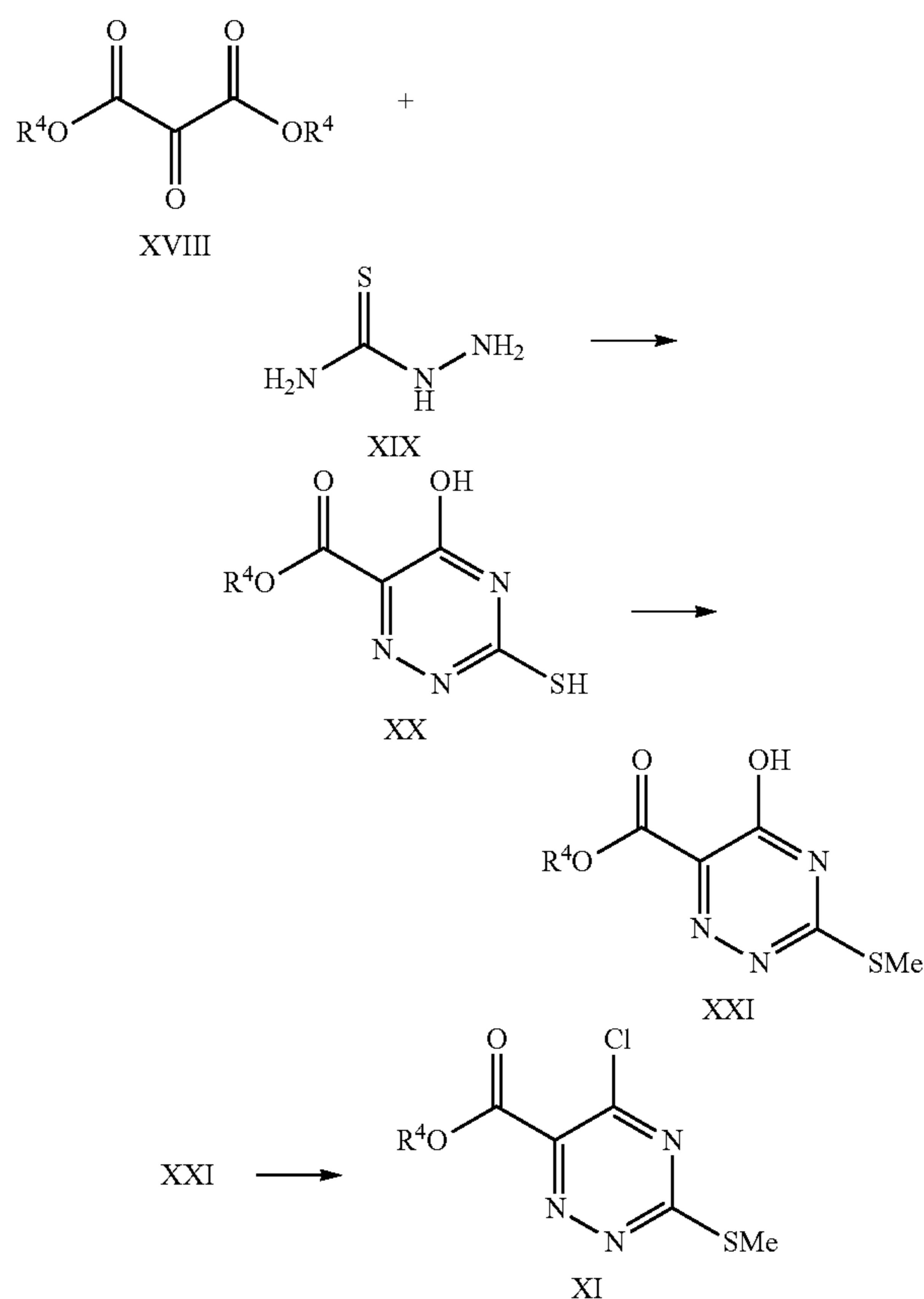
Scheme 8. Preparation of XI
