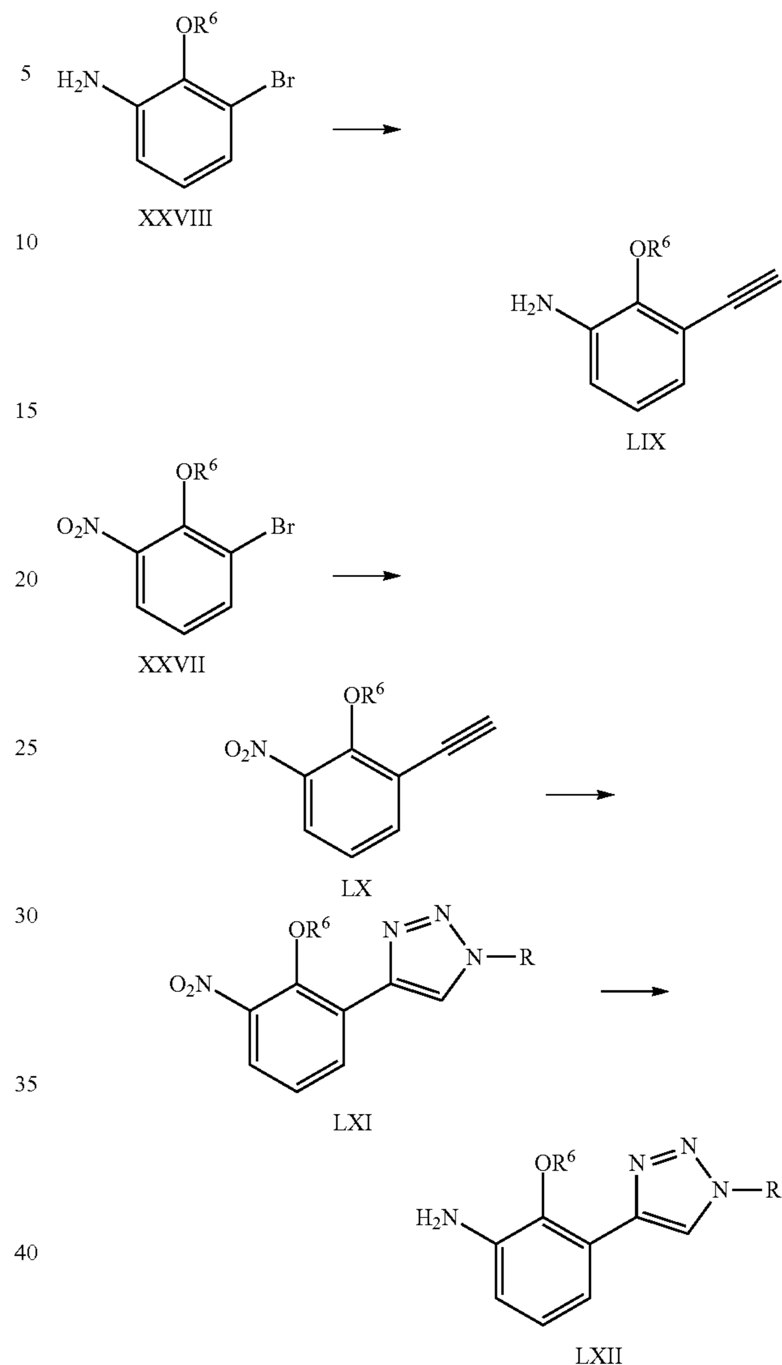
Scheme 16. Synthesis of anilines LIX and LXII (variants of XII)
