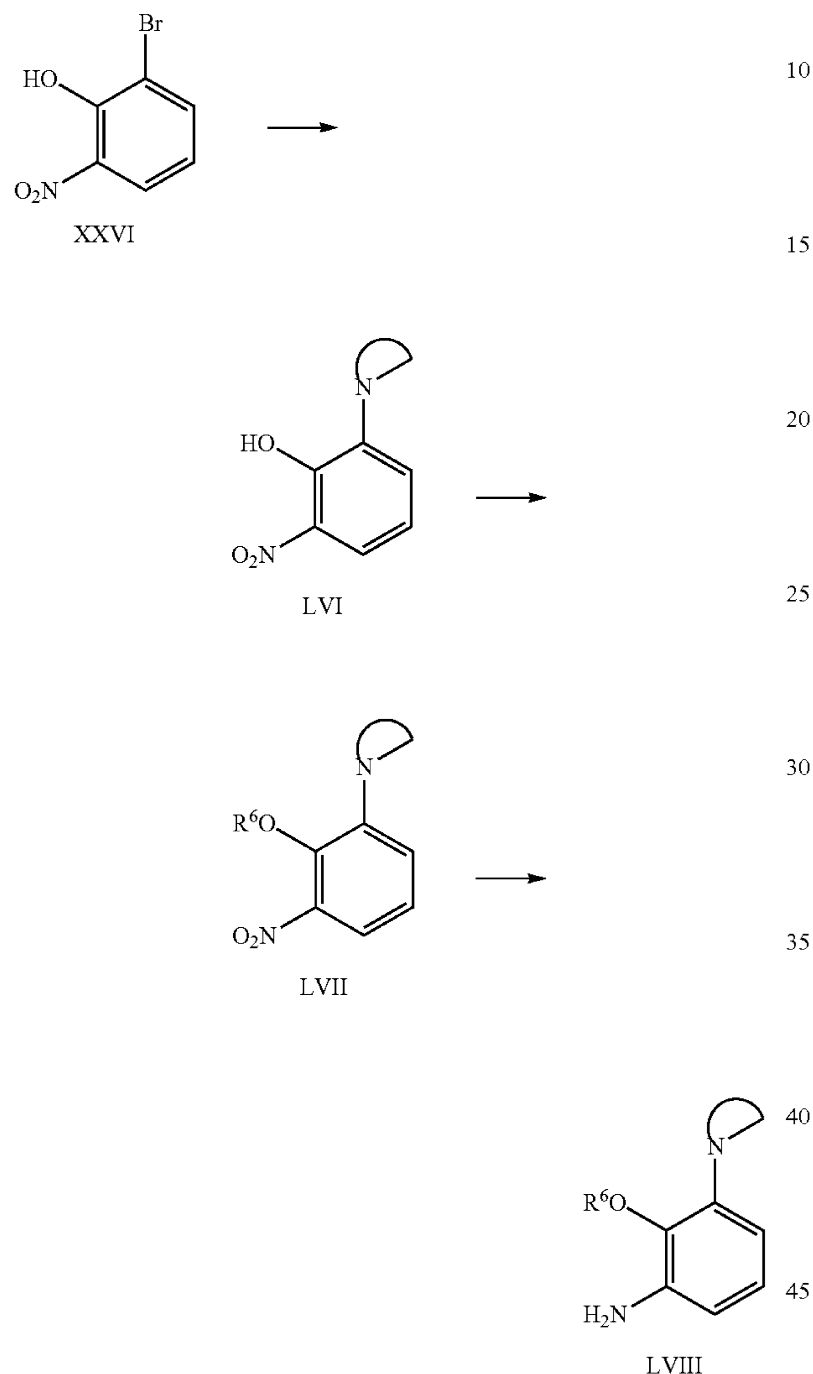
Scheme 15. Synthesis of anilines LVIII (variant of XII)
