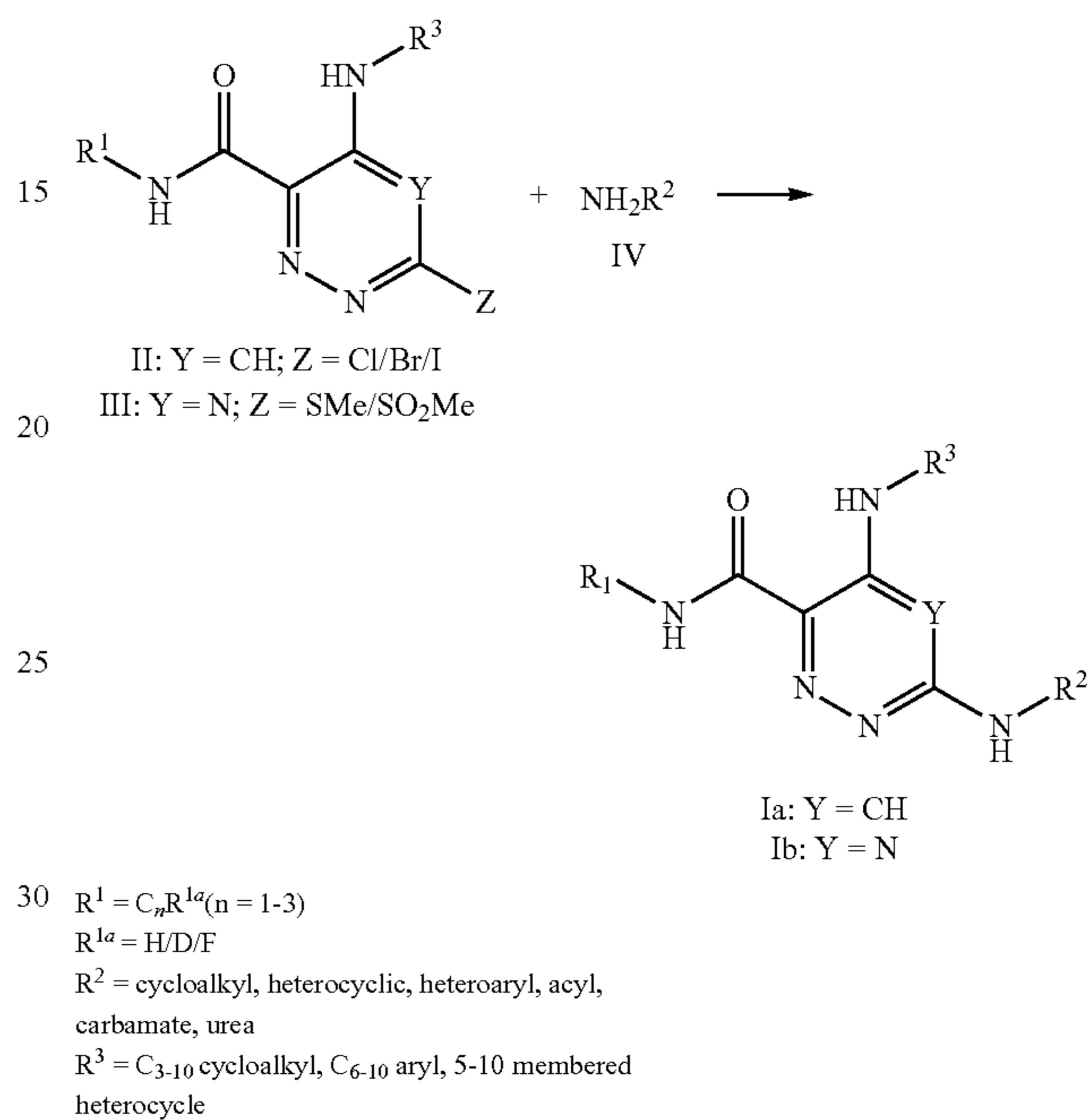
Scheme 1. Coupling of II/III with amine IV
