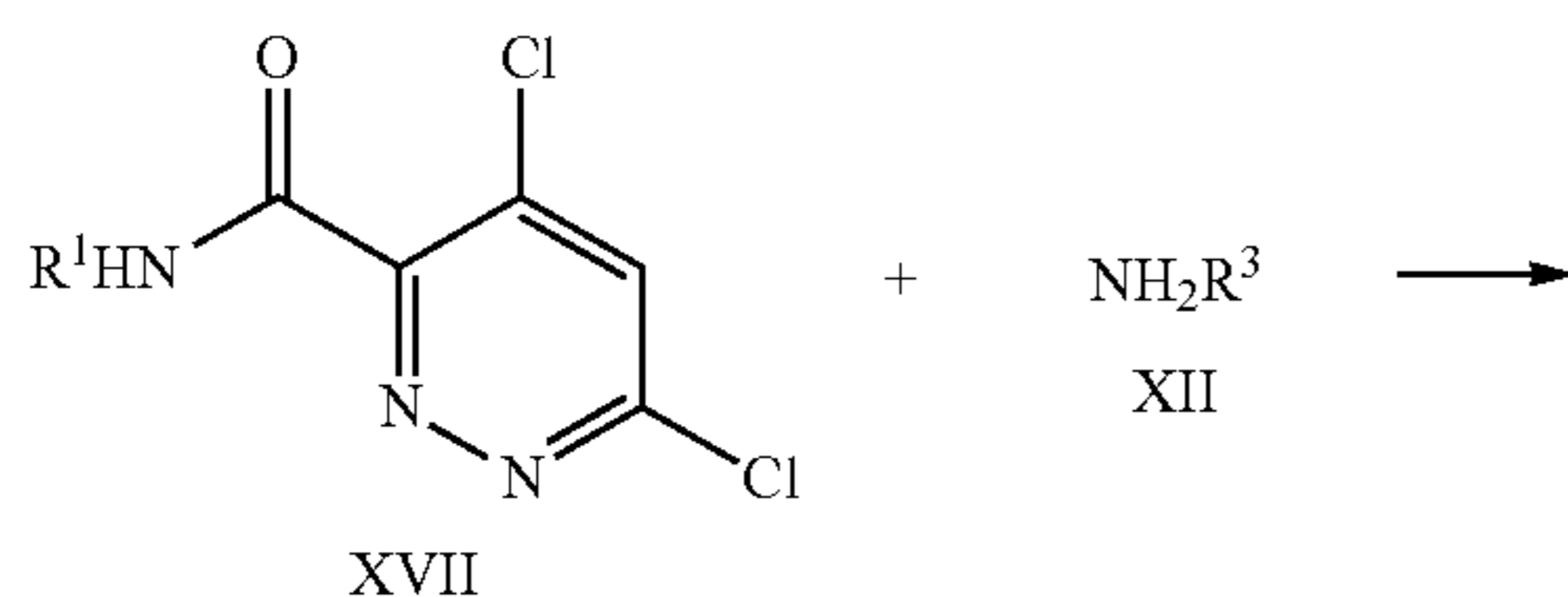
Scheme 7. Preparation of II
