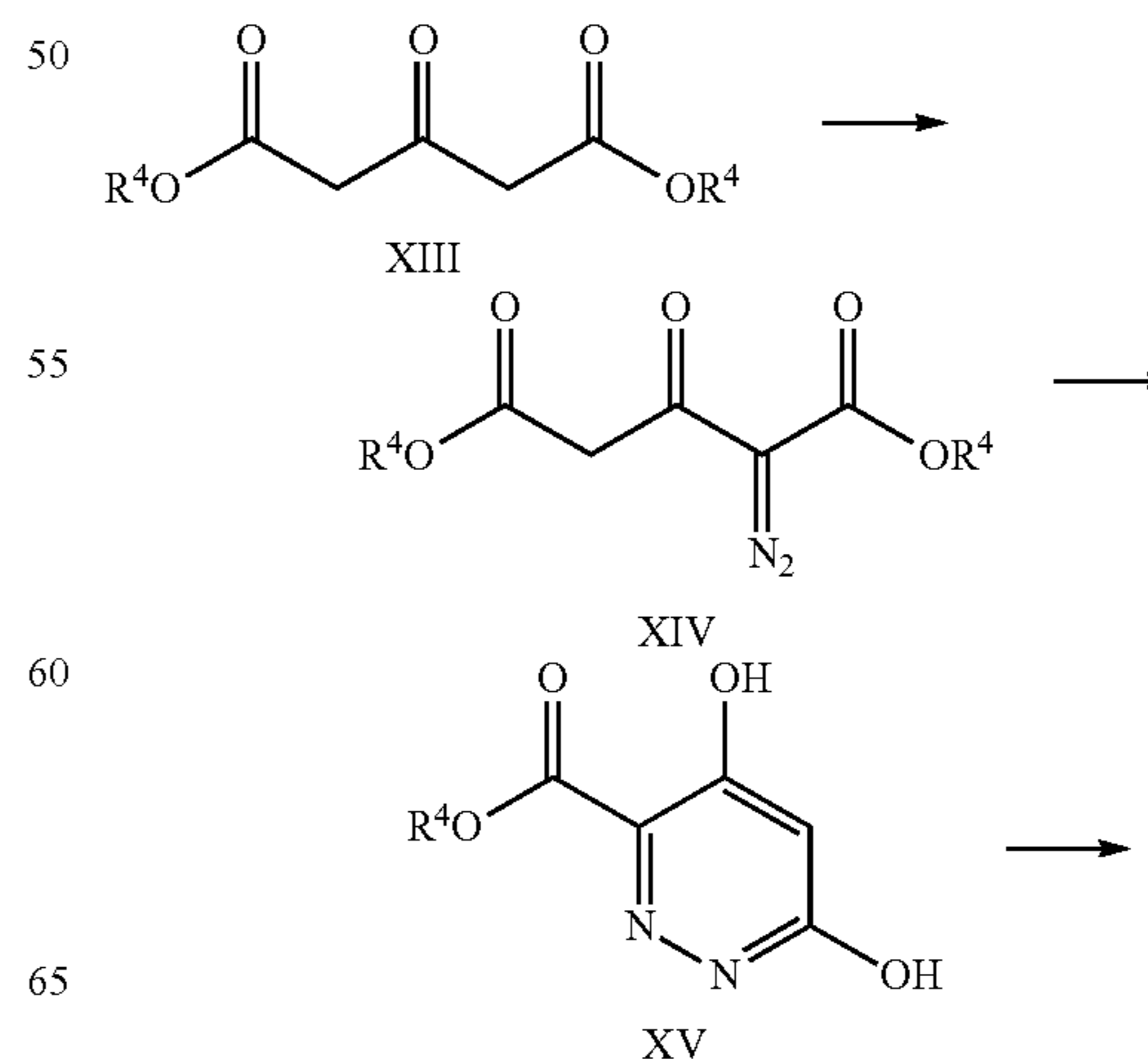
Scheme 5. Preparation of X
