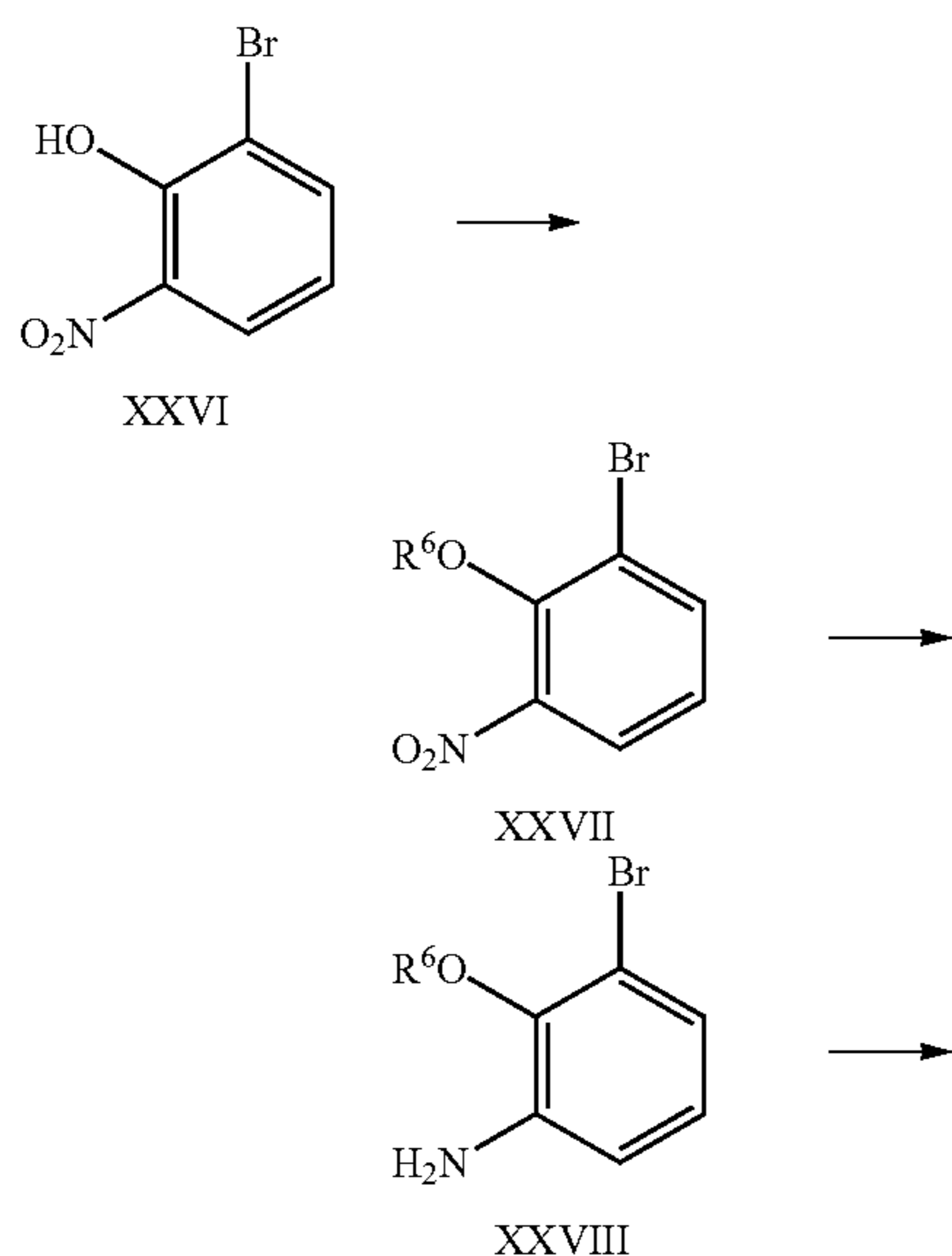
Scheme 10. Synthesis of anilines XII
