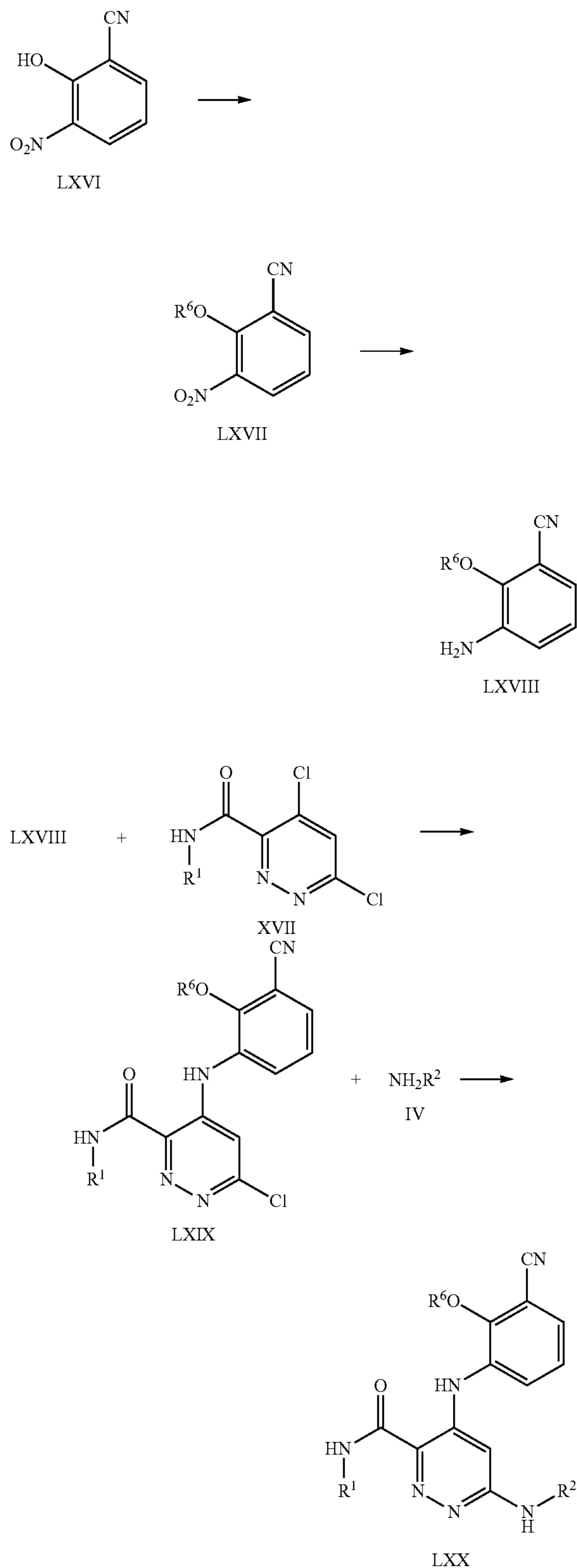
Scheme 18. Synthesis of LXXI
