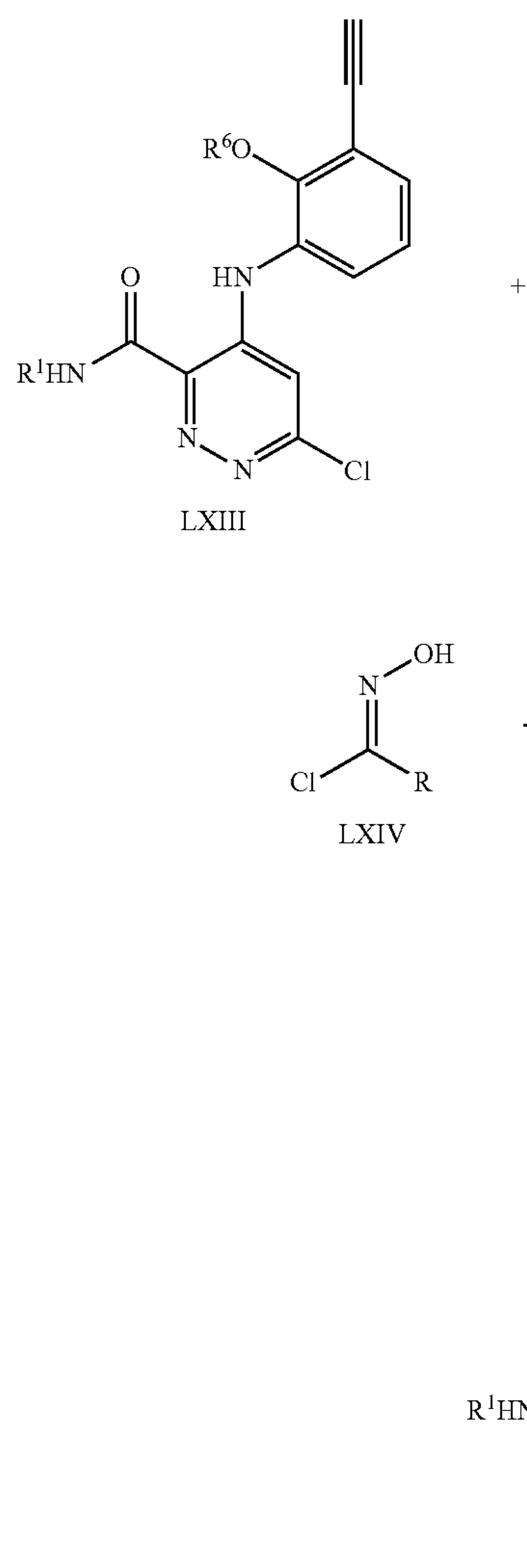
Scheme 17. Synthesis of LXV
