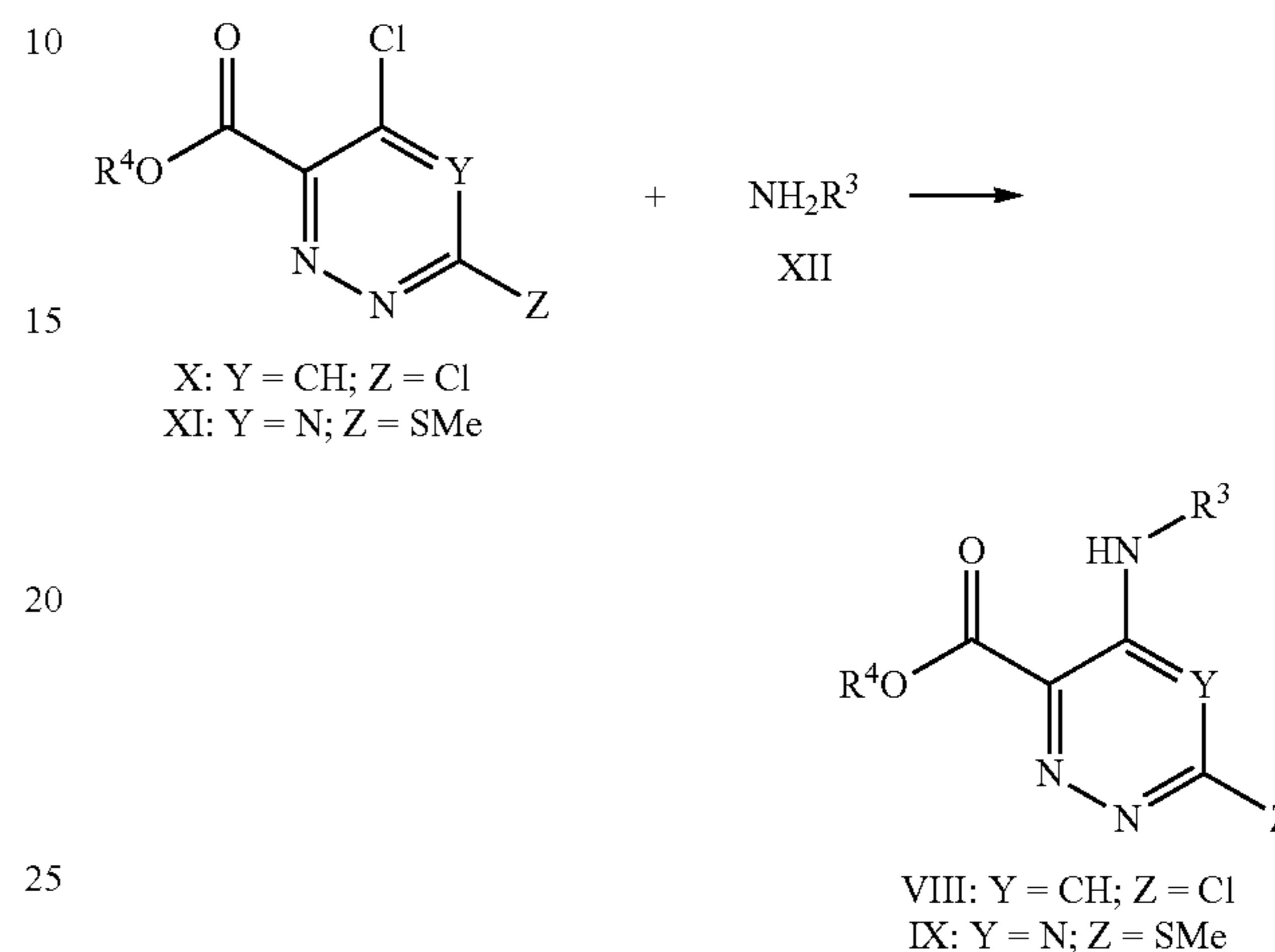
Scheme 4. Coupling of chlorides X/XI with amine XII
