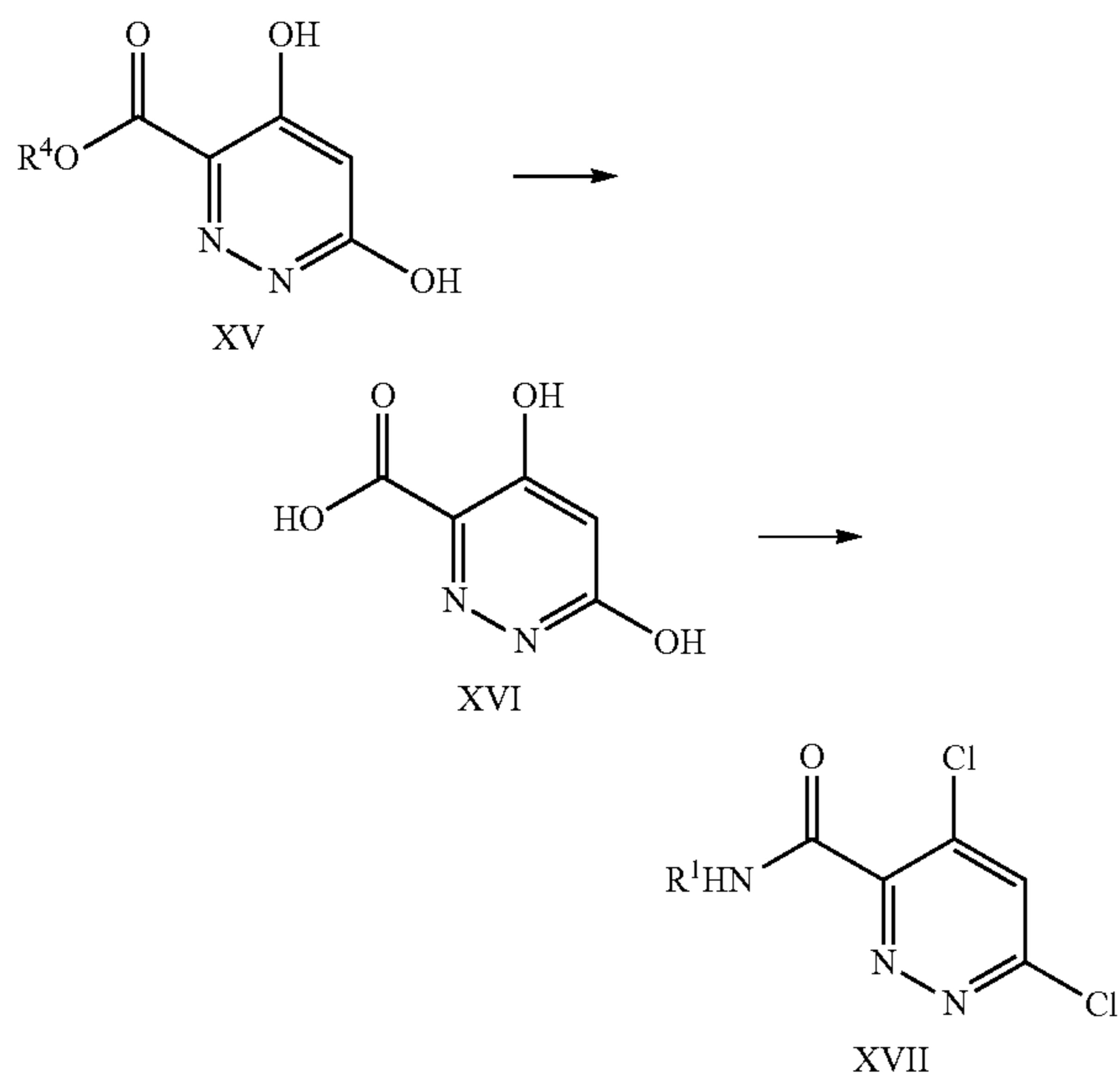
Scheme 6. Preparation of XVII
