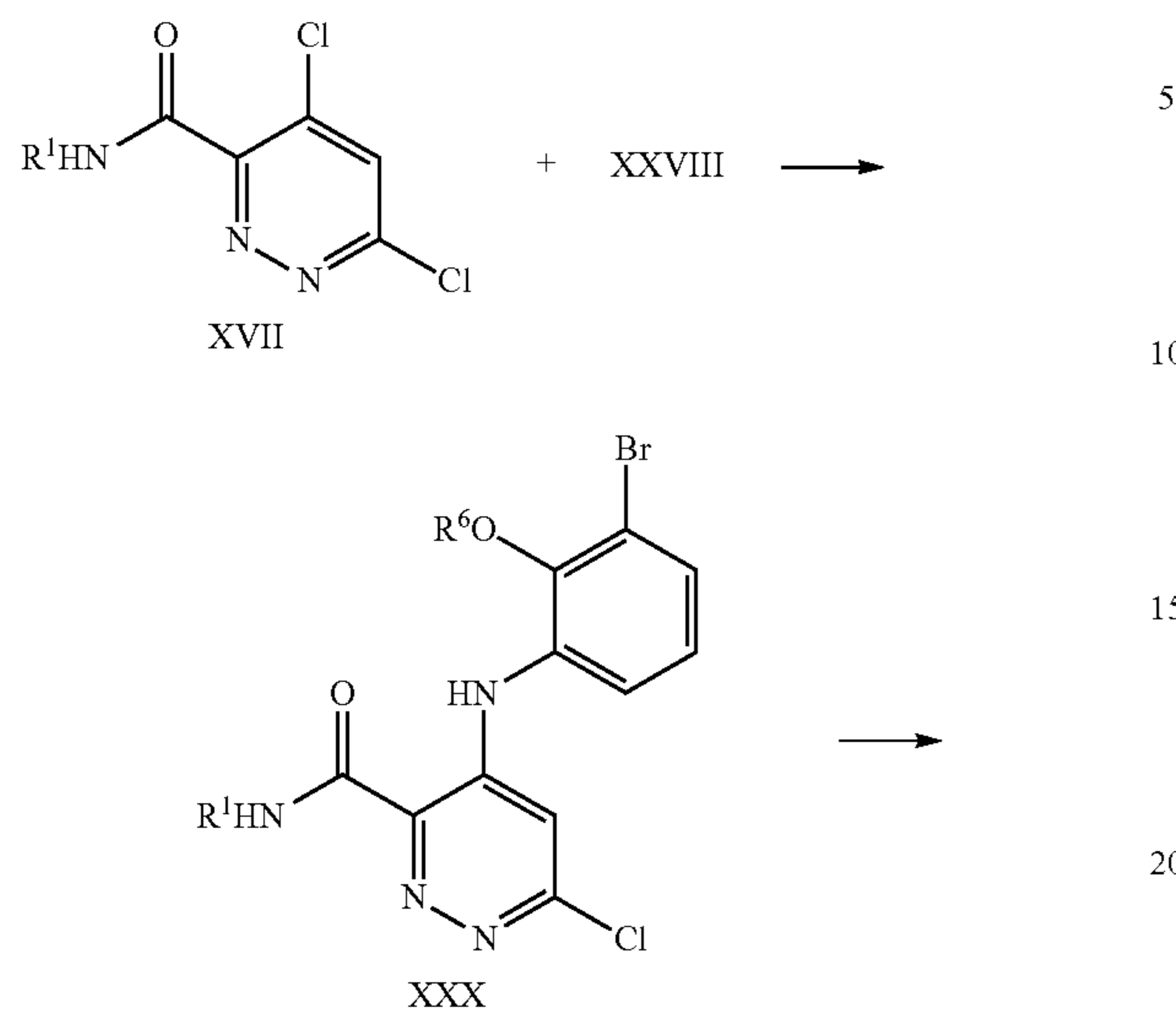
Scheme 11. Alternative preparation of I
