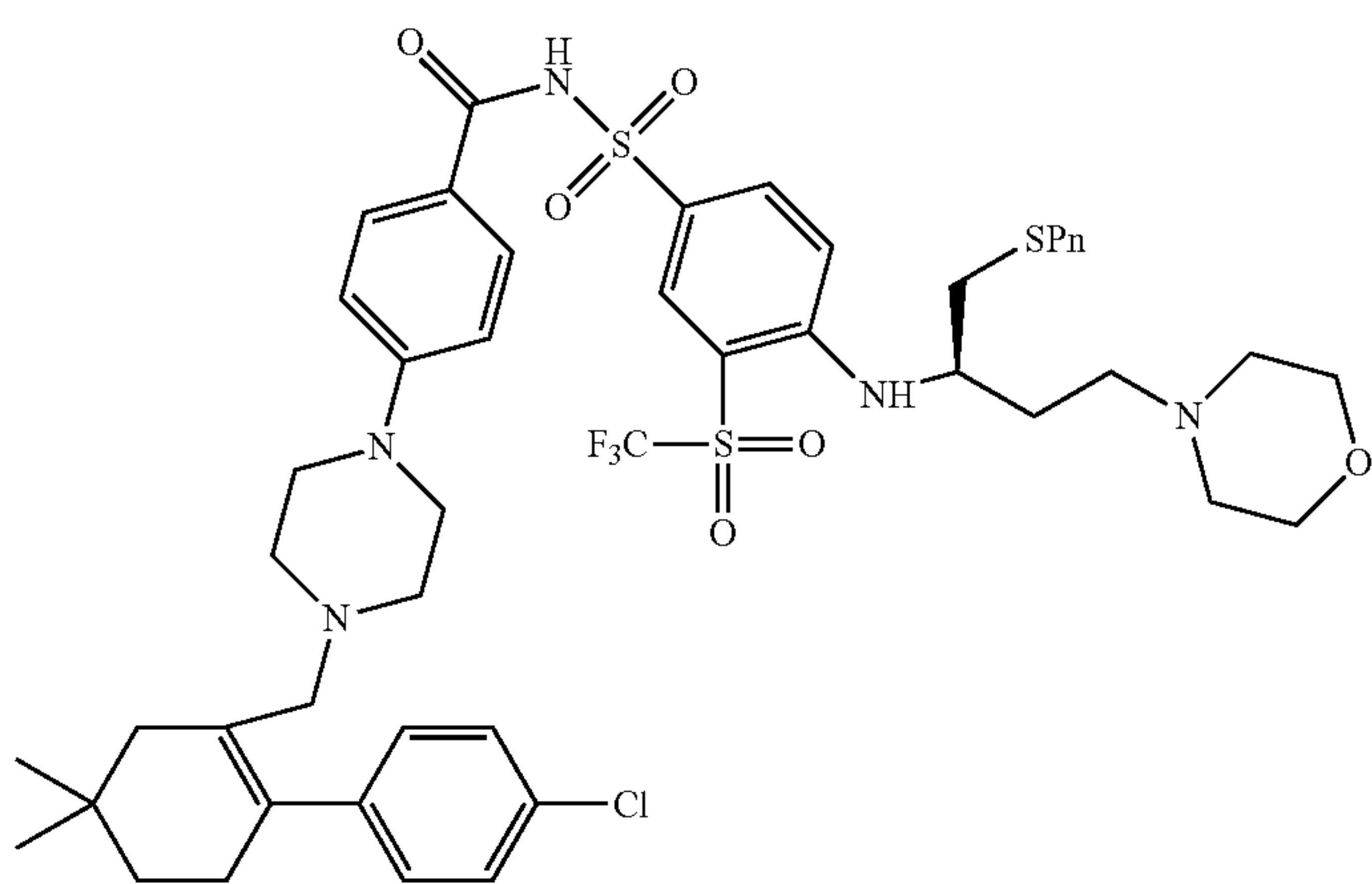
(ABT-263, Navitoclax)
