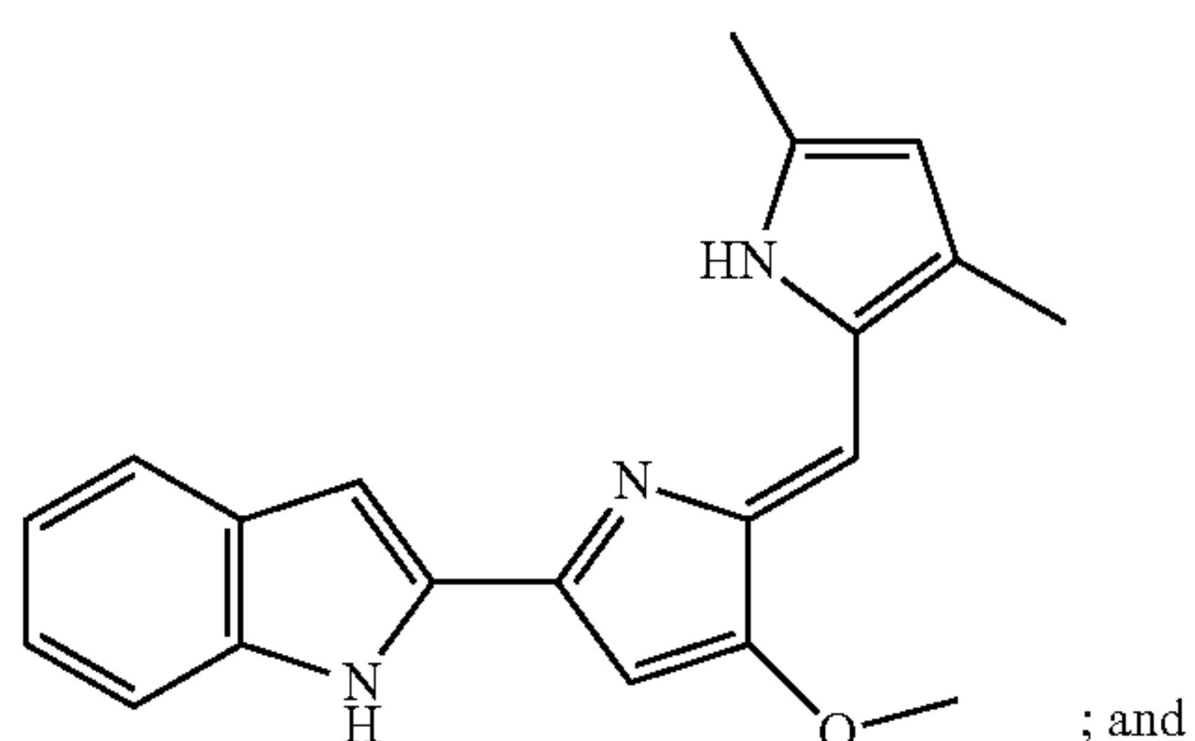
(GX15-070, Obatoclox)
