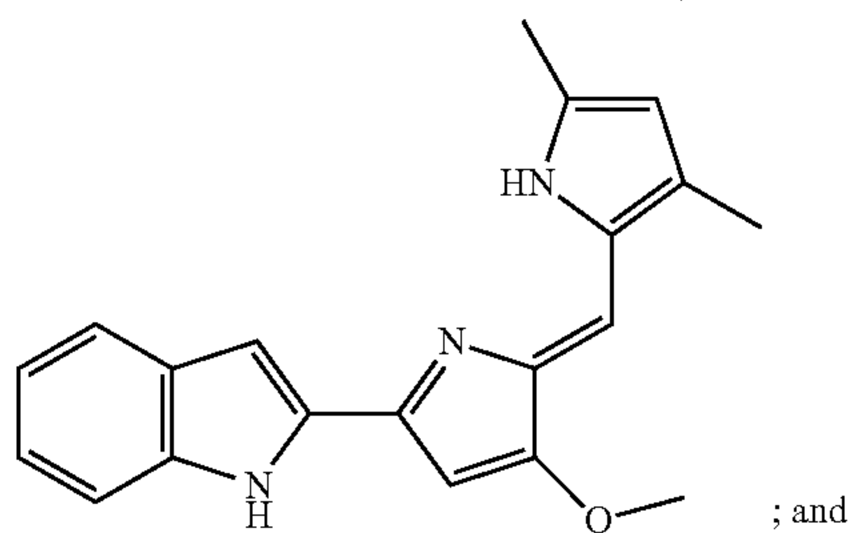
(GX15-070, Obatoclox)
