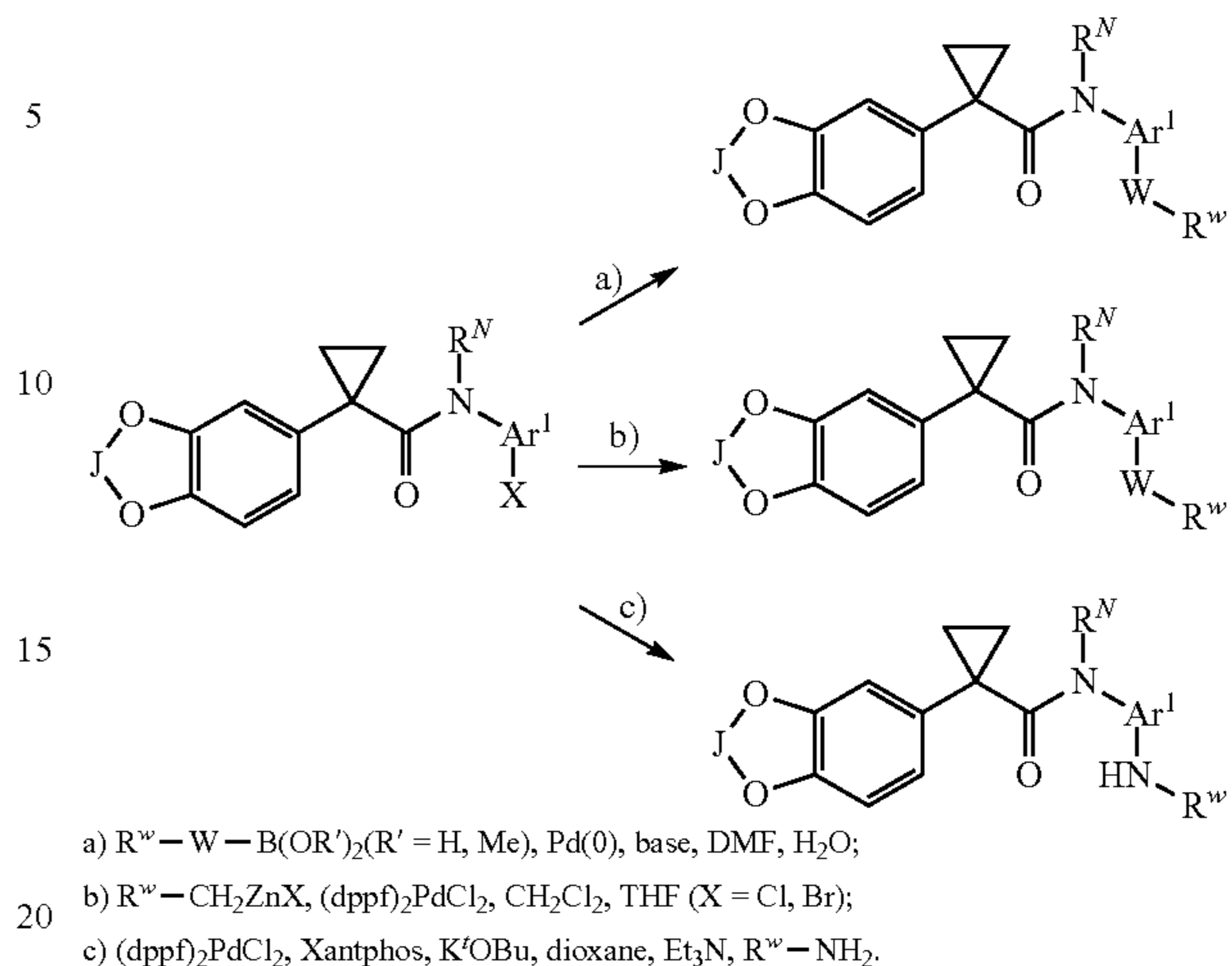
Scheme III - Derivatization of heteroarylhalides
