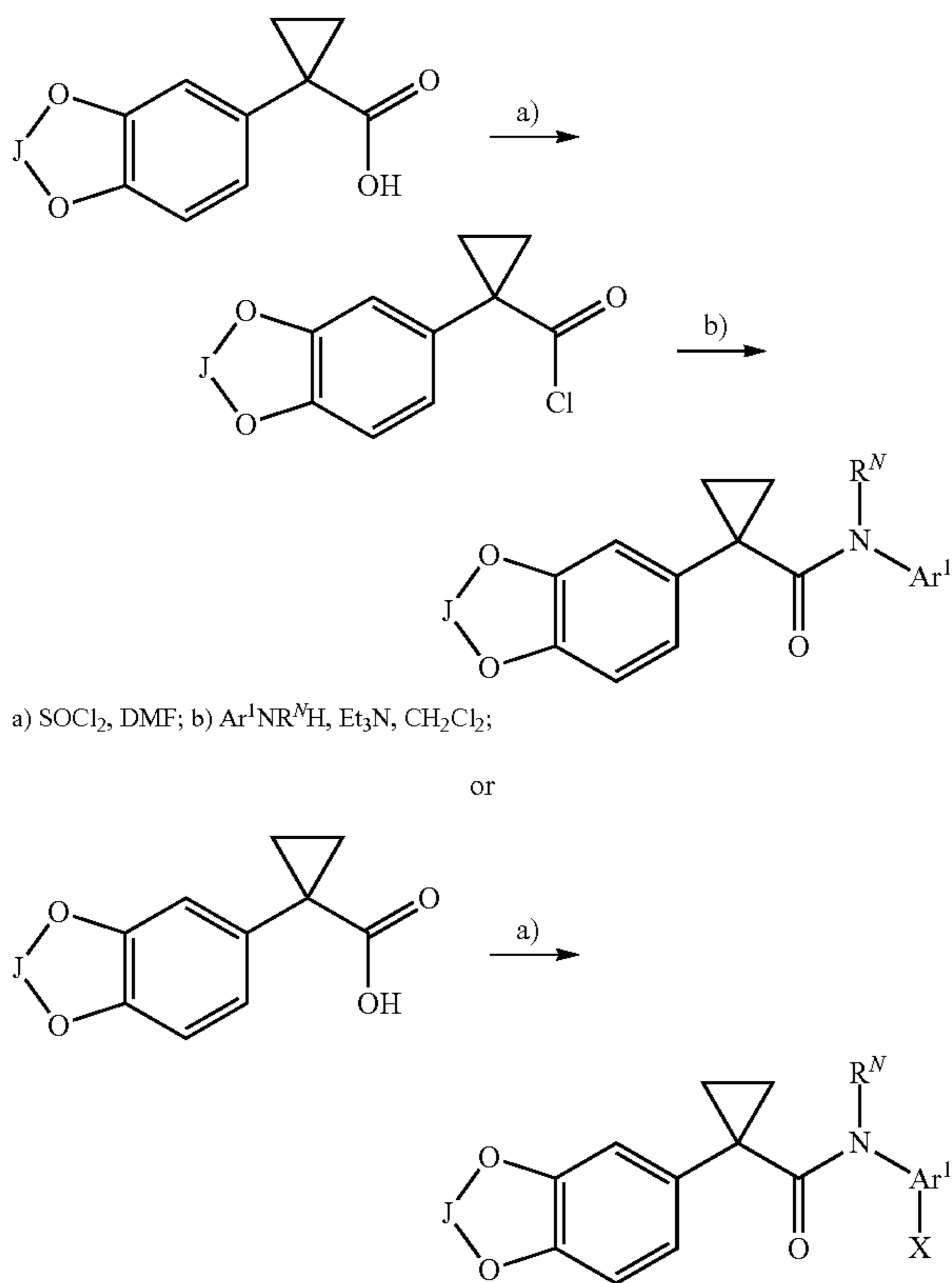
Scheme II - Amid coupling.
