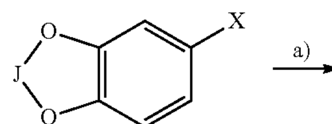
Scheme I - Preparation of cycloalkyl acids.
