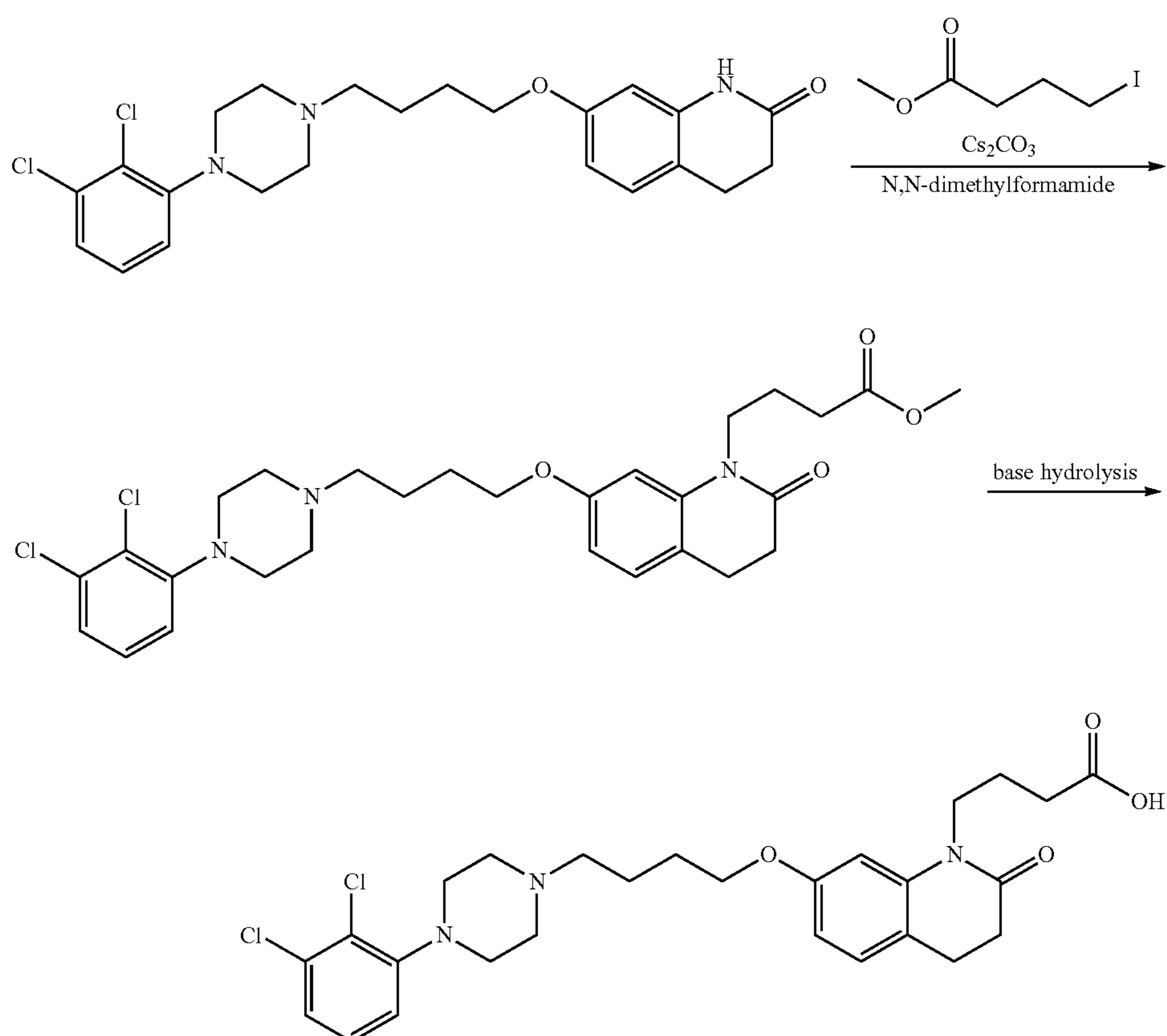
Scheme 7
