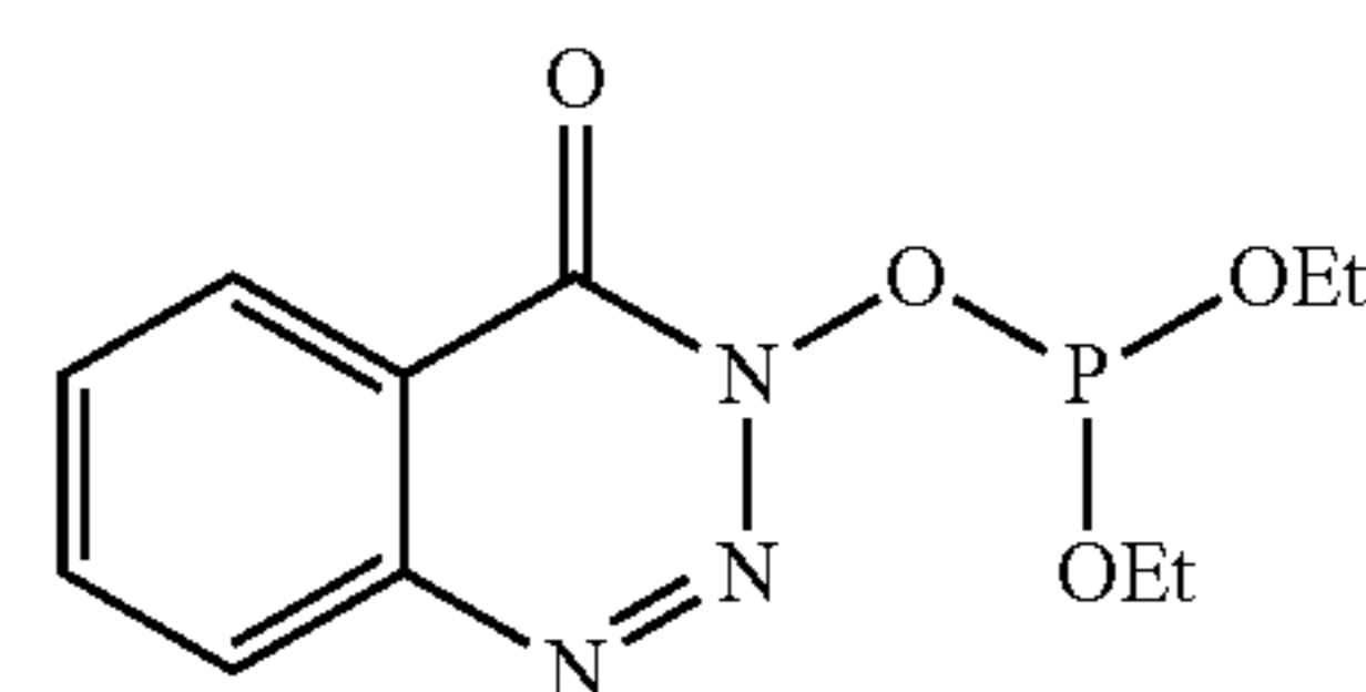
DEPT
