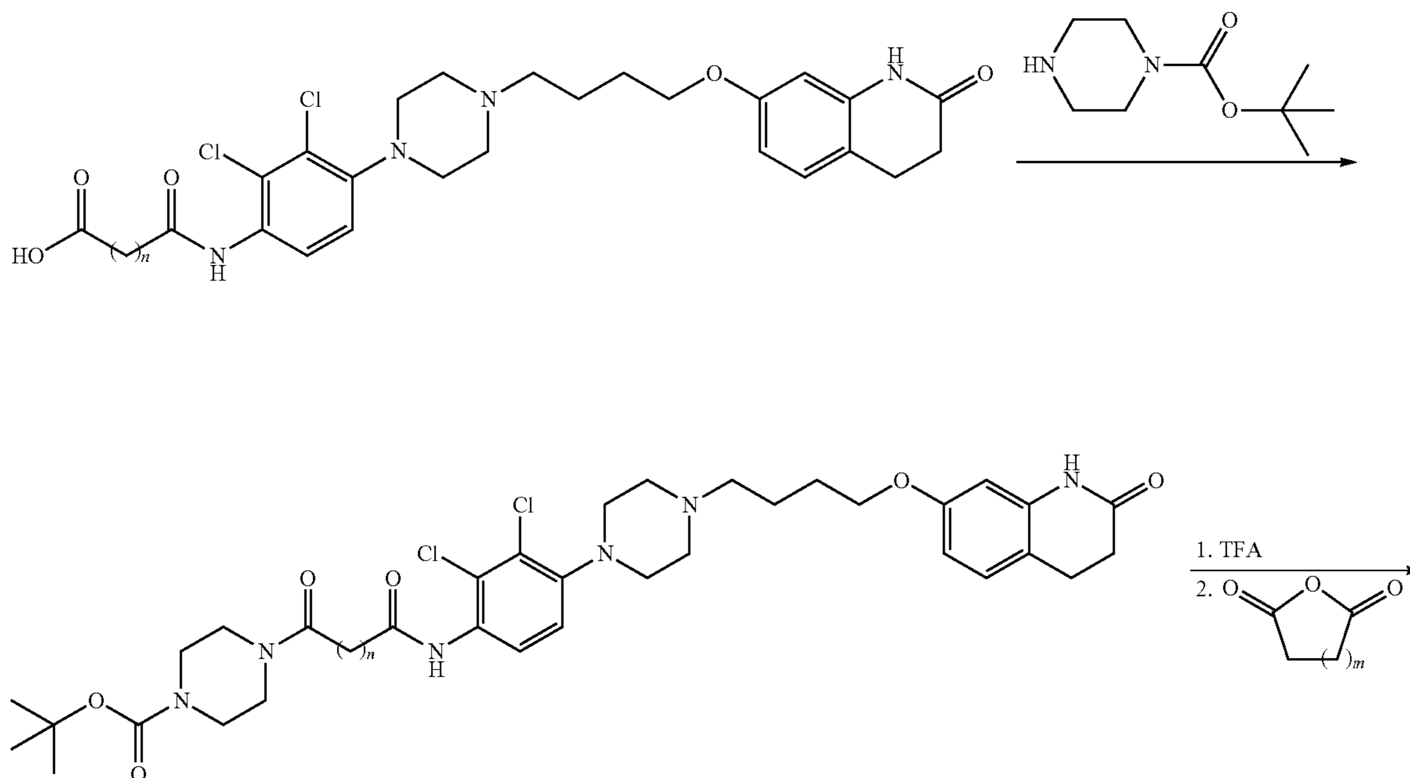
Scheme 5
