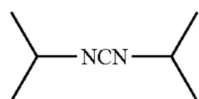
diisopropylcarbodiimide (DIC)
