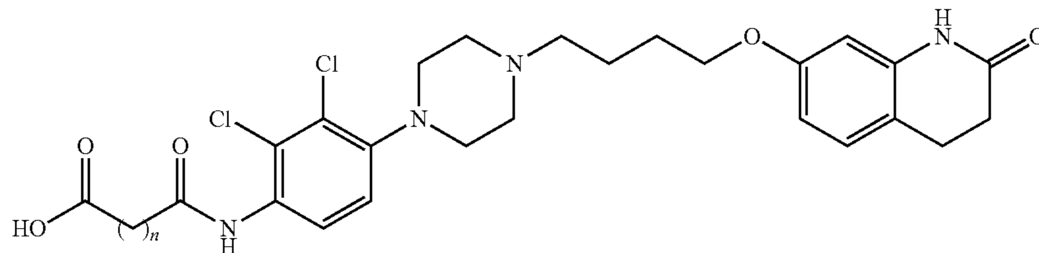
Example 2
