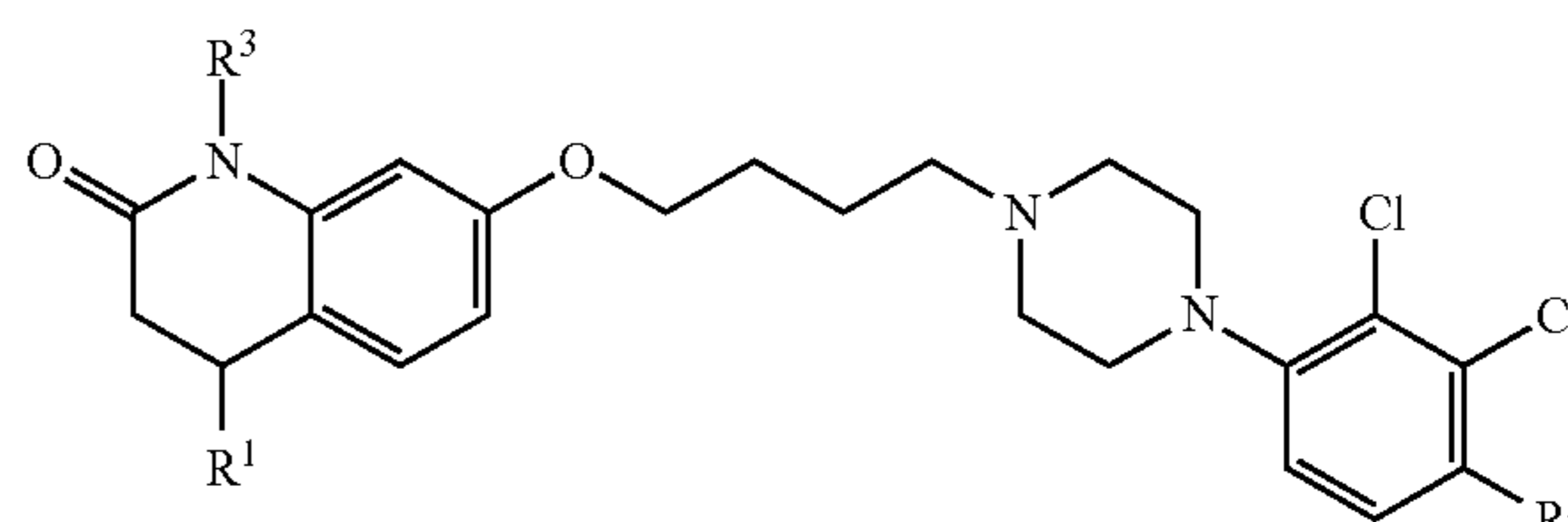
Formula I
