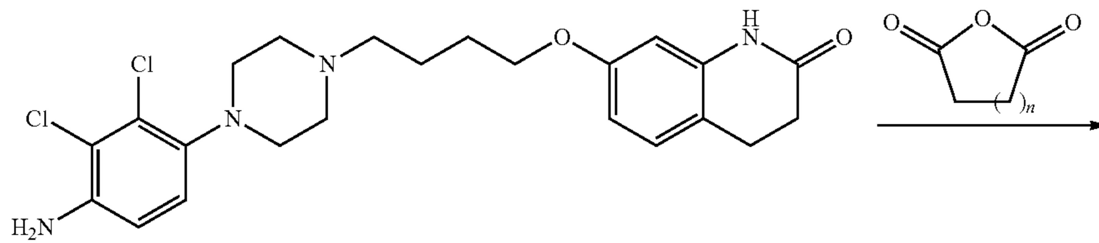
Example 2
