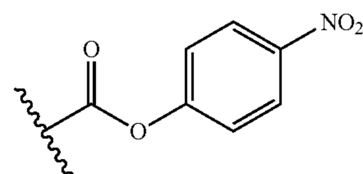
PNP
