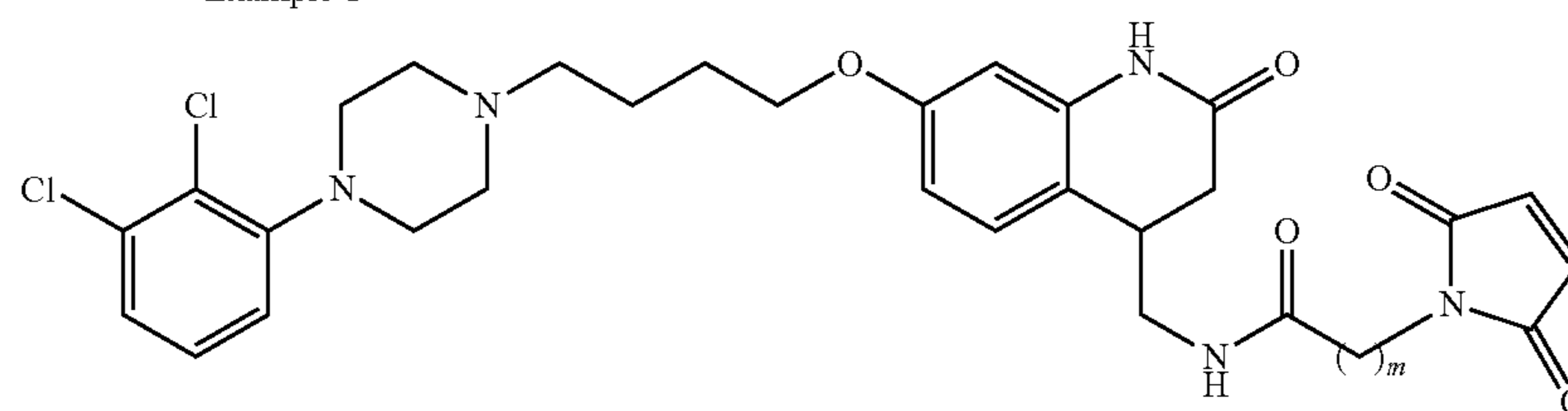
Example 1
