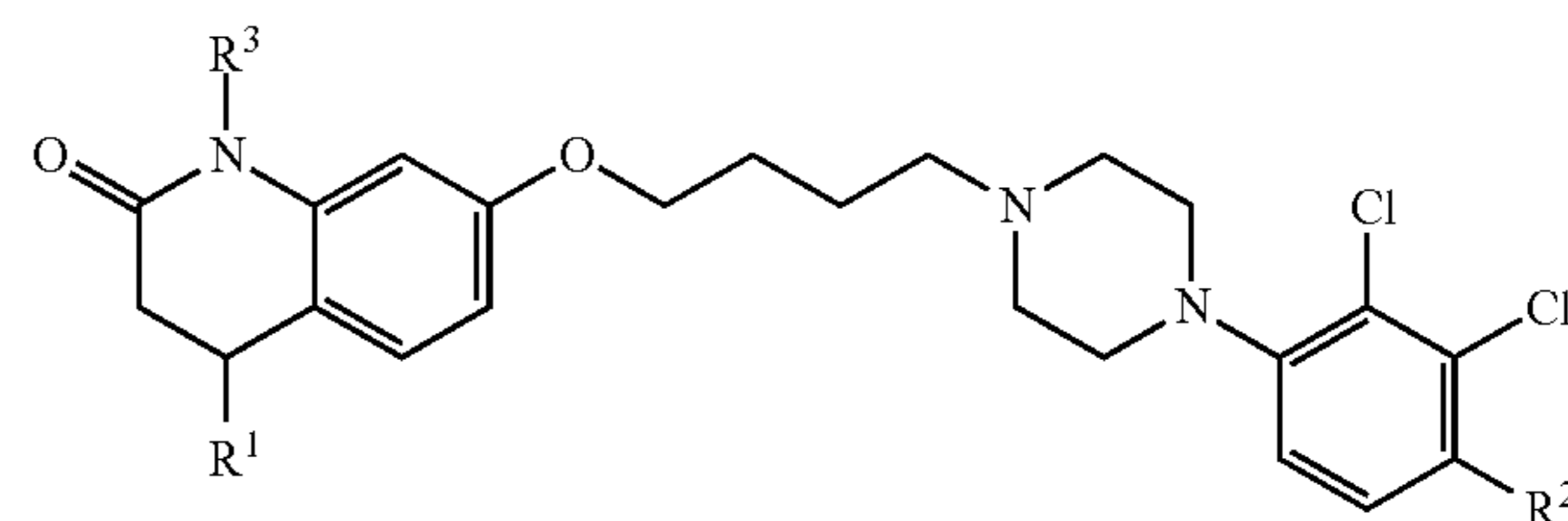
Formula I
