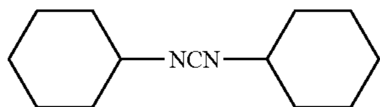
Dicyclohexylcarbodiimide (DCC)
