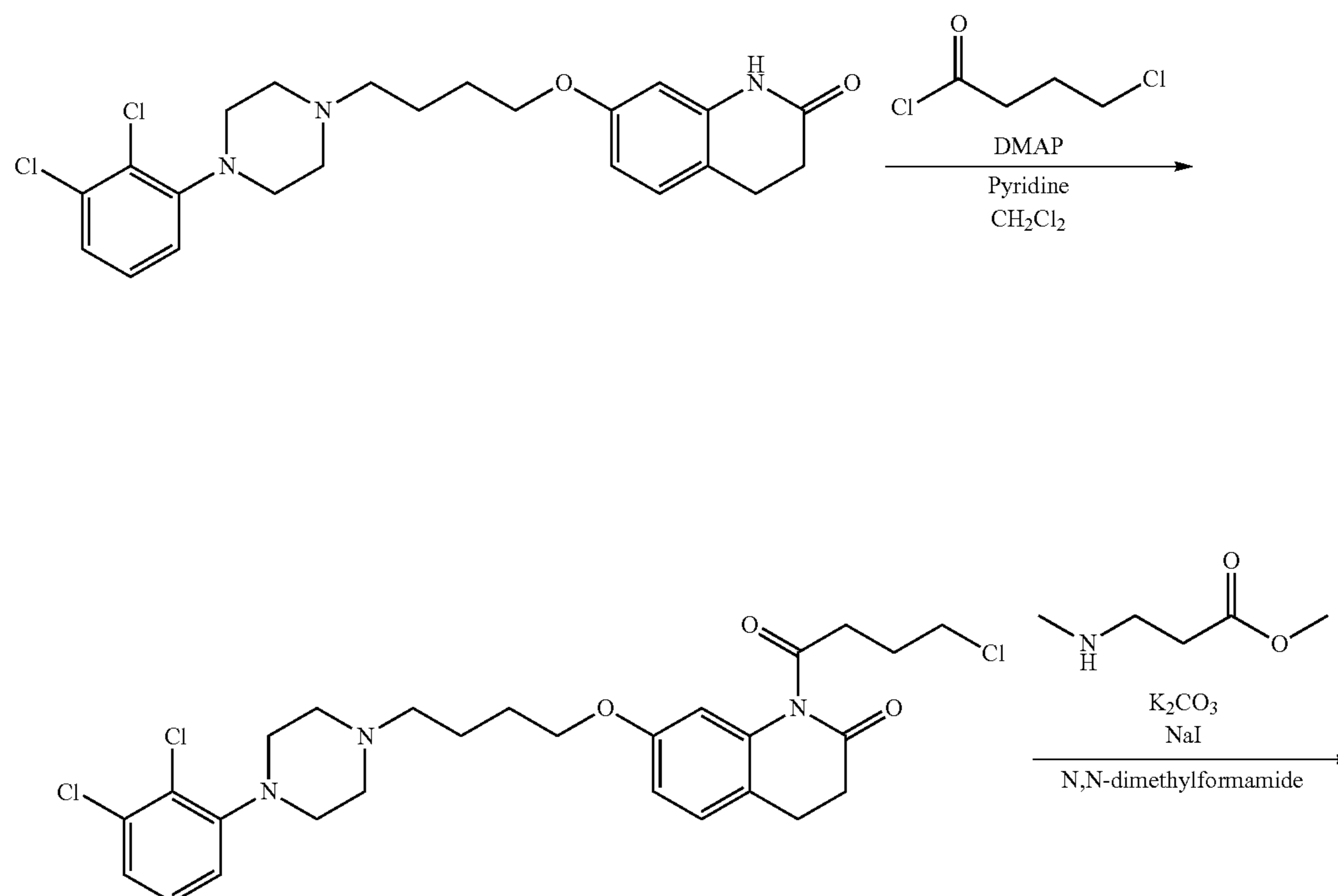
Scheme 6
