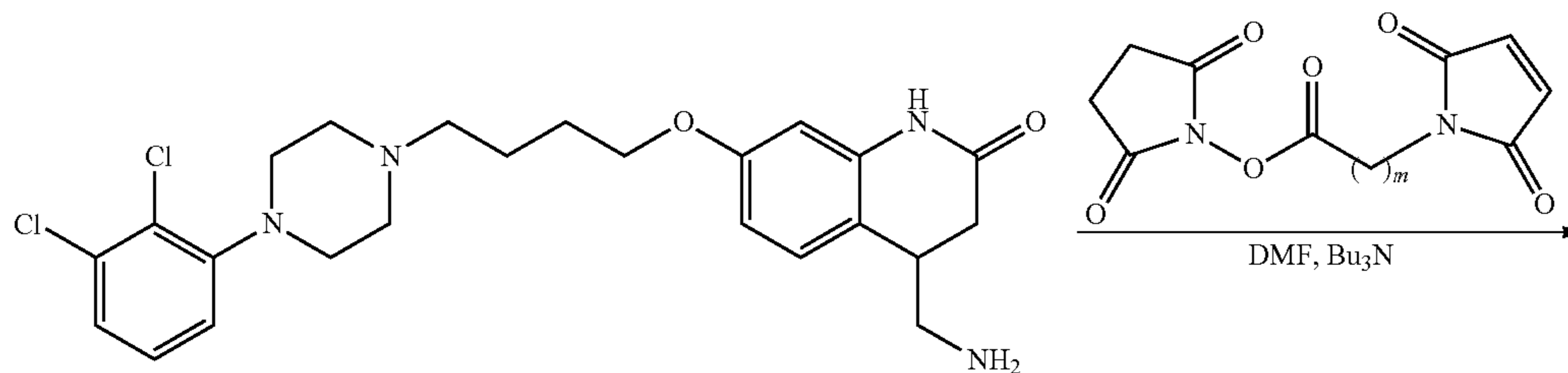
Example 1
