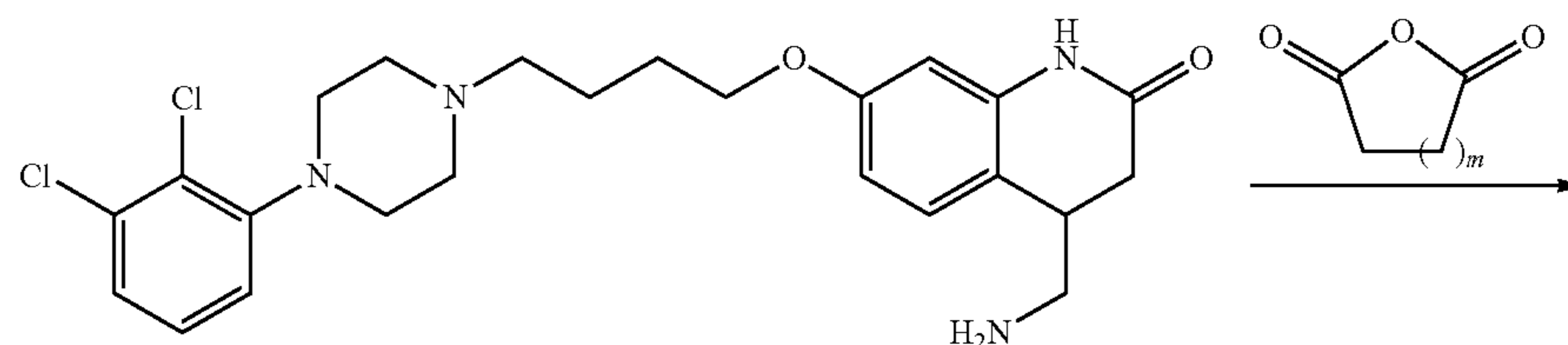
Example 1
