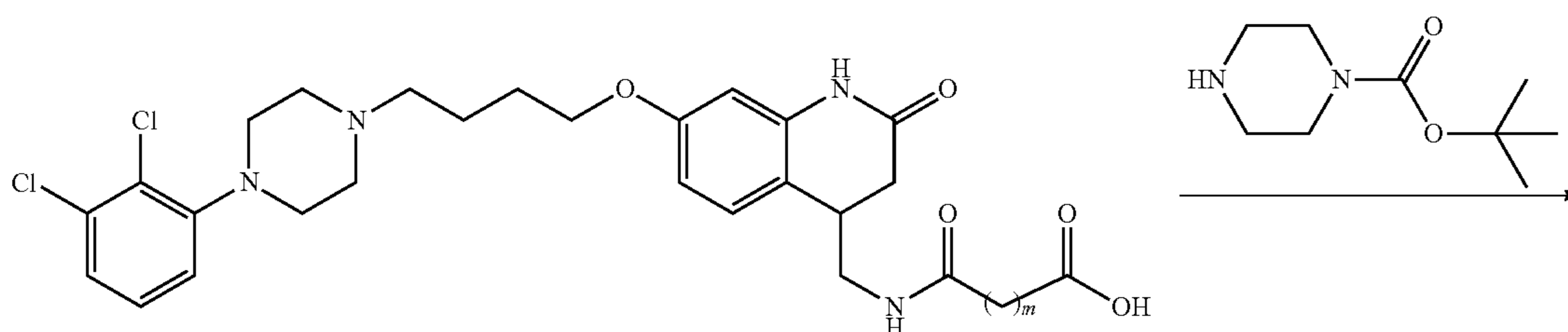
Scheme 4
