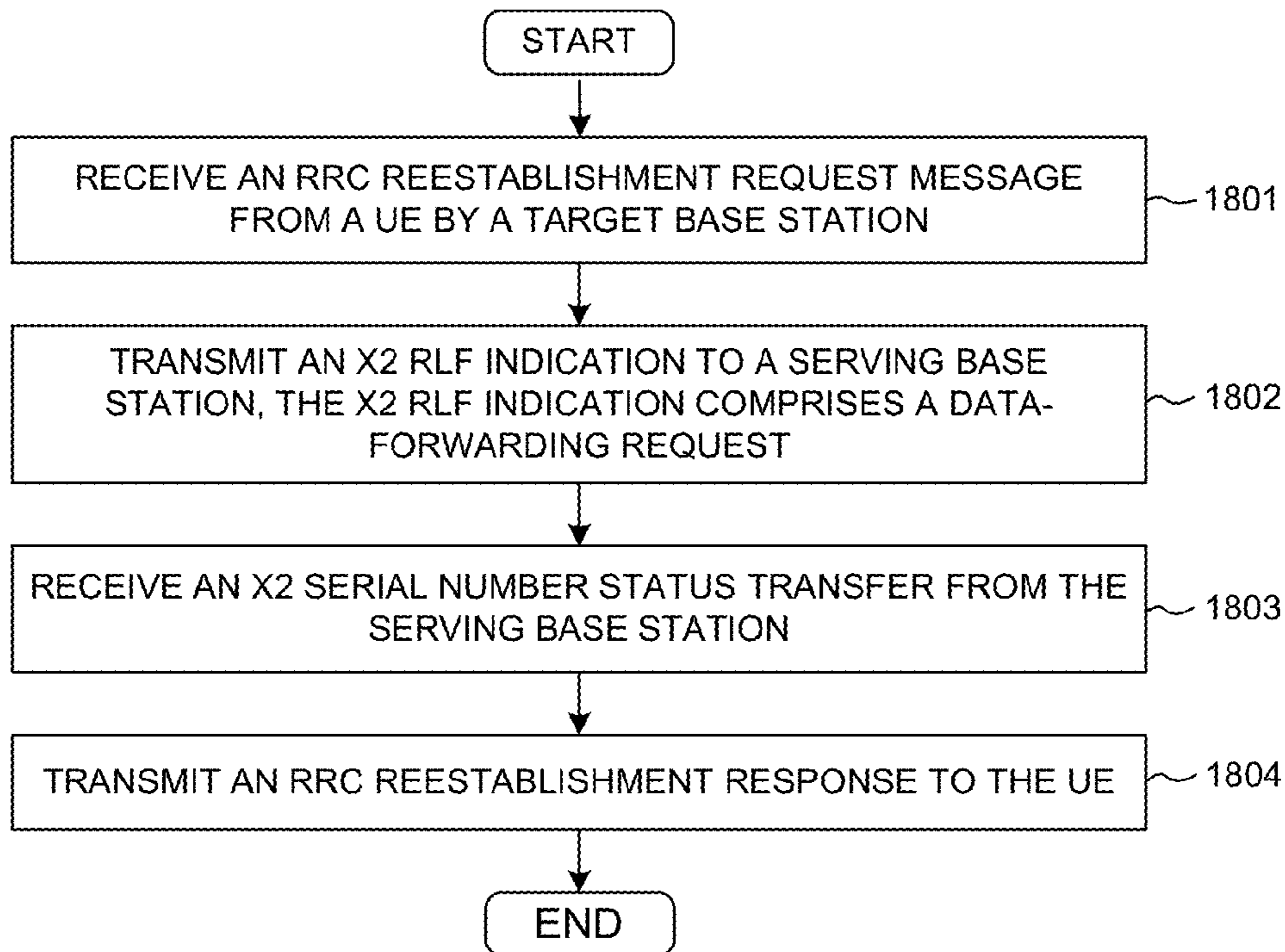
LOSS-LESS RECOVERY FIG. 18
