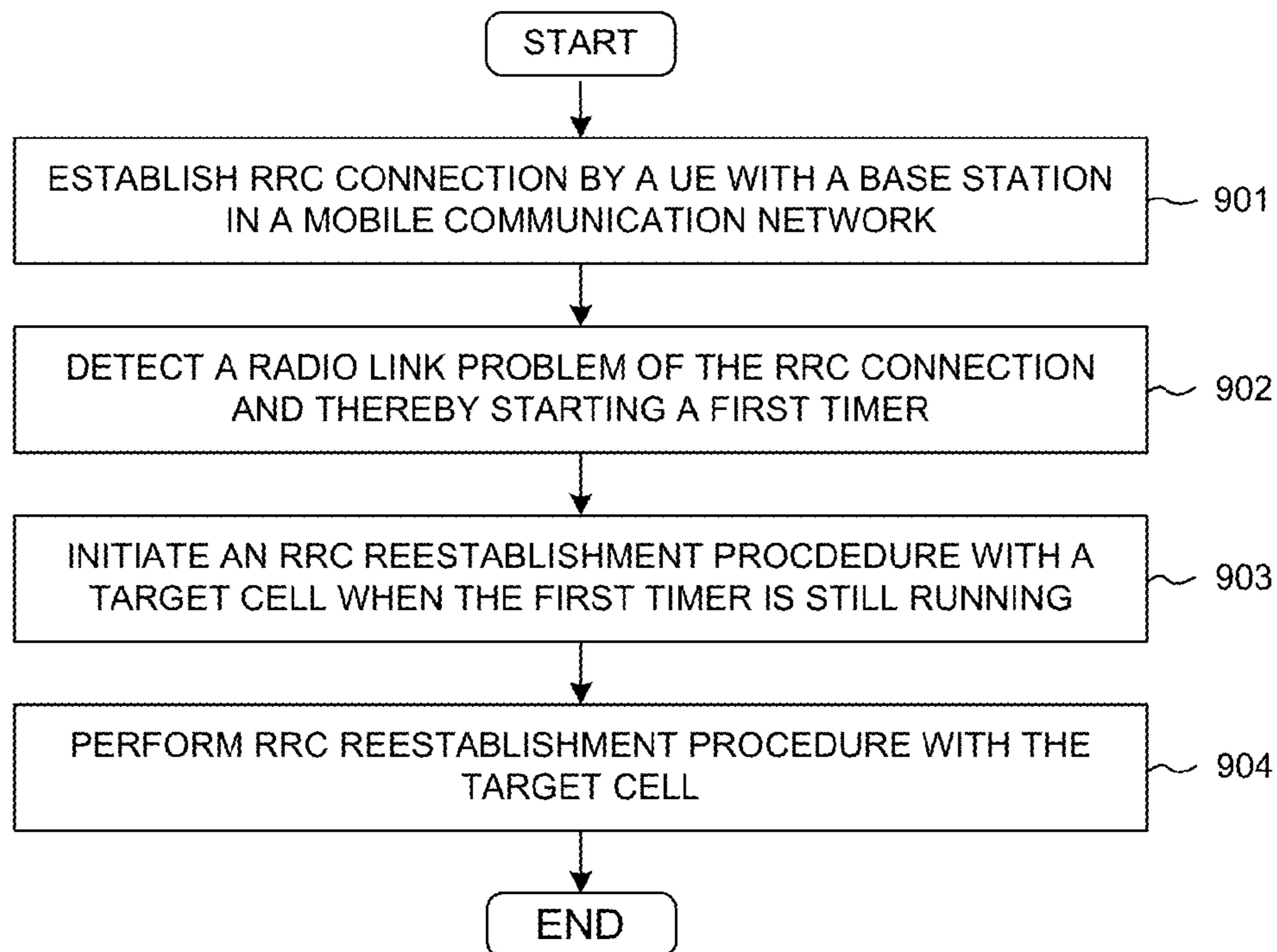
FAST RADIO LINK FAILURE
