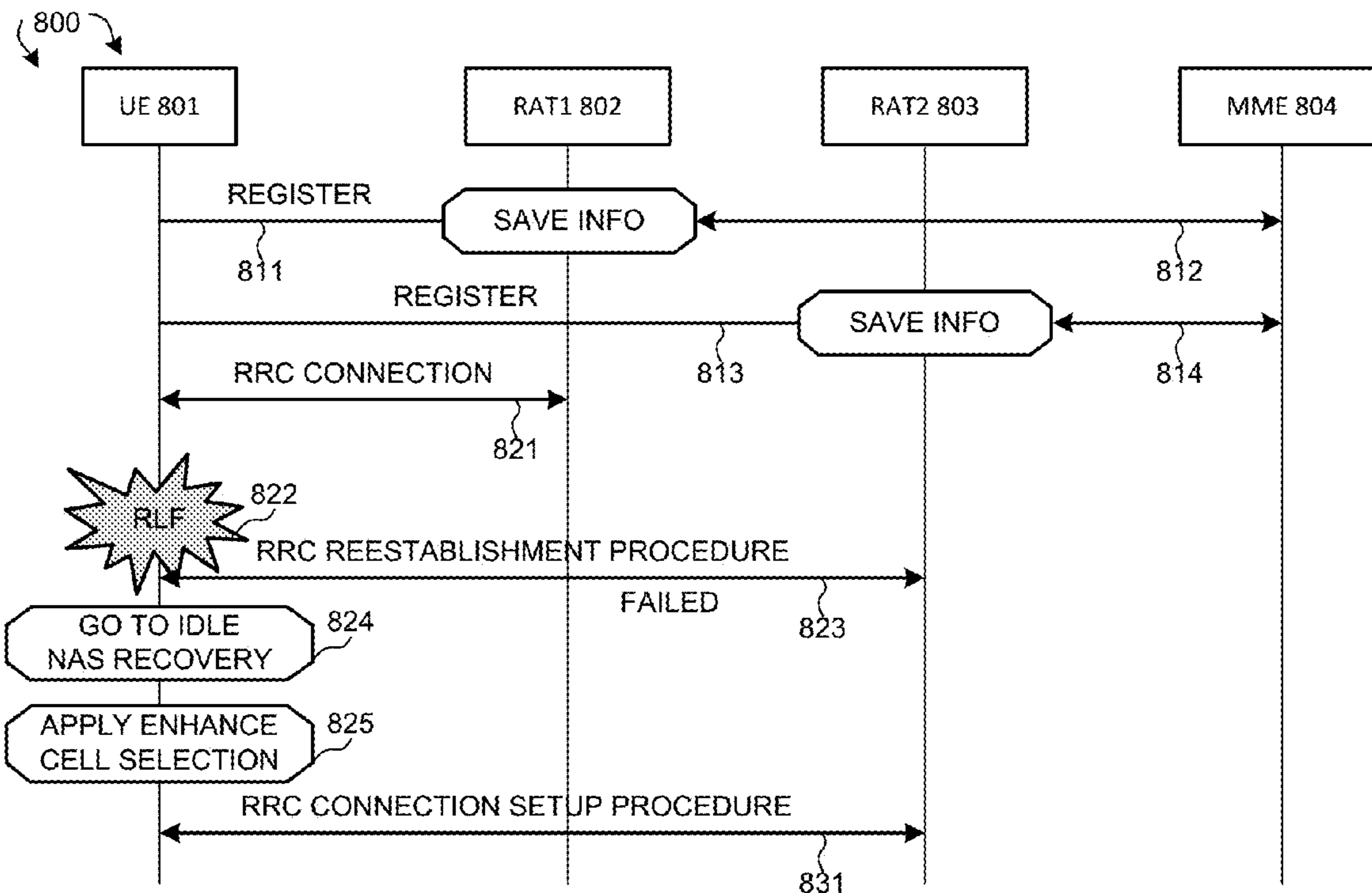
ENHANCED IRAT MULTI-REGISTRATION FIG. 8
