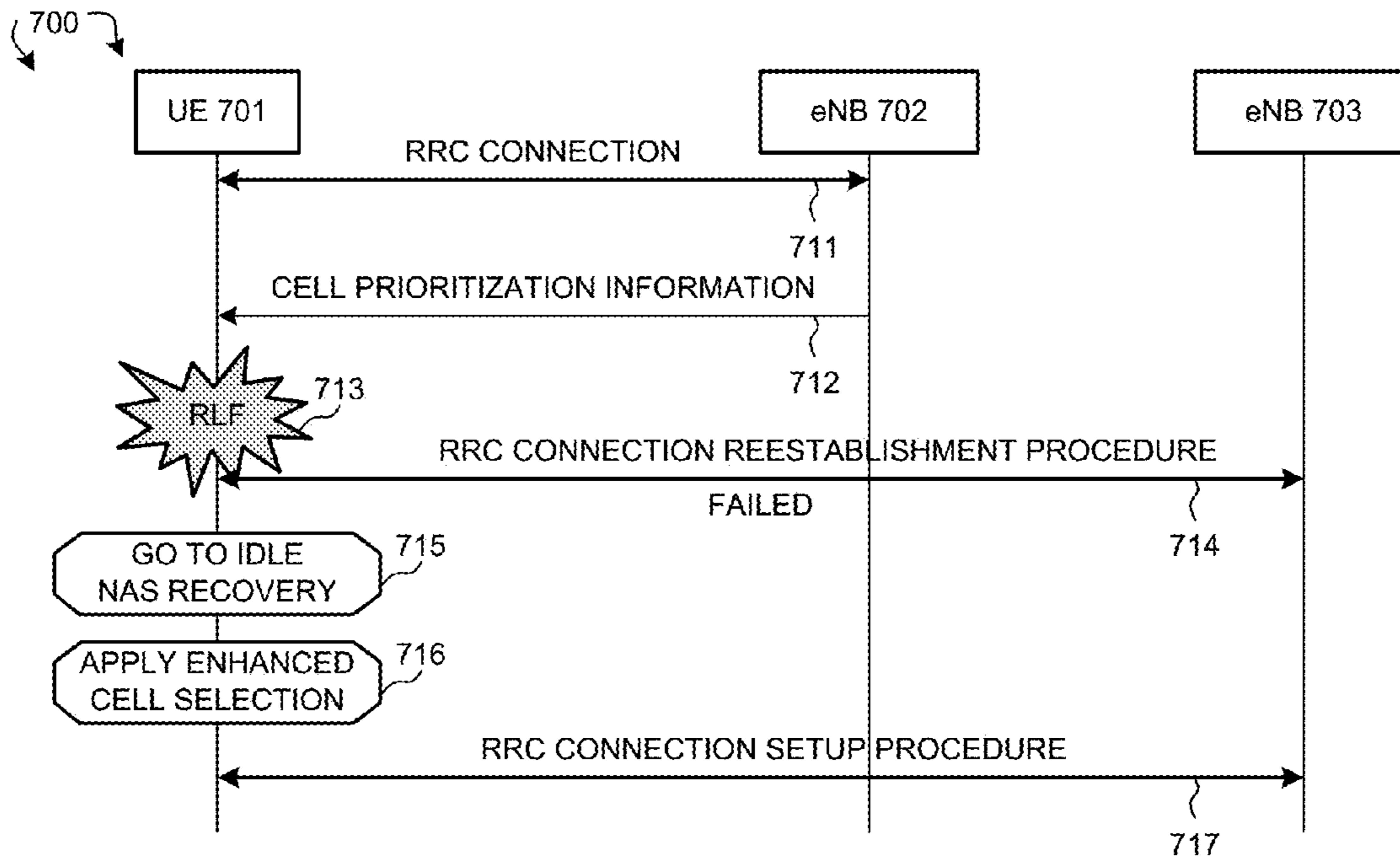
CELL SELECTION WITH PRIORITIZATION FIG. 7
