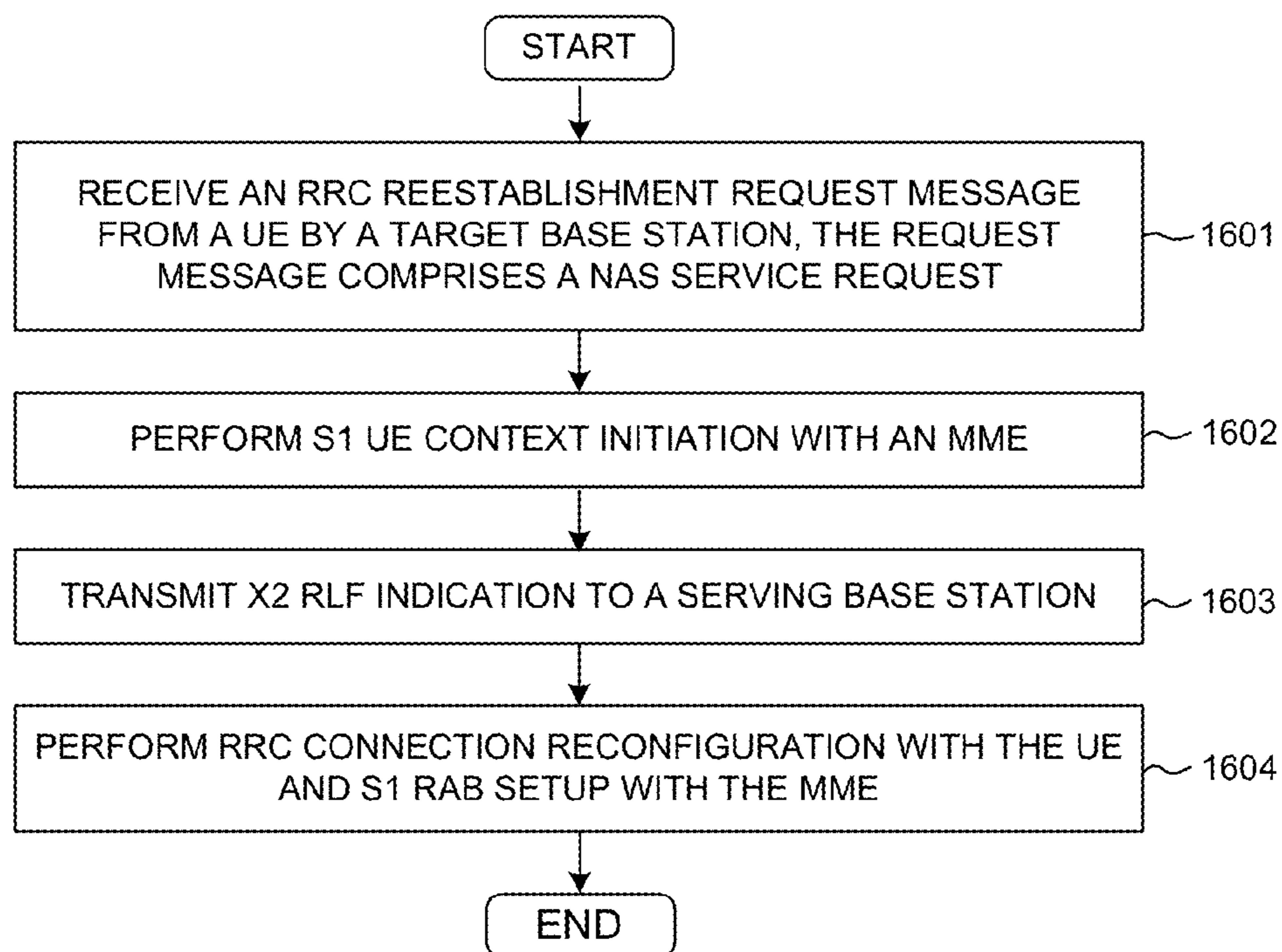
FAST NAS RECOVERY FIG. 16
