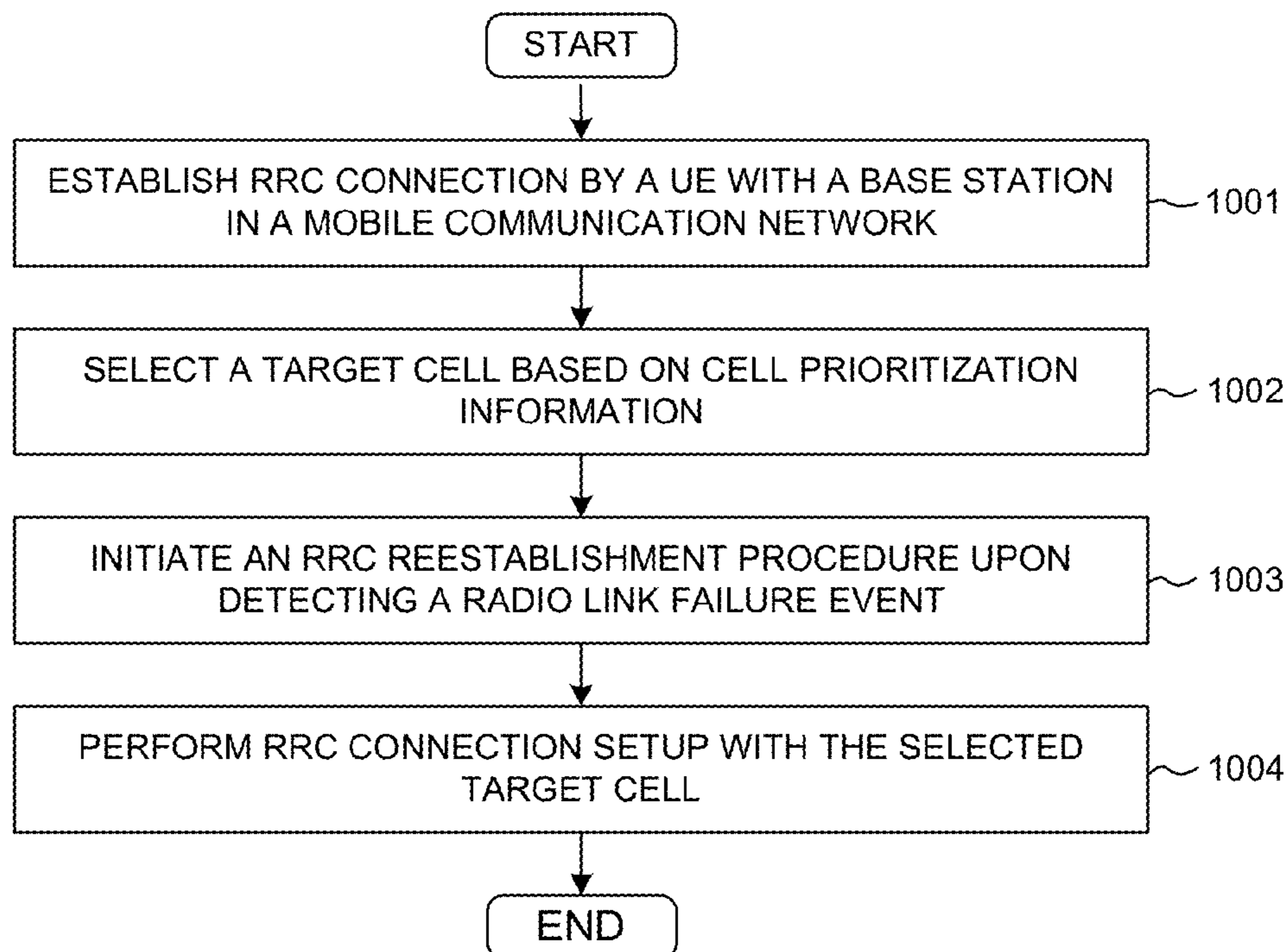
CELL SELECTION WITH PRIORITIZATION
