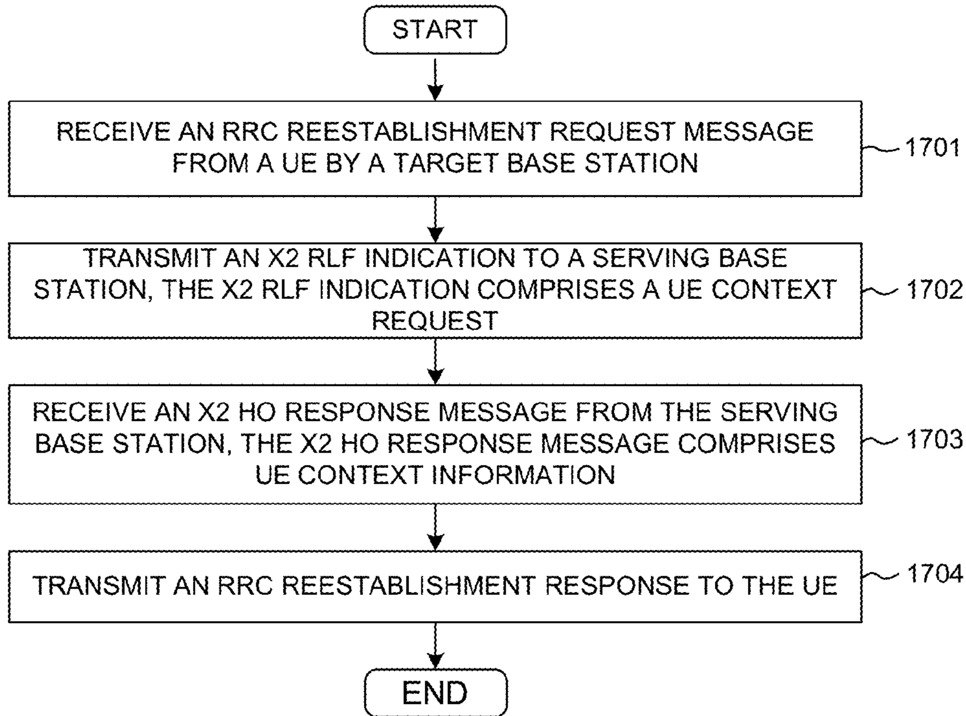
CONTEXT FETCH FIG. 17
