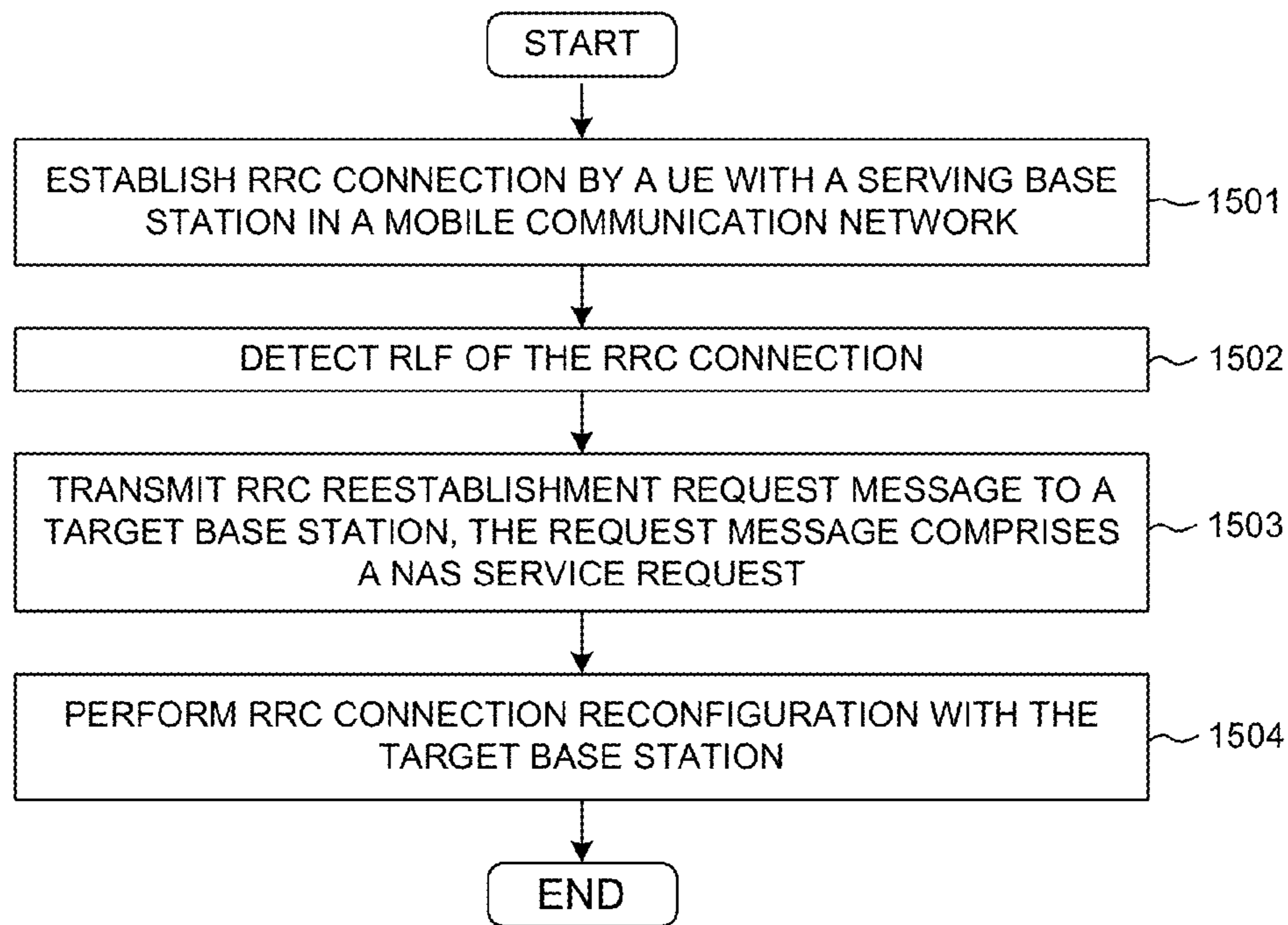
FAST NAS RECOVERY FIG. 15
